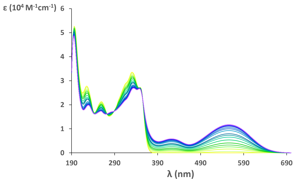
Figure S93. UV/Vis kinetic of L2-B in CH 3 CN irradiating at 370 nm, 5 \cdot 10^{-5} \text{M}
