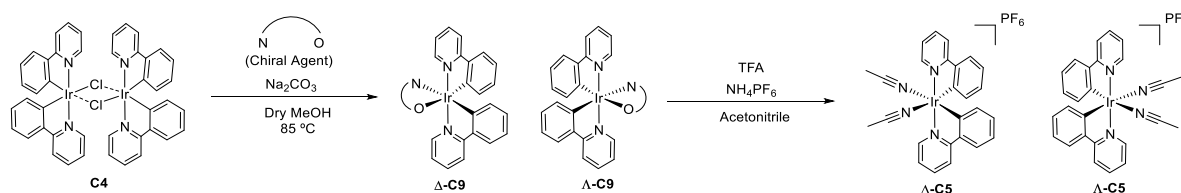
Scheme 4.6. Synthesis of \Lambda/\Delta -C5 enantiopure complexes.
