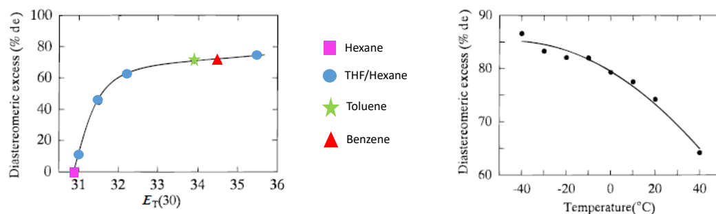
Figure 1.10. Left) Comparison of the effect of solvent polarity with the generation of diastereomers; Right) Comparison of the effect of temperature on the generation of diastereomers in toluene. 45
