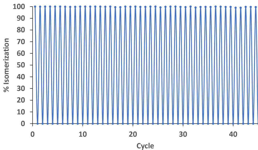
Figure S132. UV/Vis spectra of Ir-L3-A in CH 3 CN. Fatigue resistance experiment by irradiation at 370 nm, 2.7 \cdot 10^{-5} \text{M}
