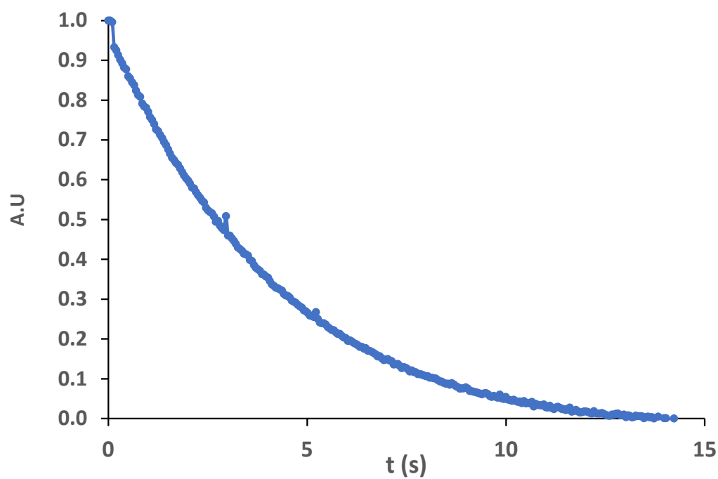
Figure S138. UV/Vis spectra of Ir-L3-B in CH 3 CN. Photocycloreversion process by irradiation at 370 nm, 1.9 \cdot 10^{-5} M
