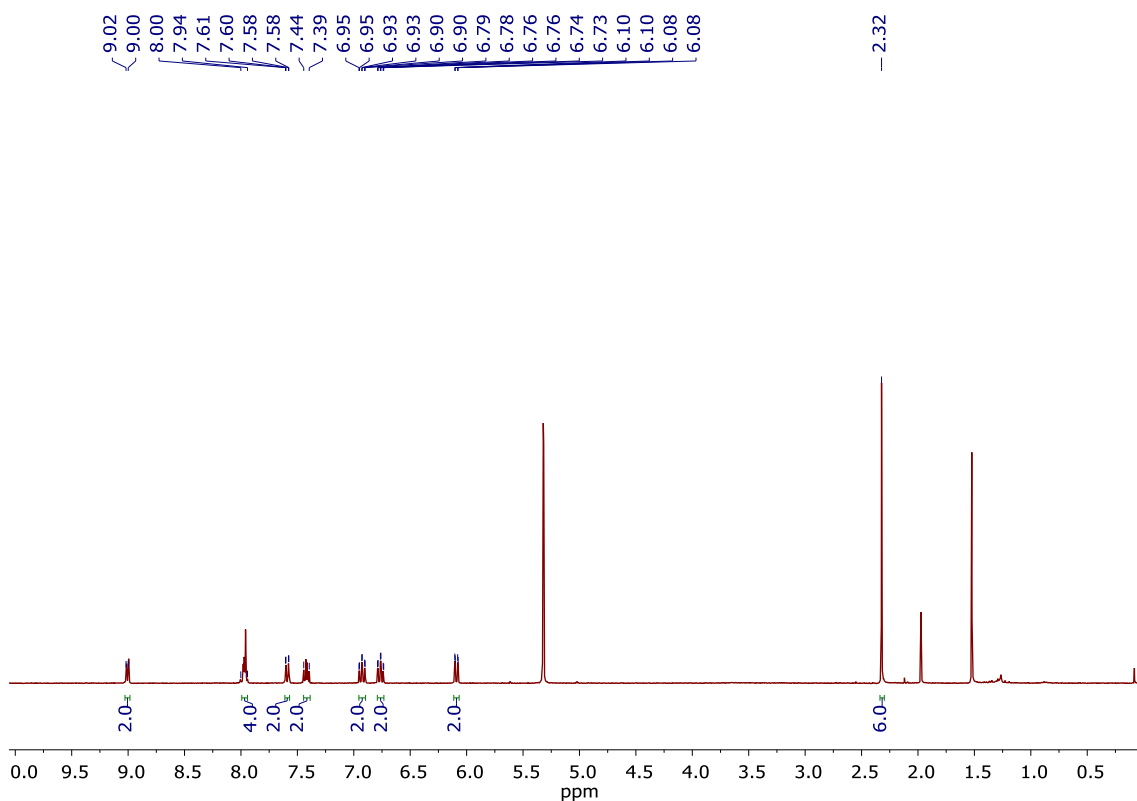
Figure S67. ^1\text{H} NMR of \Delta\text{-}[\text{Ir}(\text{ppy})_2(\text{CH}_3\text{CN})_2]\text{PF}_6 ( \Delta\text{-C5} ). ( \text{CD}_2\text{Cl}_2 , 300 MHz).
