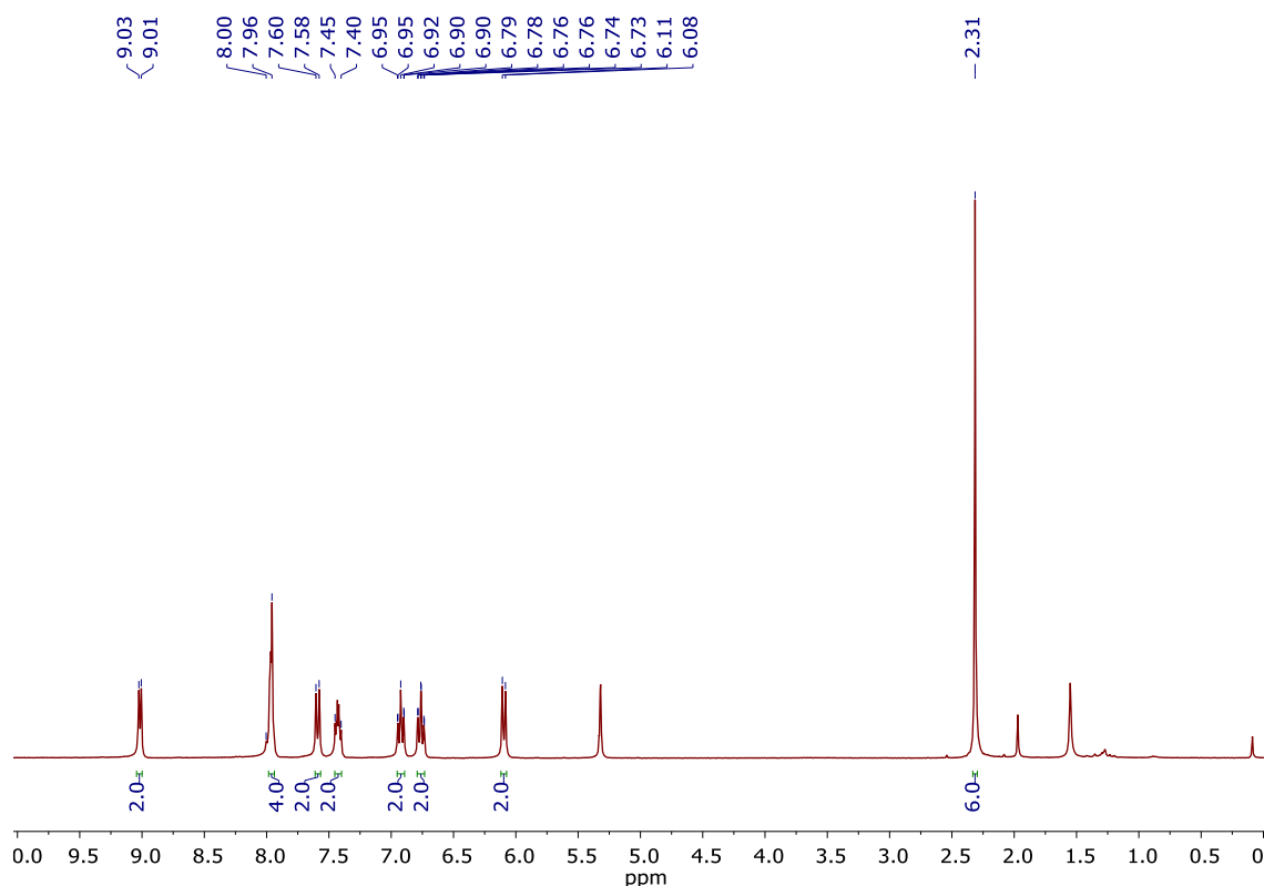
Figure S66. ^1\text{H} NMR of \Delta\text{-}[\text{Ir}(\text{ppy})_2(\text{CH}_3\text{CN})_2]\text{PF}_6 ( \Delta\text{-C5} ). ( \text{CD}_2\text{Cl}_2 , 300 MHz).
