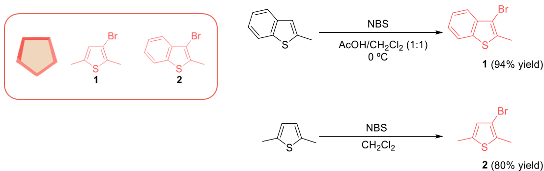
Scheme 3.2. Synthesis of non-coordinating thiophenes 1 and 2 .
