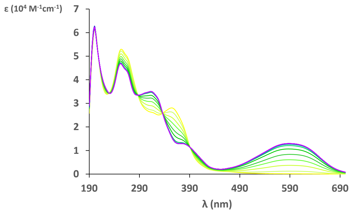
Figure S129. UV/Vis kinetic of Ir-L2-A in \text{CH}_3\text{CN} irradiating at 370 nm, 5 \cdot 10^{-5} \text{ M}
