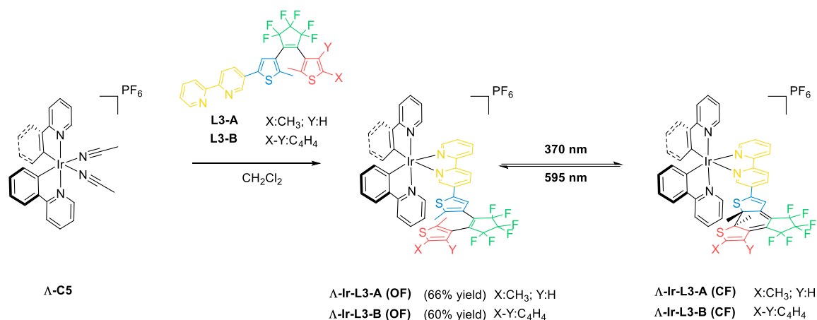
Scheme 3.23. Synthesis of \Lambda\text{-Ir-L3-A} and \Lambda\text{-Ir-L3-B} .
