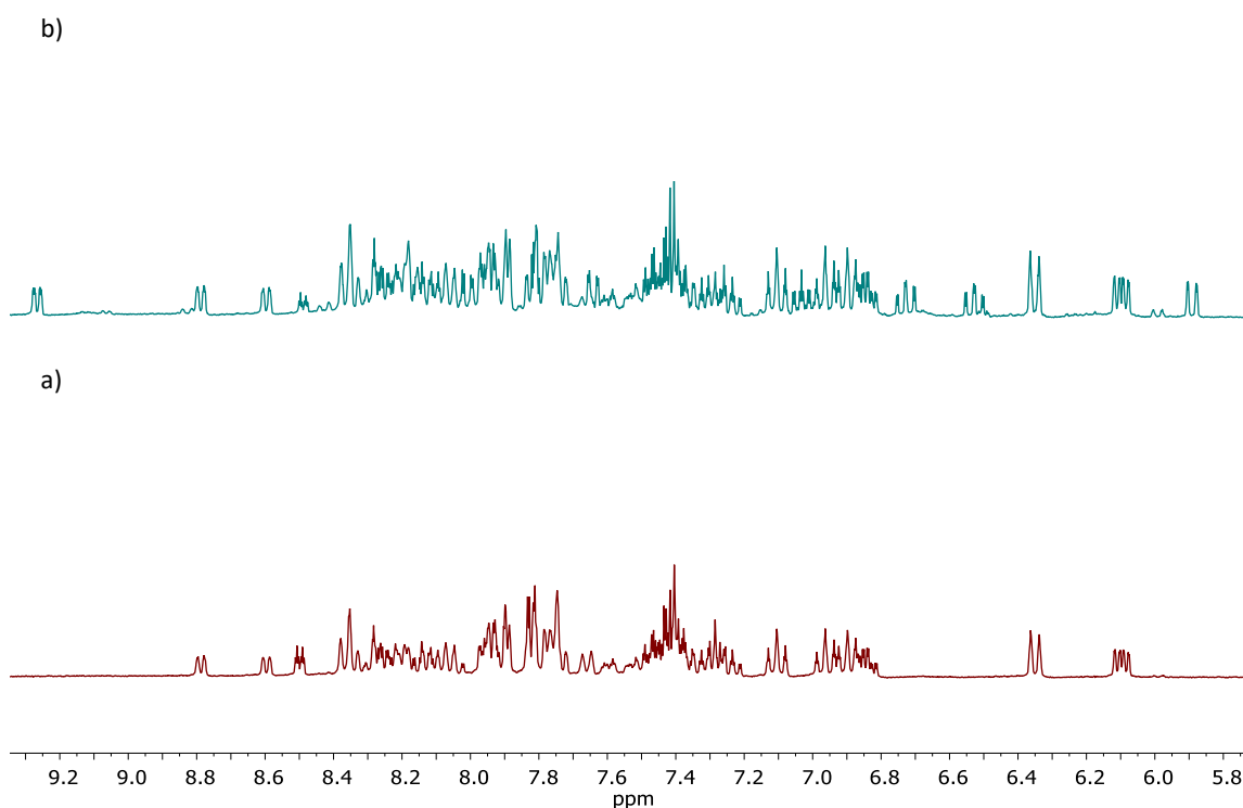
Figure 2.18. a) ^1\text{H} -NMR spectrum of compound rac -Ir-L1-C after precipitation with \text{CH}_2\text{Cl}_2/\text{Et}_2\text{O} , b) ^1\text{H} -NMR spectrum of compound rac -Ir-L1-C after purification through chromatography column. (Acetone- d_6 , 300 MHz).
