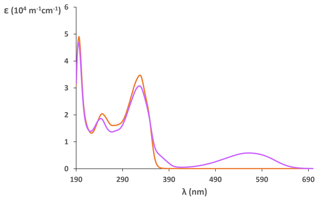
Figure S99. UV/Vis spectra of L3-A in CH 3 CN. Before (orange line) and after (purple line) irradiation at 370 nm, 5 \cdot 10^{-5} \text{ M}
