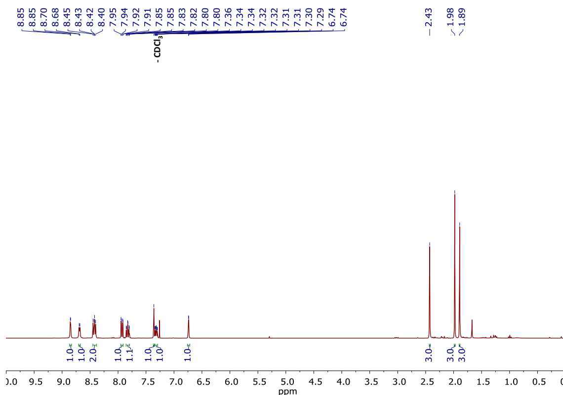
Figure S46. ^1\text{H} NMR of 5-(4-(2-(2,5-dimethylthiophen-3-yl)-3,3,4,4,5,5-hexafluorocyclopent-1-en-1-yl)-5-methylthiophen-2-yl)-2,2'-bipyridine ( L3-A ). ( \text{CDCl}_3 , 300 MHz).
