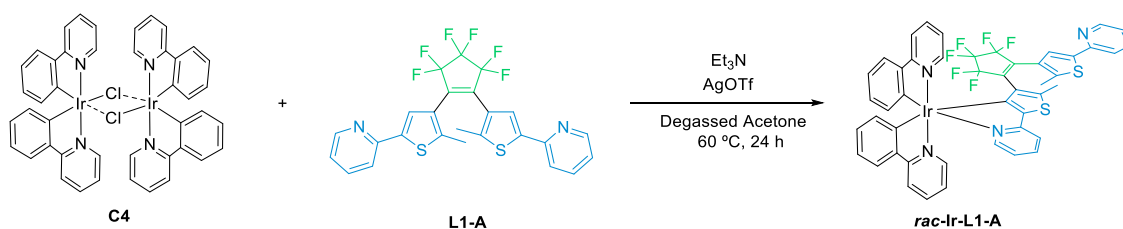
Scheme 2.14. Synthetic route for complex rac-Ir-L1-A .
