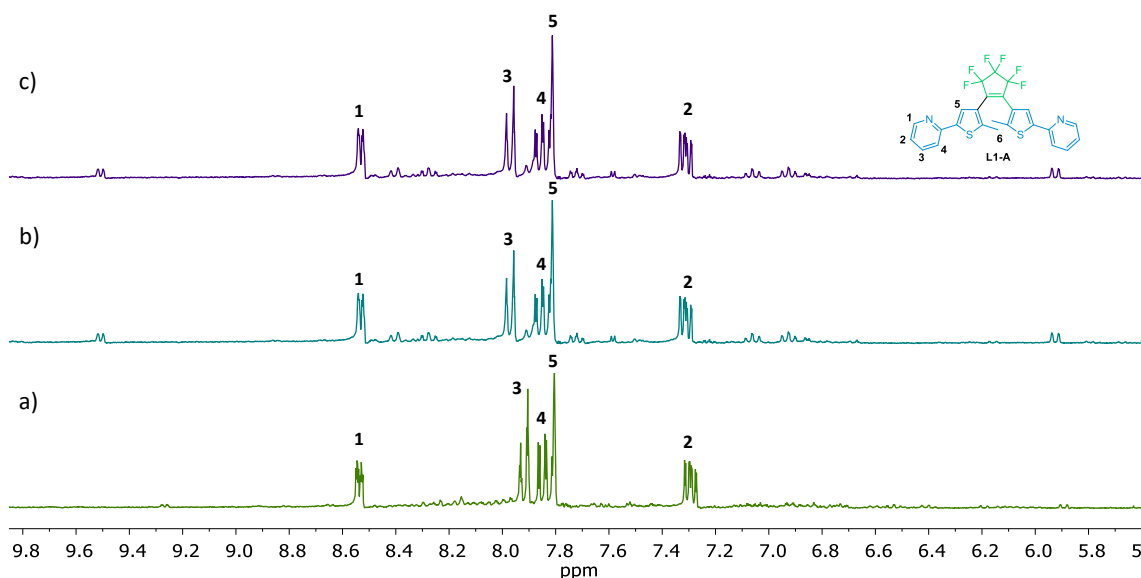
Figure 2.12. a) 1 H-NMR spectrum of the reaction between C4 and L1-A after 3 hours b) 1 H-NMR spectrum of the reaction between C4 and L1-A after 8 hours. c) 1 H-NMR spectrum of the reaction between C4 and L1-A after 24 hours. (Acetone- d 6 , 300 MHz).
