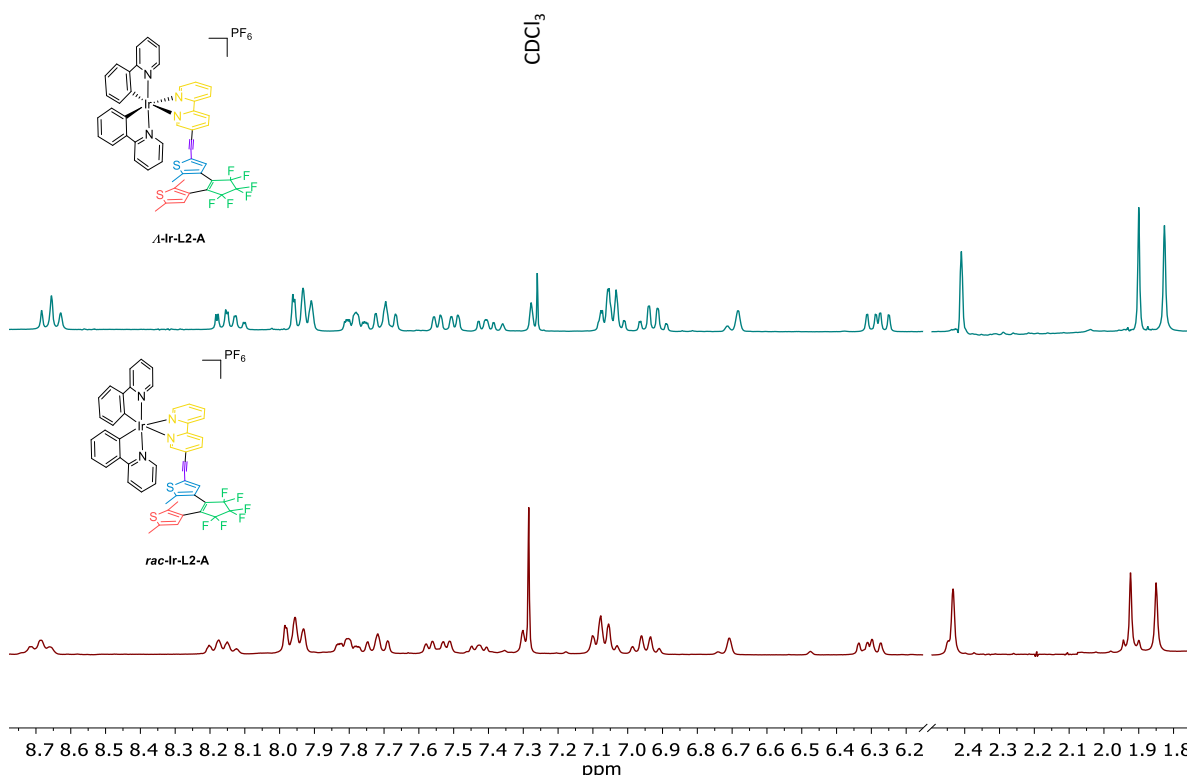
Figure 3.22. 1 H NMR spectra comparing of rac -Ir-L2-A and \Lambda -Ir-L2-A . (CDCl 3 , 300 MHz).
