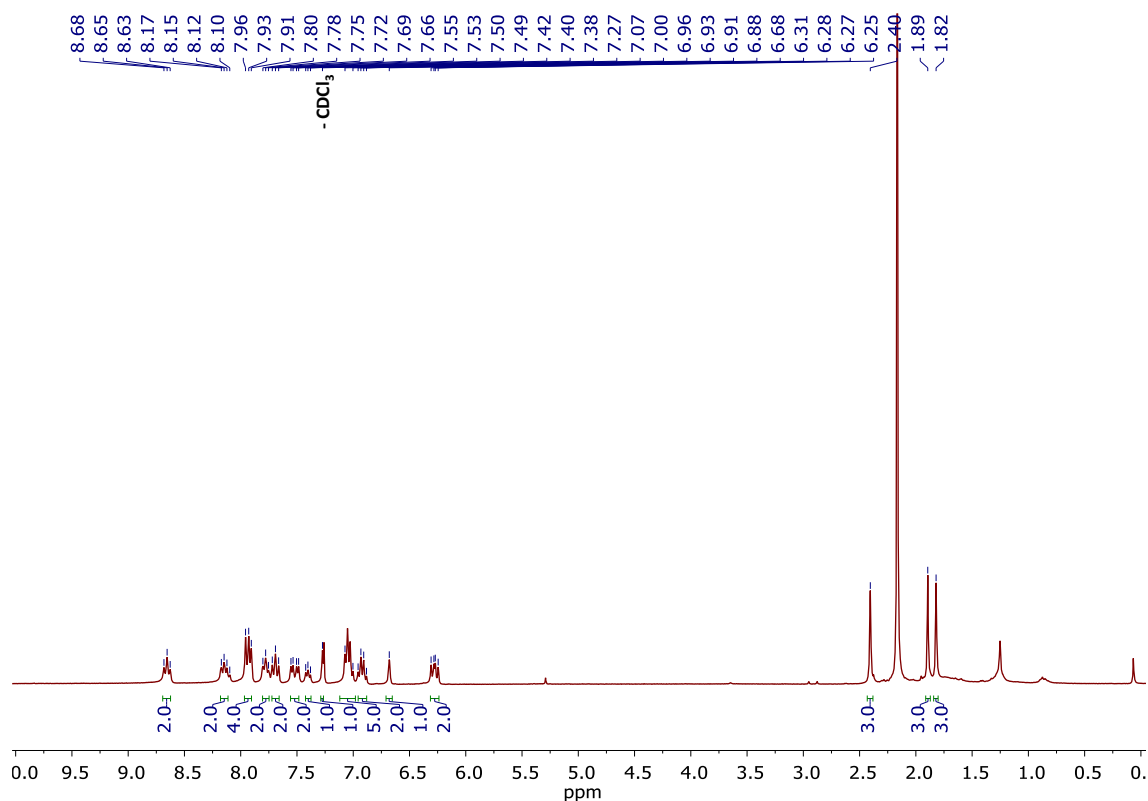
Figure S74. 1 H NMR of \Lambda -[Ir(ppy) 2 (L2-A)]PF 6 ( \Lambda -Ir-L2-A). (CDCl 3 , 300 MHz).
