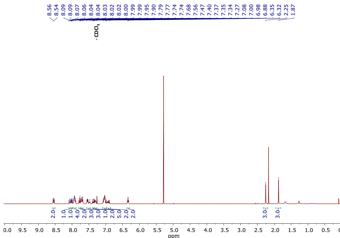
Figure S81. ^1\text{H} NMR of \Delta\text{-}[\text{Ir}(\text{ppy})_2(\text{L3-B})]\text{PF}_6 ( \Delta\text{-Ir-L3-B} ). ( \text{CDCl}_3 , 300 MHz).
