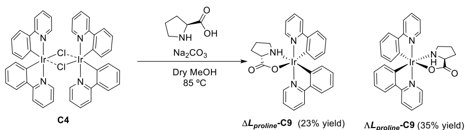
Scheme 3.19. Synthesis of \Delta\text{L-proline-C9}/\Lambda\text{L-proline-C9} complexes.
