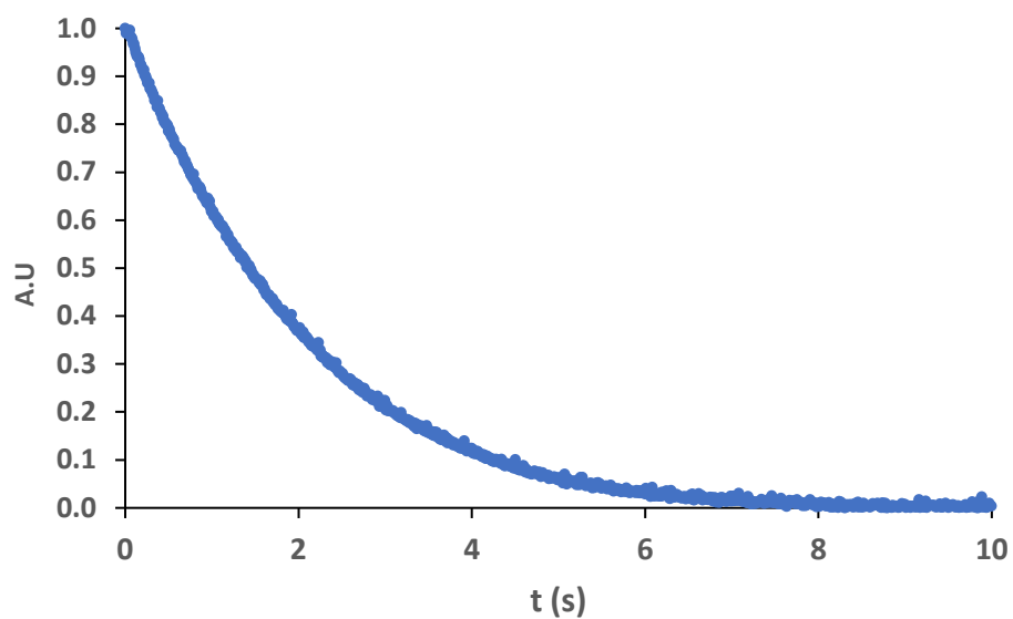
Figure S131. UV/Vis spectra of Ir-L3-A in CH 3 CN. Photocycloreversion process by irradiation at 370 nm, 2.7 \cdot 10^{-5} \text{M}
