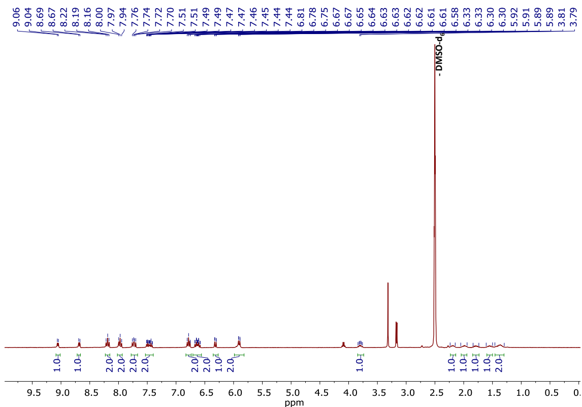
Figure S62. ^1\text{H} NMR of \Lambda -[Ir(ppy) _2 (L-Proline)]PF _6 ( \Lambda L-proline-C9). (DMSO, 300 MHz).
