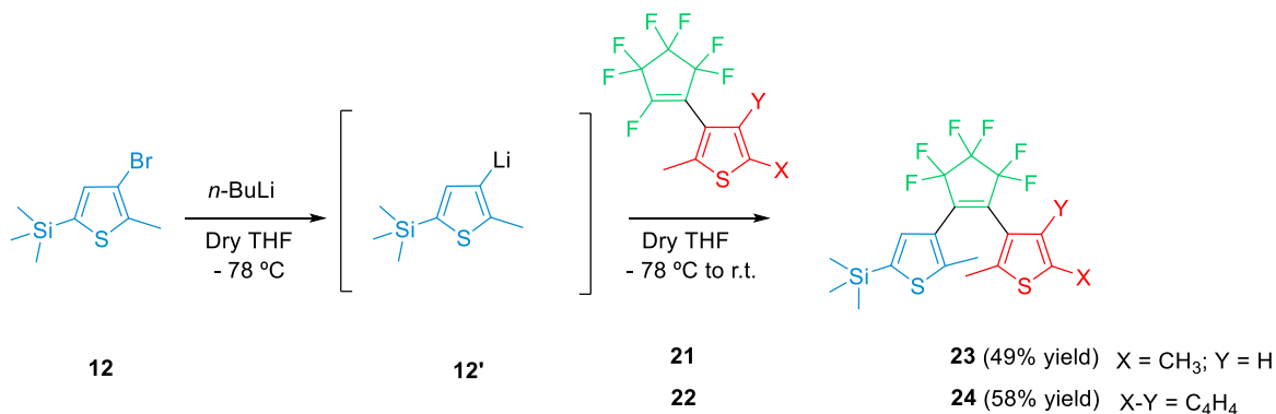
Scheme 3.8. Syntheses of 23-24 .
