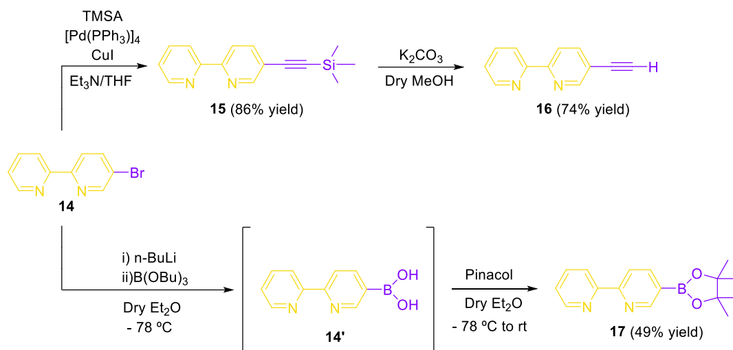
Scheme 3.5. Synthesis of compounds 16 and 17 .
