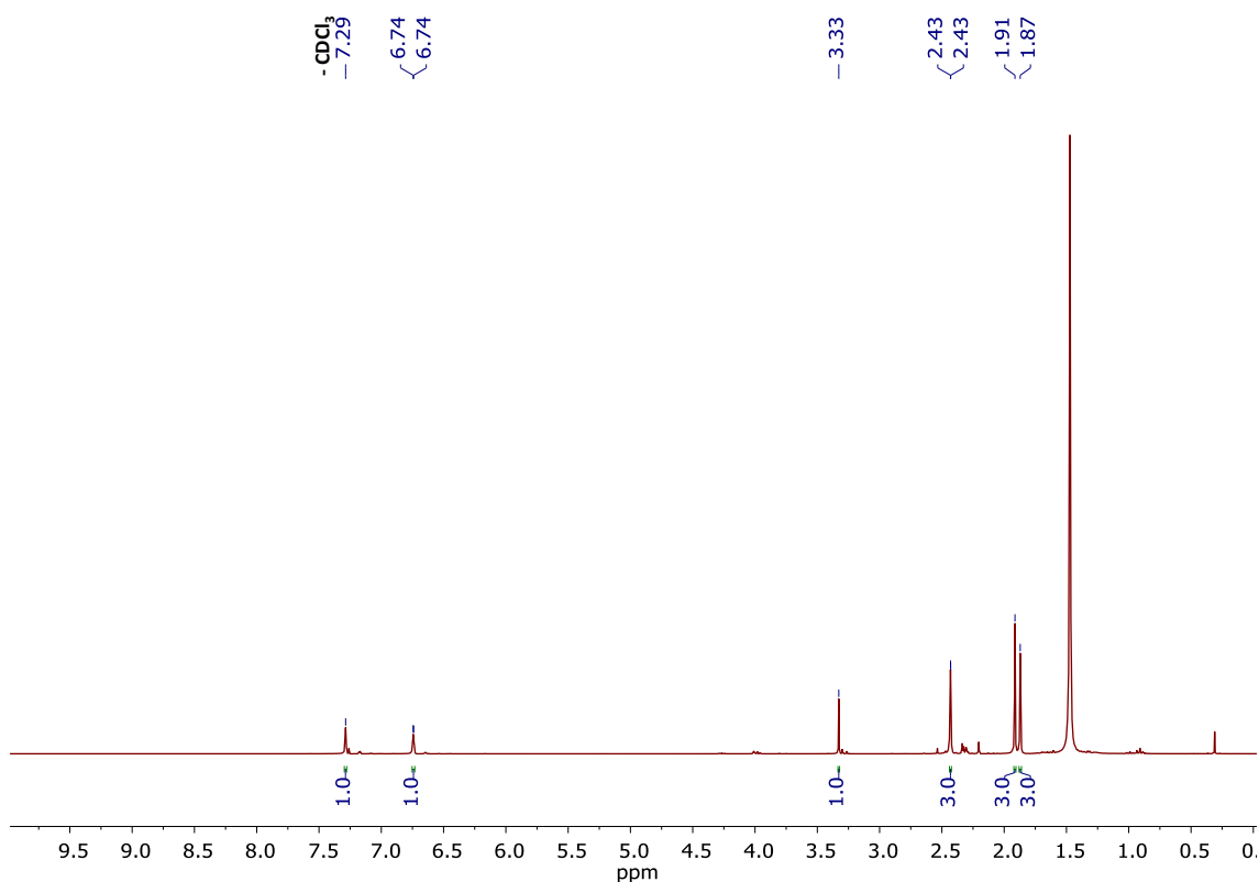
Figure S31. ^1\text{H} -NMR of 3-(2-(2,5-dimethylthiophen-3-yl)-3,3,4,4,5,5-hexafluorocyclopent-1-en-1-yl)-5-ethynyl-2-methylthiophene ( 29 ). ( \text{CDCl}_3 , 300 MHz).
