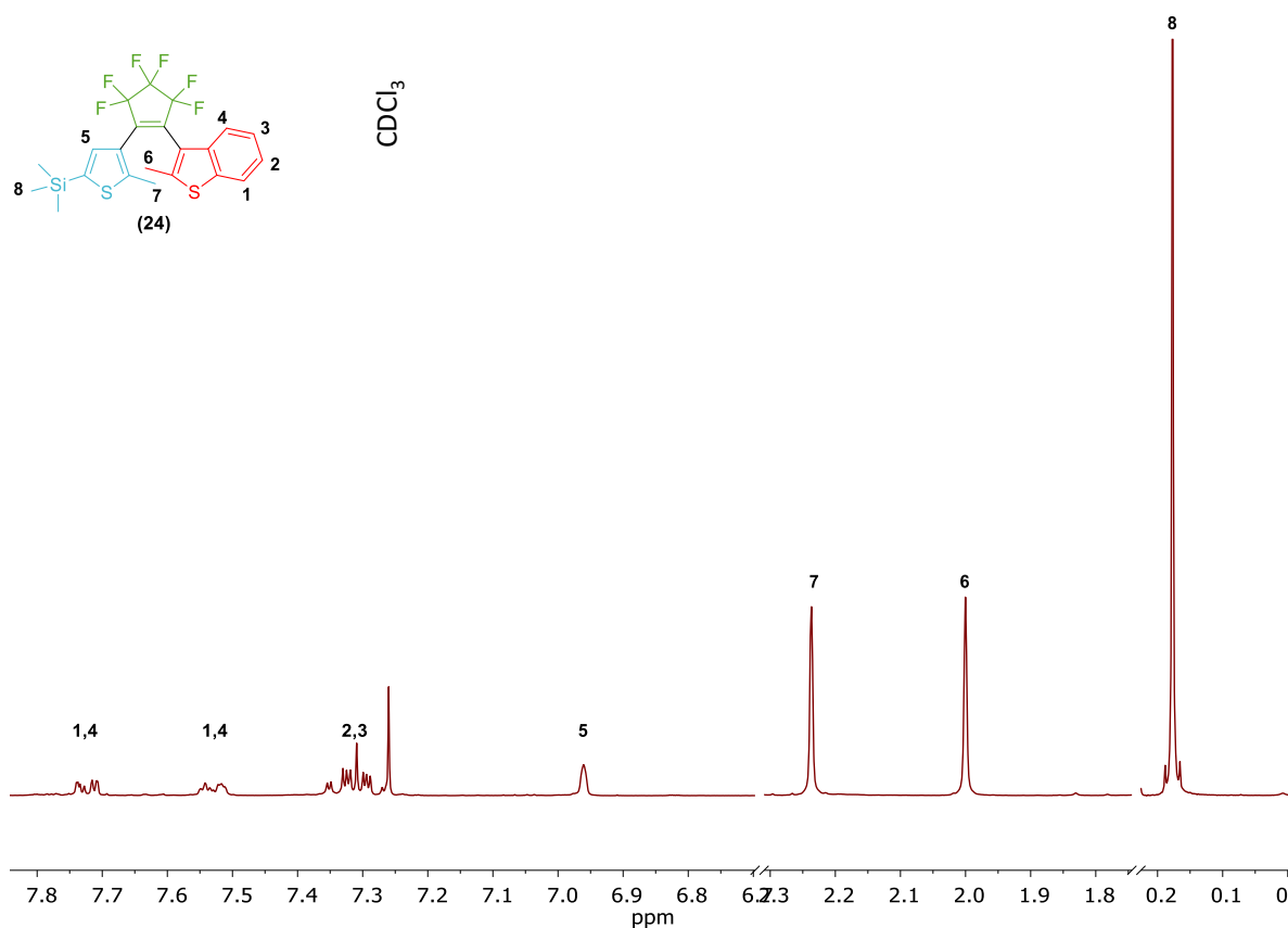
Figure 3.5. ^1\text{H} NMR spectrum of compound 24 . ( \text{CDCl}_3 , 300 MHz).
