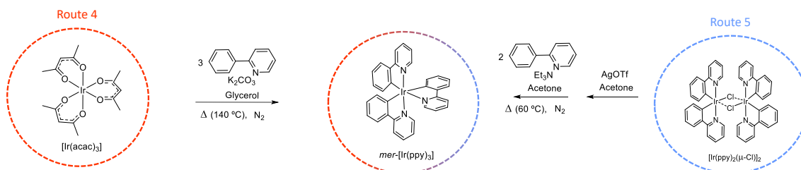
Scheme 1.32. Synthetic procedures described in the literature for the synthesis of mer -Ir(III) complexes.
