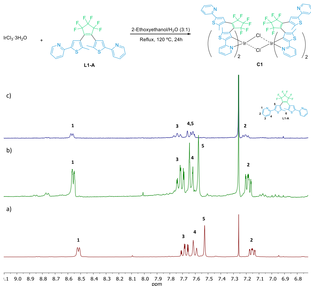
Figure 2.10. a) ^1\text{H} -NMR spectrum of the reaction after 1 hours b) ^1\text{H} -NMR spectrum of the reaction after 24 hours. c) ^1\text{H} -NMR spectrum of the reaction after work-up. ( \text{CDCl}_3 , 300 MHz).
