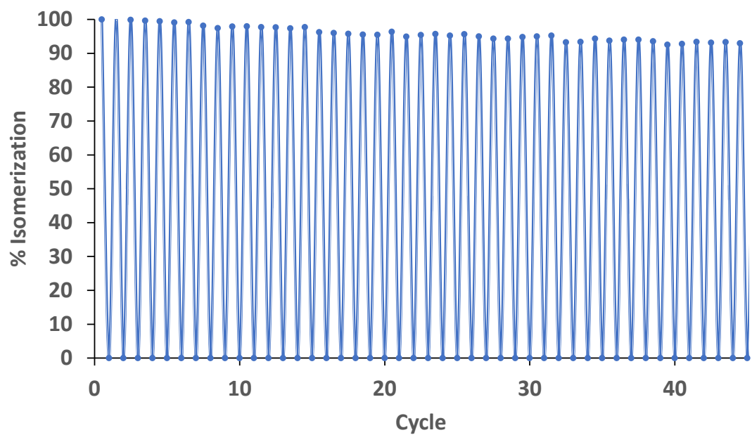
Figure S118. UV/Vis spectra of Ir-L2-A in \text{CH}_3\text{CN} . Fatigue resistance experiment by irradiation at 370 nm, 2.4 \cdot 10^{-5}\text{M}
