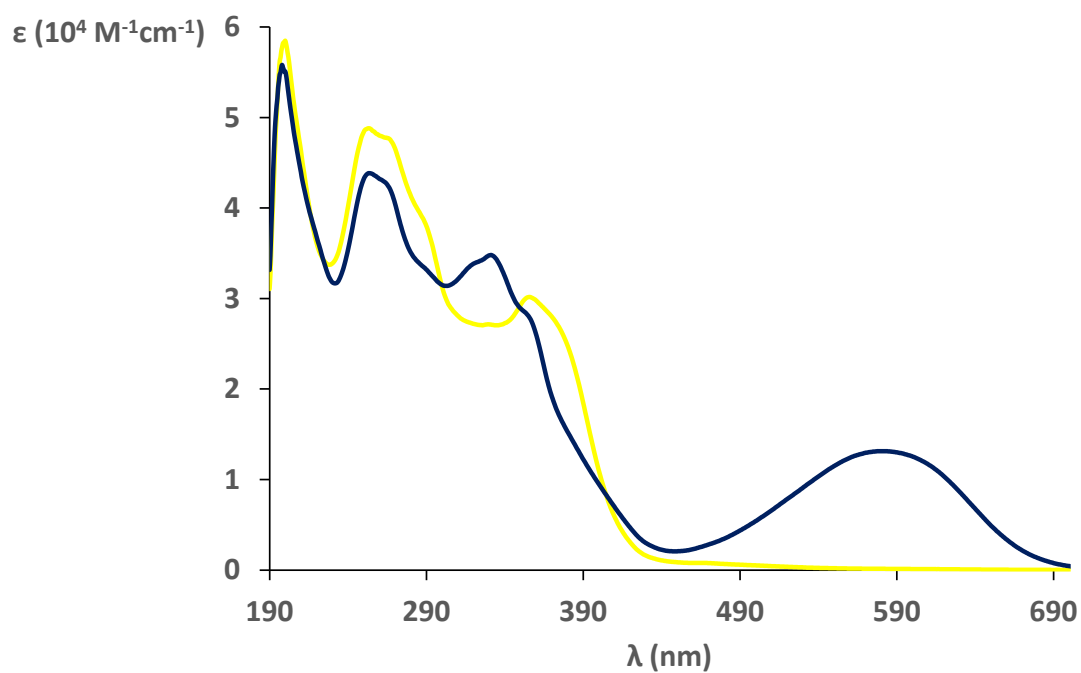
Figure S114. UV/Vis spectra of Ir-L2-A in \text{CH}_3\text{CN} . Before (yellow line) and after (blue line) irradiation at 370 nm, 5 \cdot 10^{-5}\text{M}
