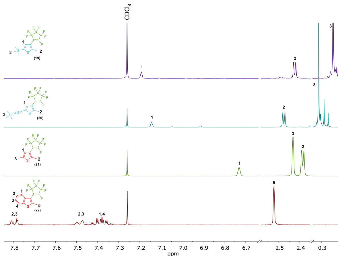
Figure 3.3. ^1\text{H} -NMR spectra of TEs 19 (purple line), 20 (blue line), 21 (green line), and 22 (red line). ( \text{CDCl}_3 , 300 MHz).
