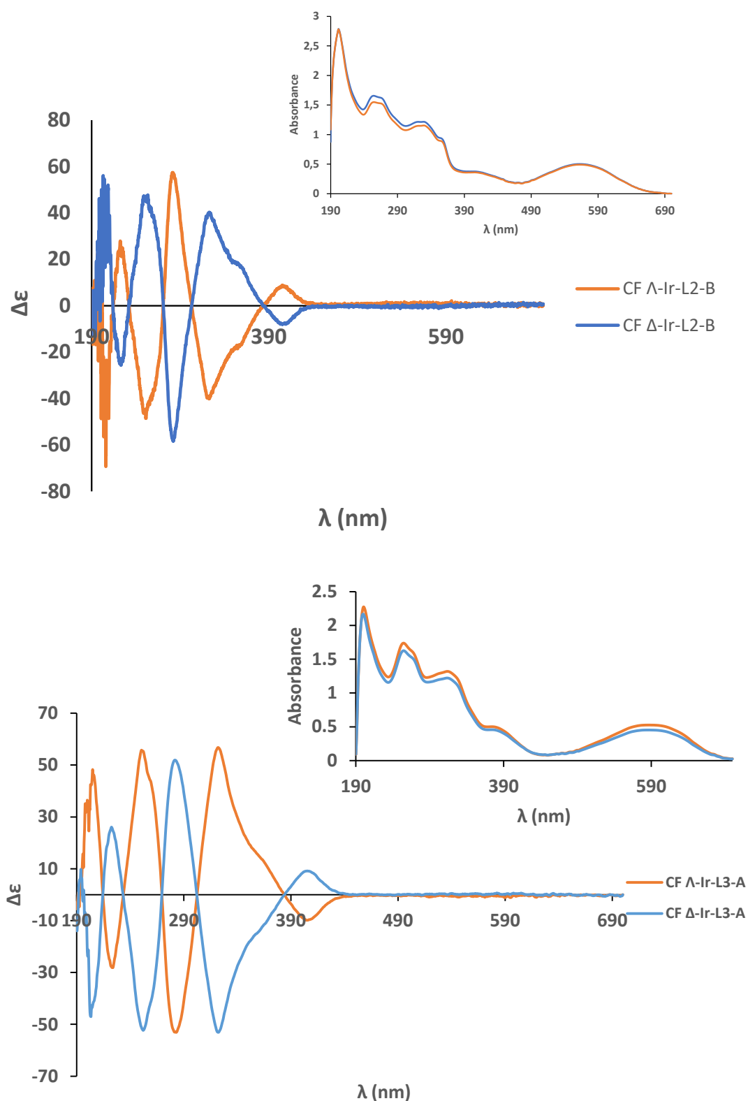
Figure 4.43. CD spectroscopy of CF- \Lambda / \Delta -Ir-L2-A, CF- \Lambda / \Delta -Ir-L2-B, CF- \Lambda / \Delta -Ir-L3-A and CF- \Lambda / \Delta -Ir-L3-B in \text{CH}_3\text{CN} . ( 3.5 \cdot 10^{-5}\text{M} ).
