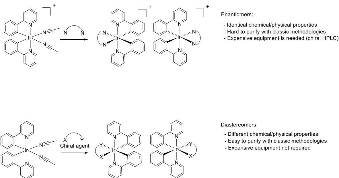
Scheme 1.38. Benefits of using diastereomers forming strategy over the classical enantiomer forming strategy.
