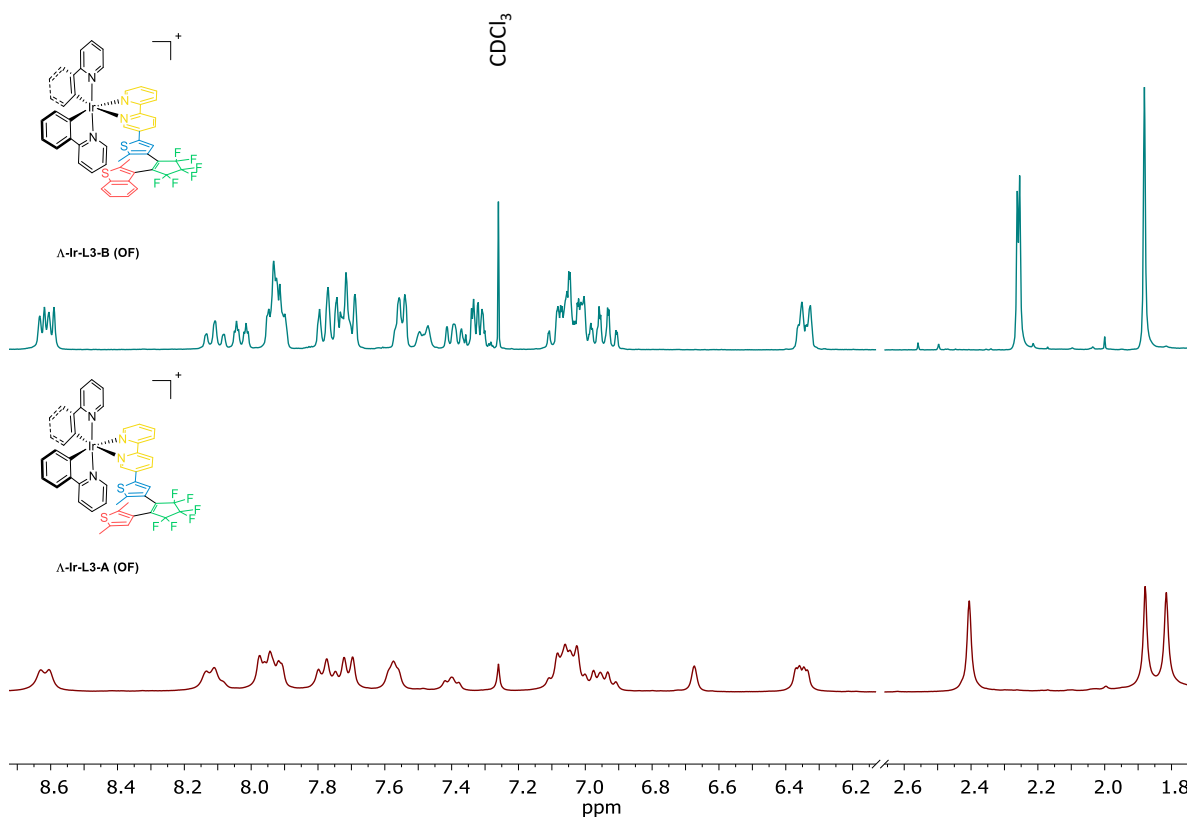
Figure 3.23. ^1\text{H} NMR spectrum of \Lambda\text{-Ir-L3-A} and \Lambda\text{-Ir-L3-B} . ( \text{CDCl}_3 , 300 MHz).
