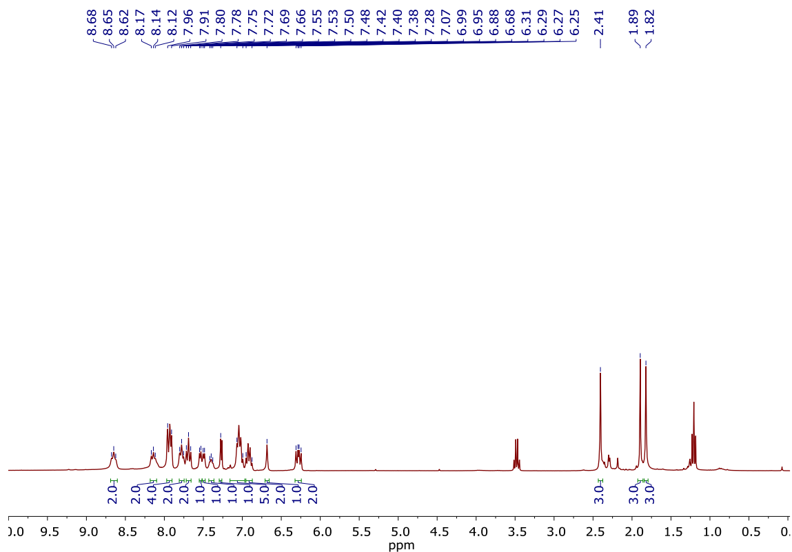
Figure S70. ^1\text{H} NMR of \text{rac-[Ir(ppy)}_2\text{(L2-A)]PF}_6 ( \text{rac-Ir-L2-A} ). ( \text{CDCl}_3 , 300 MHz).
