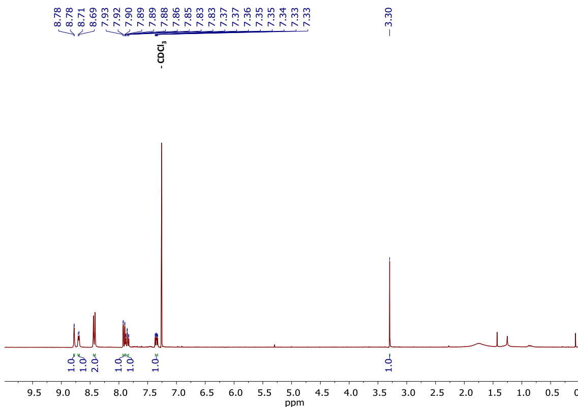
Figure S15. ^1\text{H} NMR of 5-ethynyl-2,2'-bipyridine ( 16 ). ( \text{CDCl}_3 , 300 MHz).
