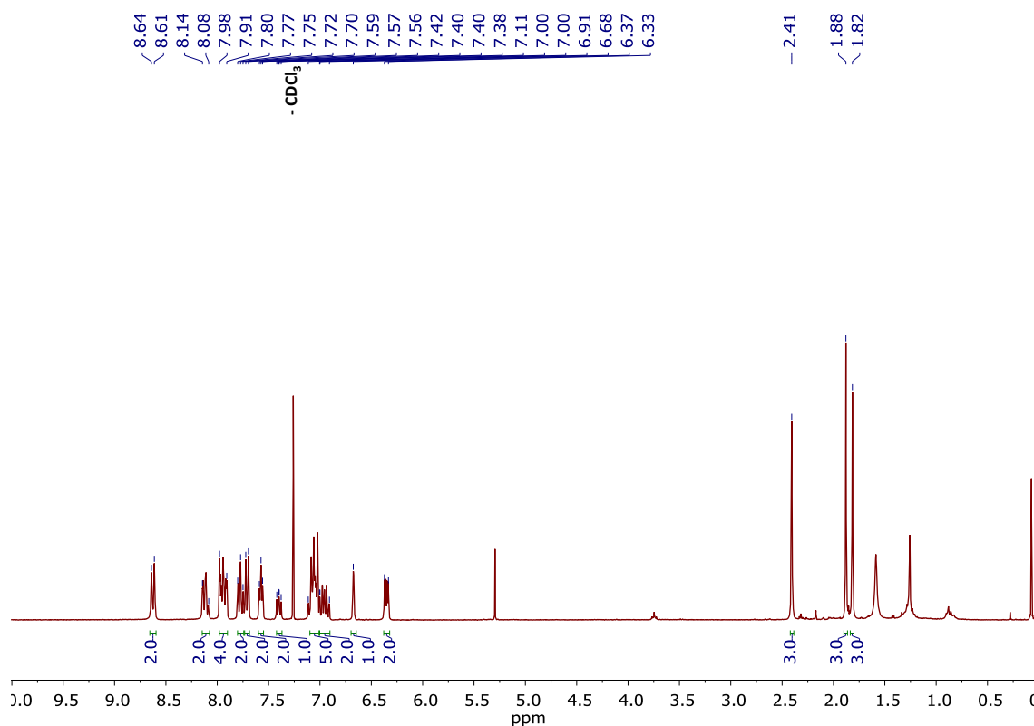
Figure S78. ^1\text{H} NMR of \Delta\text{-}[\text{Ir}(\text{ppy})_2(\text{L3-A})]\text{PF}_6 ( \Delta\text{-Ir-L3-A} ). ( \text{CDCl}_3 , 300 MHz).
