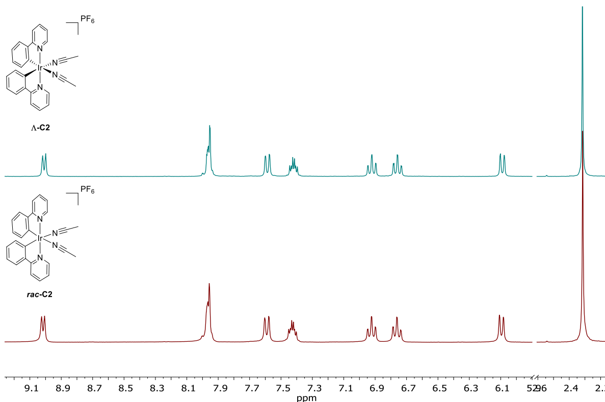
Figure 3.20. 1 H NMR comparison of rac -C5 and \Lambda -C5 . (CDCl 3 , 300 MHz).
