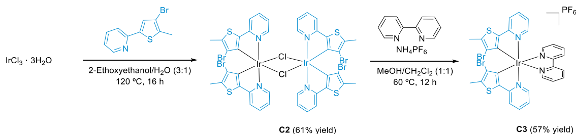
Scheme 2.10. Synthetic route for compounds C2 and C3 .
