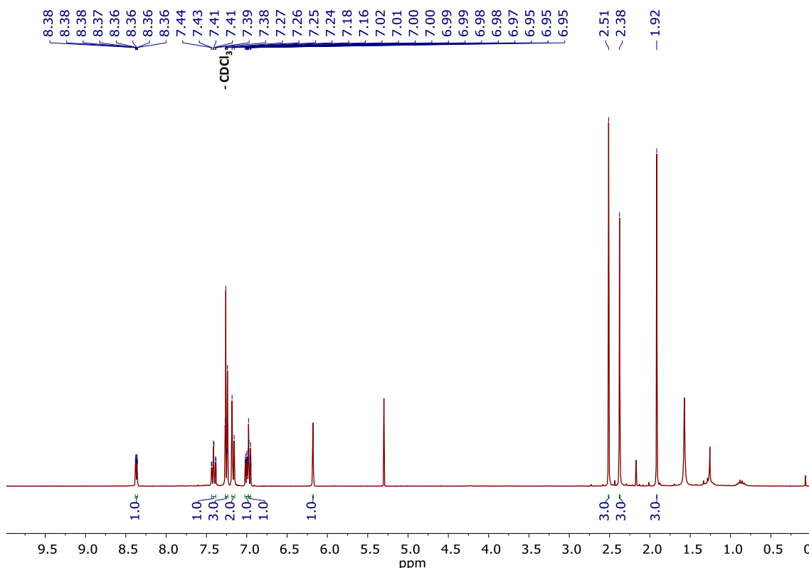
Figure S37. ^1\text{H} NMR of 2-(4-(3,3,4,4,5,5-hexafluoro-2-(2-methyl-5-(p-tolyl)thiophen-3-yl)cyclopent-1-en-1-yl)-5-methylthiophen-3-yl)pyridine ( L1-D ). ( \text{CDCl}_3 , 300 MHz).
