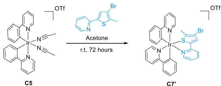
Scheme 2.20. Synthesis of iridium complex C7' .
