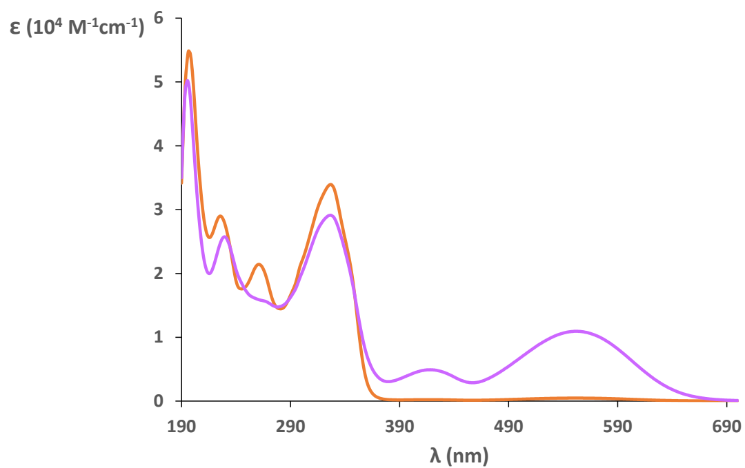
Figure S106. UV/Vis spectra of L3-B in CH 3 CN. Before (orange line) and after (purple line) irradiation at 370 nm, 5 \cdot 10^{-5} \text{ M}
