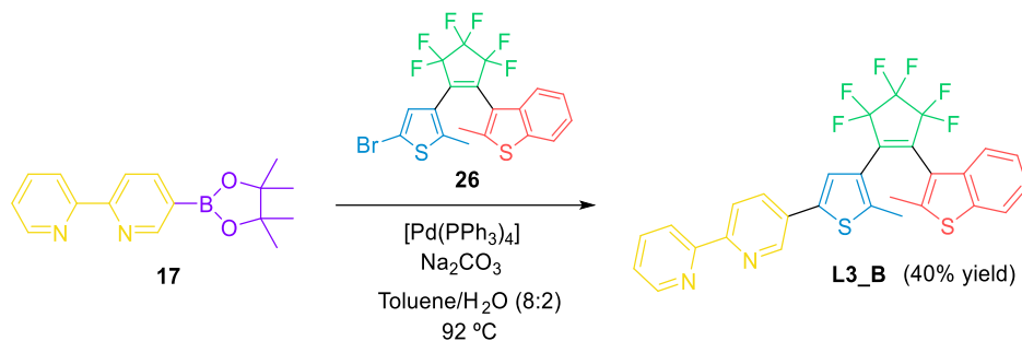
Scheme 3.11. Synthesis of L3-B .
