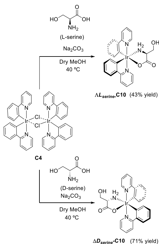
Scheme 3.20. Synthesis of \Delta\text{D}_{\text{serine}}\text{-C10} and \Lambda\text{L}_{\text{serine}}\text{-C10} complexes.
