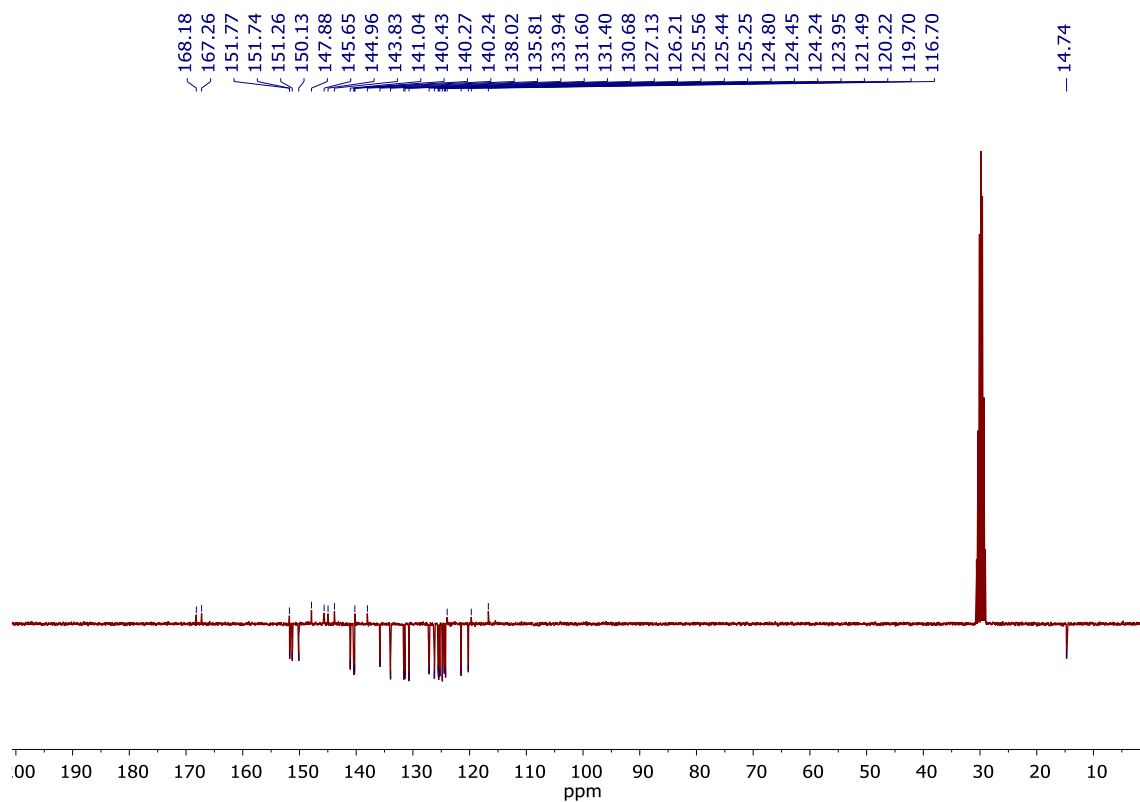
Figure S59. 13 C NMR of [Ir(ppy) 2 (2-pyridyl-4-bromo-5-methylthiophene)]. (Acetone-d 3 , 300 MHz).
