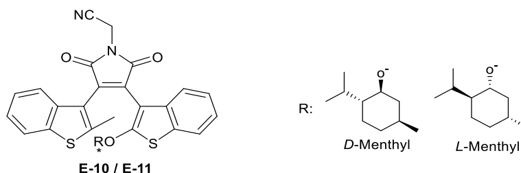
Scheme 1.18. E-10 DTE by Yamaguchi and coworkers. 45
