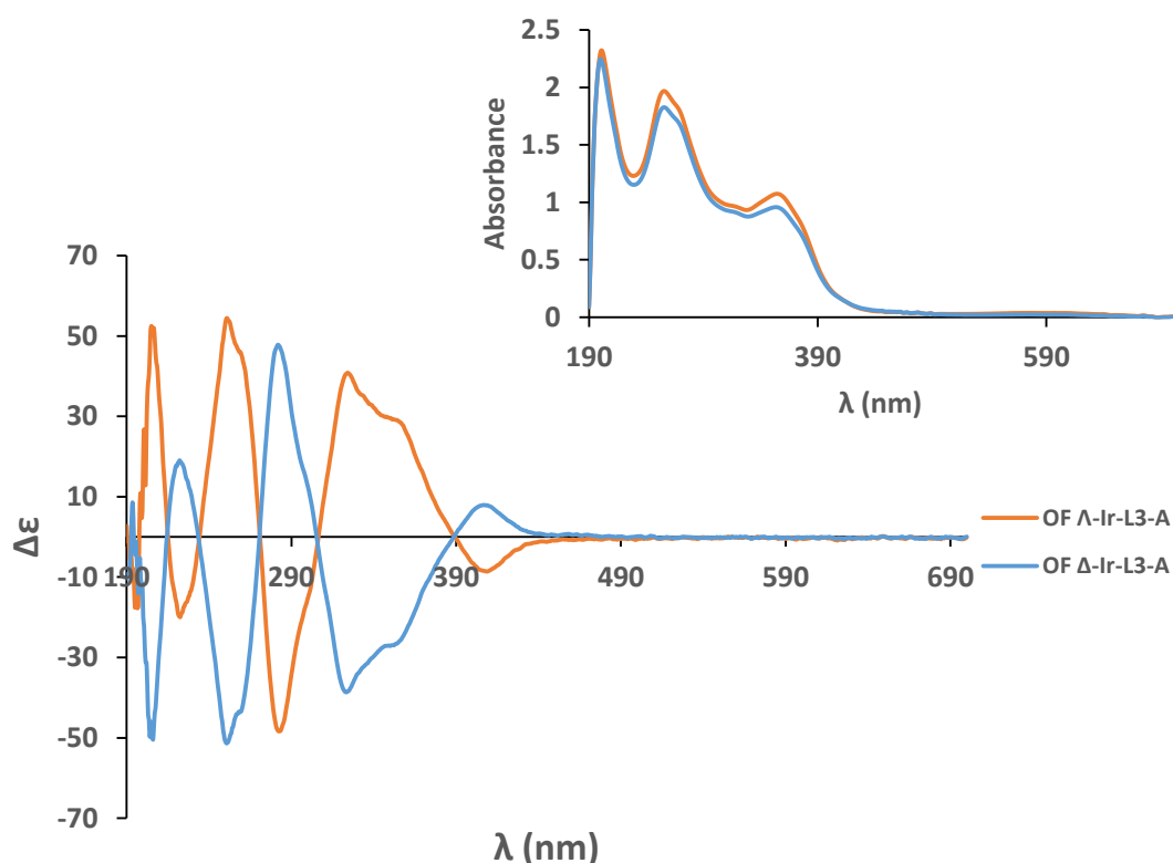
Figure 4.42. CD spectra of OF- \Lambda -Ir-L2-A , OF- \Lambda -Ir-L2-B , OF- \Lambda -Ir-L3-A and OF- \Lambda -Ir-L3-B in \text{CH}_3\text{CN} . ( 3.5 \cdot 10^{-5}\text{M} ).
