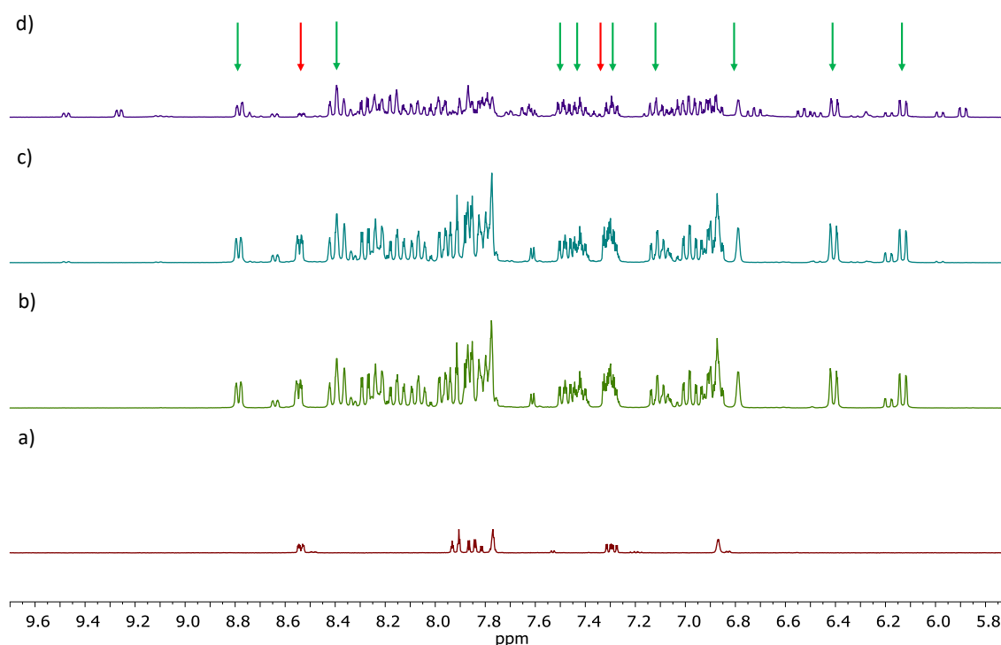
Figure 2.19. a) ^1\text{H} -NMR spectrum of free ligand L1-B ; b) ^1\text{H} -NMR spectrum of compound rac -Ir-L1-B after 1 hour of reaction; c) ^1\text{H} -NMR spectrum of compound rac -Ir-L1-B after 24 hours of reaction; d) ^1\text{H} -NMR spectrum of compound rac -Ir-L1-B after purification through column chromatography. (Acetone- d_6 , 300 MHz).
