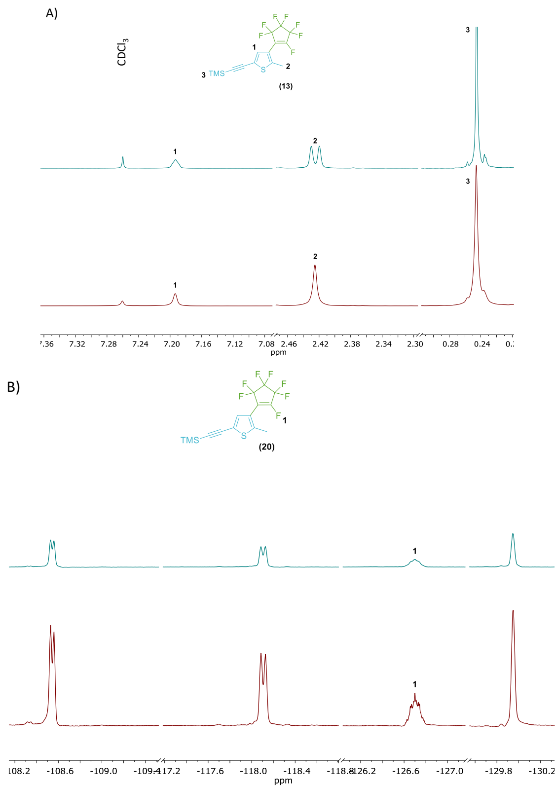
Figure 3.4. A) 1 H NMR (blue) and { 19 F} 1 H NMR (red) spectra of compound 20 . B) . { 1 H} 19 F NMR (blue) and 19 F NMR (red) spectra of compound 20 . (CDCl 3 , 300 MHz).
