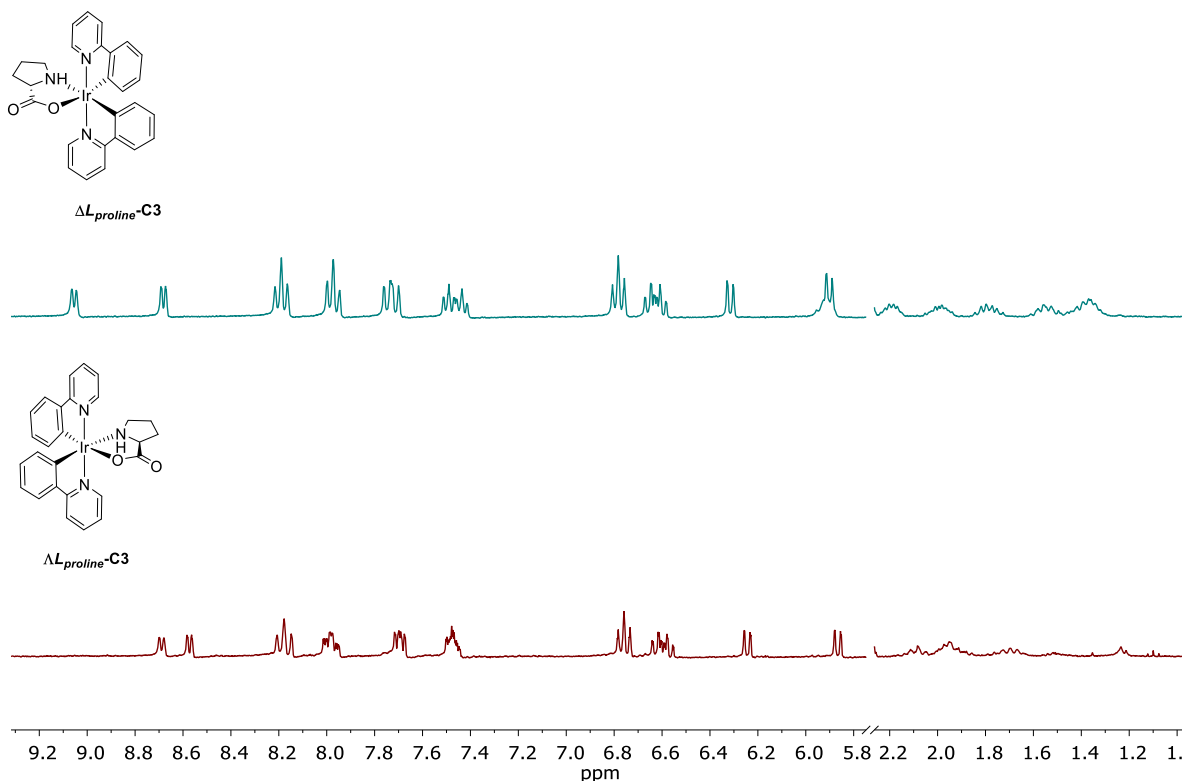
Figure 3.18. ^1\text{H-NMR} comparison of \Delta\text{L-proline-C9} and \Lambda\text{L-proline-C9} . (DMSO, 300 MHz).
