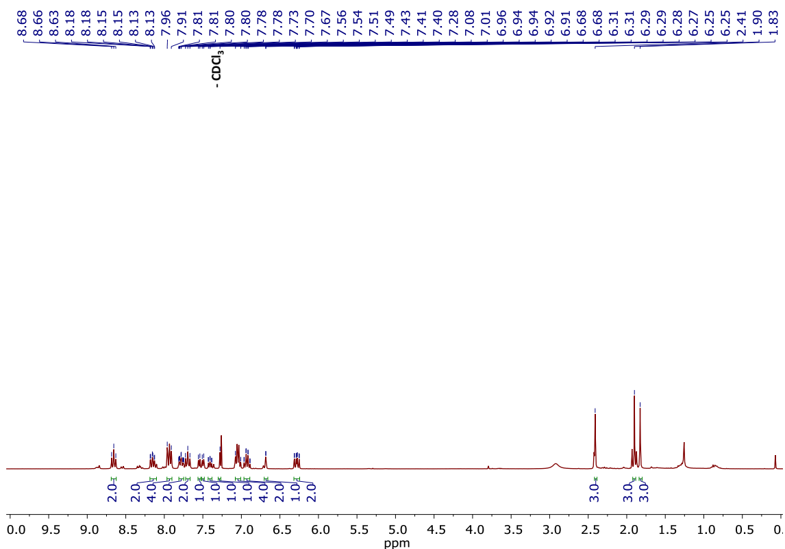
Figure S75. ^1\text{H} NMR of \Delta\text{-}[\text{Ir}(\text{ppy})_2(\text{L2-A})]\text{PF}_6 ( \Delta\text{-Ir-L2-A} ). ( \text{CDCl}_3 , 300 MHz).
