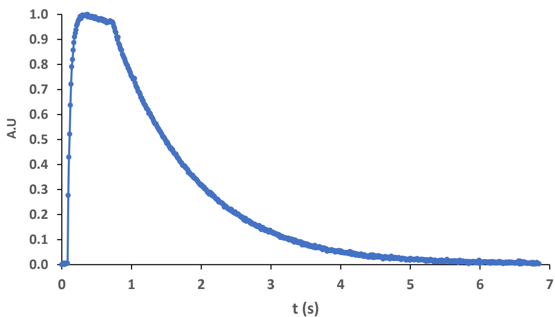
Figure S88. UV/Vis spectra of L2-A in CH 3 CN. Photocycloreversion process by irradiation at 370 nm, 3.3 \cdot 10^{-5} M
