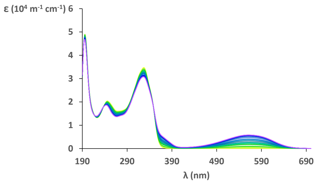
Figure S100. UV/Vis kinetic of L3-A in CH 3 CN irradiating at 370 nm, 5 \cdot 10^{-5} \text{ M}
