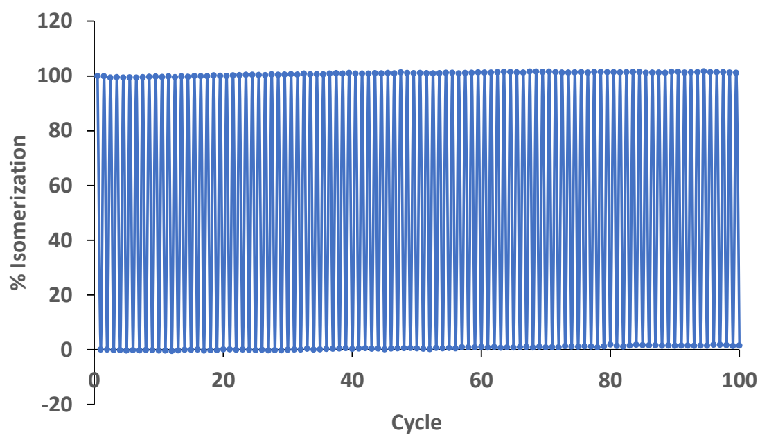
Figure S111. UV/Vis spectra of L3-B in CH 3 CN. Fatigue resistance experiment by irradiation at 370 nm and 595 nm alternatively, 2.7 \cdot 10^{-5} \text{M}
