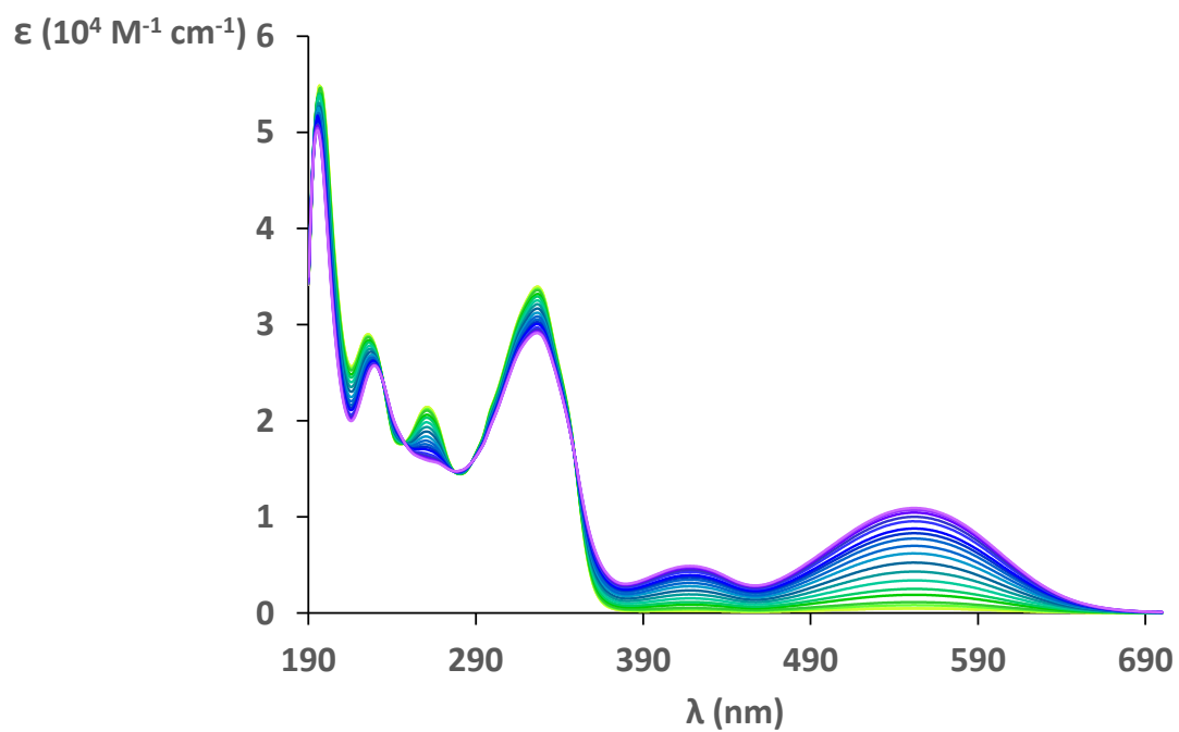
Figure S107. UV/Vis kinetic of L3-B in CH 3 CN irradiating at 370 nm, 5 \cdot 10^{-5} \text{ M}
