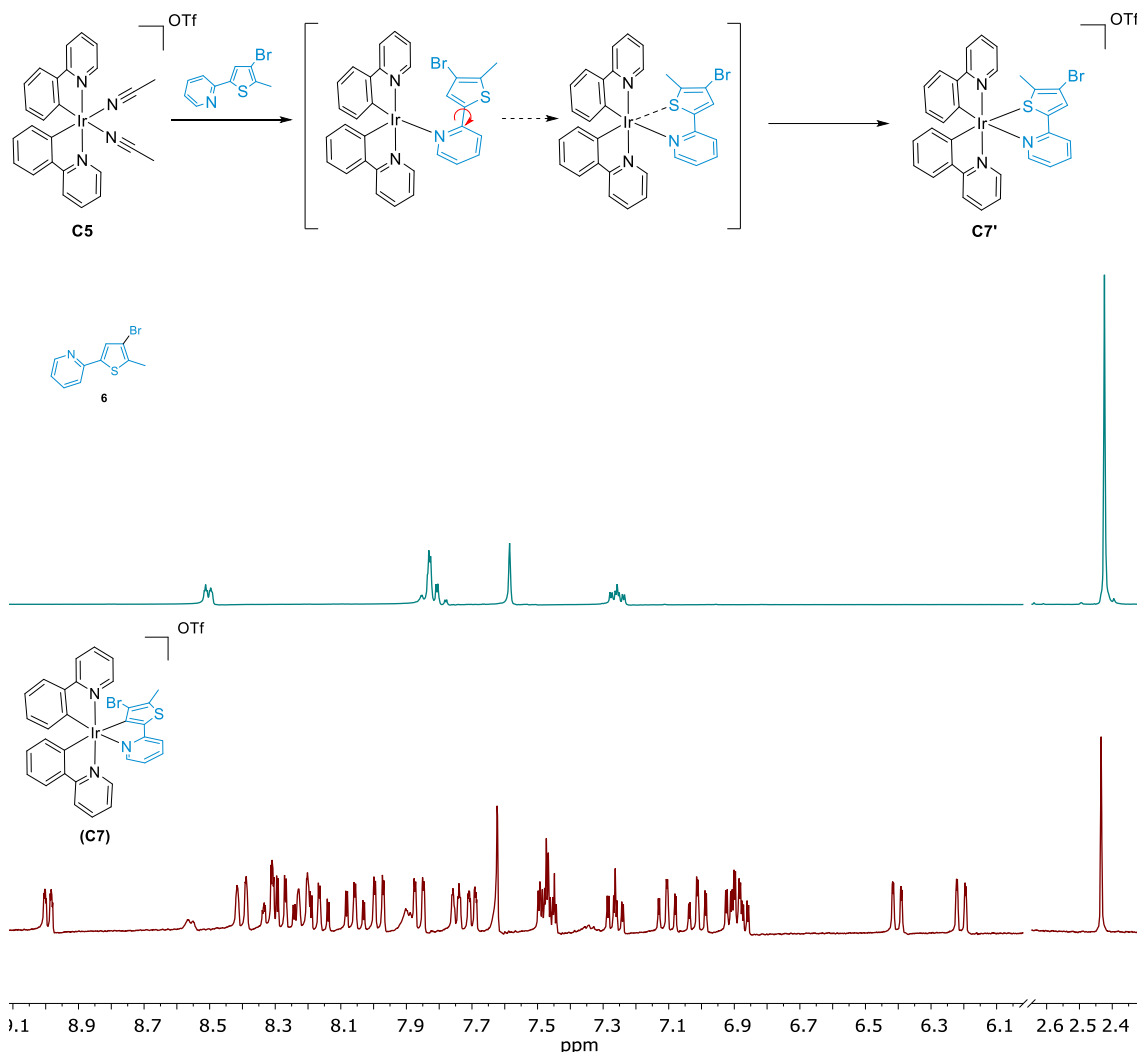
Figure 2.16. ^1\text{H} -NMR spectra and possible mechanism for the N-S coordination between C5 and compound 6 . (Acetone- d_6 , 300 MHz).
