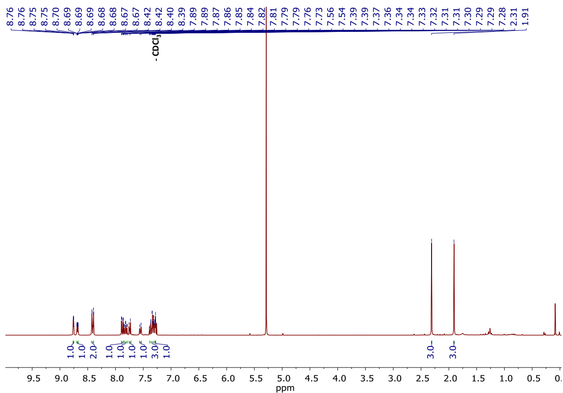
Figure S42. ^1\text{H} NMR of 5-((4-(3,3,4,4,5,5-hexafluoro-2-(2-methylbenzo[b]thiophen-3-yl)cyclopent-1-en-1-yl)-5-methylthiophen-2-yl)ethynyl)-2,2'-bipyridine ( L2-B ). ( \text{CDCl}_3 , 300 MHz).
