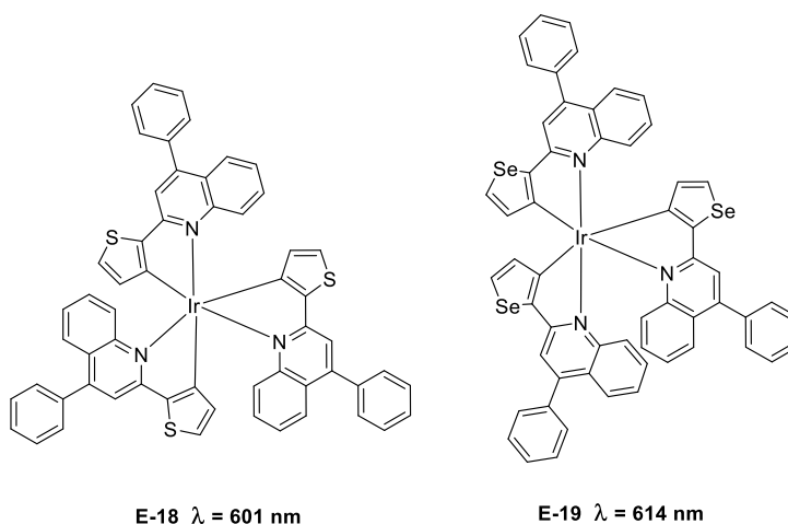
Scheme 1.36. Red emitter iridium complexes described by Lee and Jin. 106,107
