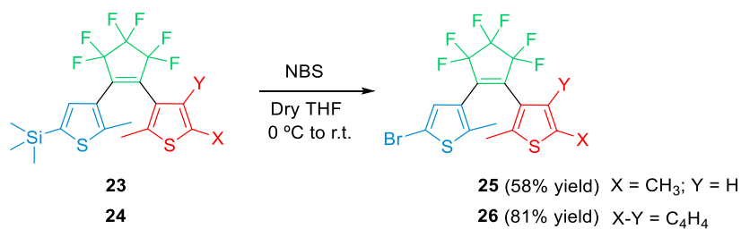
Scheme 3.9. Syntheses of 25 and 26 .
