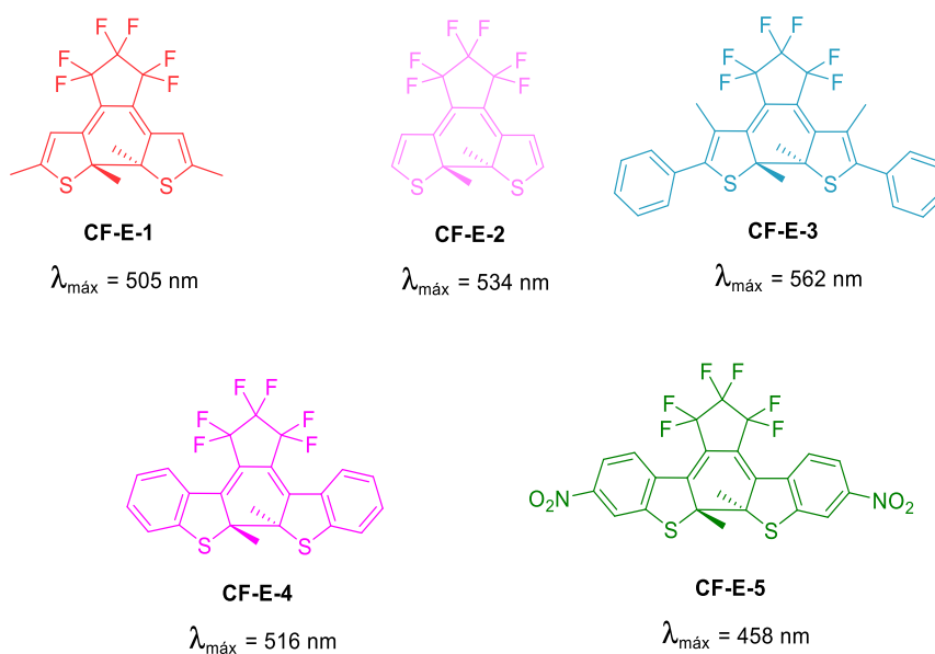
Scheme 1.6. Different \lambda_{\text{m\acute{a}x}} for DTEs. 22
