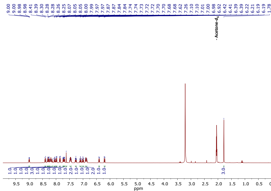
Figure S58. 1 H NMR of [Ir(ppy) 2 (2-pyridyl-4-bromo-5-methylthiophene)]. (Acetone-d 3 , 300 MHz).
