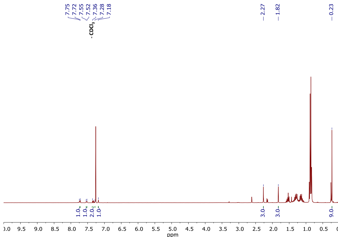
Figure S30. ^1\text{H} -NMR of ((4-(3,3,4,4,5,5-hexafluoro-2-(2-methylbenzo[b]thiophen-3-yl)cyclopent-1-en-1-yl)-5-methylthiophen-2-yl)ethynyl)trimethylsilane ( 28 ). ( \text{CDCl}_3 , 300 MHz).
