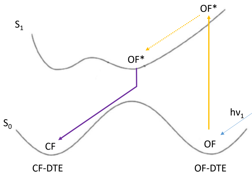
Figure 1.7. Theoretical representation of photocyclization mechanism
