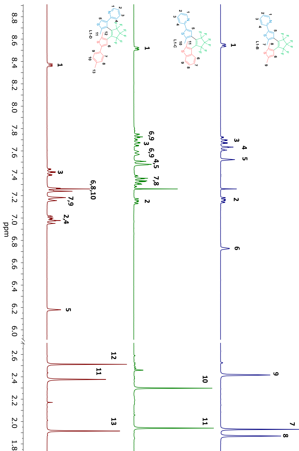
Figure 2.7. ^1\text{H} -NMR spectra of L1-B – L1-D. ( \text{CDCl}_3 , 300 MHz).
