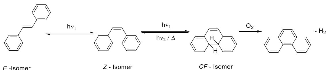
Scheme 1.2 Stilbene E/Z isomerization and H 2 elimination yielding phenanthrene.
