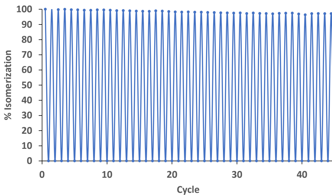
Figure S125. UV/Vis spectra of Ir-L2-B in \text{CH}_3\text{CN} . Fatigue resistance experiment by irradiation at 370 nm, 2.6 \cdot 10^{-5}\text{M}
