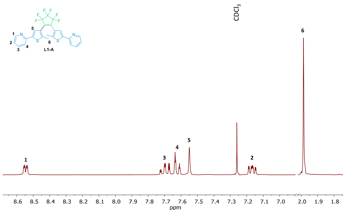
Figure 2.6. ^1\text{H} -NMR spectrum of compound L1-A . ( \text{CDCl}_3 , 300 MHz).
