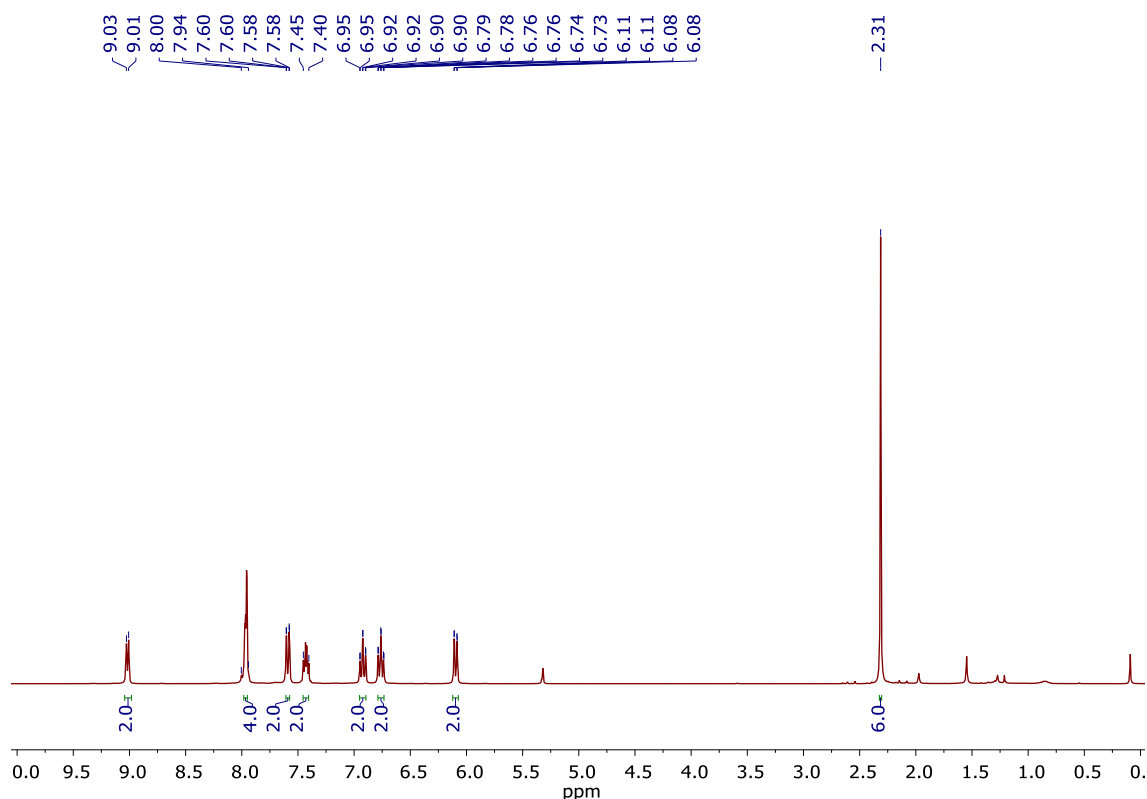
Figure S69. ^1\text{H} NMR of \Delta\text{-}[\text{Ir}(\text{ppy})_2(\text{CH}_3\text{CN})_2]\text{PF}_6 ( \Delta\text{-C5} ) ( \text{CD}_2\text{Cl}_2 , 300 MHz).
