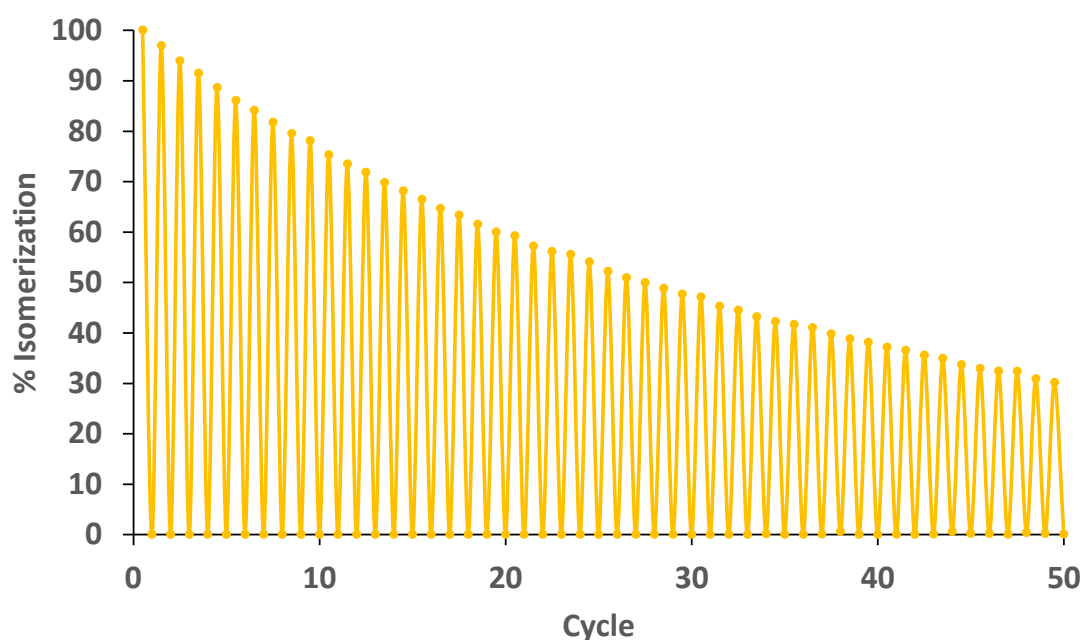
Figure 4.13. Photocyclization ( \lambda_{\text{irr}} = 370 nm)-photocycloreversion ( \lambda_{\text{irr}} = 595 nm) cycles of L2-A , showing photoinduced-decomposition in \text{CH}_3\text{CN} .
