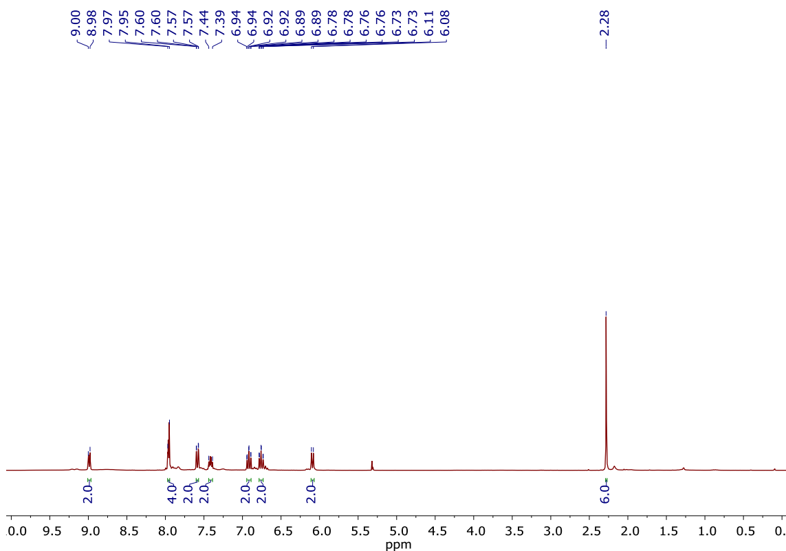
Figure S68. ^1\text{H} NMR of \Delta -[Ir(ppy) _2 (CH _3 CN) _2 ]PF _6 ( \Delta -C5 ). (CD _2 Cl _2 , 300 MHz).
