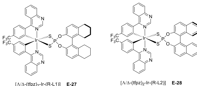
Scheme 1.40. E-27 and E-28 enantiopure complexes synthesized by Zuo et al.
