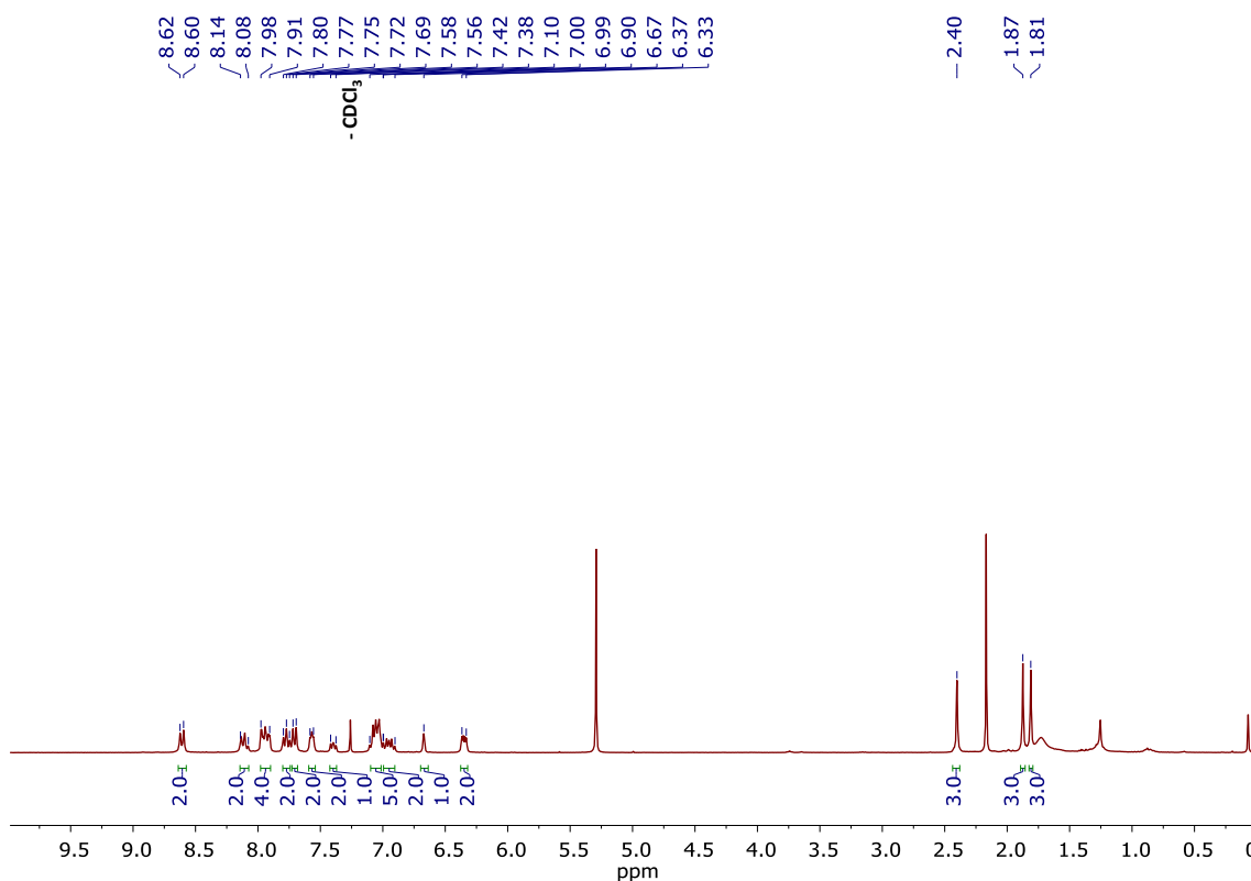
Figure S79. ^1\text{H} NMR of \Delta\text{-}[\text{Ir}(\text{ppy})_2(\text{L3-A})]\text{PF}_6 ( \Delta\text{-Ir-L3-A} ). ( \text{CDCl}_3 , 300 MHz).
