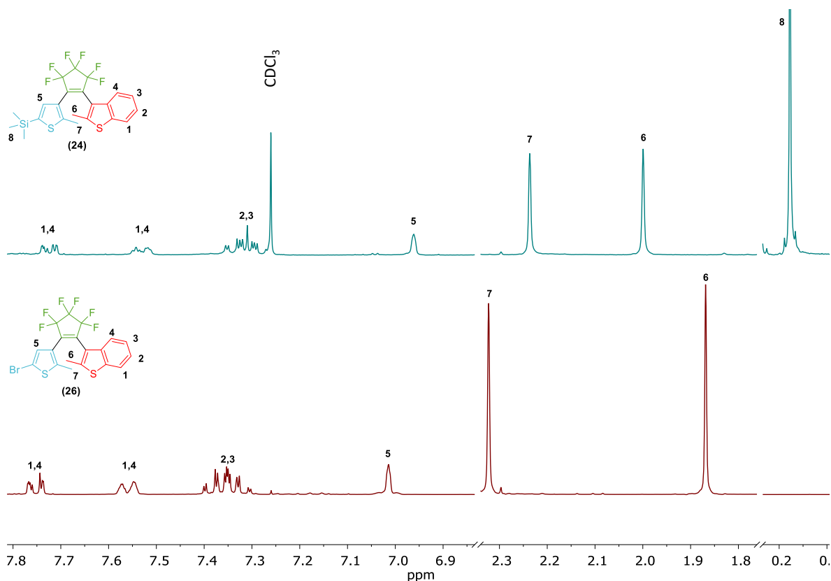
Figure 3.6. ^1\text{H} NMR spectrum of compound 26 . ( \text{CDCl}_3 , 300 MHz).
