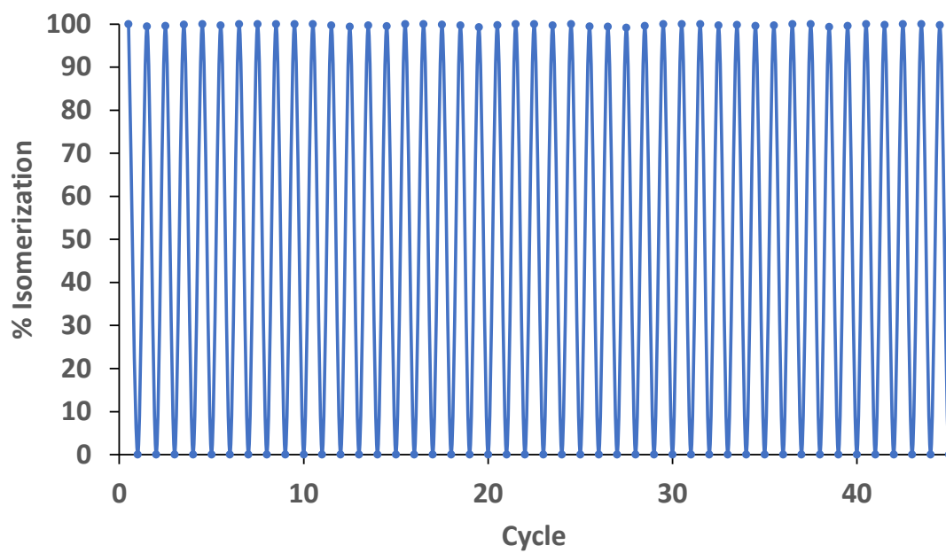
Figure S139. UV/Vis spectra of Ir-L3-B in CH 3 CN. Fatigue resistance experiment by irradiation at 370 nm, 1.9 \cdot 10^{-5} M
