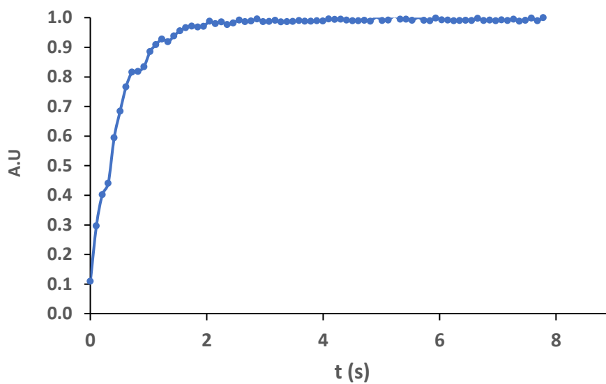
Figure S130. UV/Vis spectra of Ir-L3-A in \text{CH}_3\text{CN} . Photocyclization process by irradiation at 370 nm, 2.7 \cdot 10^{-5} \text{ M}
