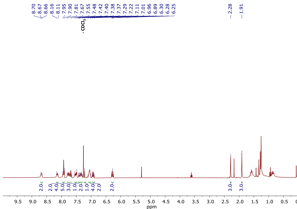
Figure S76. ^1\text{H} NMR of \Delta\text{-}[\text{Ir}(\text{ppy})_2(\text{L2-B})]\text{PF}_6 ( \Delta\text{-Ir-L2-B} ). ( \text{CDCl}_3 , 300 MHz).
