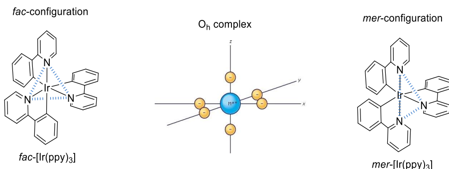
Figure 1.27. Graphical representation of the fac/mer configuration for O_h iridium complexes.
