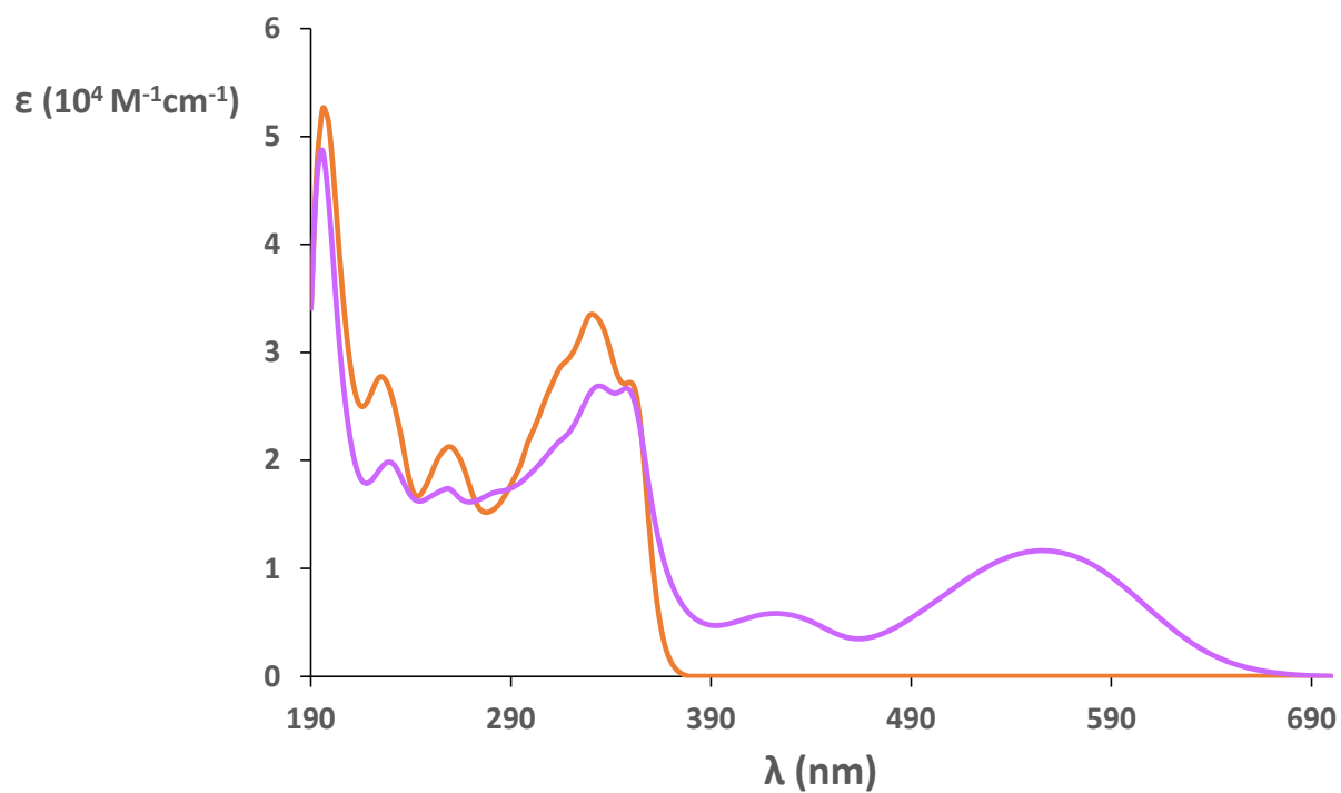
Figure S92. UV/Vis spectra of L2-B in CH 3 CN. Before (orange line) and after (purple line) irradiation at 370 nm, 5 \cdot 10^{-5} \text{M}
