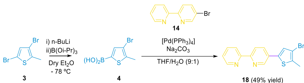
Scheme 3.6. Synthetic route for compound 18 .
