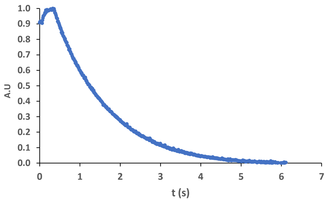
Figure S117. UV/Vis spectra of Ir-L2-A in \text{CH}_3\text{CN} . Photocycloreversion process by irradiation at 370 nm, 2.4 \cdot 10^{-5}\text{M}
