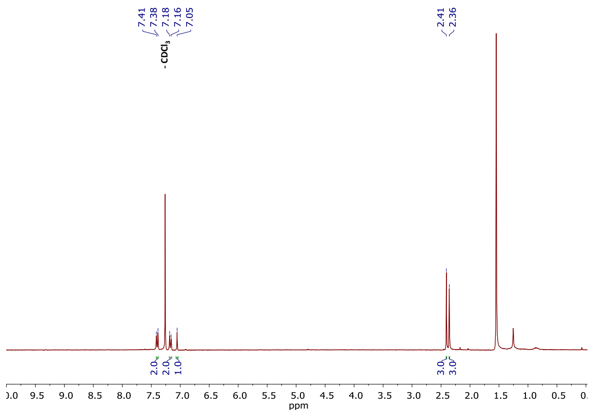
Figure S5. 1 H NMR of 3-bromo-2-methyl-5-(p-tolyl)thiophene (5). (CDCl 3 , 300 MHz).
