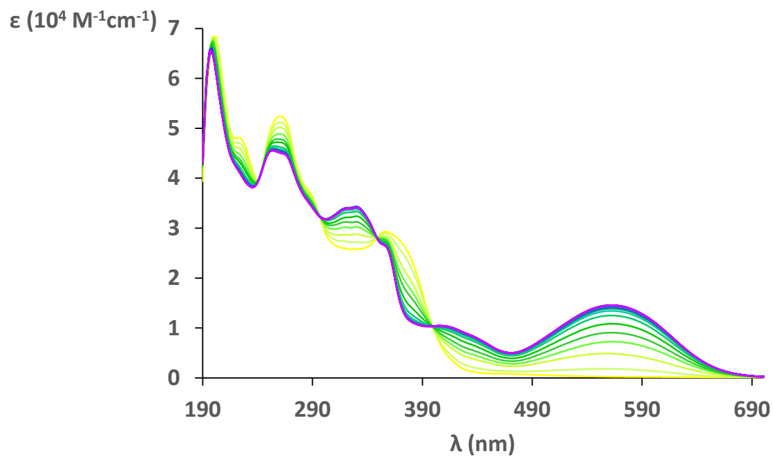
Figure S122. UV/Vis kinetic of Ir-L2-B in CH 3 CN irradiating at 370 nm, 5 \cdot 10^{-5} \text{ M}
