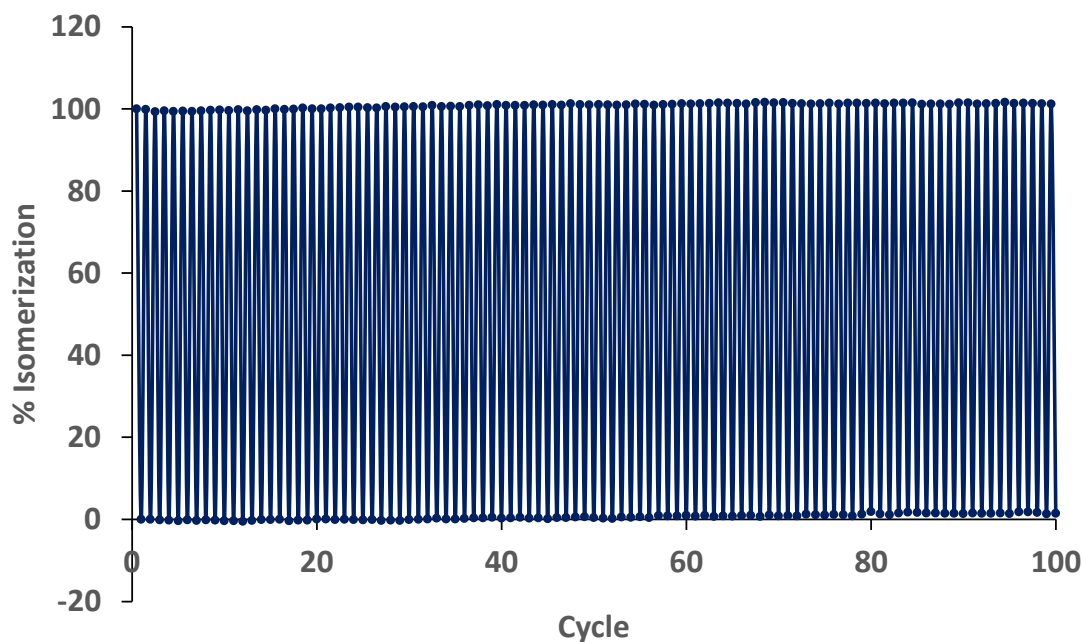
Figure 4.15. Photocyclusation ( \lambda_{irr} = 370 nm)-photocycloreversion ( \lambda_{irr} = 595 nm) cycles of L3-B , showing high fatigue resistance in \text{CH}_3\text{CN} .
