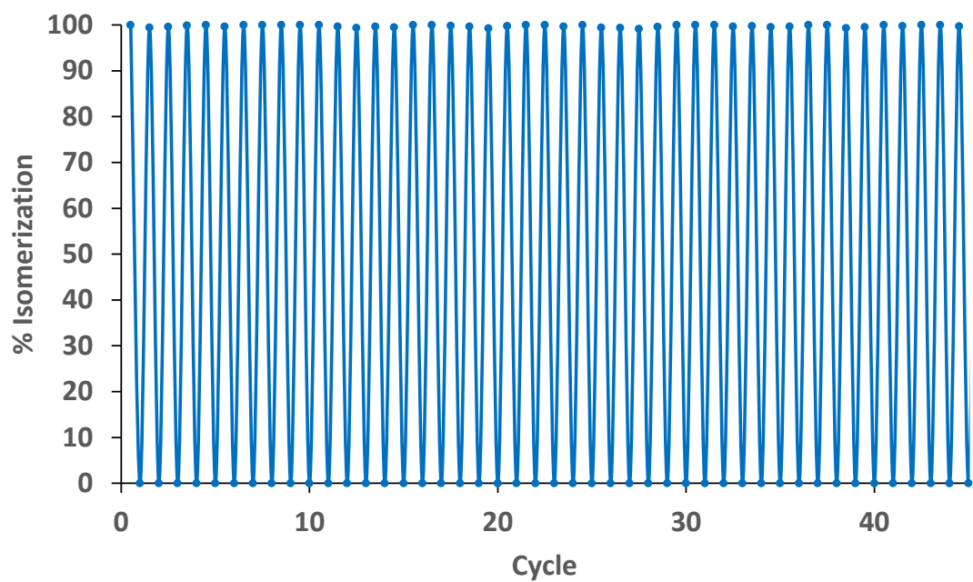
Figure S110. UV/Vis spectra of L3-B in CH 3 CN. Fatigue resistance experiment by irradiation at 370 nm and 595 nm alternatively, 2.7 \cdot 10^{-5} \text{M}
