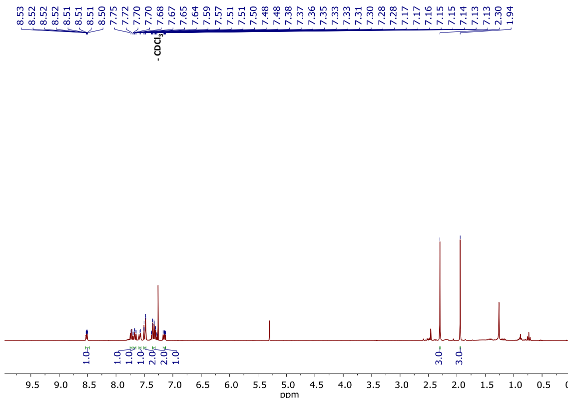
Figure S36. ^1\text{H} NMR of 2-(4-(3,3,4,4,5,5-hexafluoro-2-(2-methylbenzo[ b ]thiophen-3-yl)cyclopent-1-en-1-yl)-5-methylthiophen-2-yl)pyridine ( L1-C ) ( \text{CDCl}_3 , 300 MHz).
