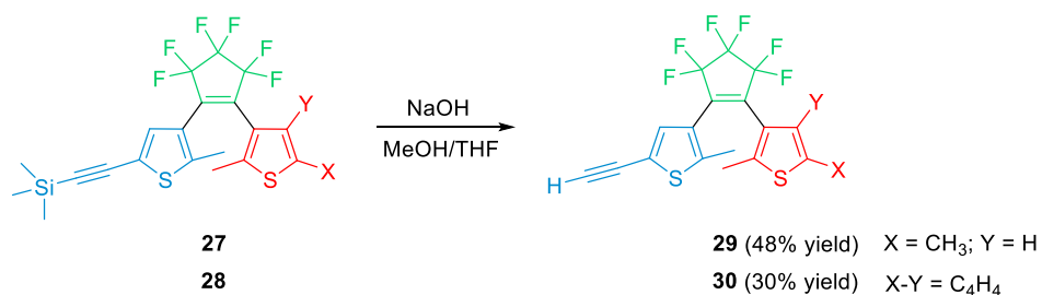
Scheme 3.13. Synthetic route for compounds 29-30 .
