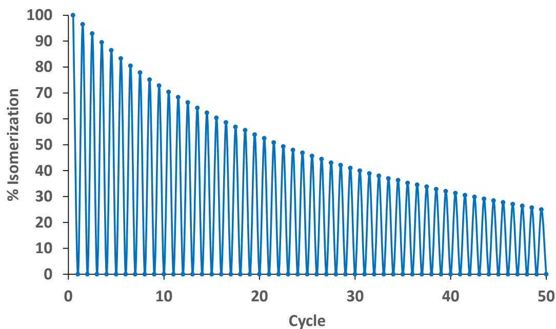
Figure S96. UV/Vis spectra of L2-B in \text{CH}_3\text{CN} . Fatigue resistance experiment by irradiation at 370 nm and 595 nm alternatively, 2.6 \cdot 10^{-5} \text{M}
