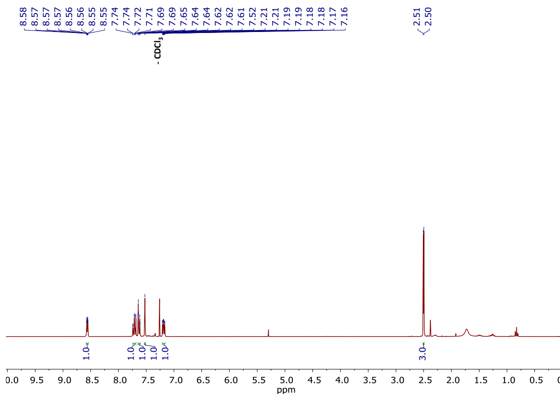
Figure S34. ^1\text{H} NMR of 2-(5-methyl-4-(perfluorocyclopent-1-en-1-yl)thiophen-2-yl)pyridine ( 11 ). ( \text{CDCl}_3 , 300 MHz).
