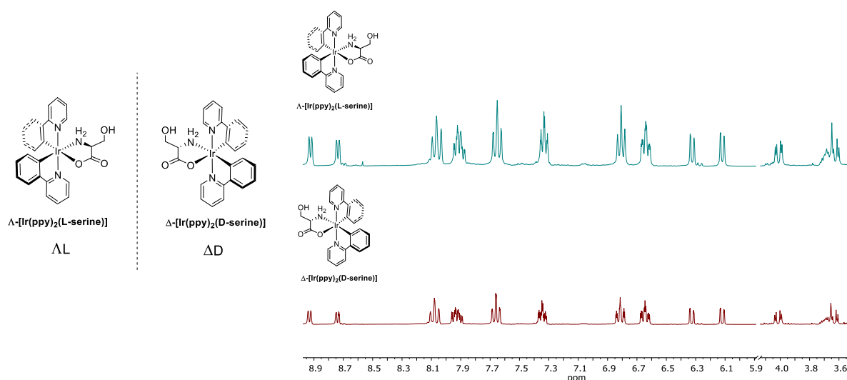
Figure 3.19. Comparison of ^1\text{H} -NMR \Delta\text{D}_{\text{serine}}\text{-C10} and \Lambda\text{L}_{\text{serine}}\text{-C10} . (MeOD, 300 MHz)
