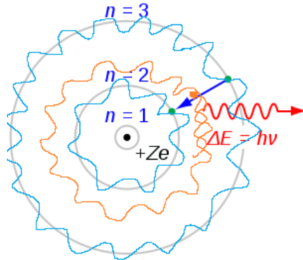
Fig 2.10. Visualization of a geometric interpretation of De Broglie's idea. The stable electronic orbitals of the atom are the ones where tuning of the phase wave of an electron with the length of the orbital matches (in blue). An electron orbiting a hypothetical orbital (in orange) would arrive out of phase at its starting point after a whole revolution (unstable orbital) and thus would lose energy and decay to a lower orbital. Source: Philippe Vincent.
