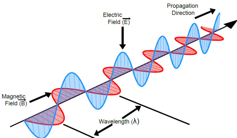
Fig. 1.5.2.a. Representation of an electromagnetic wave and its two components. The electric component is represented in blue and the magnetic component is represented in red. Source: Etienne Bonniec.
