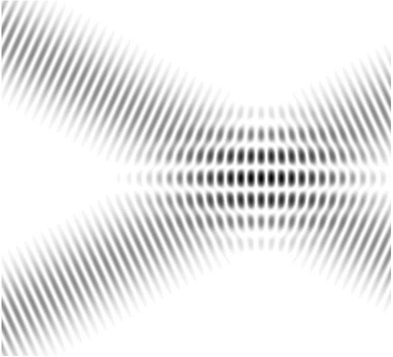
Fig. 1.7.4.b. Representation of two plane waves with different incident angles interfering and producing interference fringes. Public domain, Credit: “Ffred”.
