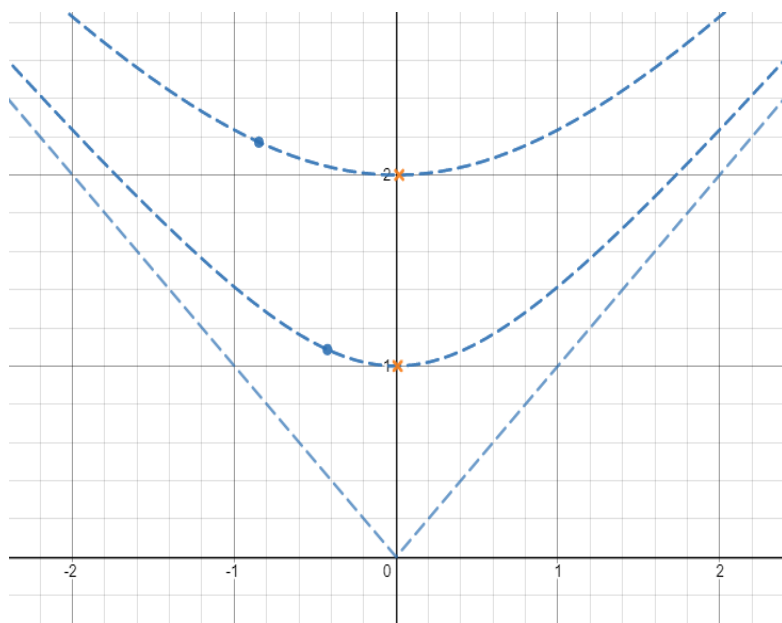
Fig. 3.2.1.1.h. Screenshot from a spacetime globe of the same situation as seen from the reference frame of the clock. In this diagram, the observer appears to be travelling at 0.4 c away from the clock.
