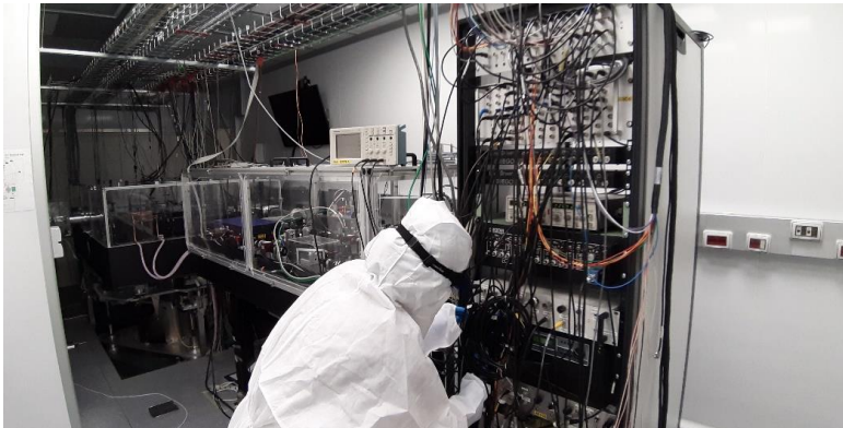
Fig. 6 Photo of Gabriel Pillant working in the clean room where the laser is located. The infrared laser (1064 nm) of the interferometer is inside the box on the left. The whole setup is located in a clean room to control the environment and avoid dust. Source: Photo taken by Philippe Vincent
