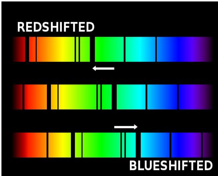
Fig. 5.3.g. Illustration of the redshift/blueshift of spectral lines compared to spectral lines as measured on Earth (middle spectrum). Source: https://sciencite.wordpress.com/2015/11/ | Public Domain
