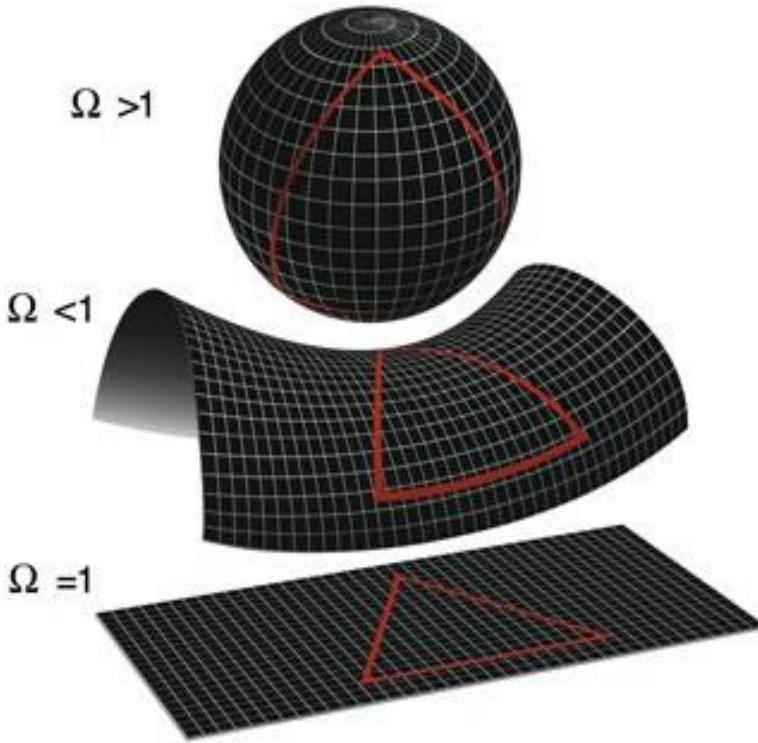
Fig. 5.3.i. 2-dimensional representations of the possible shapes of the universe. Adapted from Source: NASA / WMAP Science Team, Public Domain | https://wmap.gsfc.nasa.gov/universe/uni_shape.html
