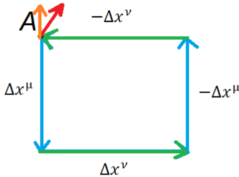
Fig. 3.2.2.d. Illustration of parallel transport of a vector (orange) associated to a point (A) along a closed path. The new (red) vector results from the parallel transport. Source: PV, made with MSPaint.
