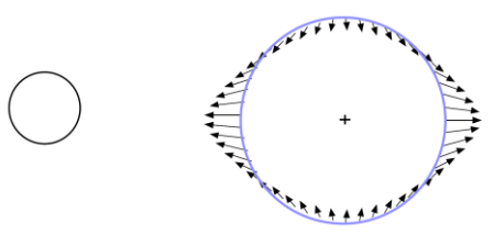
Fig. 1.9.4.3.c. Sketch of the Earth-Moon system double bulge of water due to the combined effects of gravity and inertia. Source: Etienne Bonniec.
