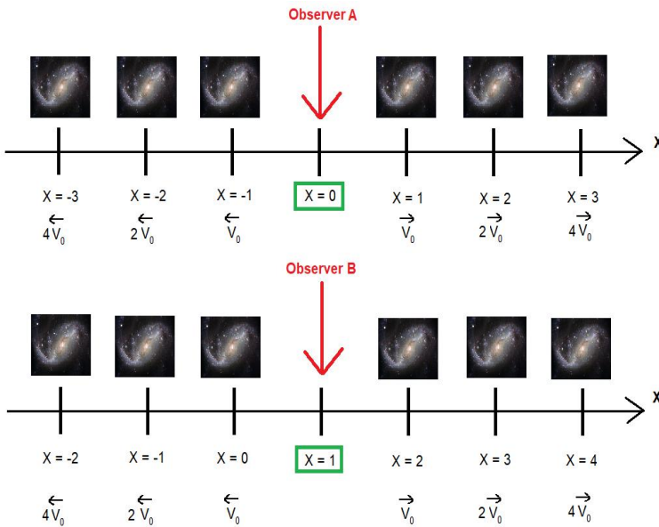
Fig 5.3.h. Illustration of the expansion of the Universe from the point of view of observers located in different galaxies. Source: PV, MS Paint.
