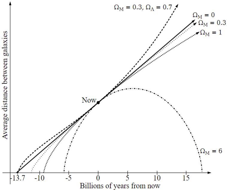
Fig. 5.3.j. Plot of the possible fates of the universe depending on matter density, \Omega_M and dark energy density, \Omega_\Lambda .
