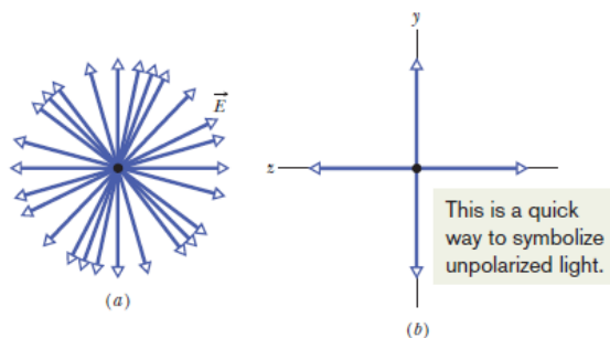
Fig. 1.3.2.c. Representation of what an observer (detector, eye, etc.) would see along the direction of motion of unpolarised light (a) and a simple way to symbolize unpolarised light.
