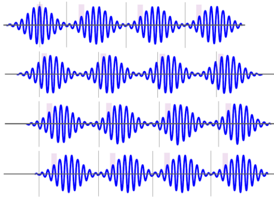
Fig. 1.2.c. Representations of wave packets (wave trains) with a direction of propagation to the right. Adaptation from a Mathematica plot. Source: Etienne Bonnet.
