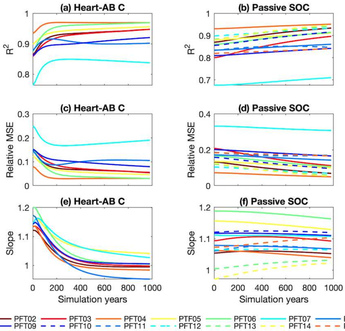
Figure S4.9 Evolution of the fitness of pool sizes from ML-based re-run to the “true equilibrium” state with increasing simulation years of re-run. Two pools, passive soil organic carbon (Passive SOC) and aboveground heartwood C (HeartAB C), were evaluated using three statistics that are the same with Figure S8.
