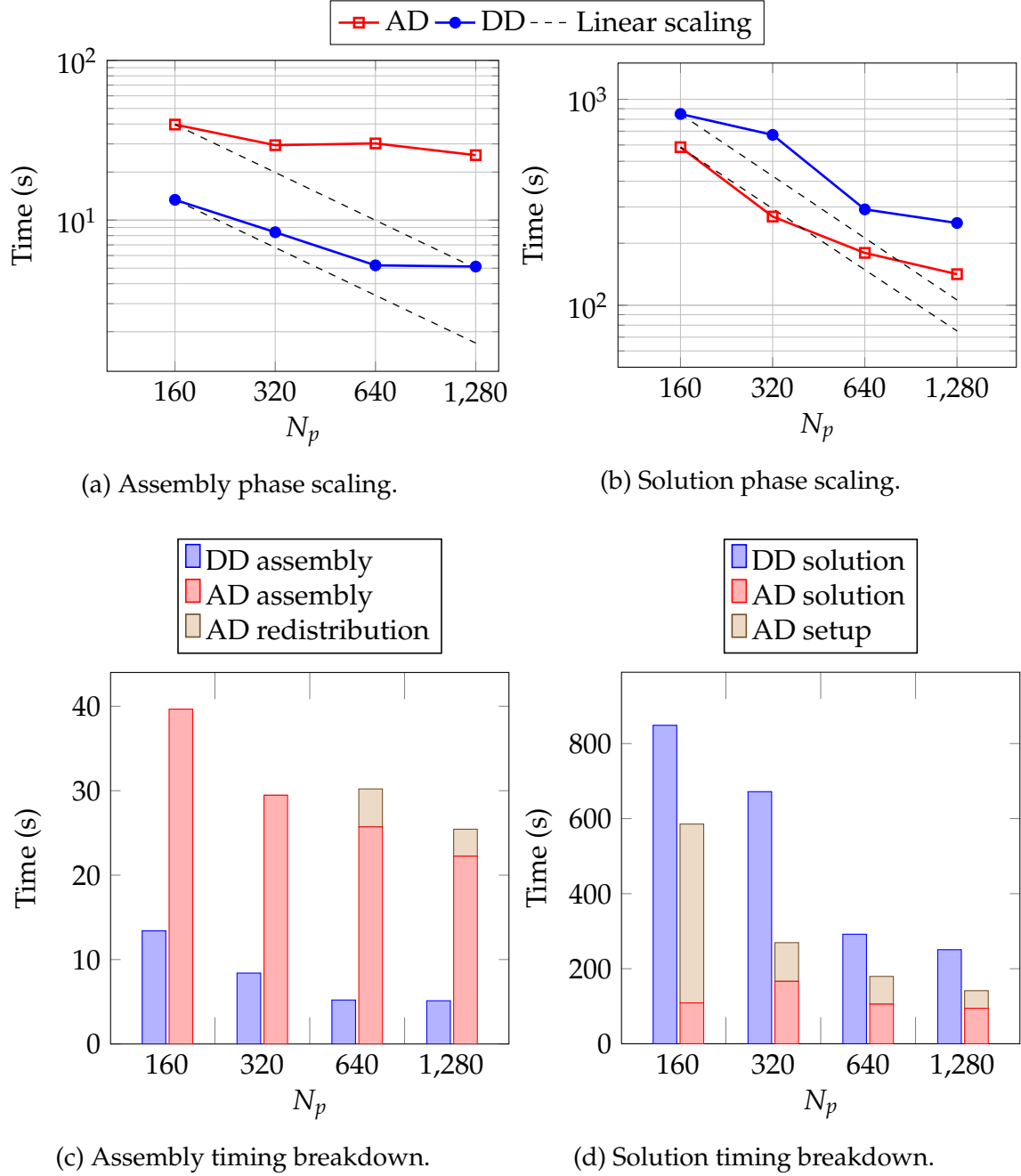
Figure 3.9: Scaling comparison between AD and DD for the three-dimensional test.
