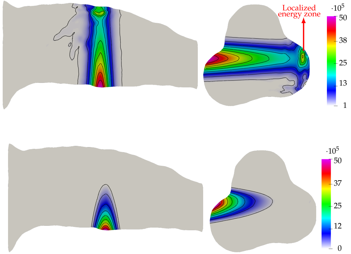
Figure 5.17: Radiative density fields G(x) within the \text{Al}_2\text{O}_3 ligament (top row) and the SiC ligament (bottom row) presented on the two orthogonal cross sections. G(x) is given in \text{W cm}^{-2} .
