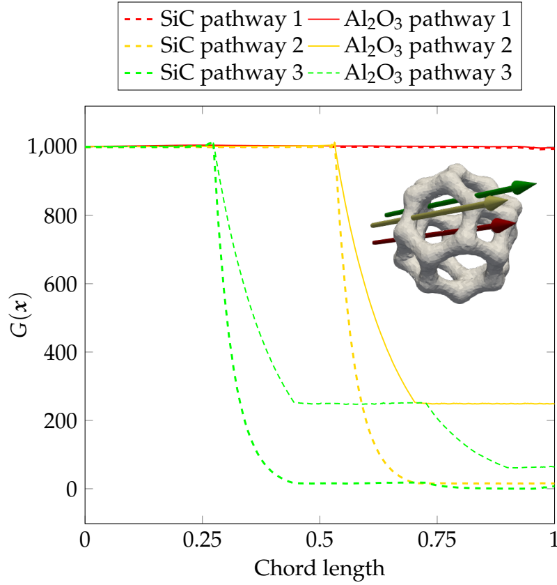
Figure 5.23: One dimensional radiative density plot along three different pathways within the Kelvin-cell for the SiC and the \text{Al}_2\text{O}_3 cases. G(x) is given in \text{W cm}^{-2} and the chord length is normalized from 0 to 1.
