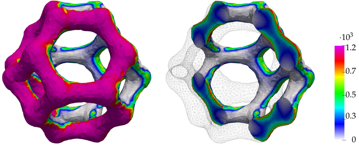
(a) The SiC based Kelvin-cell.
