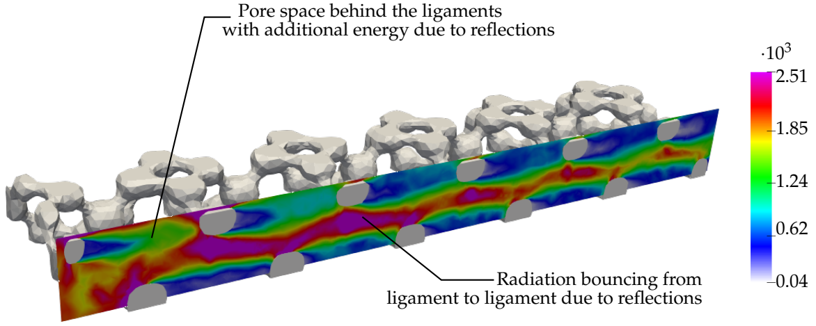
Figure 5.30: Radiative density field G(\mathbf{x}) on a sliced plane along the pore channel for a SiC based open-cell foam. G(\mathbf{x}) is given in \text{W cm}^{-2} .
