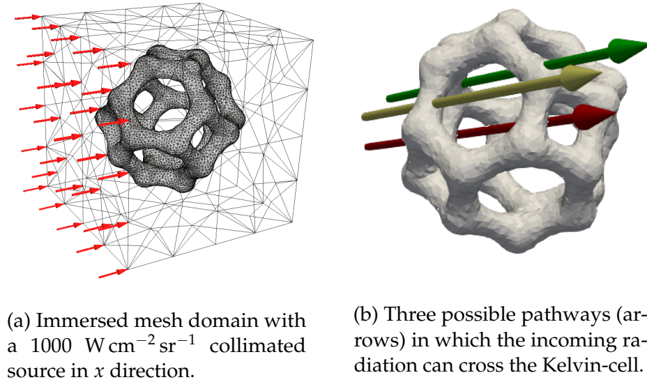
Figure 5.20: Immersed Kelvin-cell domain and the possible pathways for radiation within the cell domain. Red arrow represents pathway 1: radiation directly escapes without any contact with the ligaments, yellow arrow represents pathway 2: radiation comes in contact with one ligament before escaping, and green arrow represents pathway 3, radiation has to traverse through two ligaments before escaping.
