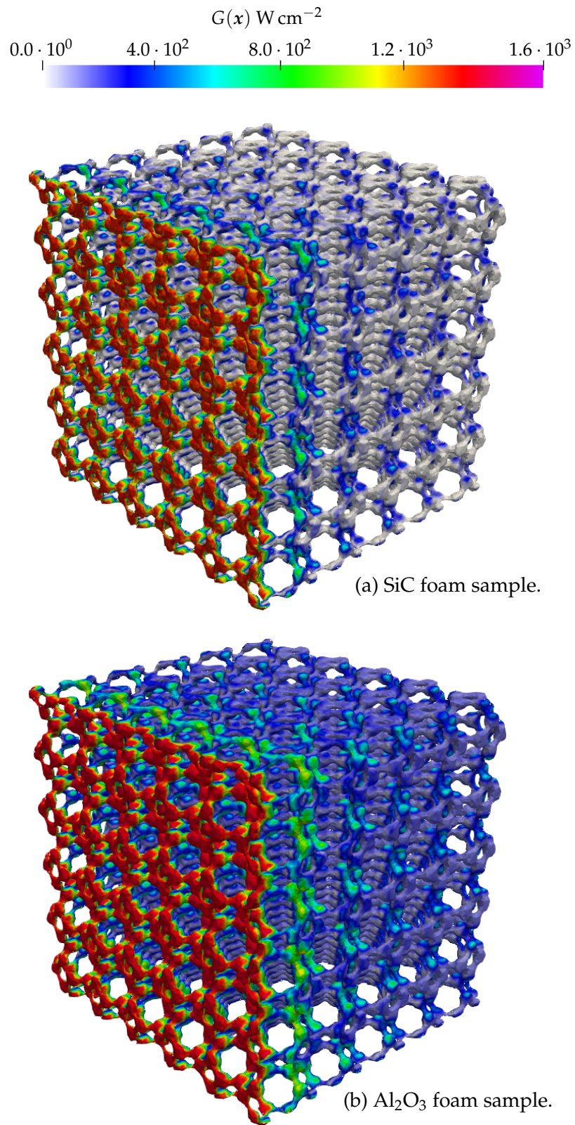
Figure 5.26: Radiative density fields for Kelvin-cell based open-cell foams under collimated radiation.
