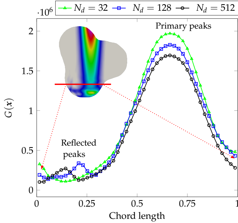
Figure 5.15: One dimensional radiative density plot for the Al_2O_3 ligament simulated using different directions. G(x) is given in W\,cm^{-2} and the chord length is normalized from 0 to 1.
