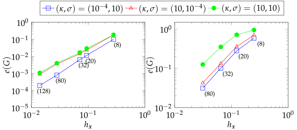
Figure 5.3: Spatio-angular mesh convergence for the vectorial FEM. Left: 2D test, right: 3D test. The numbers in the braces are the number of directions N_d used for each test.
