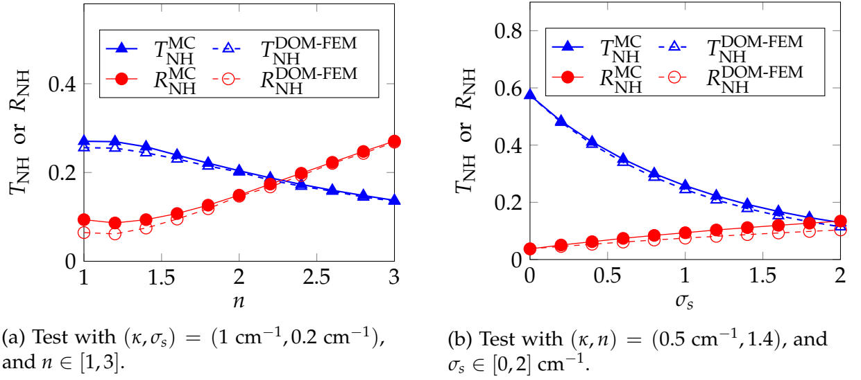
Figure 5.7: Normal hemispheric transmittance and reflectance for 3D test cases.
