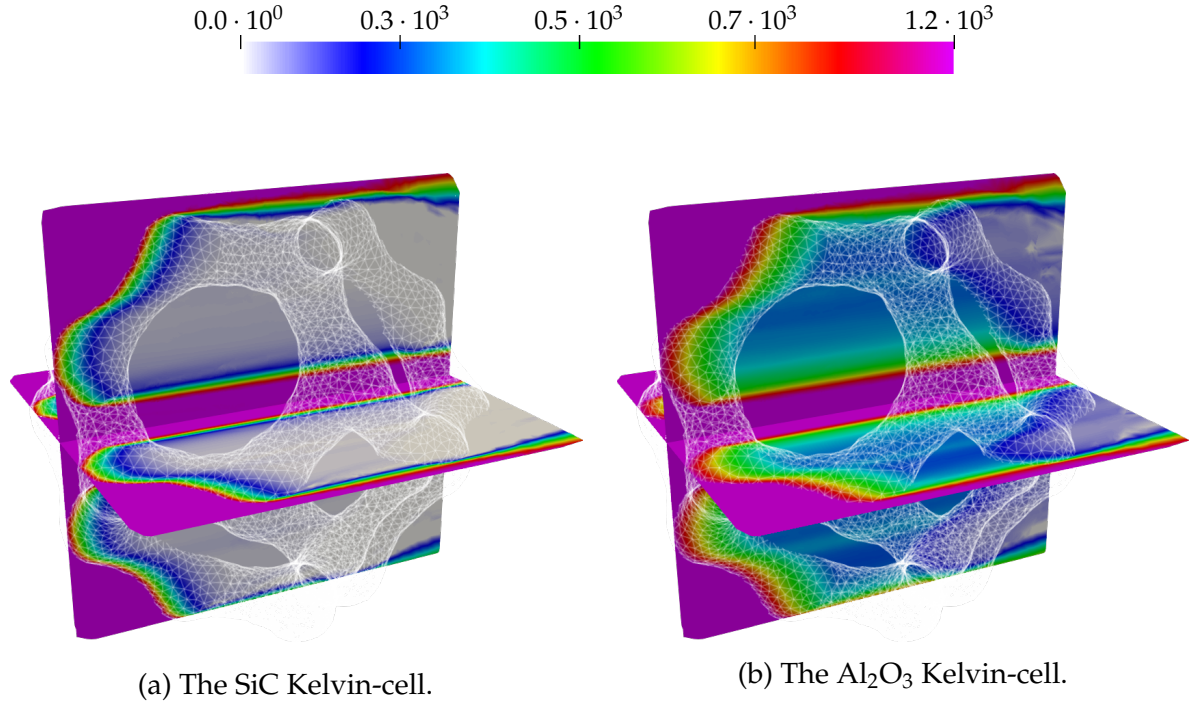
Figure 5.22: Sliced section view of radiative density fields on two orthogonal planes within the SiC and the \text{Al}_2\text{O}_3 based Kelvin-cells under collimated radiation. Radiative density G(x) is given in \text{W cm}^{-2} .
