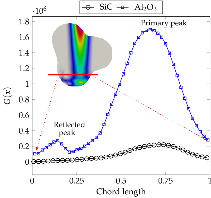
Figure 5.16: One dimensional radiative density plot comparing the SiC ligament to the Al_2O_3 ligament. G(x) is given in W\,cm^{-2} and the chord length is normalized from 0 to 1.
