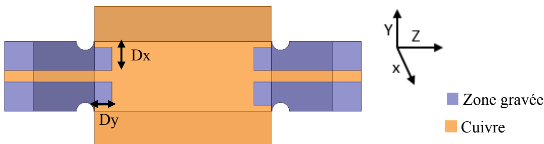
Figure III-15- Excitation micro-ruban
