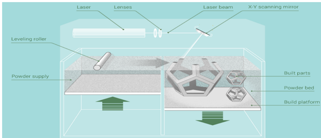
Figure I-37 - Laser sintering [31]
