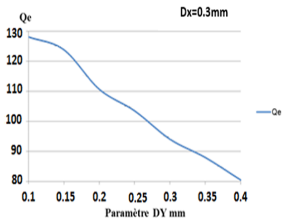
Figure III-17- Variation de Q_e de D_y
