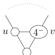
Figure 1.6 – A semi-weak neighbor v of u .
