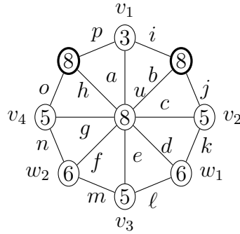
Figure 1.62 – Notation for Lemma 1.58
