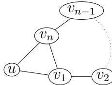
Figure 1.26 – Configuration of Lemma 1.20
