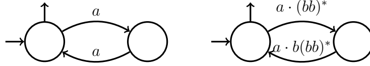
Figure 3.9 – Running example of Subsection 3.3.4
