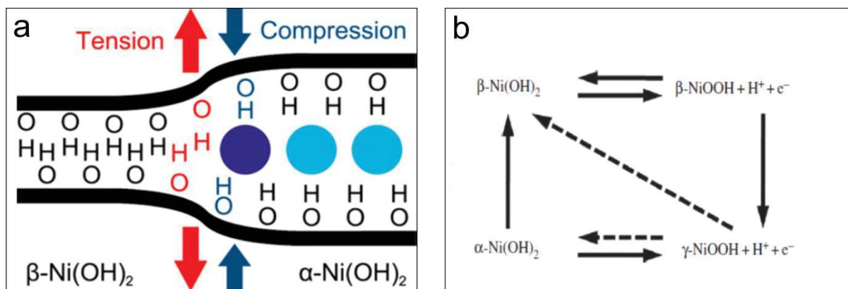
Fig. 1.5 (a) Schematic representation of the \alpha/\beta -phase transition. Blue circles represent water molecules located between the \text{NiOH} layers in \alpha\text{-Ni(OH)}_2 . Given from the Ref. [104]; (b) A general scheme of the chemical and electrochemical processes that occur on the surface of Ni electrode in the high-potential region. Given from the Ref. [65].
