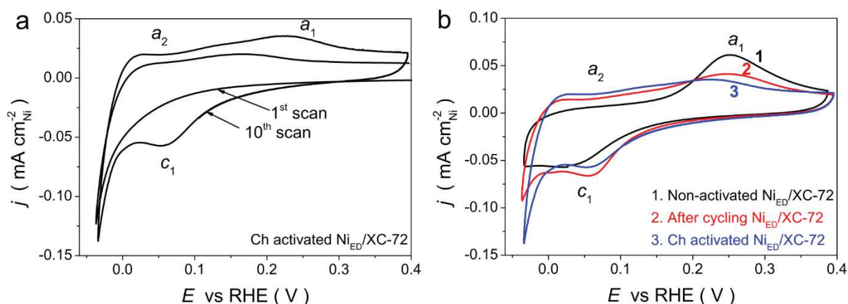
Fig. 4.10 (a) CVs obtained for Ch activated \text{Ni}_{\text{ED}}/\text{XC-72} just after an immersion of the electrode in \text{N}_2 -saturated 0.10 \text{ M NaOH} at \nu = 20 \text{ mV}\cdot\text{s}^{-1} ; (b) Comparison of the CVs registered for non-activated \text{Ni}_{\text{ED}}/\text{XC-72} electrode before (curve 1, black) and after (curve 2, red) cycling in the potential interval of [-0.06 - 0.40 \text{ V}] and Ch activated (curve 3, blue) \text{Ni}_{\text{ED}}/\text{XC-72} electrode.
