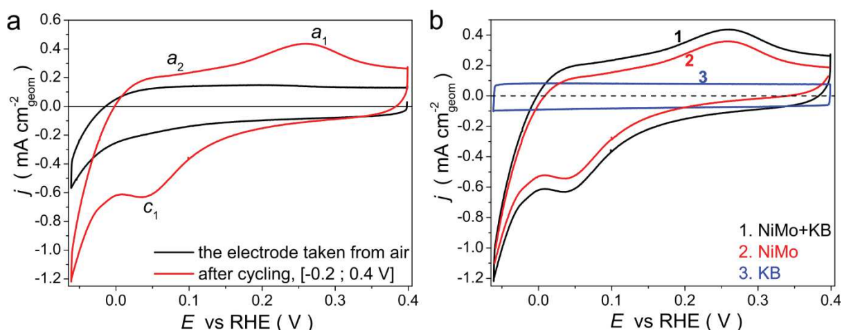
Fig. 5.12 (a) CVs obtained in N_2 -saturated 0.10 M NaOH at v = 20 \text{ mV} \cdot \text{s}^{-1} for Ni_{0.90}Mo_{0.10}/C sample after its immersion in the electrolyte (black curve) and after electrochemical reduction of its surface (red curve); (b) Comparison of CVs obtained for Ni_{0.9}Mo_{0.1}/C ( 100 \mu\text{g cm}^{-2}_{geom} , curve 1, black) and KB carbon support ( 50 \mu\text{g cm}^{-2}_{geom} , curve 3, blue); in addition, the CV obtained after subtraction of the currents corresponding to the KB support (curve 2, red) is presented.
