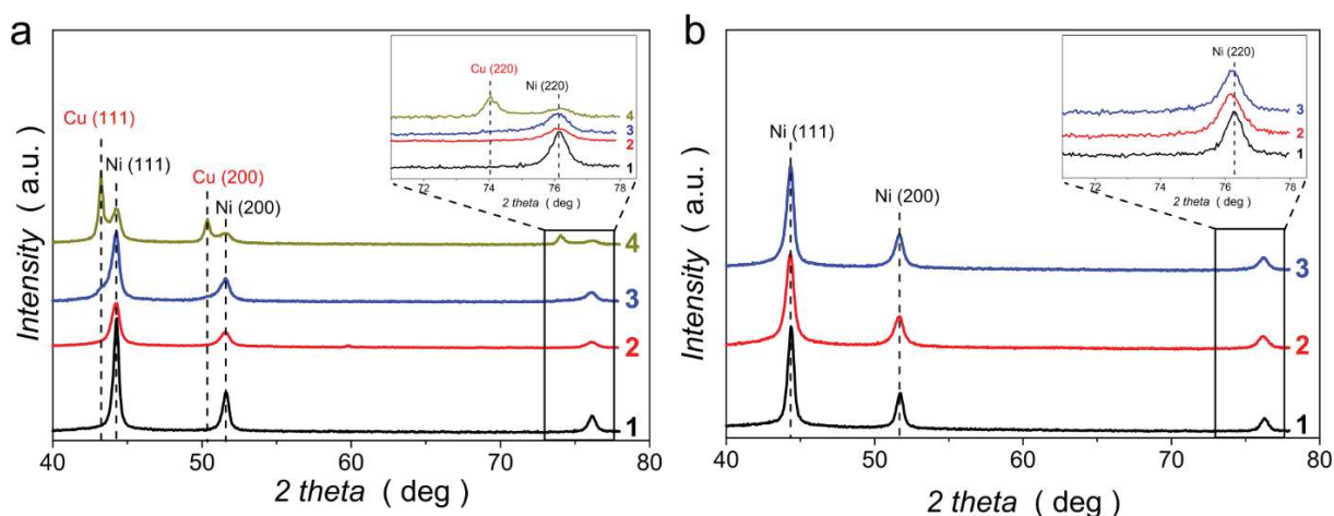
Fig. 5.3 XRD patterns for (a) \text{Ni}/\text{C} (1), \text{Ni}_{0.95}\text{Cu}_{0.05}/\text{C} (2), \text{Ni}_{0.80}\text{Cu}_{0.20}/\text{C} (3), \text{Ni}_{0.50}\text{Cu}_{0.50}/\text{C} (4) and (b) \text{Ni}/\text{C} (lyo) (1), \text{Ni}_{0.95}\text{Cu}_{0.05}/\text{C} (lyo) (2), \text{Ni}_{0.90}\text{Cu}_{0.10}/\text{C} (lyo) (3). Insets on the panels zoom into selected areas corresponding to the Cu (220) and Ni (220) diffraction peaks.
