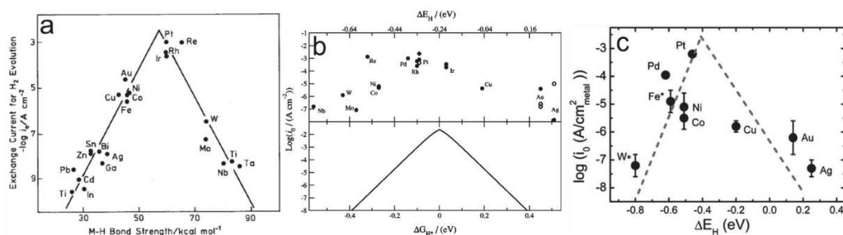
Fig. 1.1 Exchange current density of the HER (in acidic (a, b) and alkaline (c) medium) plotted as a function of \text{M-H}_{\text{ad}} binding energy (a, given from the Ref. [18]) or free energy of adsorption of \text{H}_{\text{ad}} atoms on the catalyst (b and c, given from the Refs. [22,23]).
