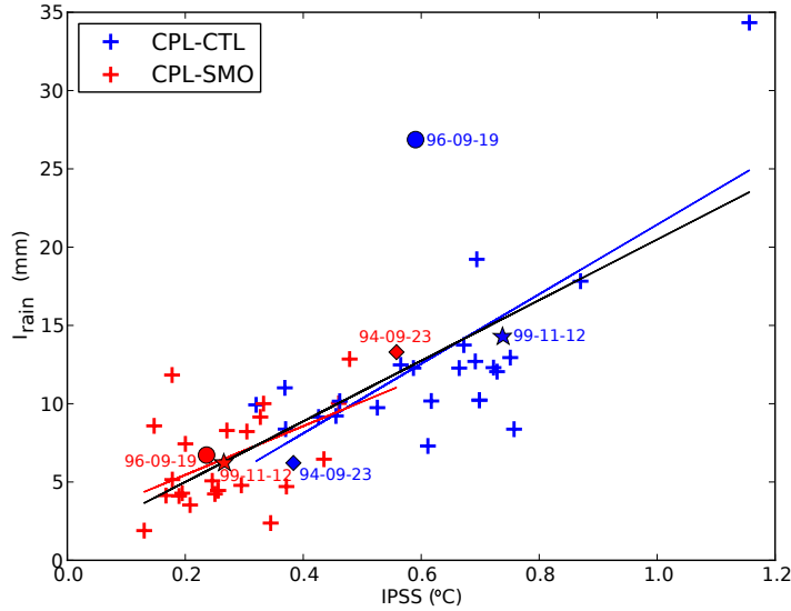
Fig. 4.10 Index of the precipitation difference ( I_{rain} ) (mm) as a function of the coupling index IPSS ( ^{\circ}C ) for the 22 strongest events represented by the model in the Cevennes area. Each event is represented by one red and one blue crosses : red crosses represent the calculation of I_{rain} and IPSS for CPL-SMO and blue crosses for CPL-CTL. Moreover, 3 cases among the 22 are highlighted : squares show the case of 23 September 1994, discs the case of 19 September 1996 and stars the case of 12 November 1999.
