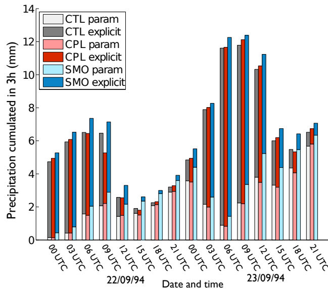
Fig. 4.5 Precipitation cumulated every 3h (RR3) averaged over the Cvn box shown in Fig. 4.6a. C_v = convective rain (resulting from the parametrization scheme), Non C_v = rain resulting from resolved processes in CTL, CPL and SMO simulations; no graupel was recorded.
