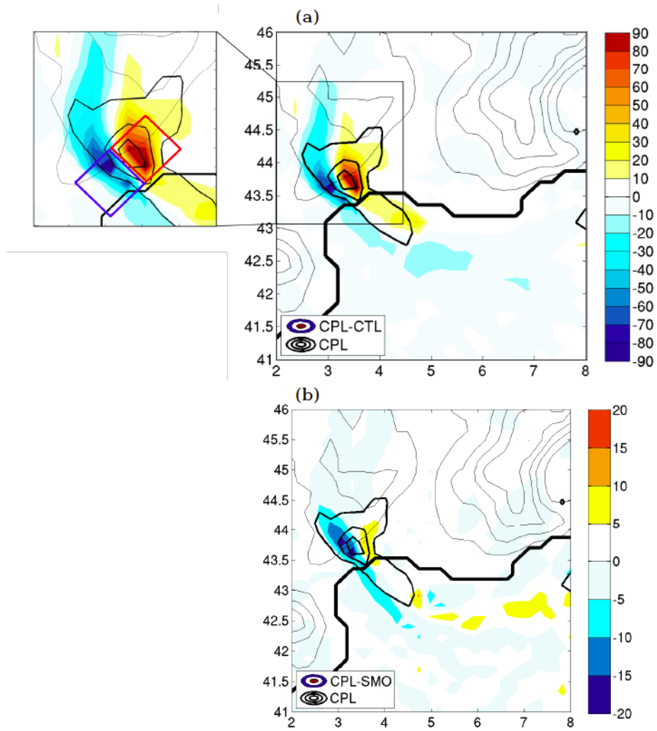
Fig. 3.5 daily precipitation on the 19 September 1996 ( \text{mm dy}^{-1} ): a. colours: difference between CPL and CTL; b. colours: difference between CPL and SMO; a-b. thick contours: CPL ( 50 \text{ mm dy}^{-1} ) (note the difference in colour scales)
