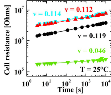
Figure 2.11: Resistance evolution over time for devices integrating GST (black circle), GST+5%C (blue square), GST+8%C (red triangle) and GST+15%C (green triangle) [107]. The drift coefficient \nu is decreased for carbon-doped GST-based devices w.r.t. undoped devices.
