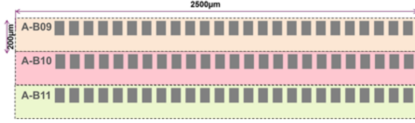
Figure 4.16: Scribe lines of the on-wafer pulse generator.
