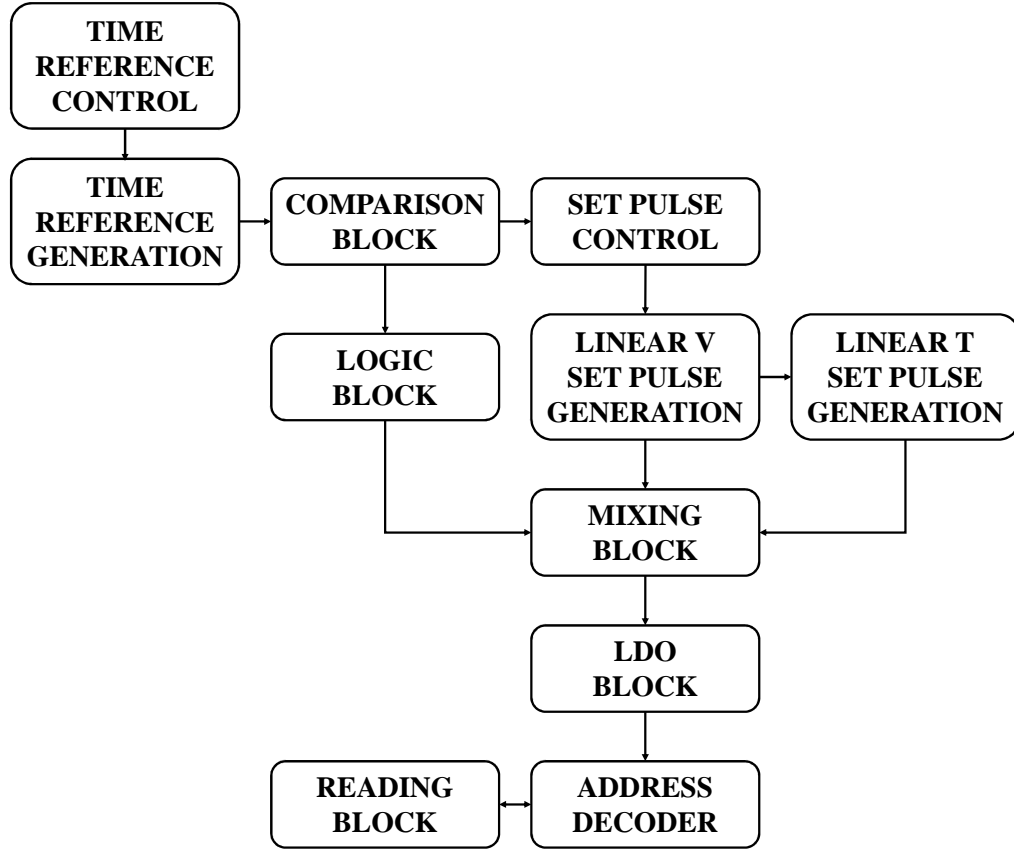
Figure 4.3: Block diagram of the on-wafer implementation of the R-SET pulse generator.
