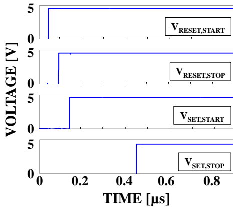
Figure 3.6: Input signals of the Logic Block. The signals are generated by the Comparators Block and their duration is controlled by reference voltages V_{REF,i} .
