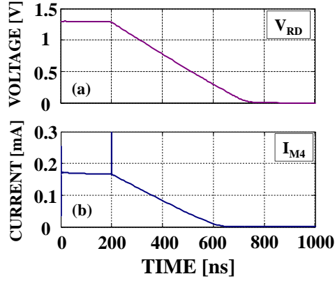
Figure 3.18: Simulated waveforms of the linearly decreasing (a) voltage pulse V_{RD} and (b) current through the drain of transistor M_4 , I_{M4} (first design).
