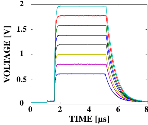
Figure 4.37: Measured RESET pulses with varying amplitude.
