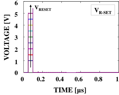
Figure 3.13: Simulated single RESET pulse sequence ( V_{SET} = 0 ): an increasing amplitude of the RESET pulse is obtained by increasing voltage V_{RESET} .
