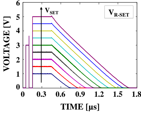
Figure 3.12: Simulated R-SET pulse sequence: an increasing SET pulse amplitude is obtained by increasing voltage V_{SET} .
