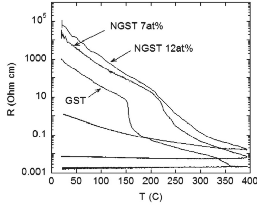
Figure 2.7: Resistivity of GST and N-doped GST films as a function of temperature [110]. Resistivity increases in both phases in N-doped GST films, while no formation of the hcp phase for temperatures of up to 400 °C can be observed.
