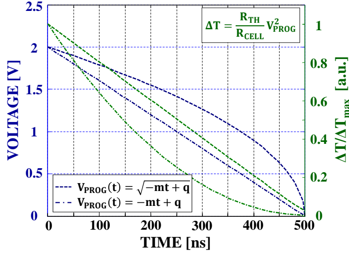
Figure 3.15: Relationship between the voltage applied to the cell (blue curves) and the temperature increment \Delta T = T - T_{\text{EXT}} developed in the active material (green curves): corresponding curves are drawn with the same line pattern. A linear voltage decrease does not guarantee a linear temperature decrease.
