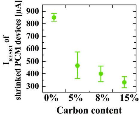
Figure 2.10: RESET current, I_{\text{RESET}} of shrunken PCM devices for varying carbon content. A RESET current reduction, resulting in a RESET power reduction, can be clearly seen as carbon doping increases. An I_{\text{RESET}} reduction of up to 61% can be obtained on GST+15%C-based devices [107].
