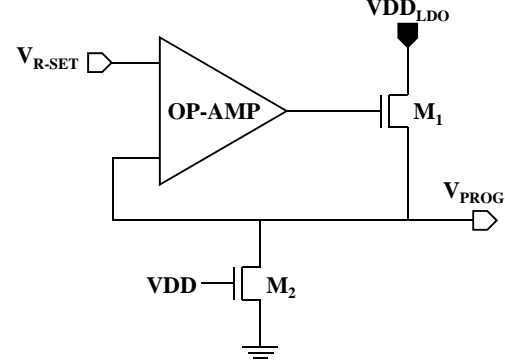
Figure 4.11: Circuit schematic of the unity-gain buffer (LDO Block).
