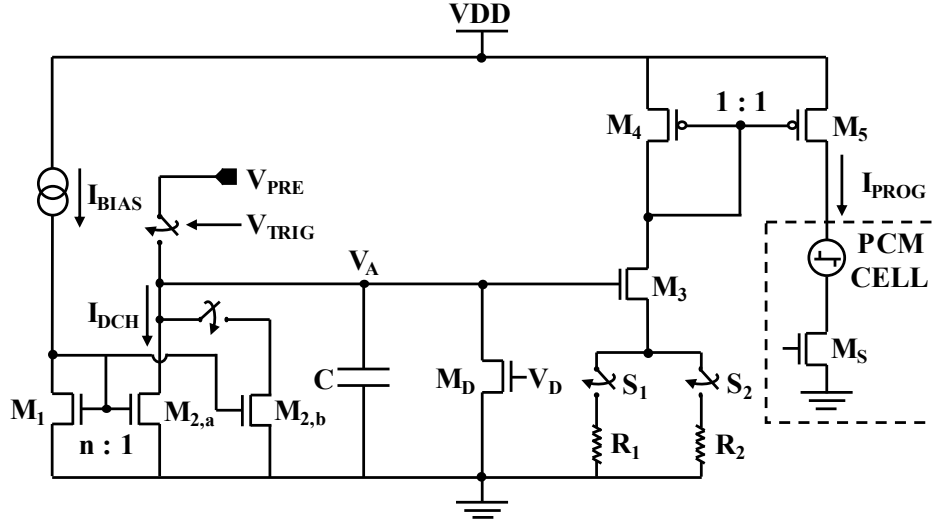
Figure 3.27: Circuit schematic of the proposed current pulse generator for MLC programming.
