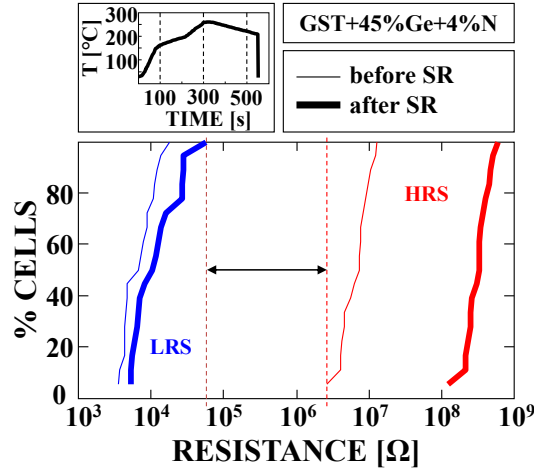
Figure 2.20: Soldering Reflow (SR) procedure applied to the HRS and the LRS of GST+45%Ge+4%N. A window of more than one order of magnitude is preserved after the application of the Soldering Reflow temperature profile (top left corner).
