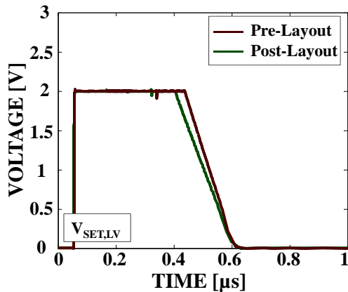
Figure 4.26: Schematic and post-layout simulations of the SET pulse with a linear voltage decrease.
