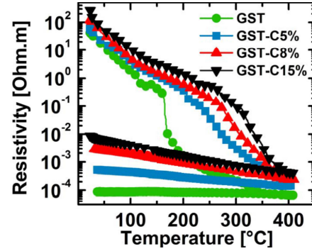
Figure 2.9: Electrical resistivity of GST and carbon-doped GST as a function of temperature [107]. The transition between the amorphous and the crystalline phase is smoother for C-doped GST. Crystallization temperature increases with increasing C content.
