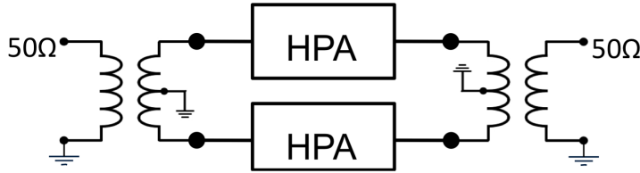
Figure 3.25: Elementary HPA combined with baluns -
