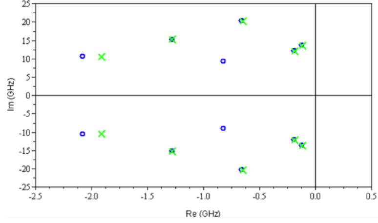
Figure 4.17: Bilbao stability analysis : 10 to 20 GHz, pertubator at drain -
