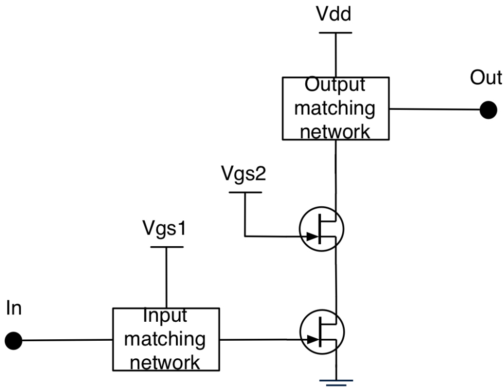
Figure 2.19: Cascode power amplifier -
