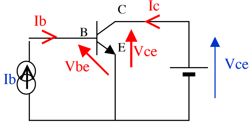
Figure 2.5: Heterojunction bipolar transistor -
