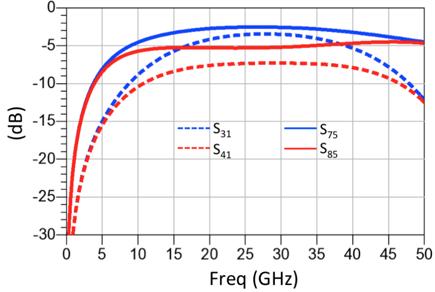
Figure 3.20: Comparaision of energy transfer between planar and vertical coupling -
