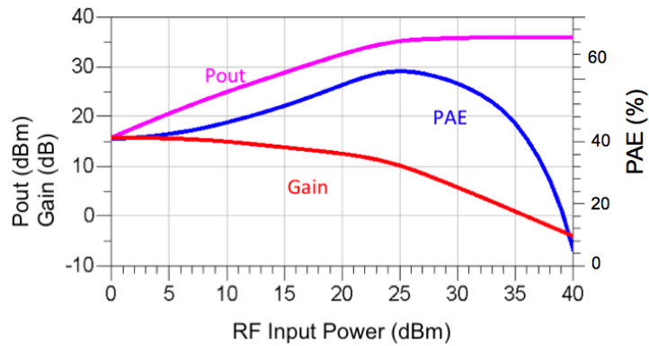
Figure 4.7: Non linear simulation results for an 8*125\mu\text{m} device at 10GHz -
