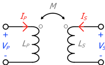
Figure 3.5: Transformer representation -
