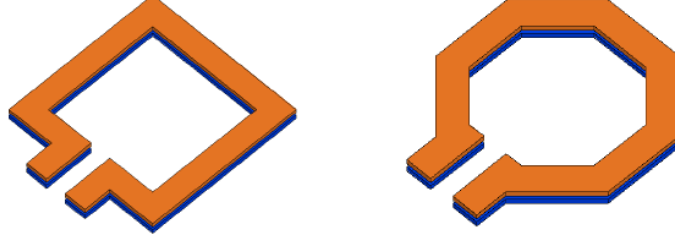
Figure 3.26: Elementary balun shapes : rectangular (left) and circular (right)
