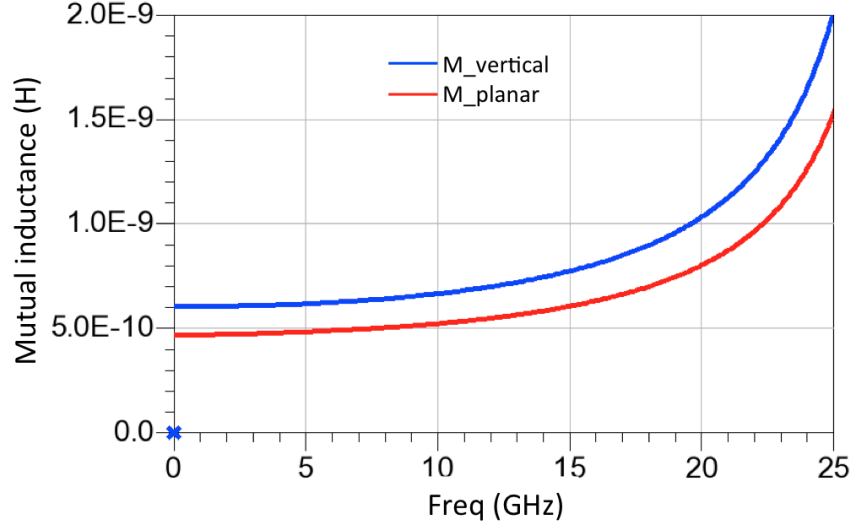
Figure 3.22: Comparaision of mutual inductance between planar and vertical coupling -
