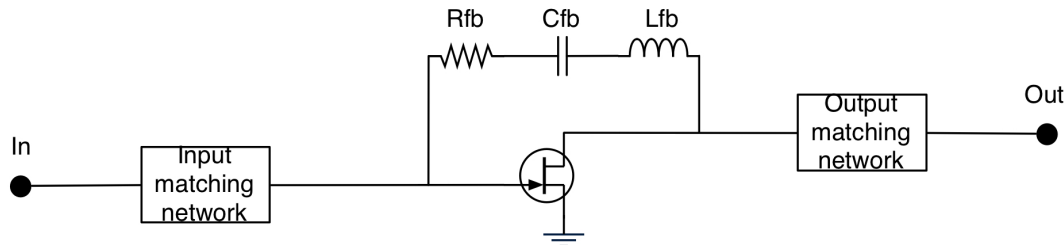
Figure 2.24: Feedback amplifier -
