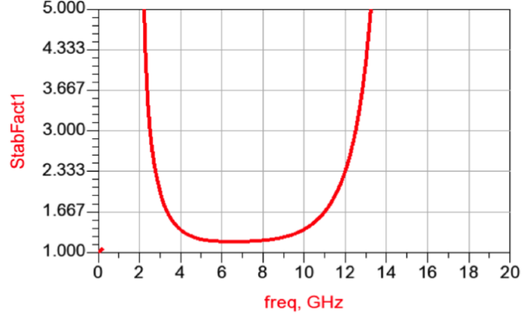
Figure 4.14: Rollet factor from DC to 20GHz -
