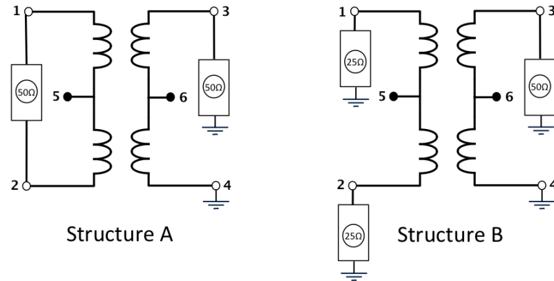
Figure 3.24: Optimal impedances for a balun with a transformation ratio of one -
