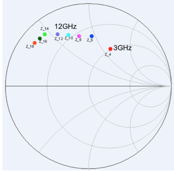
Figure 4.9: 8 \times 125 \mu\text{m} device selected optimal impedances in Smith chart -
