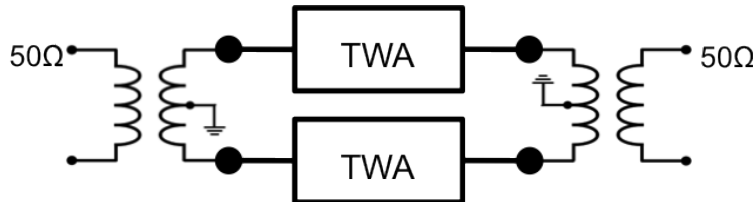
Figure 4.48: Differential TWA representation -
