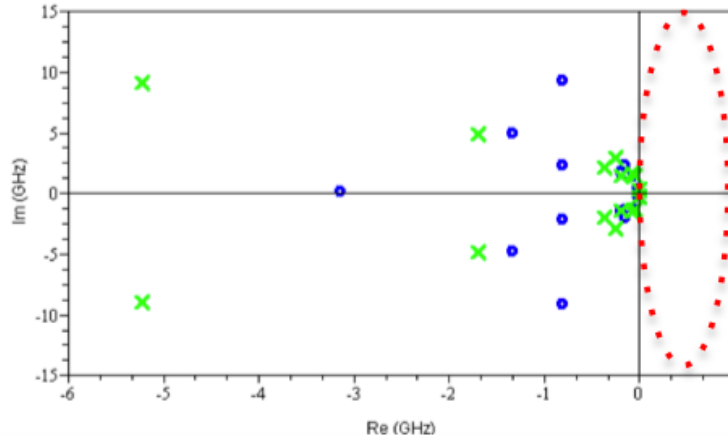
Figure 4.15: Example of a Bilbao stability analysis -
