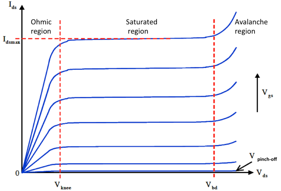
Figure 2.9: Output static characteristic of an HEMT transistor -
