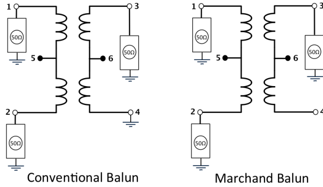
Figure 3.30: Conventional and Marchand balun architecture -
