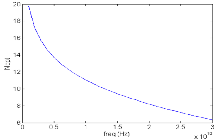
Figure 4.40: Optimal number of cells vs. maximal frequency of operation -
