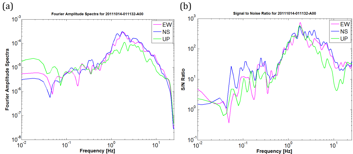
Figure 3.5: (a) FAS and (b) SNR for the event no. 12 (ML=3.5) at the central station, A00, of Array A.
