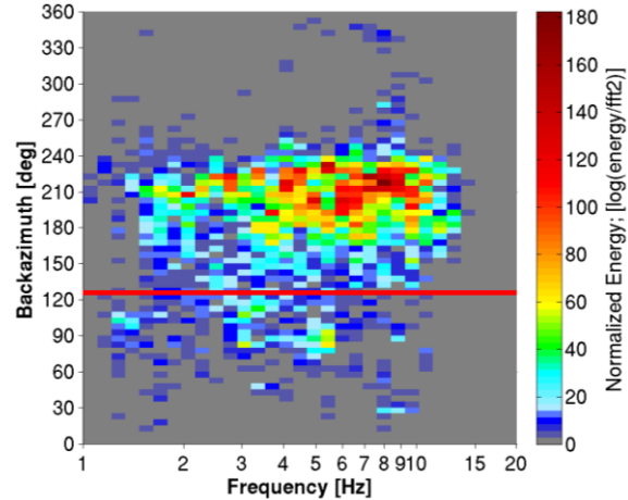
Figure 3.8: Identified back-azimuth distribution of the dominant waves, for event 12, propagating across the Array A. (a) Location of the event with respect to the central station A00. (b) Identified back-azimuths as function of time with colorbar indicating normalized energy as estimated in Equation 3.26. (c) Histogram of identified back-azimuths as a function of frequency with colorbar indicating the summation of normalized energy as estimated in Equation 3.29. Red line indicates the back-azimuth of the event.
