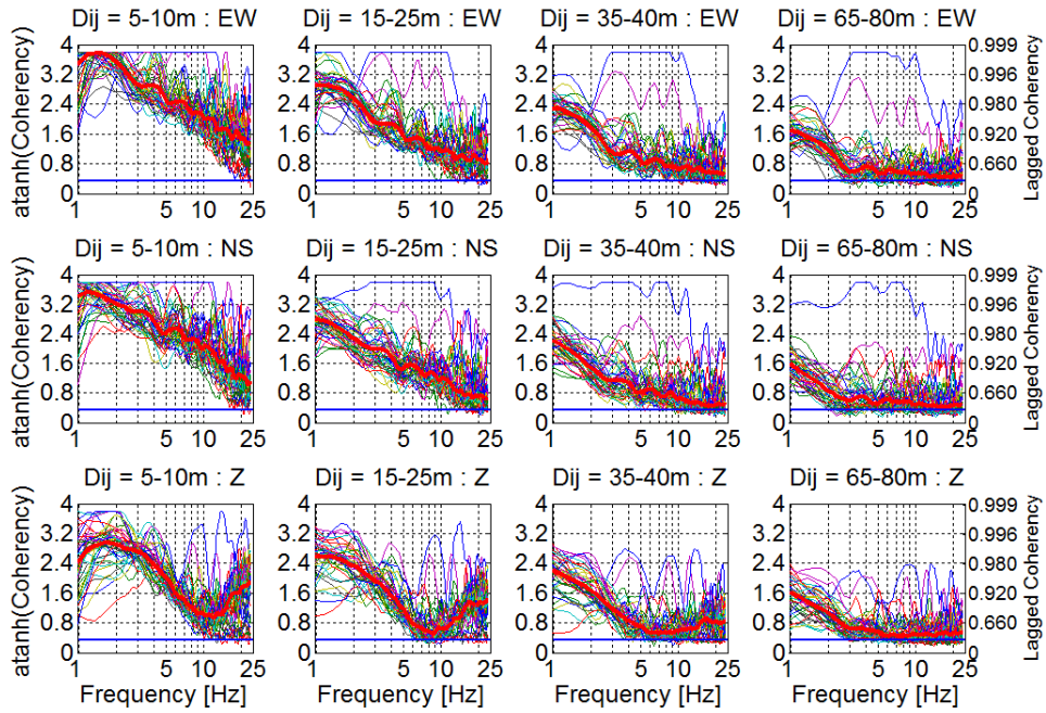
(b) Residual
