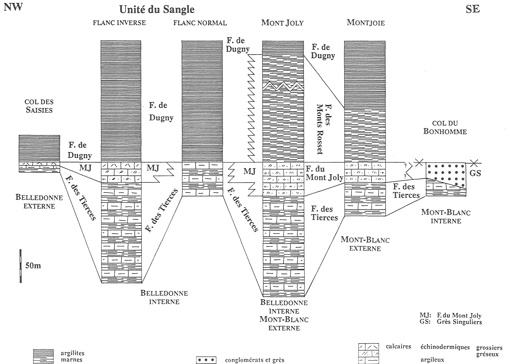
Fig. 12. Lias, variations transversales
