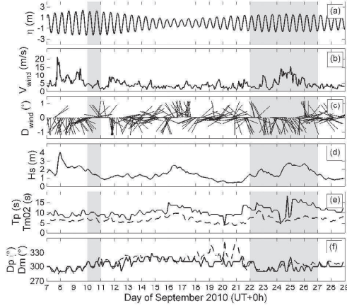
Figure 3. Environmental conditions during the LOREA 2010 field experiment. (a) Water elevation \eta measured by Socoa tide gauge inside the bay. (b) Wind velocity V_{wind} and (c) wind direction D_{wind} measured by the Socoa meteorological station (Météo France). (d) Offshore significant wave height H_s ; (e) offshore peak period T_p (full line) and mean period T_{m,02} (dashed); (f) offshore peak direction D_p (full line) and mean direction D_m (dashed). Offshore wave data are measured by the Donostia directional buoy, located 30 km off the bay at (-2.0126°E, 43.56°N). Shaded areas: periods of interest.
