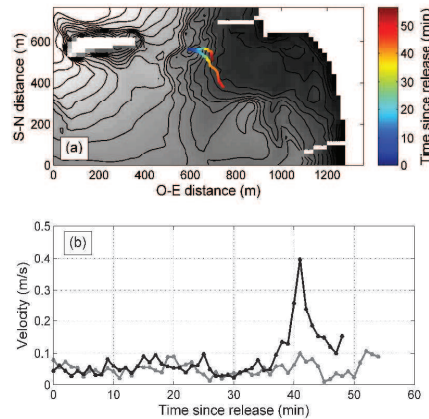
Figure 9. (a) Trajectories of the two surface drifters released in the vicinity of the surf zone at low tide, with the colorscale indicating the time after the release. Representation is centered on the northeastern part of the bay. Grayscale indicates the bathymetry, with isobaths plotted in black every 1 m. (b) Velocity estimated along the trajectories. Northern trajectory is in gray, southern trajectory is in black. Velocity computation is based on 60 s-averaged drifter locations.
