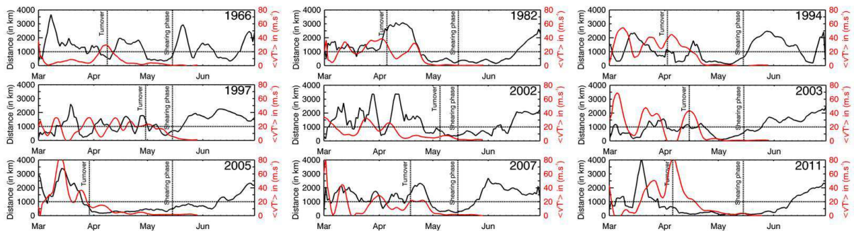
Figure 6. Distance L_{GPH-PV} (in km) between the geopotential height maximum and the PV minimum northward of 70^{\circ}\text{N} (black curve) at 850 K from the March 1 to June 30 for the years 1966, 1982, 1994, 1997, 2002, 2003, 2005, 2007 and 2011. Also shown is the zonal-
