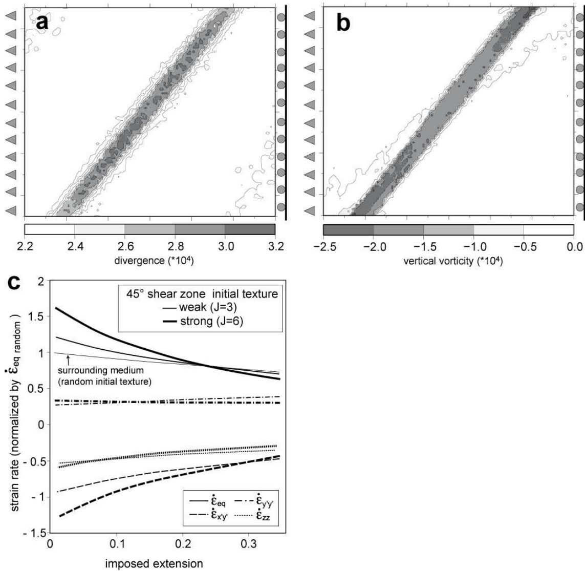
Supplementary Figure S3: Results for a model with an 'inherited wrench fault' (thick lines) at 45^\circ to the imposed extension (geometry and boundary conditions as in Fig. 1), but with an initial texture twice as strong ( J=6 ) as the one presented in Figs. 1 & 2 ( J=3 ). The J index is a measure of the texture concentration based on the integral of the orientation distribution function. For comparison, naturally deformed peridotites have J indexes ranging from 2 to 26, with a peak at 8^2 . Poloidal and toroidal partitioning, represented as maps of the divergence (a) and vorticity (b) of the horizontal flow field, respectively. Higher divergence marks localization of the poloidal flow in the inherited texture domain. Toroidal flow is restricted to the inherited texture. Flow in the surroundings is purely poloidal, in agreement with the boundary conditions (extension parallel to the X direction). Note that the divergence and vorticity variation ranges are respectively 2 and 3 times larger than those in the 45^\circ model with a weaker initial texture
