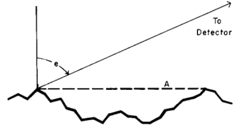
Figure E.14 – (Hapke, 1984)
