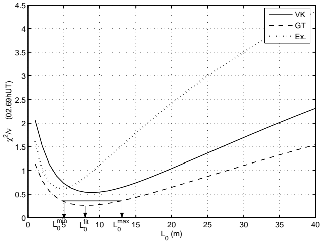
Figure 2. Example of \chi^2_{\nu} obtained with normalized covariances measured at 02.69hUT for several models of turbulence in function of the outer scale value.
