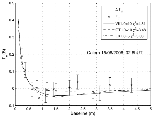
Figure 3. Example of normalized AA longitudinal covariances (star plot) measured at Calern the 15th June 2006 (2.6UT) and error bars calculated with Eq.7. Theoretical covariances are fitted with the WLSF method in order to minimize the \chi^2 . It gives an estimation of the outer scale for each model.
