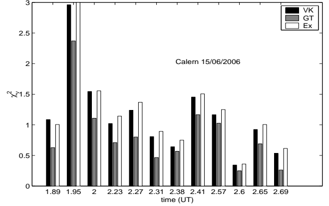
Figure 4. Minimal \chi^2_{\nu} obtained during GSM acquisitions the 15th June 2006 for the vK model (black chart), GT model (grey chart) and exponential model (white chart). In this night, GT is the most suitable model as it gives minimal \chi^2 but some acquisitions shows significant departure from all of these usual outer scale model.
