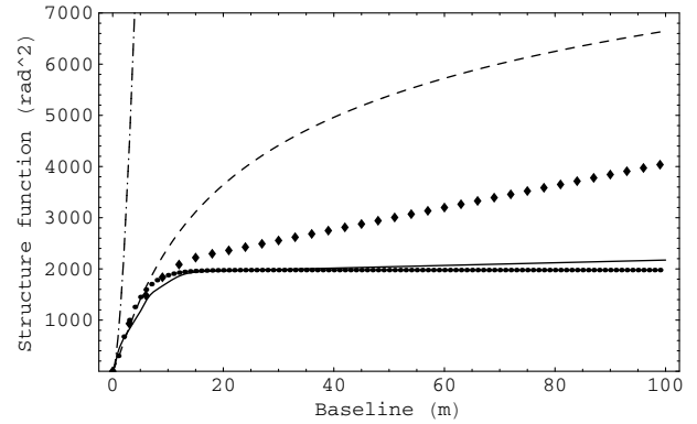
Fig. 4. Same than Fig. 3. The diamond plot correspond to an artificial increase of 0.5\lambda of the \sigma_{OPD} for a baseline of 15.2 m (see text). The von Kármán and Greenwood-Tarazano models have been obtained with \mathcal{L}_0 = 17 m and r_0 = 6.23 cm.
