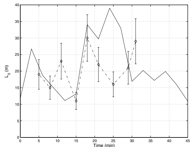
Fig. 5. Comparison of outer scale \mathcal{L}_0 measurements obtained with the GSM (solid line) and derived from the GI2T interferometer data (diamond dots) during the night of June 7th 2003. Origin is at 0h36' UT.
