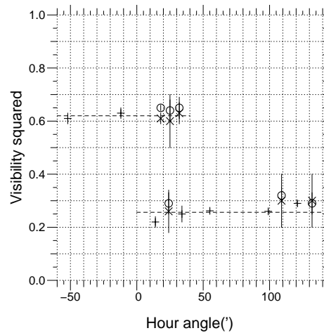
Figure 7. Natural (+), High (o), and Low (x) squared visibility versus hour angle obtained on \alpha Lyr (top) and on \alpha Cep (bottom) during the July 29, 2004 observations. The dash on the visibility curves gives the average of the Natural squared visibility for each data set. \alpha Lyr visibilities squared have been shifted by 0.5. Visibilities are not calibrated but only corrected for main instrumental effects (see Appendix B).
