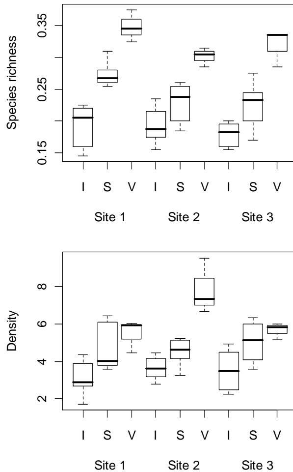
Figure 4: Boxplots of species richness per transect (in number of species per m 2 (top) and abundance density per transect (in number of individuals) per m 2 (bottom) per site and transect type. “I”, “S” and “V” respectively denote I-type, S-type and UVC transects. I-type and S-type respectively refer to straight and browsing transects (see § 2.1). For each boxplot, the thick line in the box corresponds to the median value, the lower and upper limits of the box correspond to the 25% and 75% percentiles of the data. The plot whiskers extend out from the box to the most extreme data point which is no more than 1.5 times the interquartile range from the box and all values were plotted.
