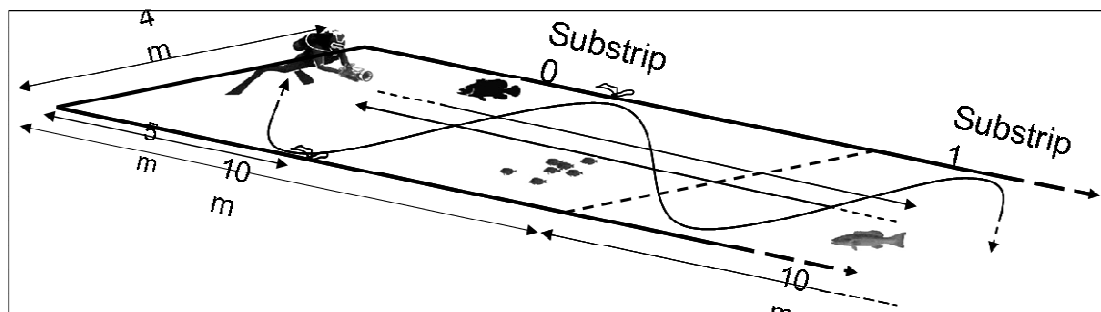
Figure 2: Sketch of the transect area. The transect area was delineated by bands around the 50 m per 4 m area, and additional bands were set every 10 m inside the transect area. In addition to UVC, two transect types were used : one with the diver swimming along a straight trajectory (I-type) and one with the diver browsing through the transect area (S-type) (see § 2.1).
