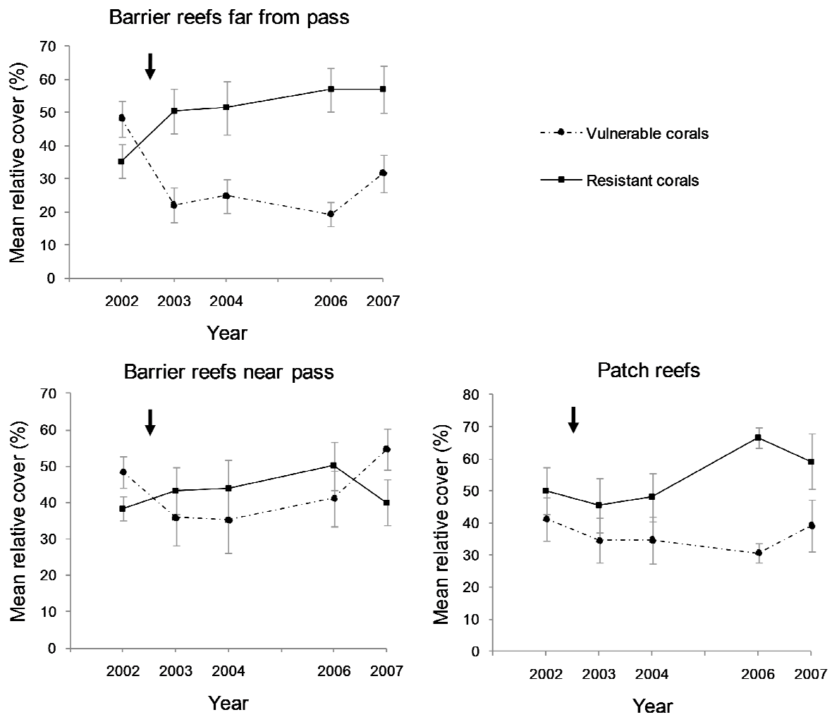
Figure 3: Temporal variations in the mean relative cover (as a percent of total live hard coral cover) of two coral types (resistant and vulnerable), for three reef types, between 2002 and 2007. Error bars indicate 95% confidence intervals. Arrows indicate the occurrence of the cyclone.
