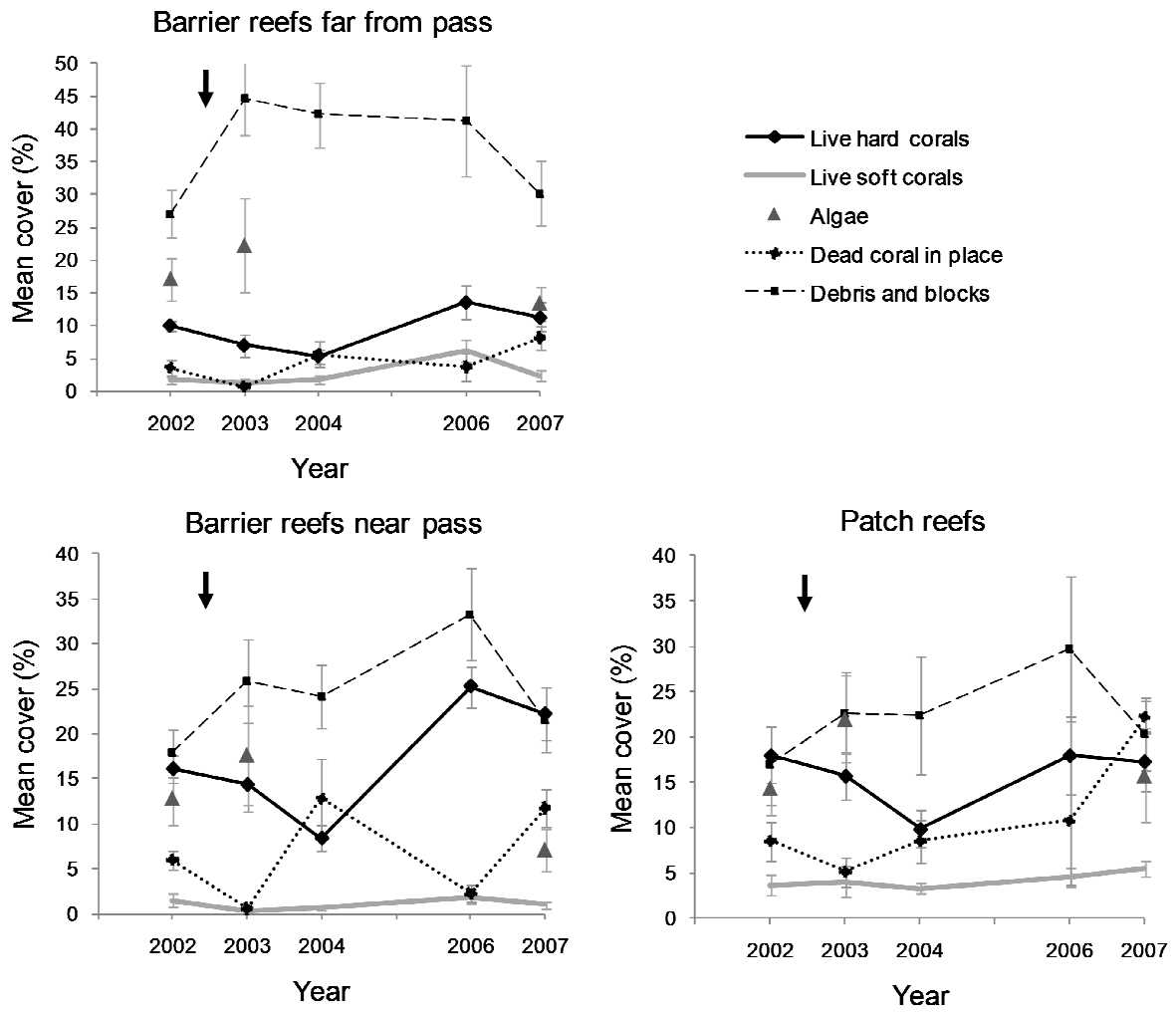
Figure 2: Temporal variations in the mean percent cover of habitat variables, for three reef types, between 2002 and 2007. Error bars indicate 95% confidence intervals. Arrows indicate the occurrence of the cyclone.
