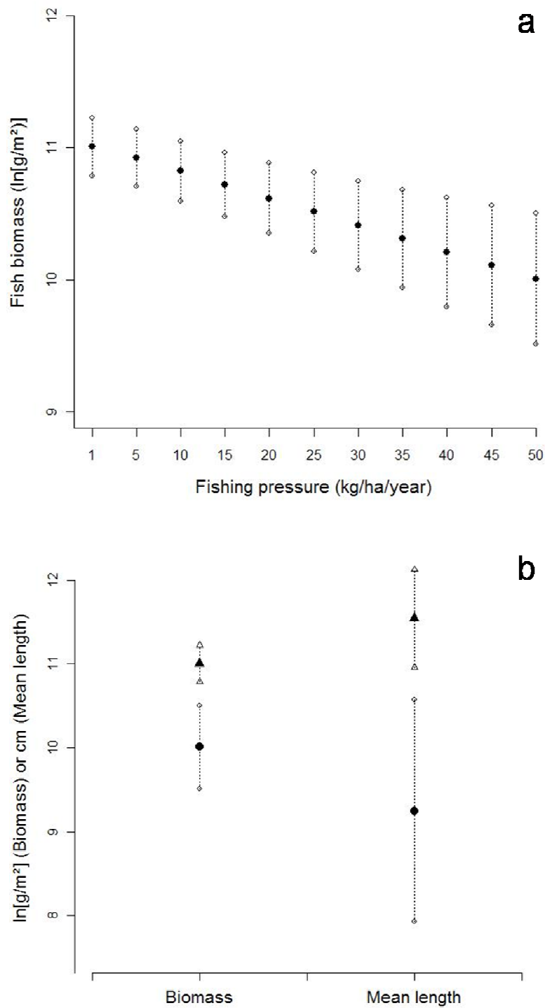
Figure 5: (a) prediction of fish biomass for increasing fishing pressure; (b) prediction of fish biomass and mean length for two levels of fishing pressure (1 kg.ha -1 .year -1 : triangles; 50 kg.ha -1 .year -1 : circles). Both parts of the figure were built using fitted values from the models considering one case study: northern site, year 2002, barrier reefs far from pass, and habitat composed of medium live coral cover (11 to 20%) and a soft substrate cover over 50%. Confidence intervals of the predictions are indicated.
