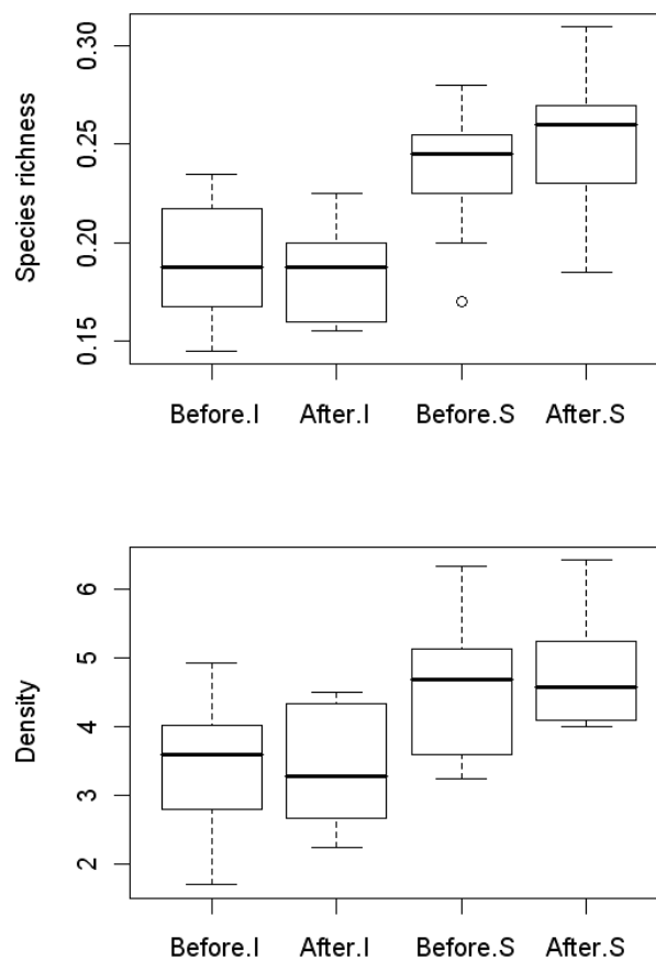
Figure 3: Boxplots of species richness per transect (in number of species per m^2 (top) and abundance density per transect (in number of individuals) per m^2 (bottom) per video transect type and per timing (before/after) with respect to UVC transect. “I” and “S” respectively denote I-type and S-type video transects, i.e. to straight and browsing transects (see § 2.1). For each boxplot, the thick line in the box corresponds to the median value, the lower and upper limits of the box correspond to the 25% and 75% percentiles of the data. The plot whiskers extend out from the box to the most extreme data point which is no more than 1.5 times the interquartile range from the box and all values were plotted.
