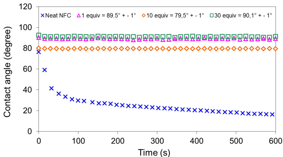
Figure 1-8 : Contact angle vs. time performed with water for (x) Neat NFC, (◇) NFC 10equiv, (△) NFC 1equiv and (□) NFC 30equiv
