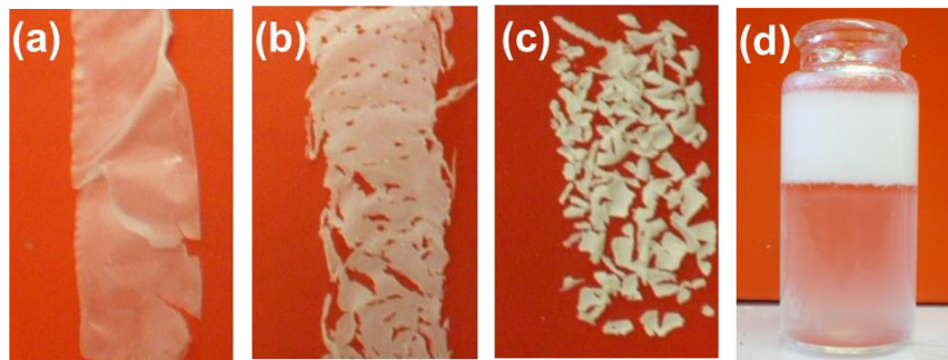
Figure 1-3 : Pictures of films obtained after casting of suspensions of (a) Neat NFC, NFC grafted with (b) 10equiv, (c) 30 equiv and (d) dispersion in water of NFC grafted with 10 equivalent
