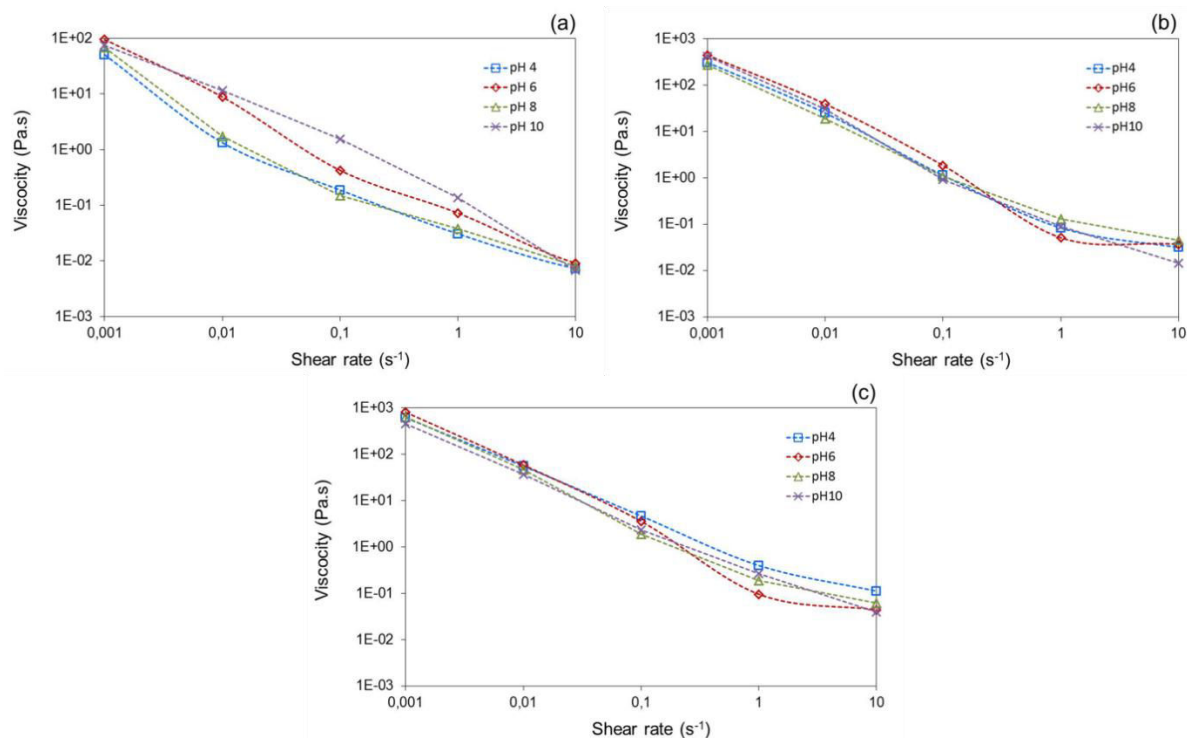
Figure 1-9 : Rheology curves – viscosity function of shear rate for sample of (a) NFC1, (b) NFC2 and (c) NFC3
