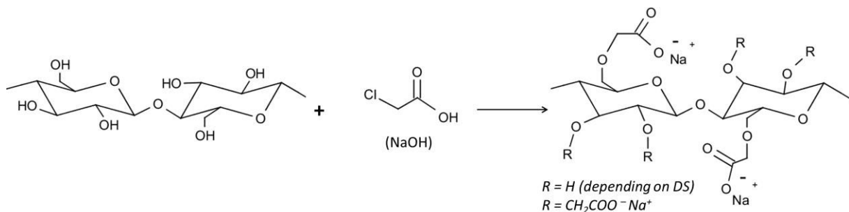
Figure I-17 : Chemical reaction for preparation of carboxymethylcellulose
