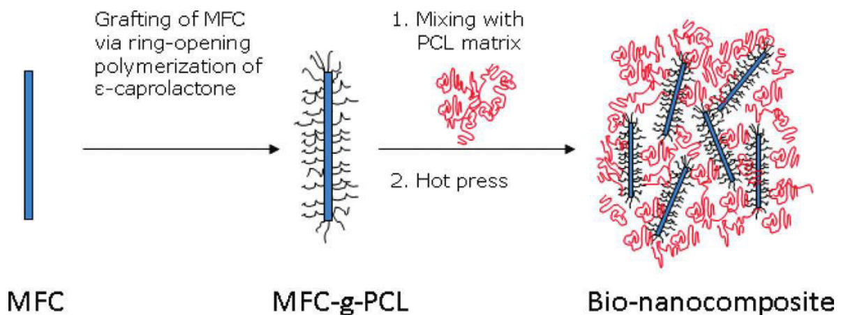
Figure I-37 : Principle to obtain Bio-nanocomposite of PCL reinforced with NFC (Adapted from Lönnberg et al. 2011)
