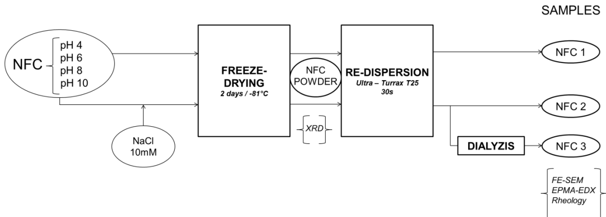
Figure 1-1 : Process for drying NFC using freeze-drying device
