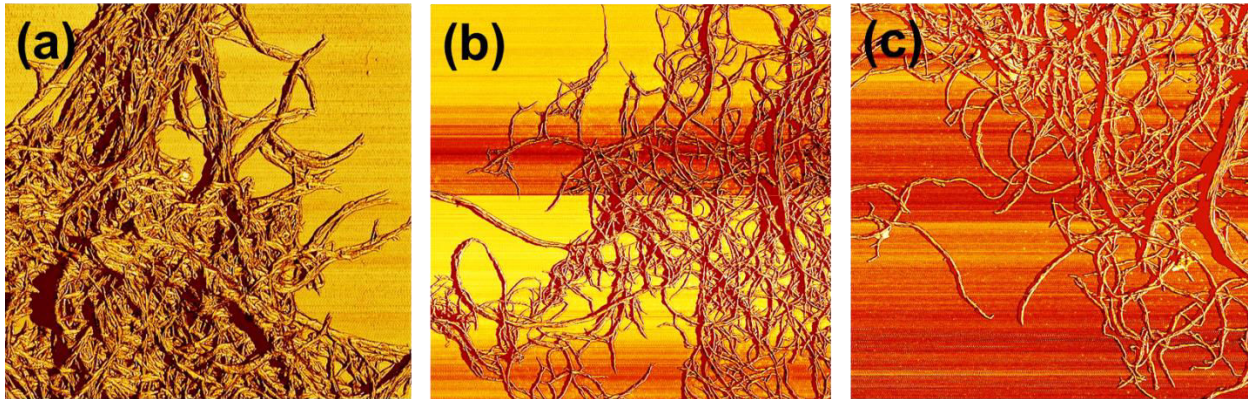
Figure 1-2 : AFM characterizations of grafted NFC with (a) 1equiv, (b) 10equiv and (c) 30equiv
