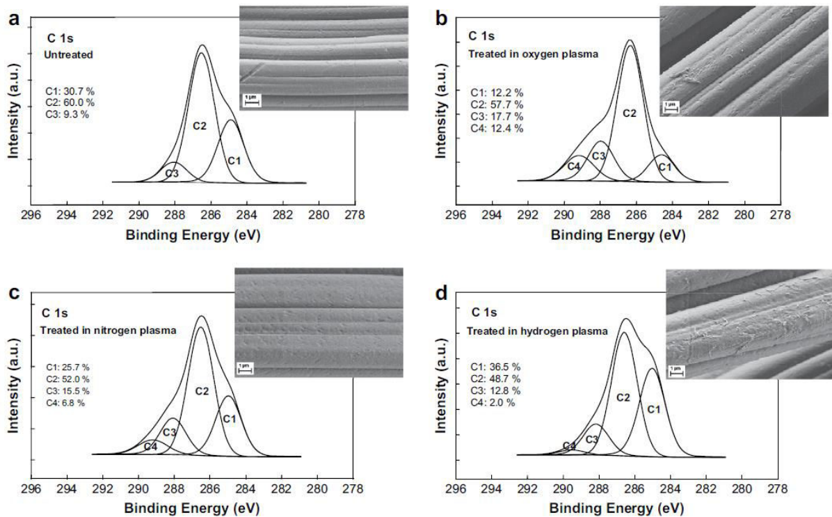
Figure I-21 : SEM images and C1s high-resolution of viscose textile (a) untreated, and after 5s with (b) oxygen plasma, (c) nitrogen plasma and (d) hydrogen plasma (adapted from Vesel et al. 2009)
