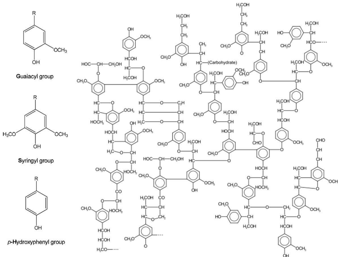
Figure I-9 : Chemical composition of typical lignin according to Adler (taken from Wiki-Lignin web page)
