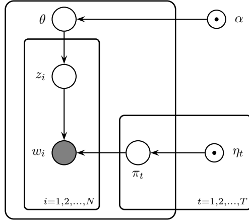
Figure 3.7 – Graphical representation of LDA. The outer plate refers to images. The index i runs over patches, and index t over topics.
