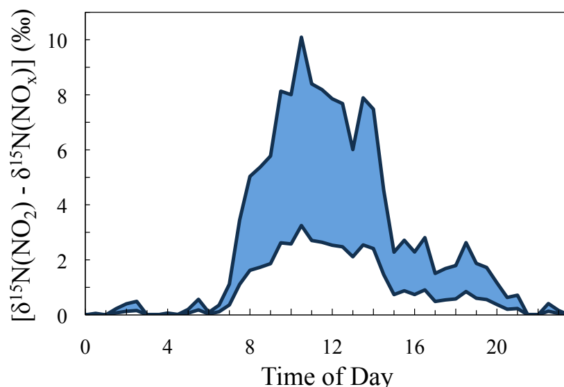
FIGURE 4.13 - The diurnally averaged trend in [\delta^{15}\text{N}(\text{NO}_2) - \delta^{15}\text{N}(\text{NO}_x)] calculated using the \text{O}_3 and \text{NO}_x mixing ratios determined in-situ and Equations 4.11 and 4.12. The shaded surface represents estimates computed over a range of K values (1.022 to 1.046) for the isotopic exchange between \text{NO} and \text{NO}_2 .
