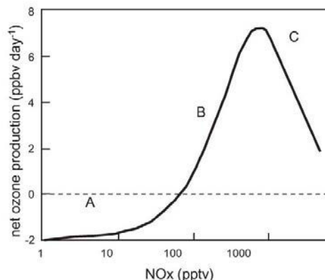
FIGURE 1.13 - Schematic representation of the dependence of the net ozone production (or destruction) on the concentration of NO x . The magnitudes reflect clean free tropospheric condition (Monks, 2005).
