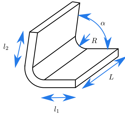
FIGURE 3.15 – Cornière composite
