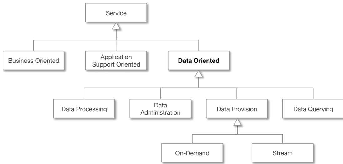
Figure 2.1 Service classification (UML class diagram)
