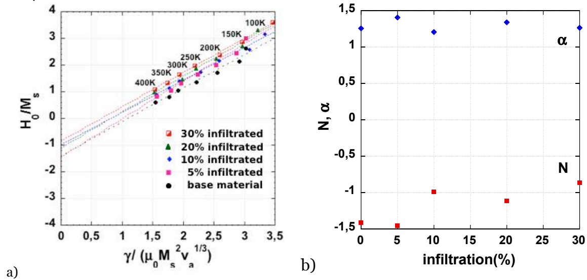
Fig. 4. 14 ( H_0/M_s ) versus \gamma / (\mu_0 M_s^2 v_a^{1/3}) for TMC bulk samples (a) dots - experimental points; discontinuous lines: linear fit; N and \alpha as a function of the infiltration degree (b).
