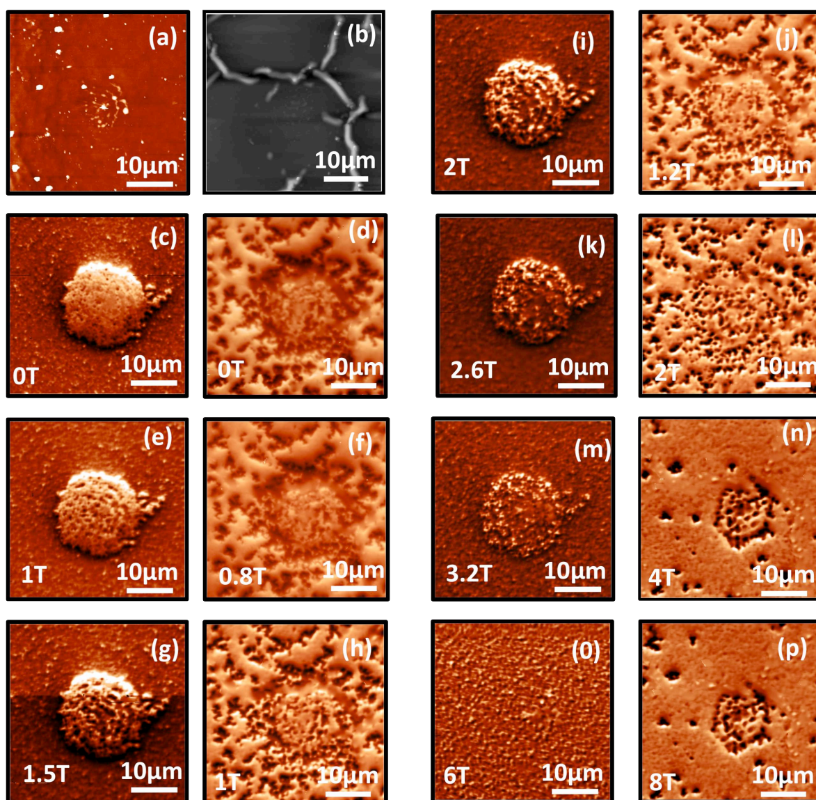
Fig. 5. 19 MFM magnetization reversal for a high H_c NdFeB film with elongated grains, S_{2,6} (column 1 and 3) and a medium coercivity NdFeB film with columnar grains, S_{1,2} (column 2 and 4). The ripples in (b) are due to the squeeze out of a Nd-rich phase during the post deposition annealing step.
