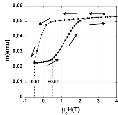
Fig. 5. 20 Minor loop measured for a non-patterned columnar film
