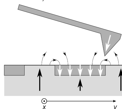
Fig. 5. 7 Schematic of the real tip-sample geometry during scanning.
