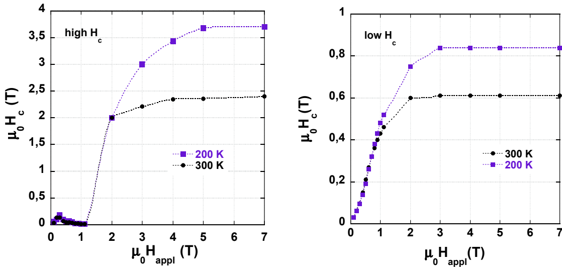
Fig. 4. H_c(H_{app}) for high H_c thick film at 300 K and 200 K (a) and low H_c thick film at the same two temperatures (b).
