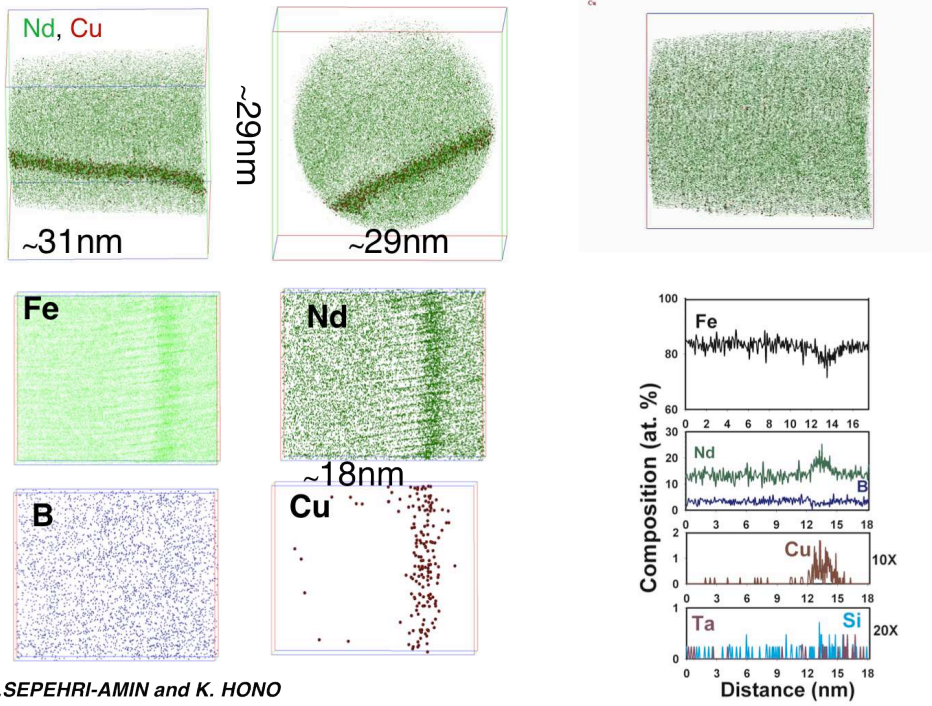
Fig. A7. 6 Atome probe maps and elemental analysis of the high H_c film, S_{2.55} , grain boundary.
