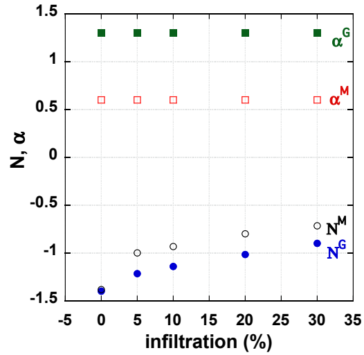
Fig. 4. 15 Values of N and \alpha obtained for TMC bulk samples using the global model ( N^G and \alpha^G ) and micro-magnetic model ( N^M and \alpha^M ) when the value of \alpha is fixed (0.6 for MM and 1.3 for GM). N is taken negative here to make the graph easier to read.
