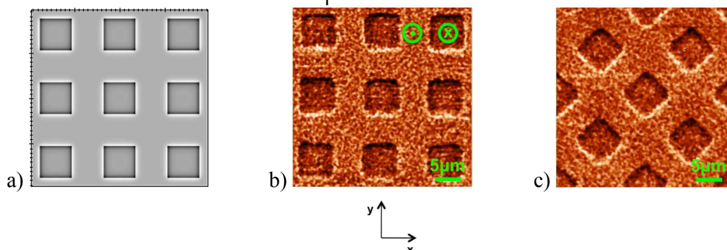
Fig. 5. 5 Calculated 2D stray field map (a) compared to experimental phase shift map (b) and experimental map after a 45 deg rotation of the sample (c).
