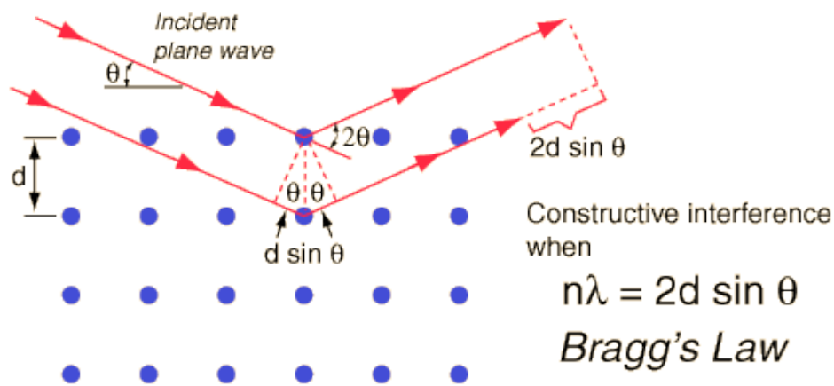
Fig. 3.4 Schematic showing the geometry of X-ray diffraction technique 4 ;
