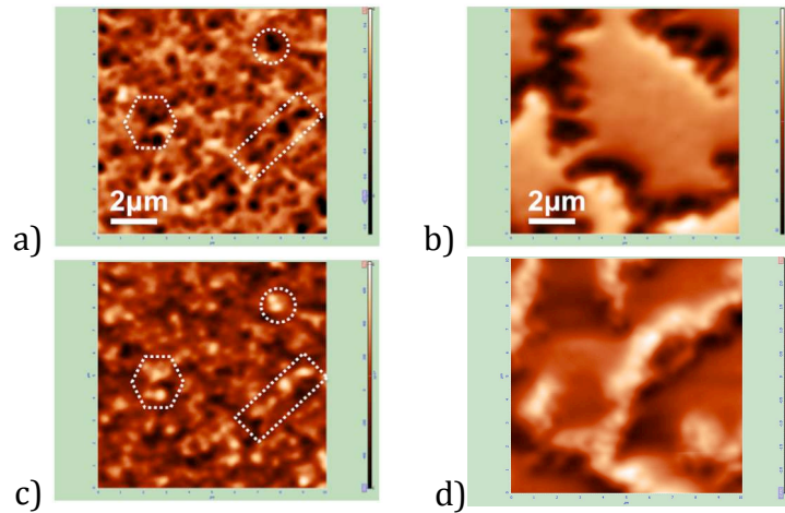
Fig. 5. 17 Comparison of magnetic states after applying +8T and -8T for high coercivity NdFeB film (a and c) and lower coercivity NdFeB film (b and d).
