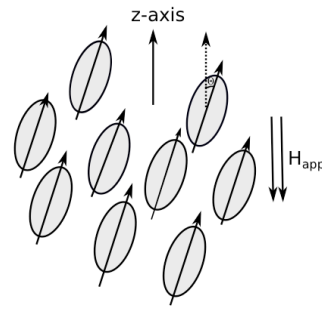
Fig. A3. 2 Scheme that shows how the angle between the average easy axis and the z-axis can be changed as the angle between the applied field and magnetization can be changed.
