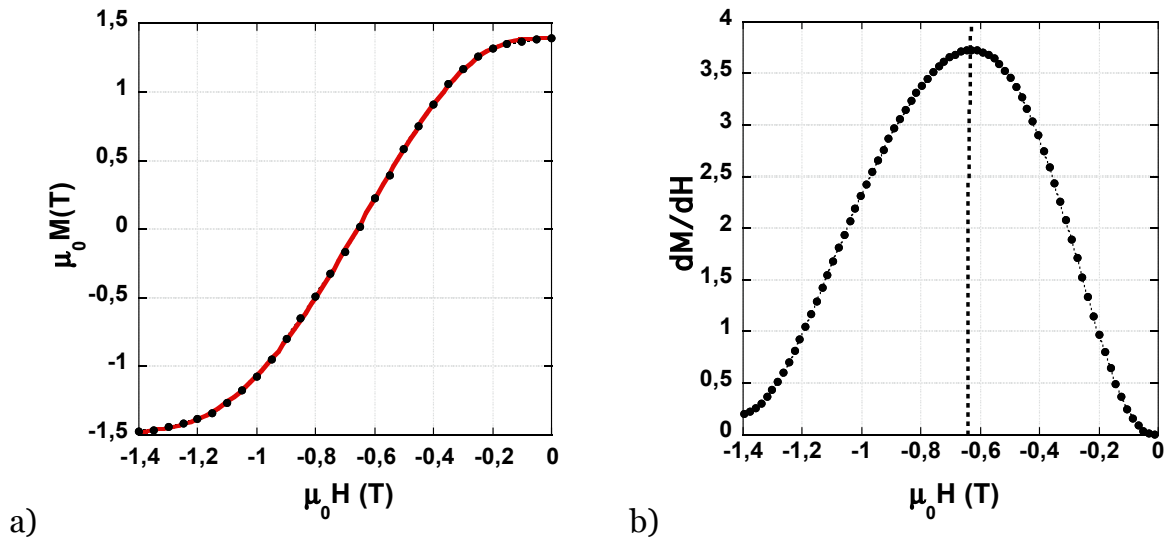
Fig. 4. 2 M(H) in the vicinity of the coercive field measured on the base material at 400 K (a) and the corresponding susceptibility function of the applied field plot (b). The black dots in (a) correspond to experimental points; the red (continuous) line is the polynomial fit and the dotted vertical line in (b) corresponds to H_c .
