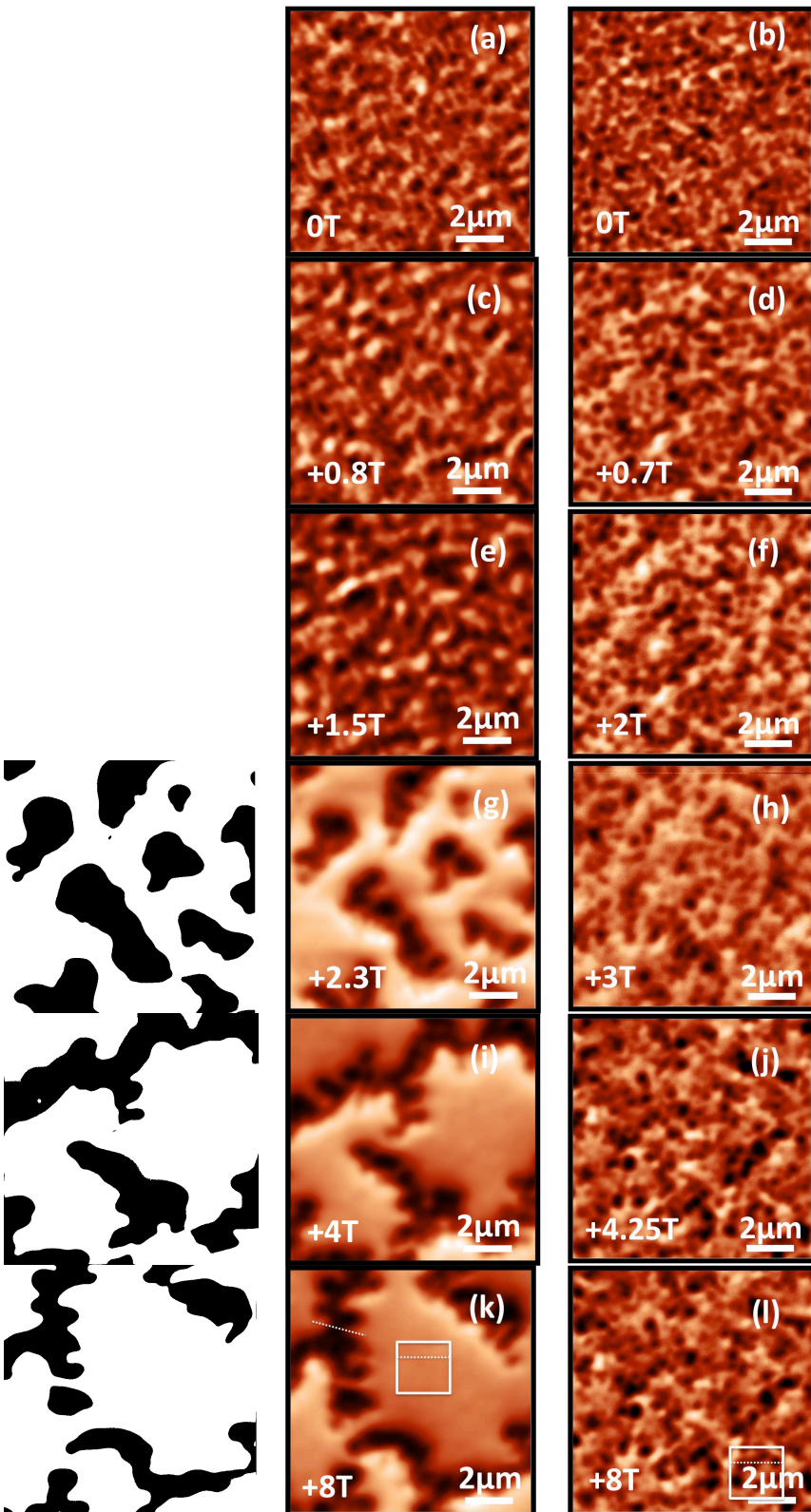
Fig.5.12bis Binarization of the last three MFM images corresponding to S_{0.7} .
