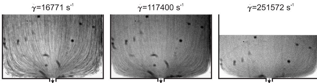
Figure 5.8.: Picture series of PBS 15/85-Hct50 immediately upstream of the contraction for different flow rates. The corresponding shear rates are given above each picture. For this polymer-free solution with RBCs no instabilities are observed.
