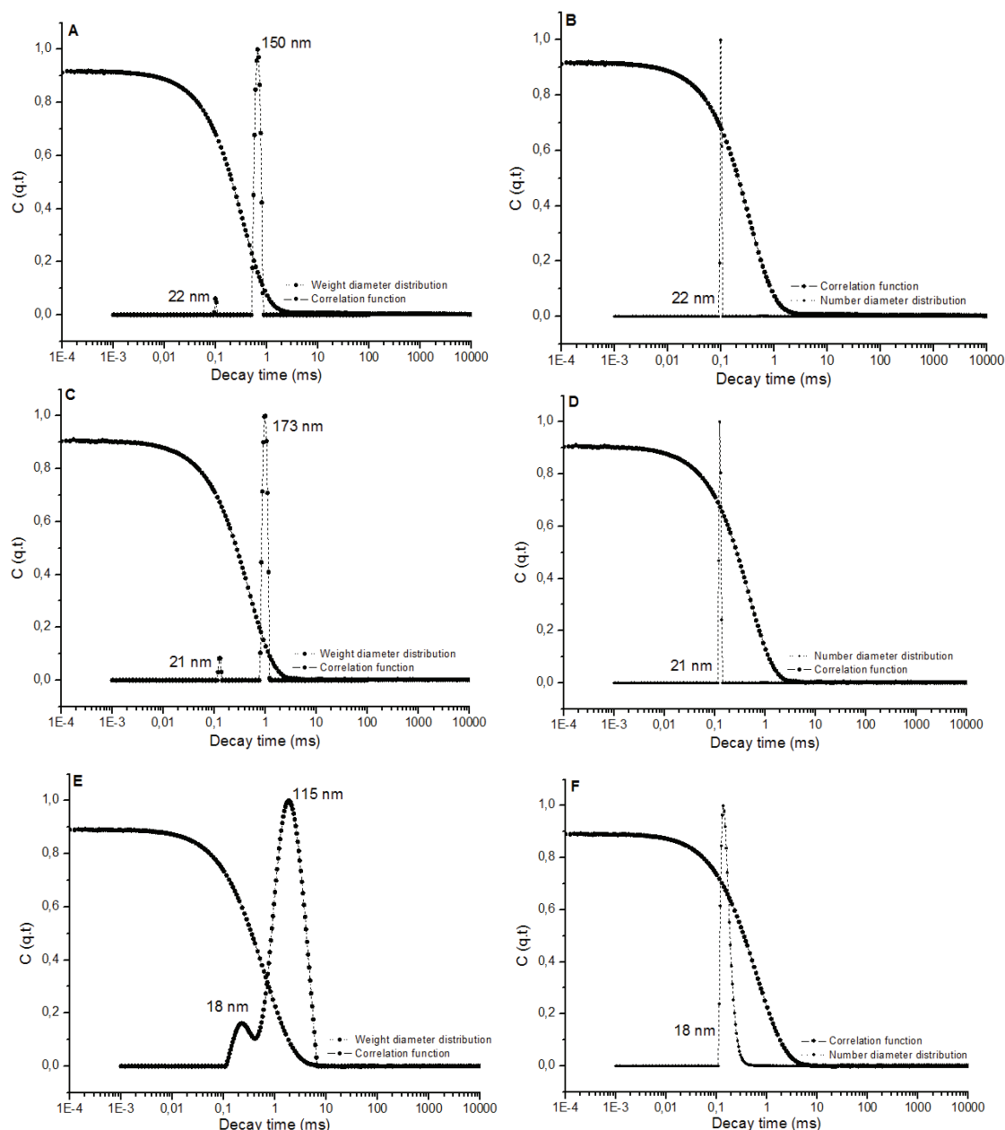
Figure 6. Dynamic light scattering autocorrelation function and diameter distribution of XGO- b -XGO,Ac ( 5 ) in water by DLS ( A,B : 1.0 mg mL -1 ; C,D : 3.0 mg mL -1 ; E,F : 5.0 mg mL -1 , scattering angle = 90°, temperature = 25 °C).
