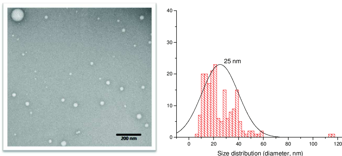
Figure 7. Transmission electron micrograph with size distribution of XGO- b -XGO,Ac ( 5 ) micelles ( 3 \text{ mg mL}^{-1} ).
