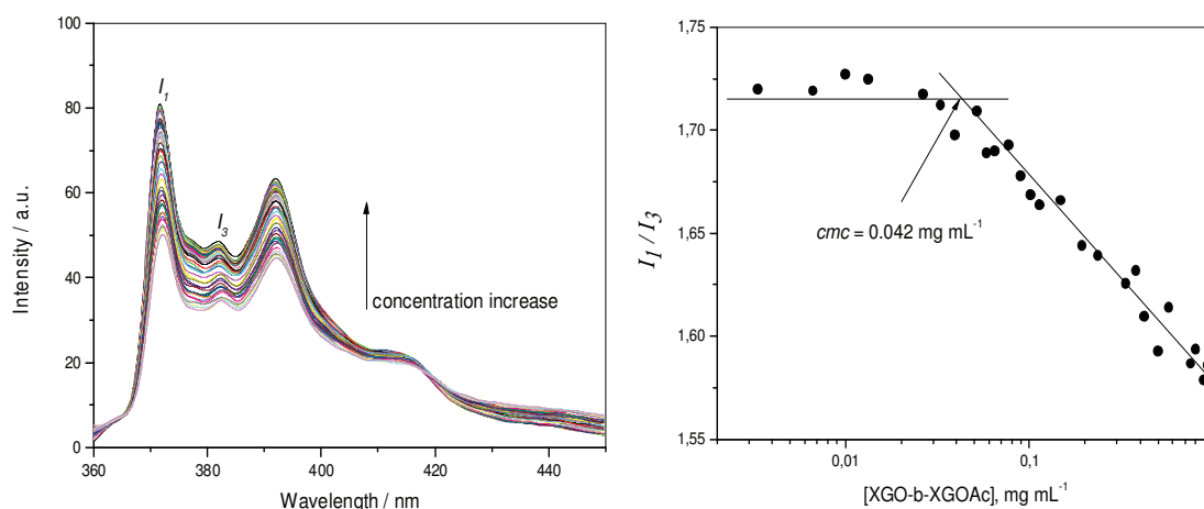
Figure 2. Pyrene fluorescence emission spectra and the corresponding variation in the I_1/I_3 ratio as a function of XGO- b -XGO,Ac concentration ( [\text{pyrene}] = 6 \cdot 10^{-7} \text{ mol L}^{-1} ).
