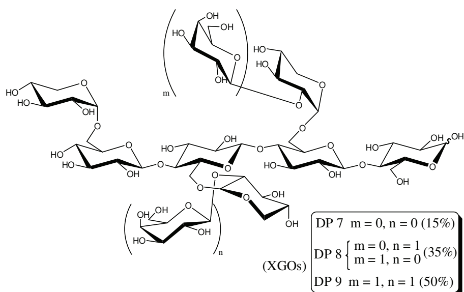
Figure 1. General structure of xyloglucan oligosaccharides.
