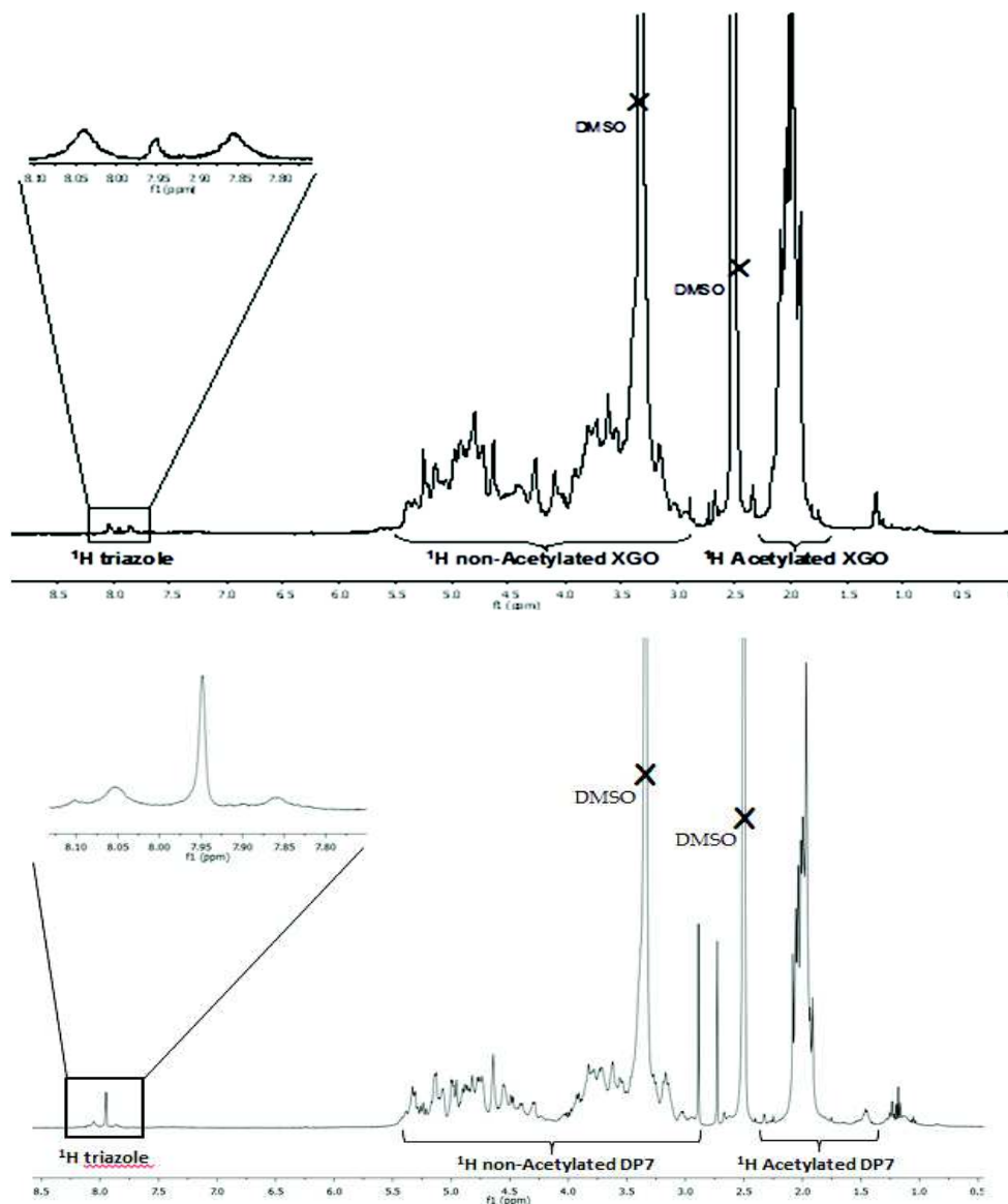
Figure 4. 1 H RMN spectra of XGO- b -XGO,Ac and DP7- b -DP7,Ac.
