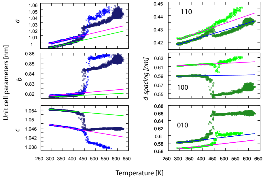
Figure III.7. Variation of the converted unit cell parameters ( a' , b' , c' ) and d -spacing ( d_{110} , d_{100} , d_{010} ) of Ia\alpha as a function of temperature by using Gr53a6FF (deep blue and deep green) and Gr56A carbo FF (blue and green). The fitted lines were used to calculate the TEC.
