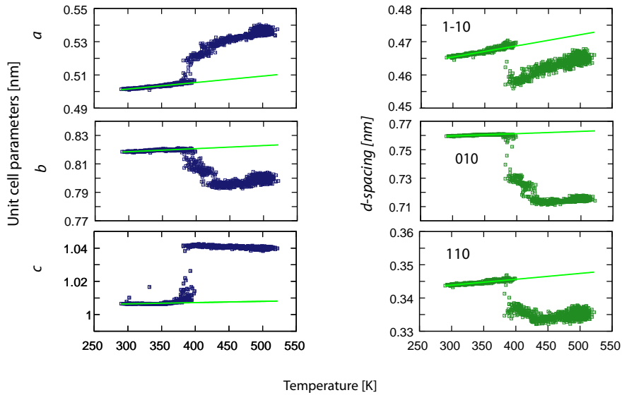
Figure III.9. Variation of unit cell parameters ( a , b , c ) and d -spacings ( d_{1-10} , d_{010} , d_{110} ) of III 1 as a function of temperature by using \text{Gr56A}_{\text{carbo}} FF (blue and green). The fitted lines were used to calculate the TEC.
