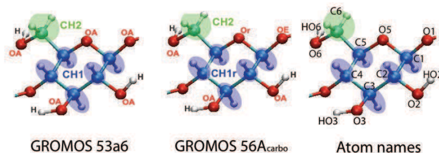
Figure III.1. The definition of the atom types and names in a glucosyl residue in Gr53a6FF and Gr56A carbo FF.
