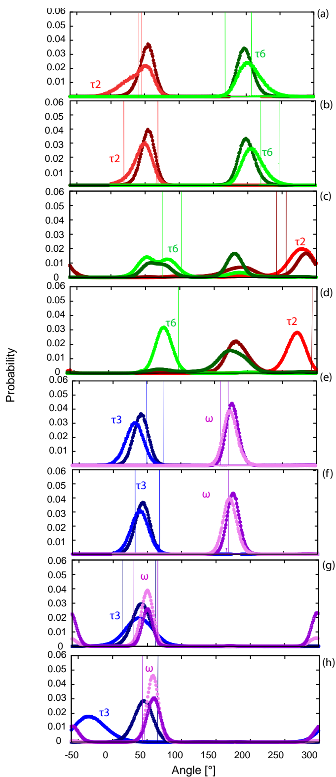
Figure III.3. Calculated dihedral angles of three hydroxyl groups ( \tau_2 , \tau_3 and \tau_6 ) and one hydroxymethyl group ( \omega ) of cellulose I _{\beta} (a,e), I _{\alpha} (b,f), II (c,g) and III _{I} (d,h) by using Gr53a6FF (deep colors: dark red, dark blue, dark green and dark violet) and Gr56A carbo FF (bright colors: red, blue, green, violet). The straight lines indicate the experimental values. The two lines with same color represent conformational differences either from the center chain and the origin chain, or from the two neighbor residues in one chain.
