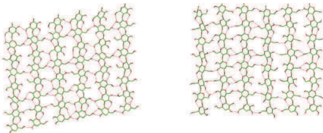
Figure V.3.4. Two types of hydrogen bonding patterns of I_\alpha and I_\beta during MD simulations by using four GROMOS force fields. Hydrogen bonds are indicated in red dotted lines. The left pattern is a snapshot from the high temperature structure of I_\alpha by using native Gr53a6FF, while the right pattern is from I_\beta by using the same force field
