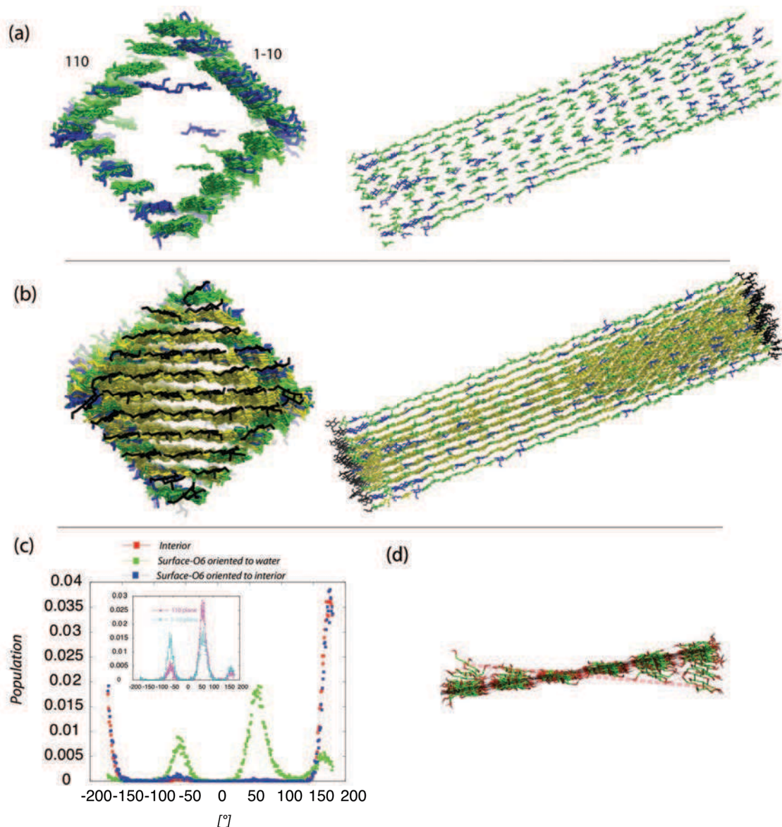
Figure V.4.10. Snapshots of finite models of I\beta at 100 ns by using revised Gr56A_{carbo}FF (a and b, yellow: tg , blue: gg , green: gt , terminal groups: black) and the populations of the conformation of \omega in different regions of fiber (c).
