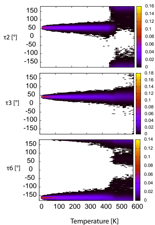
Figure III.15. Histogram of the \tau_2 , \tau_3 and \tau_6 angles as a function of temperature during heating by using Gr53a6FF.
