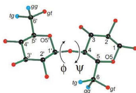
Figure I.2. Definition of the glucosidic linkage angles and the three staggered conformations of the hydroxymethyl group of cellulose (French and Johnson 2006)
