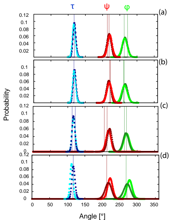
Figure III.2. Estimated glycosidic linkage angles ( \phi : green, \psi : red, \tau : blue and cyan) of cellulose I \beta (a), I \alpha (b), II (c) and III _1 (d) by using Gr53a6FF (dark blue, dark red, forest green) and Gr56A carbo FF (cyan, red, green). The vertical lines indicate the experimental values. The two lines with the same color represent conformational difference either from the center chain and the origin chain or from the two neighbor residues in one chain.
