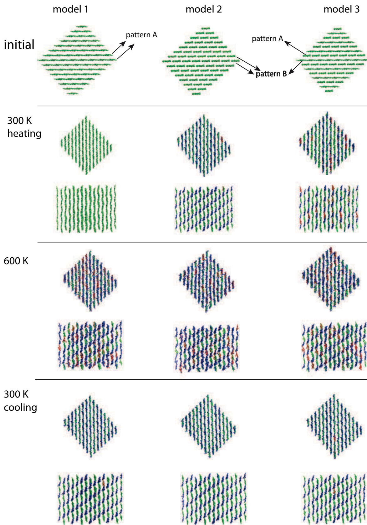
Figure V.2.3. Snapshots of the three models of cellulose I α at different temperatures. The conformations of hydroxymethyl groups are colored in green ( tg ), blue ( gt ) and red ( gg ).
