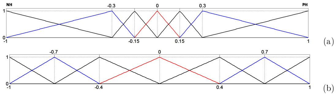
Figure 3.30: Type-1 fuzzy membership functions ( U=0\% ) to represent e (a) and de (b)
