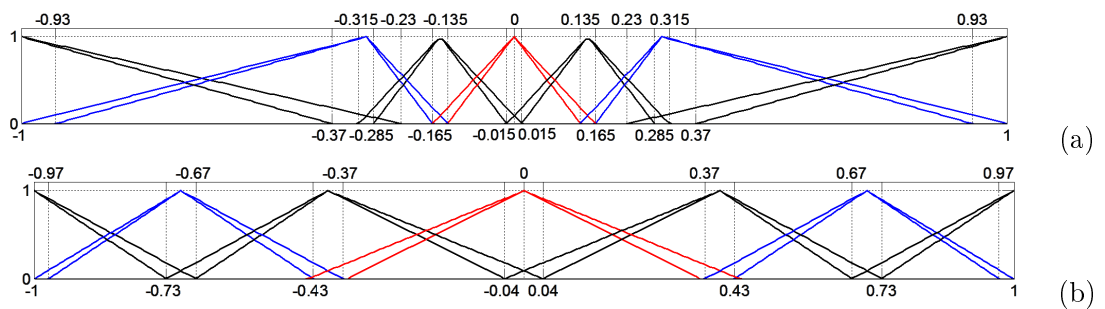
Figure 3.31: Type-2 fuzzy membership functions ( U=20\% ) to represent e (a) and de (b)
