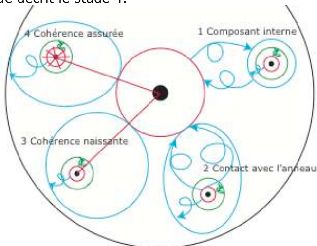
Figure 6.16 Cohérence progressive
