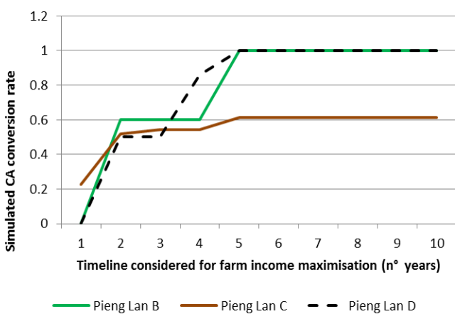
Fig. 2c. Simulated CA conversion rate for diverse timelines of farm income maximisation (Pieng Lan village of Chieng Hac commune)
