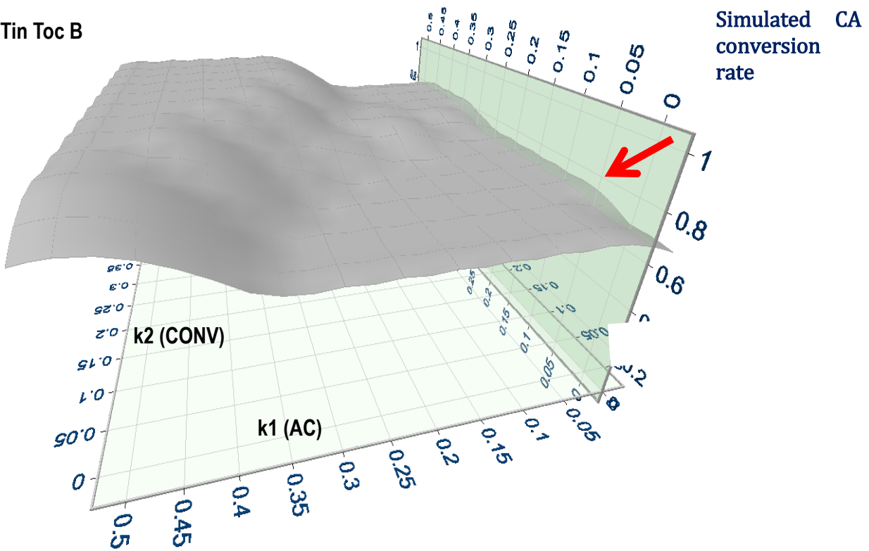
Figure 5a (top) and 5b (bottom). Simulated CA conversion rate upon a 5 year profit maximisation for farms Tin Toc B (top) and Ta So C (bottom) considering different values of k1 and k2, respectively representing the amplitude of cumulated impact over time of CA and conventional agriculture on crop yields (Alternative scenario).
