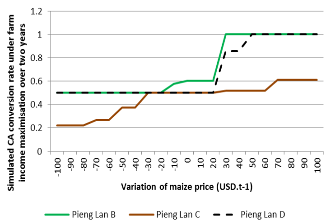
Fig. 3c. Sensitivity analysis to maize price of simulated CA conversion rate under maximisation of farm income over 2 years (Pieng Lan village)
