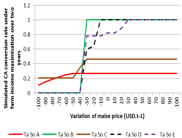
Fig. 3a. Sensitivity analysis to maize price of simulated CA conversion rate under maximisation of farm income over 2 years (Ta So village)
