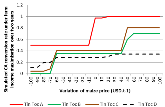
Fig. 3b. Sensitivity analysis to maize price of simulated CA conversion rate under maximisation of farm income over 2 years (Tin Toc village)
