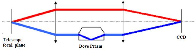
Figure 2. The optical device of the PBL instrument.
