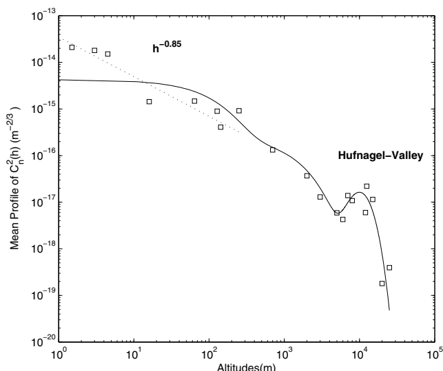
Fig. 13. Reconstructed C_n^2(h) mean profile at Paranal for the December 2007 campaign using the simultaneous measurements of the energy at different altitudes and different height sampling plotted in squares. We show the Hufnagel-Valley model in solid line and the adjustment of the first meters layer to a power law of height h^{-0.85} in dotted lines.
