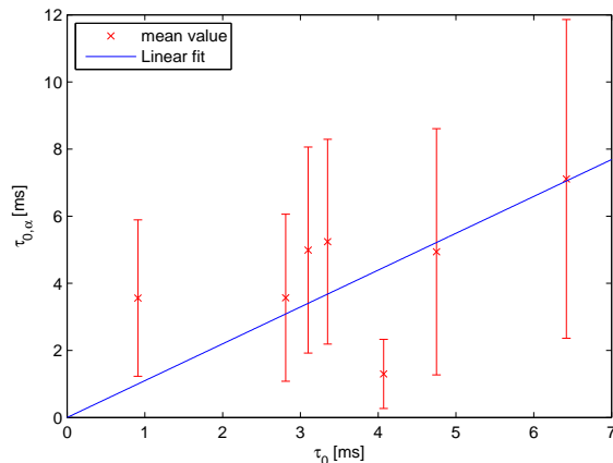
Figure 5. Comparison of the coherence time measured with the GSM \tau_{0,\alpha} and \tau_0 deduced from in-situ balloon data using equation 6 in the case of a whole atmosphere integrated wind speed as indicated in equation 7. The error bars indicate the standard-deviation of GSM data during the ascent time.
