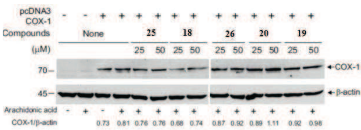
Figure 4. Effect of type (I) and type (II) compounds on COX-1.
