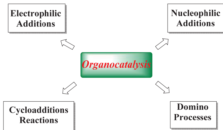
Figure 3. Use of organocatalysis in a wide range of asymmetric synthesis.
