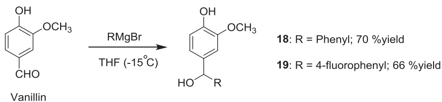
Scheme 11. Preparation of phenol 18 and its fluorinated analogue 19 .
