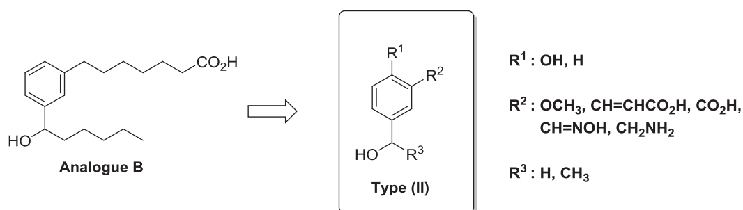
Scheme 16. General structure of type (II) compound.
