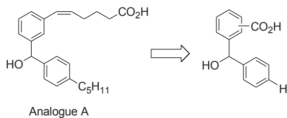
Scheme 6. General structure of acids 10 and 15 .
