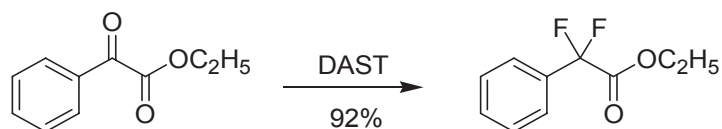
Scheme 4. Fluorination of \alpha -ketoesters using DAST.
