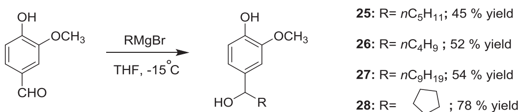
Scheme 17. Preparation of first series of type (II) compounds.
