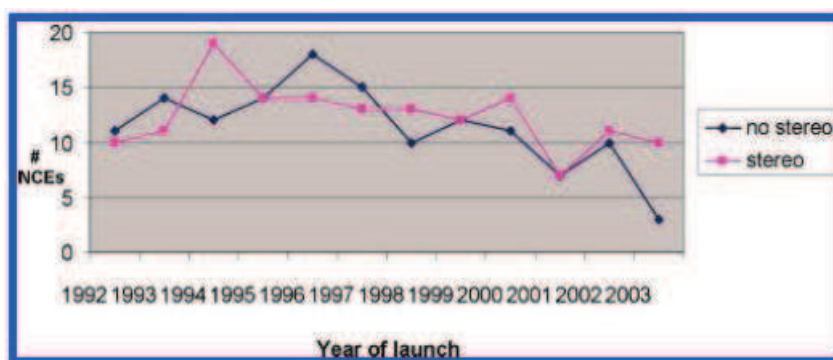
Figure 1. Marketed drugs with, or without, stereochemistry 1
