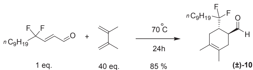
Scheme 15. Non-catalyzed Diels-Alder cycloaddition.
