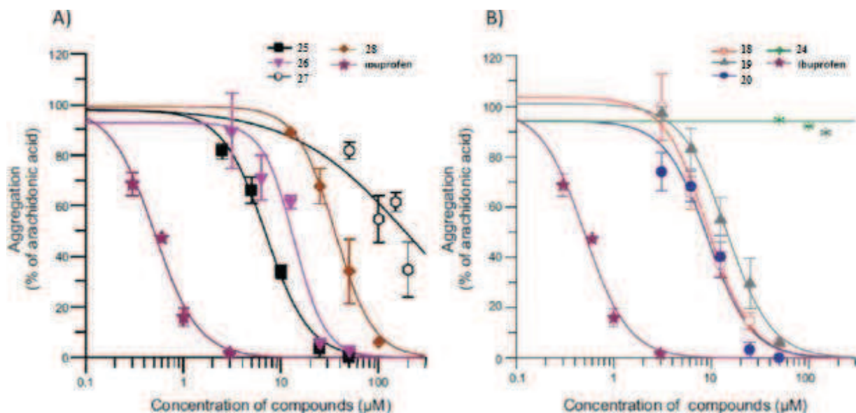
Figure 2. Comparison between biological activity of Type (I)/Type (II) compounds and Ibuprofen.
