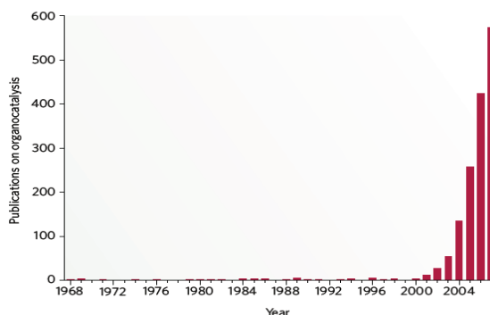
Figure 4. Quantitative evolution of organocatalysis. 7
