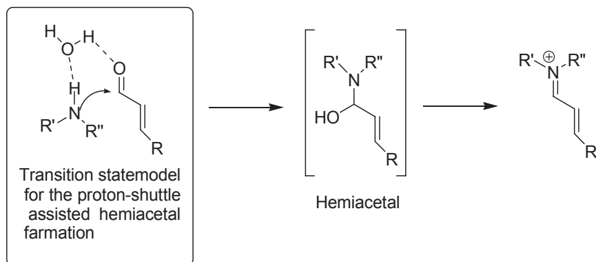
Scheme 19. Effect of water in first and final step of catalytic cycle. 14
