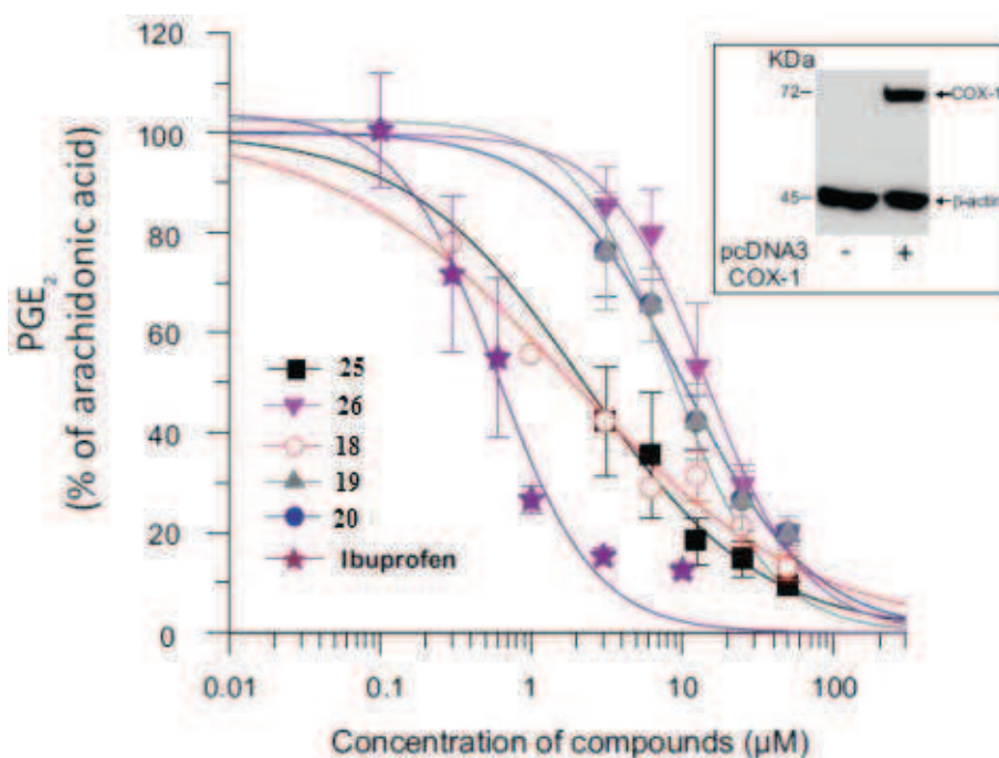
Figure 3. Effect of the synthesized molecules on COX-1.
