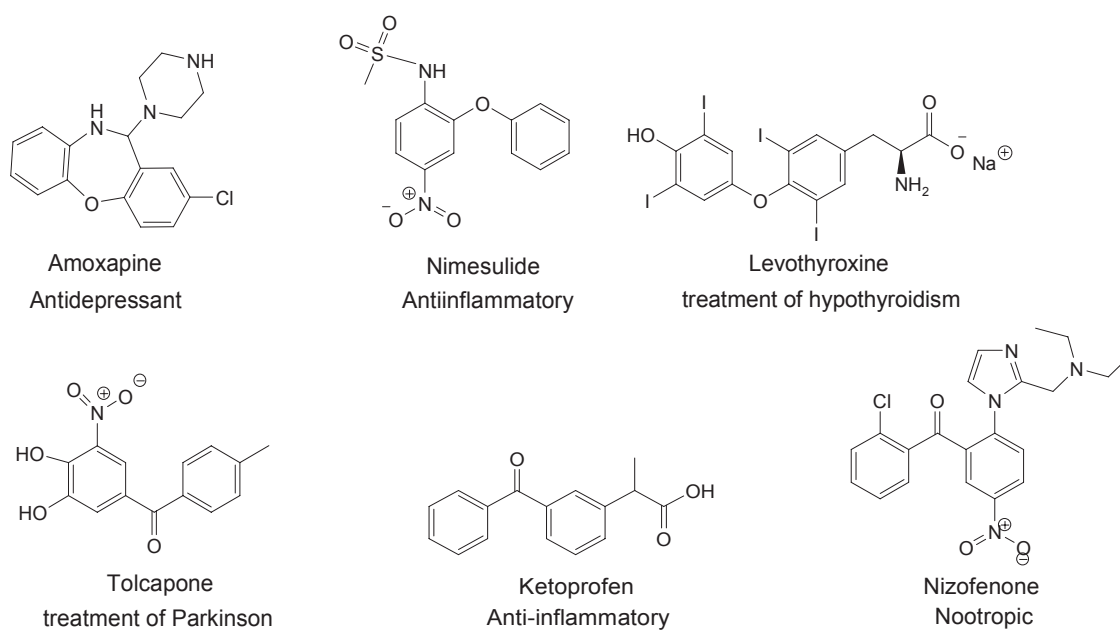
Fig. 1 Selected examples of diaryl ethers and diaryl ketones and their medical applications.
