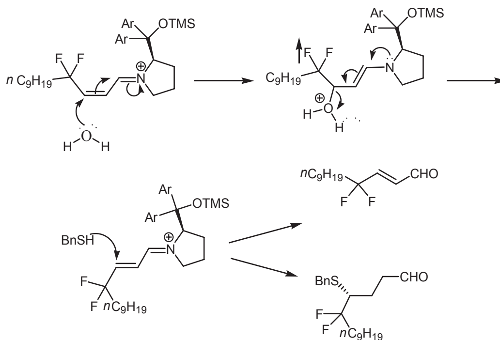
Scheme 23. E/Z isomerisation of aldehyde under the effect of catalyst.
