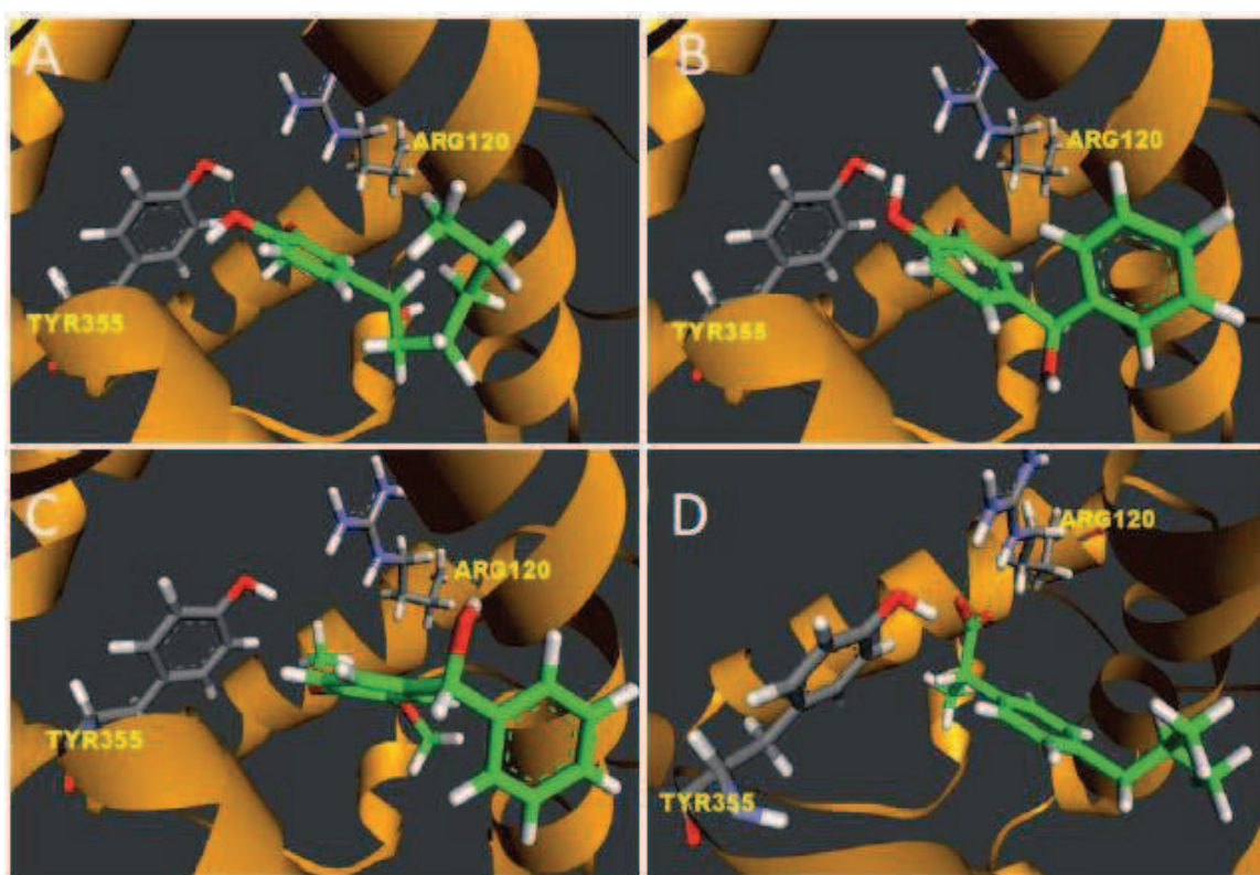
Figure 7. Modeling analysis of the synthesized molecules.
