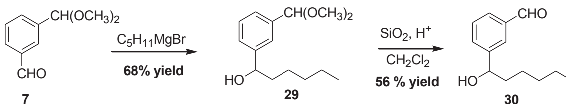
Scheme 18. Synthesis of aldehyde intermediate 30 .
