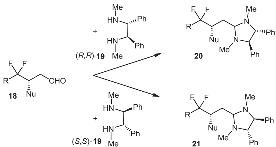
Scheme 24. NMR method used to measure the ee's on the 1,4 adducts.
