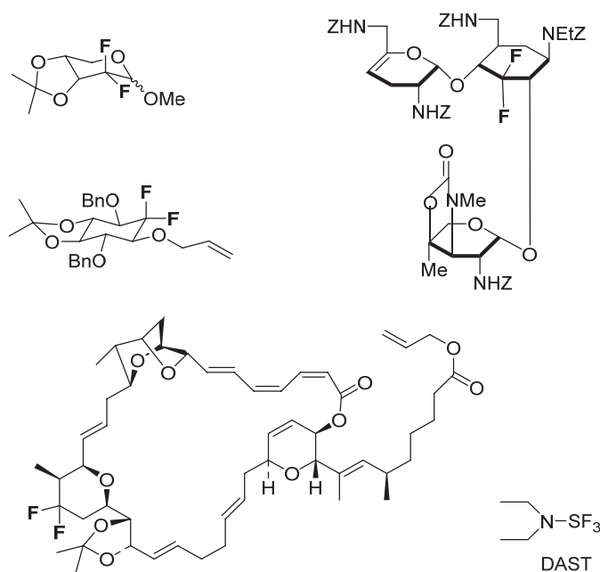
Scheme 3. Representative gem -difluoro compounds prepared by DAST fluorination. 21
