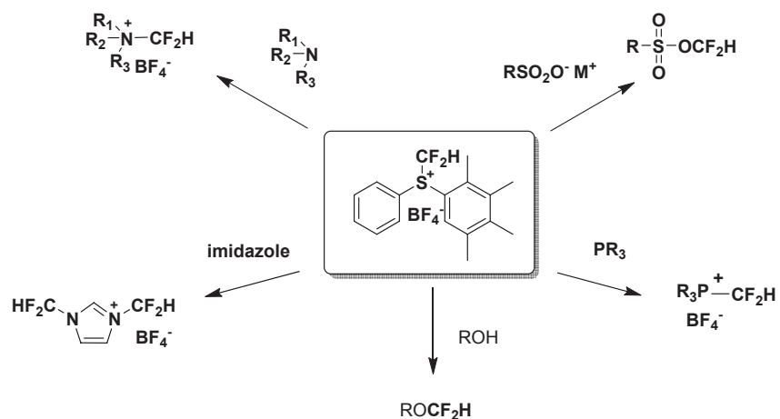
Scheme 22. New reagents for introduction CF 2 H group
