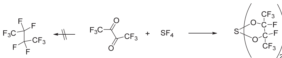
Scheme 2. Unexpected reaction of sulfur tetrafluoride with \alpha -dicarbonyl compounds.
