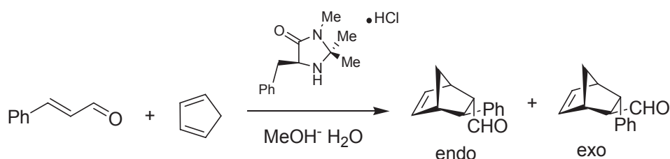
Scheme 10. Asymmetric organocatalytic Diels-Alder cycloaddition.
