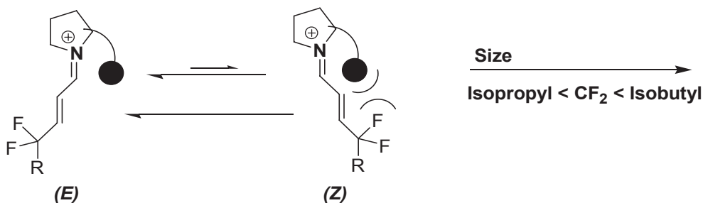
Scheme 27. Effect of fluorine atoms on ( Z )/( E ) equilibrium.
