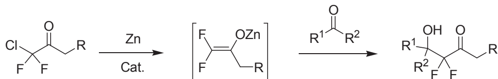
Scheme 12. Reformatsky reaction of chlorodifluoro compounds.
