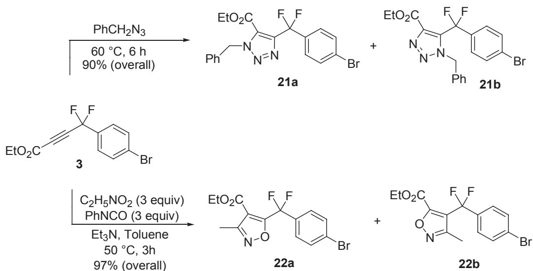
Scheme 18. Synthesis of mixed gem -difluoro aromatic-heteroaromatic derivatives 21 and 22 .
