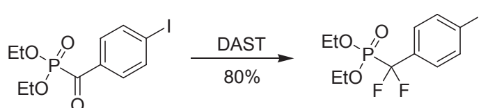
Scheme 5. Extension of DAST fluorination toward ketophosphonates.
