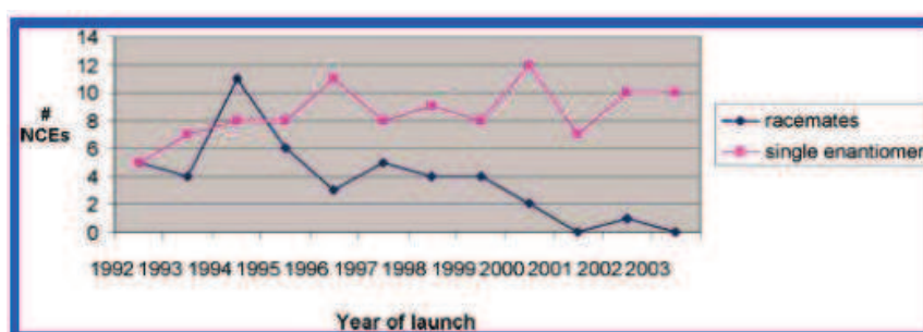
Figure 2. Single enantiomers versus racemates 1
