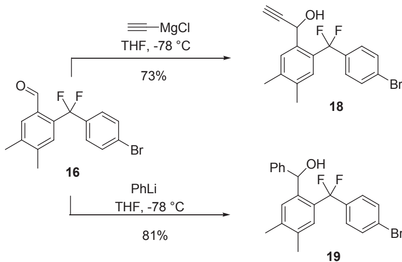
Scheme 16. Addition of an organolithium and an organomagnesium reagent.
