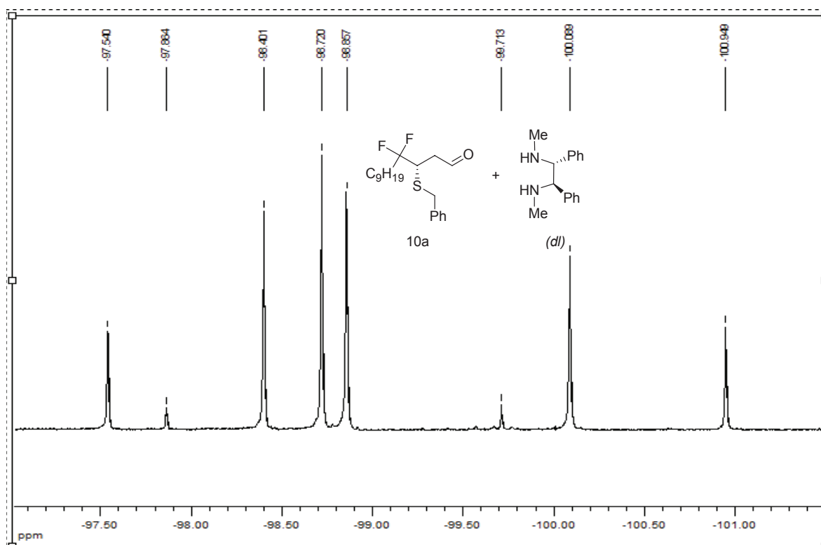
Fig 5. Representative example for determination of ee using ^{19}\text{F} NMR.
