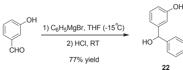
Scheme 14. Preparation of phenol 22 .
