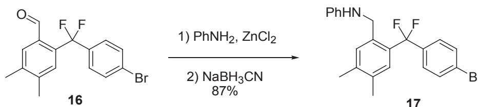
Scheme 15. Reductive amination of aldehyde 16 .
