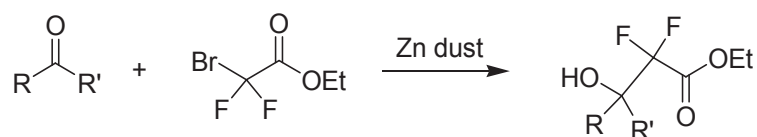
Scheme 11. Reformatsky reaction using bromodifluoro compounds.
