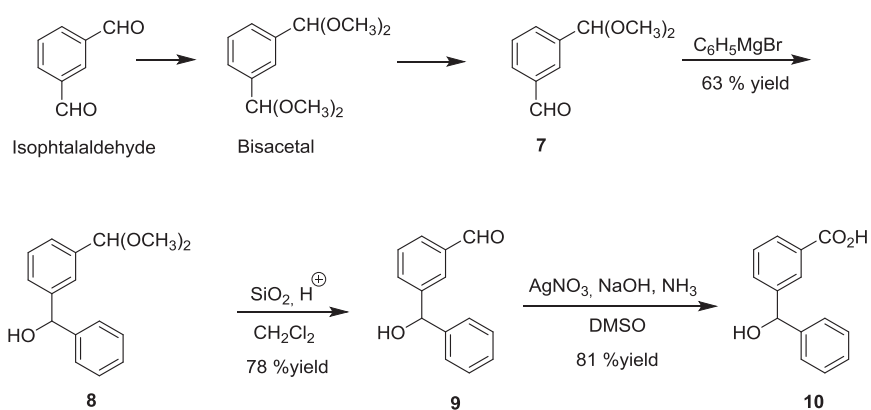
Scheme 7. Synthesis of meta -carboxylic acid 10 .
