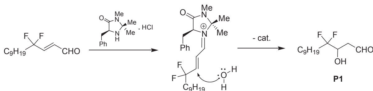
Scheme 17. Addition of water to the reactive iminium salt and proposed structure for P1 .
