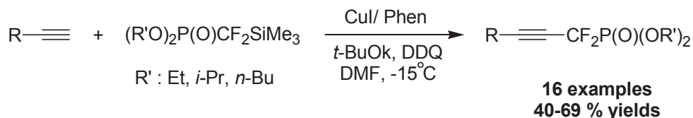
Scheme 19. Copper-mediated oxidative cross-coupling reactions.
