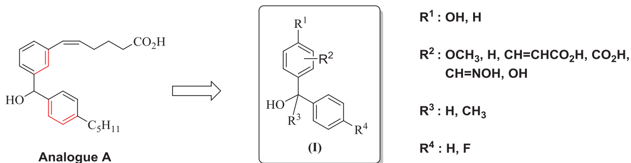
Scheme 2. General structure of type (I) molecules
