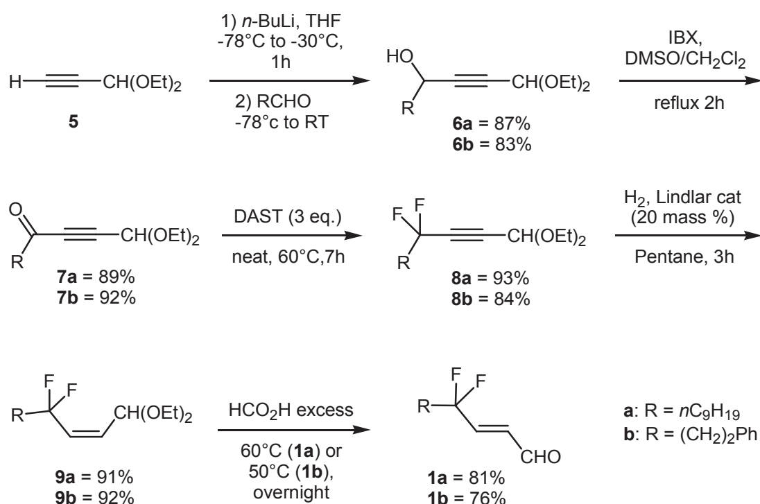
Scheme 14. Synthesis of gem -difluoro enals 1a and 1b .
