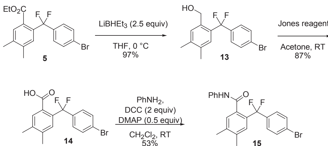
Scheme 13. Reduction of ester followed by oxidation to acid and synthesis of amide.
