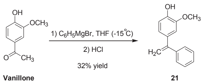
Scheme 13. Preparation of compound 21 .
