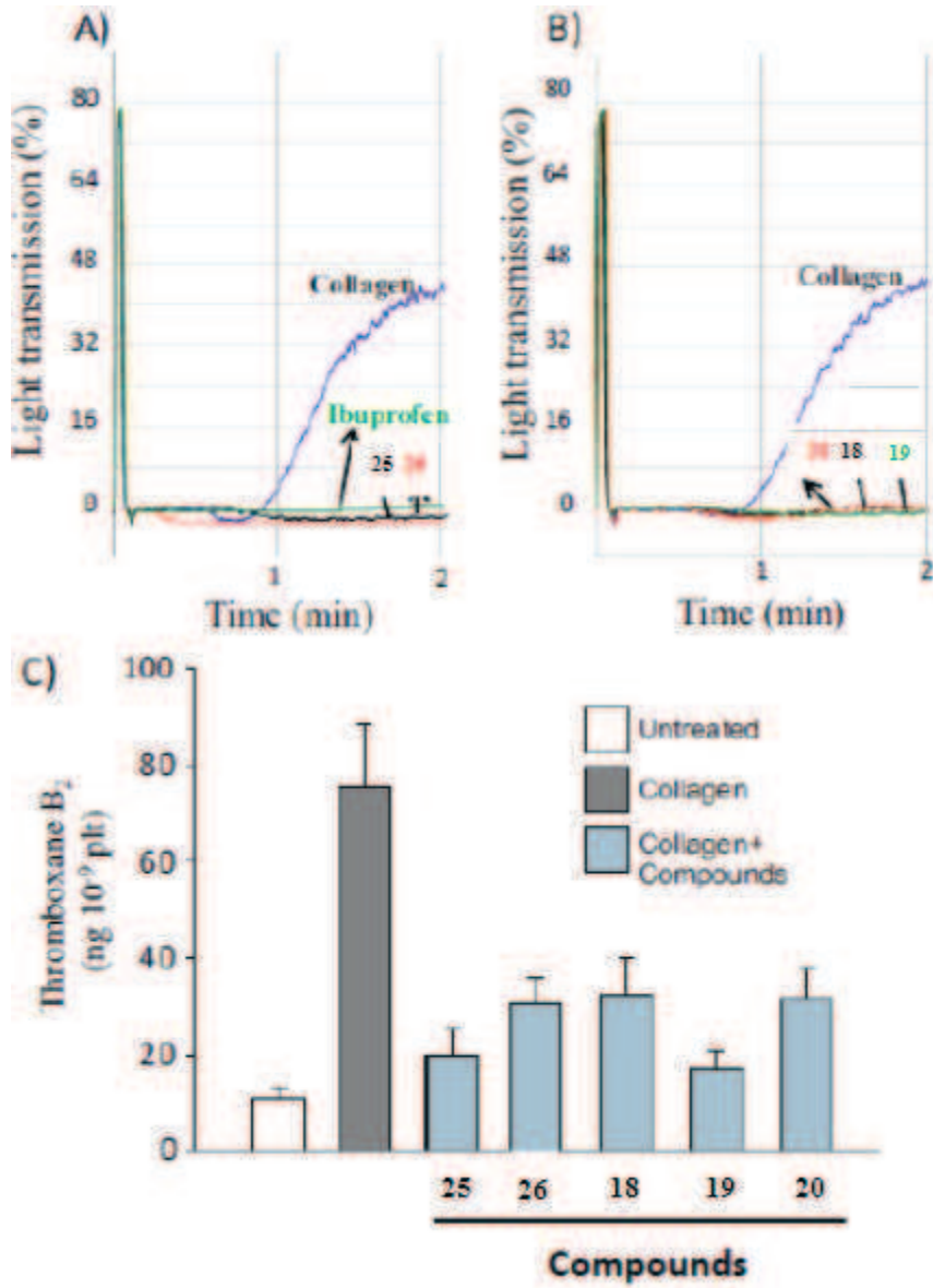
Figure 5. Effect on collagen- and thromboxane.
