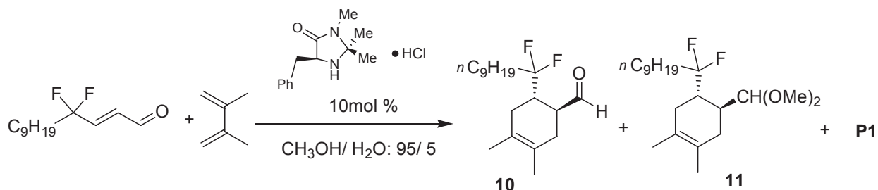
Scheme 16. Catalyzed Diels-Alder cycloaddition in methanol/water solvent
