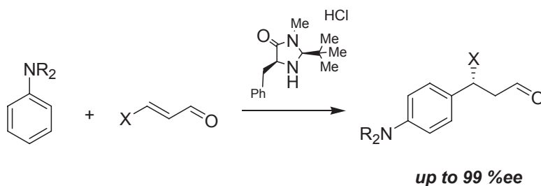
Scheme 12. Organocatalytic conjugated addition of aniline.
