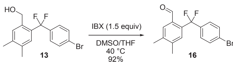
Scheme 14. Oxidation of alcohol 13 to aldehyde 16 .
