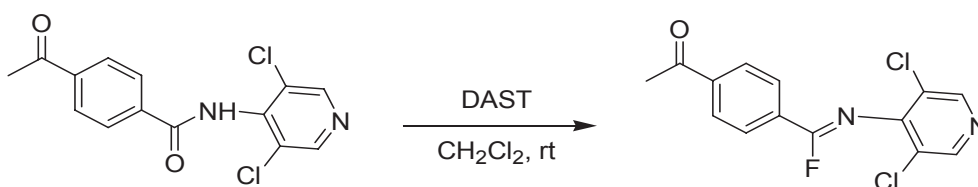
Scheme 7. DAST fluorination side product.
