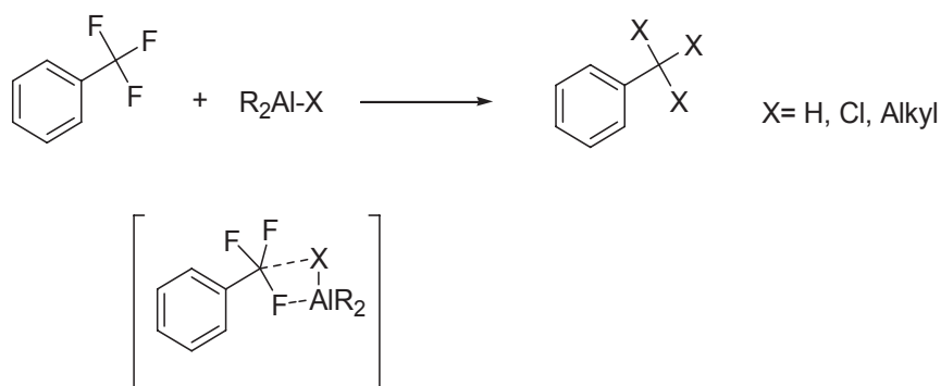
Scheme 11. Cleavage of benzylic C-F bonds using organoaluminium reagents.
