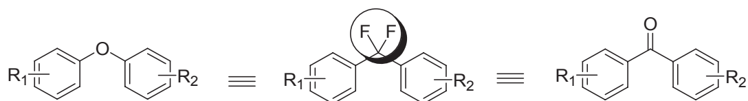
Scheme 1. Diaryl ethers, benzophenones and gem -difluoro-bisarylic derivatives.
