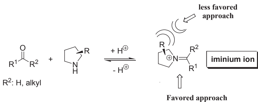
Scheme 4. Activation, with stereinduction, of aldehydes/ketones by chiral amine.
