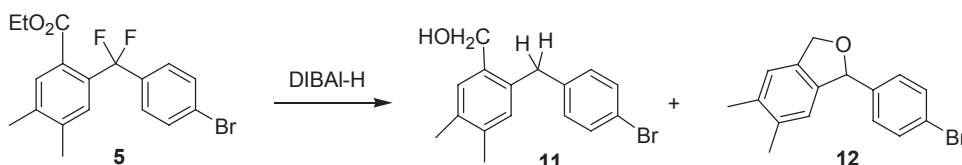
Scheme 10. Reduction of intermediate 5 by DIBAL-H.
