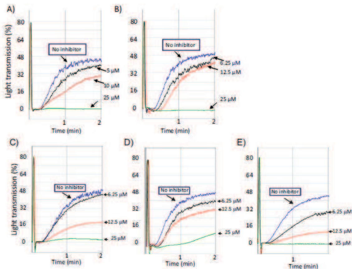
Figure 1. Biological activity of type (I) compounds.
