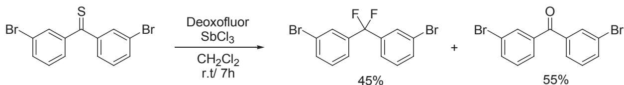
Scheme 2. gem -difluorination of benzophenone-derived thioketone.
