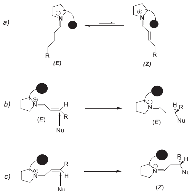
Scheme 26. ( Z )/( E ) equilibrium of iminium ion and its effect on the final product.
