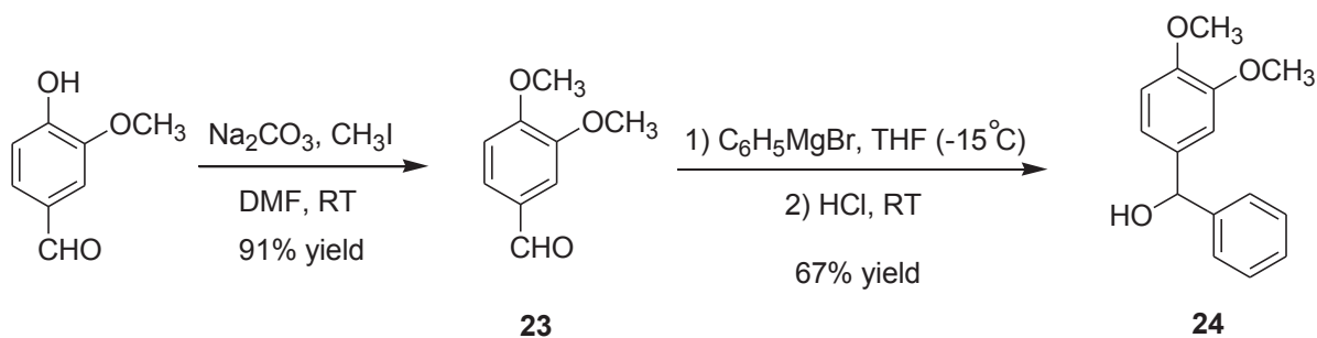
Scheme 15. Synthesis of protected phenol 24 .
