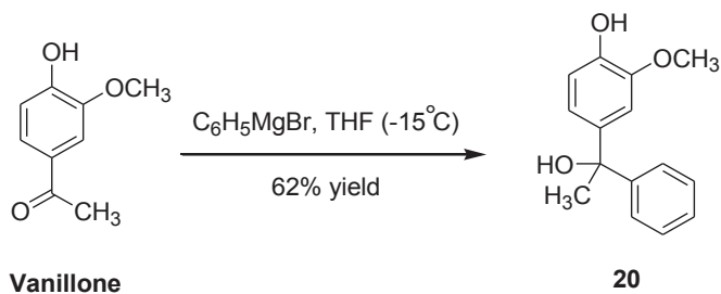
Scheme 12. Preparation of phenol 20 .
