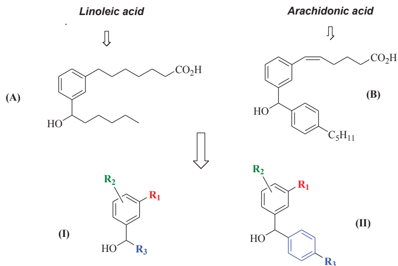
Figure 2. Simplified analogues of A and B.
