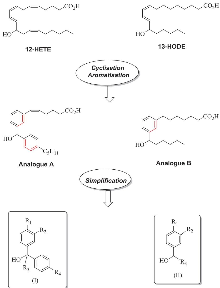
Scheme 1. Simplified analogues of 12-HETE and 13-HODE.
