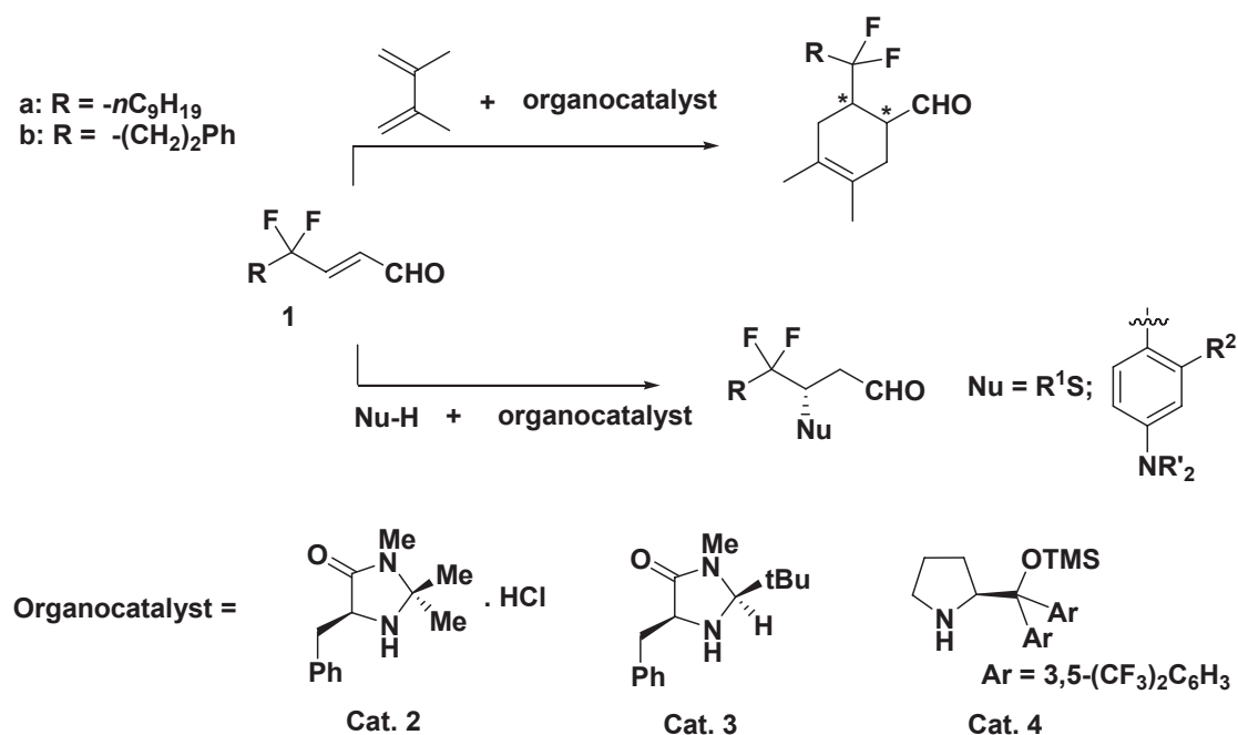
Scheme 13. Goals for Diels-Alder cycloaddition and 1,4-conjugated additions to enals 1 .
