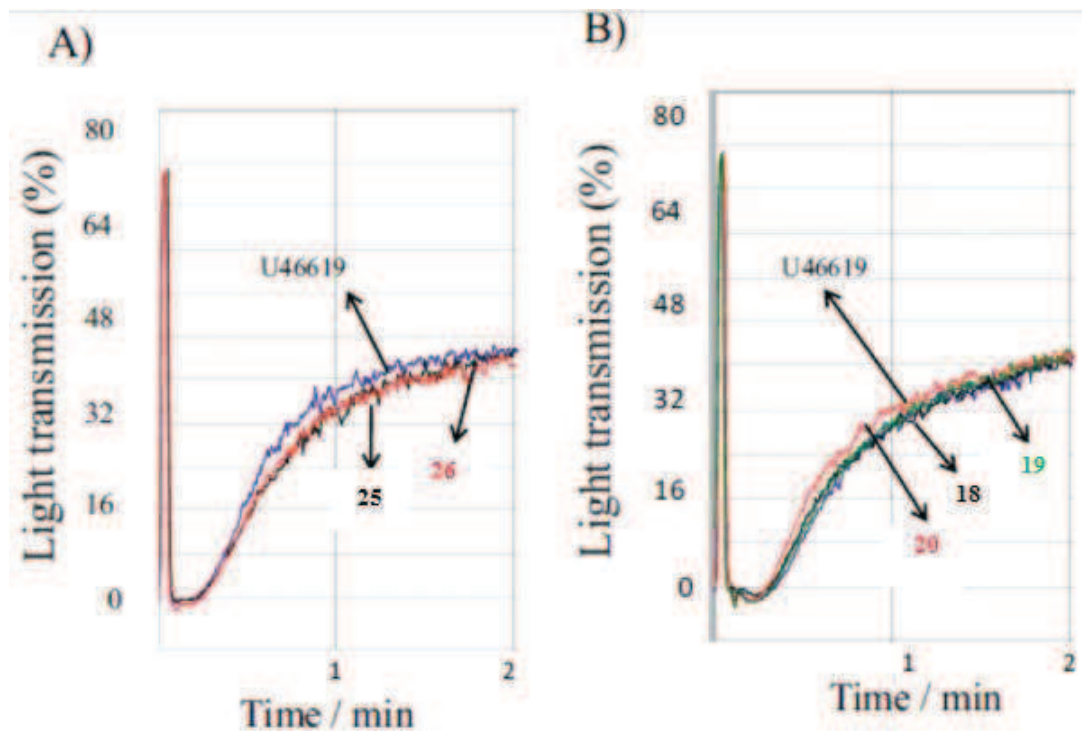
Figure 6. Action on thromboxane receptor.
