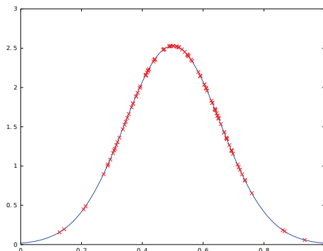
Figure 2.6 – We illustrate the process of importance sampling a 1D distribution. From the target pdf (in blue), we draw samples (in red) whose density is equal to the pdf.
