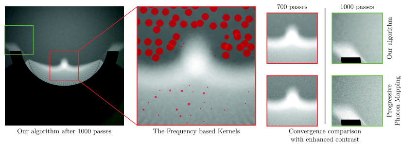
Figure 5.16 – We compare the convergence of two regions of the caustic scene. Those regions contain both high frequency and low frequency content. The low frequency regions exhibit less noise than the high frequency ones.
