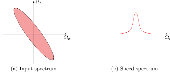
Figure 5.2 – We want to estimate the spectrum of the signal (here in space-time) along the spatial axis, after integration of the time domain ((a) in blue). We apply the slice theorem and evaluate the covariance matrix based on a Gaussian approximation.
