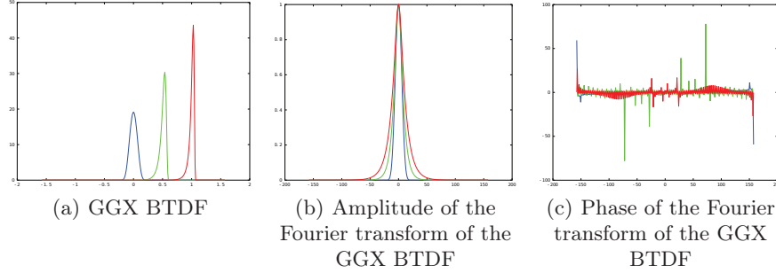
Figure 3.27 – GGX BTDFs are not isotropic for grazing angles (a), but the amplitude of their Fourier transform is (b). The non-symmetrical information is stored in the phase (c). We approximate the Fourier spectrum of GGX BTDFs by Gaussians which standard deviation correspond to the inverse roughness, much like de Rousiers et al. [39]. We used a glass index of n = 1.1 , the incoming angles are 0 , \frac{\pi}{6} , and \frac{\pi}{3}
