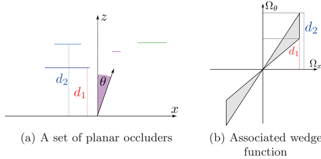
Figure 4.4 – The wedge function describes the area in which the occluders spectrum is enclosed.
