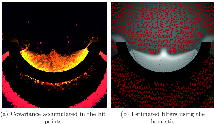
Figure 5.14 – Covariance can be visualised as hit points map to pixels. We show here the accumulated covariance at the surface of objects (a). The scene is composed of a curved mirror on a diffuse surface. The light creates a caustic and a soft shadow. Aside (b), we display estimated filters drawn on top of the final image. The filters are small in the high frequency regions (caustic and shadow).
