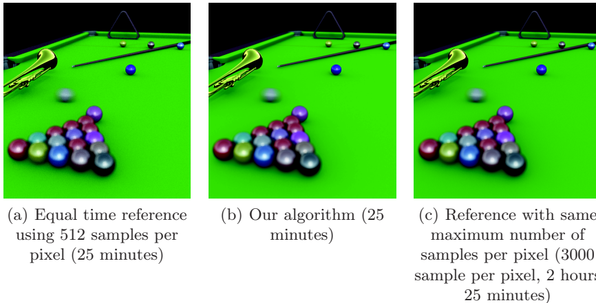
Figure 5.9 – The snooker scene rendered using our algorithm at the center, with a path tracer using the maximum number of samples in a pixel used in our algorithm at the right (same quality), and using the same amounts of time as our algorithm at the left.
