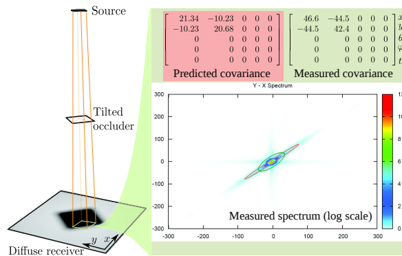
Figure 4.10 – We analyse a soft shadow cast by a tilted plane. The covariance is estimated after the reflection by the diffuse plane. The resulting spectrum exhibits the same orientation. The measured spectrum is estimated using a windowing of the measured light-field. This windowing increases the frequency content of the spectrum. We can see this difference on the plot (the cross) and on the measured covariance.
