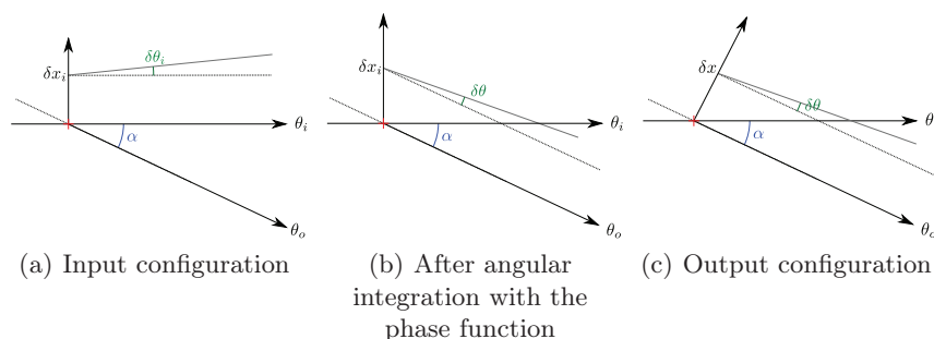
Figure 3.31 – The input configuration of the scattering operator. The input local light-field (a) is first convolved with the phase function resulting in an intermediate light-field with angular and spatial components unaligned (b). Finally, we integrate the spatial component in the outgoing frame along the outgoing direction (c).
