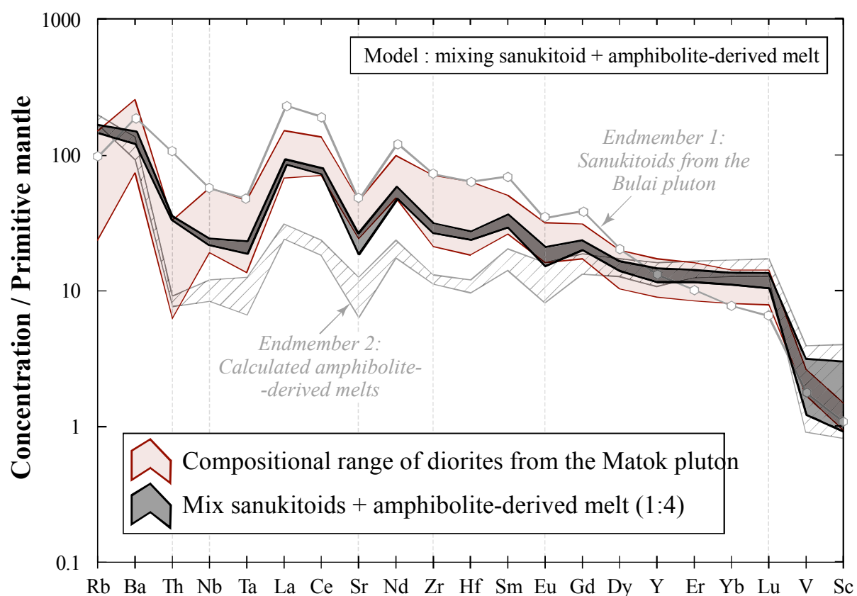
FIGURE 5.17: Results of the mixing model between the amphibolite-derived melt (calculated as described in caption of Figure 5.16a) and average composition of mafic sanukitoids ( \text{SiO}_2 = 46\text{--}57 wt.%) from the Bulai pluton (Laurent et al., 2011), presented in multi-element diagrams (normalization values as in Figure 5.13). The resulting compositional range reasonably well fit that of diorites from the Matok pluton.
