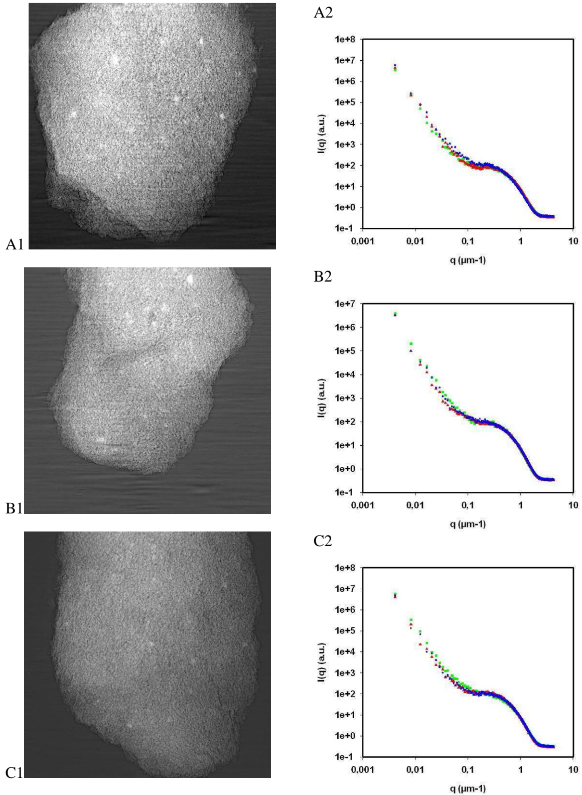
Figure 3: X-ray micro-tomography 3D projections images (A1, B1, C1) and corresponding to small-angle scattering curves (A2, B2, C2) for samples before treatment (T0) (A1, A2), after treatment - (B1, B2) and after treatment + (C1, C2).
