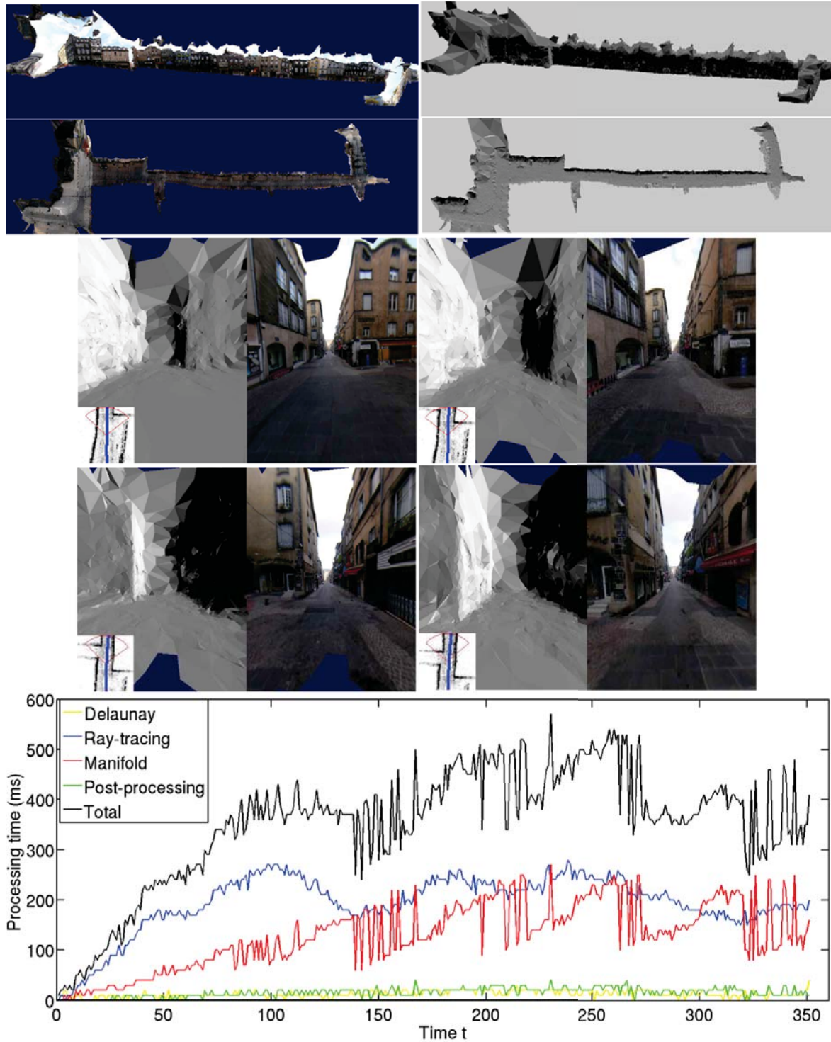
Figure 7.28: Incremental surfaces of Clermont-Ferrand Downtown sequence. Row 1,2 show two bird views of the final surface. Row 3,4 show local views of the surface at four times. Row 5 shows the processing time in function of time. Here, about 200 points are added in the Delaunay each time.
