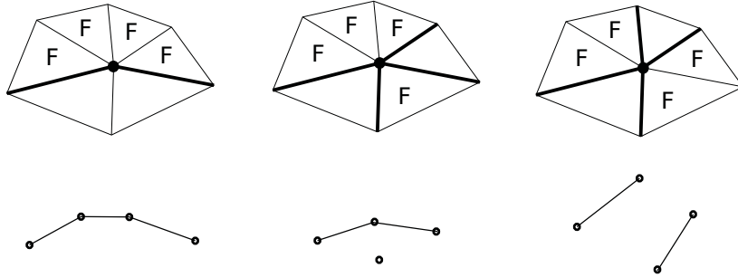
Figure 4.4: Tetrahedra incident to edge e in the original surface \delta F and the adjacency graph g_e in the 2d case. In the 2d case, edge e is a vertex and tetrahedra are triangles. In top, we see free-space tetrahedra (triangles labeled F) and matter tetrahedra (triangles with no label). All these tetrahedra contain edge e (round point). We see also triangles (bold segments) in \delta F which contain e . In bottom, we see the corresponding adjacency graphs of F_e .
