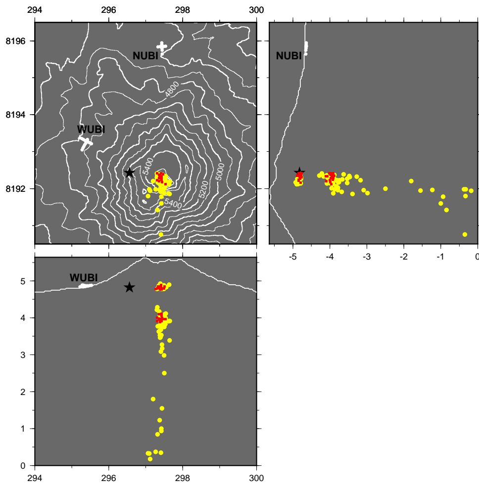
Figure 4.3: Hypocenter located at Ubinas volcano, with some events recorded during the field experiment at Ubinas in 2009. Yellow circles correspond to localization of long-period events, red circles correspond to explosion events and black star corresponds to volcano tectonic event.
