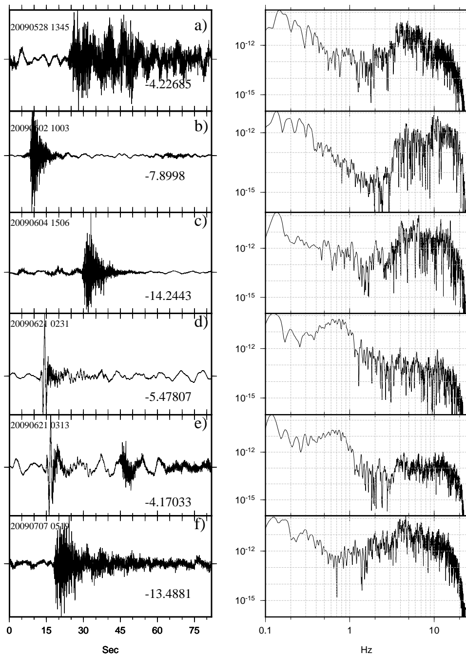
Figure 1.21: Typical unfiltered seismograms, indicating date in the upper left and minimum amplitude in \mu\text{m/s} (left) and their spectra (right), recorded at Ubinas experiment in 2009. . a) LP, b) VT, c) hybrid, d) LP e) LP and f) LP.
