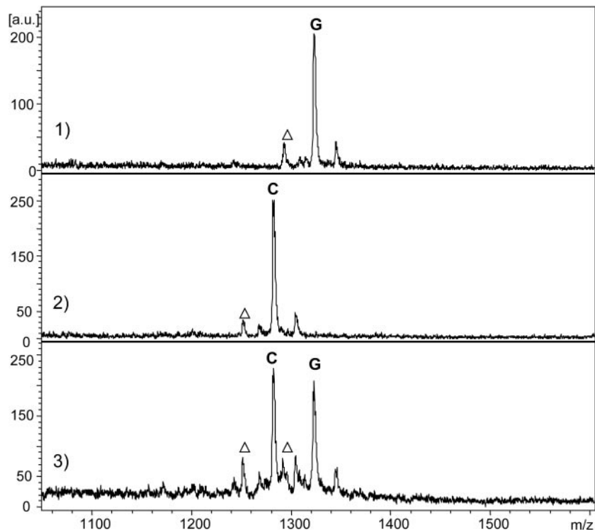
Figure 3. Spectra of the SNP FANCA 10191: (a) shows the protocol using desalting with ion exchange resin, Na + adducts are labeled with (asterisk); (b) shows the protocol with alkylation and no desalting. Peaks associated with exchanges of S by O, which then cannot be alkylated, are labeled with open triangle. Homozygous samples for each of the two alleles and a heterozygous sample are shown (1–3°).
