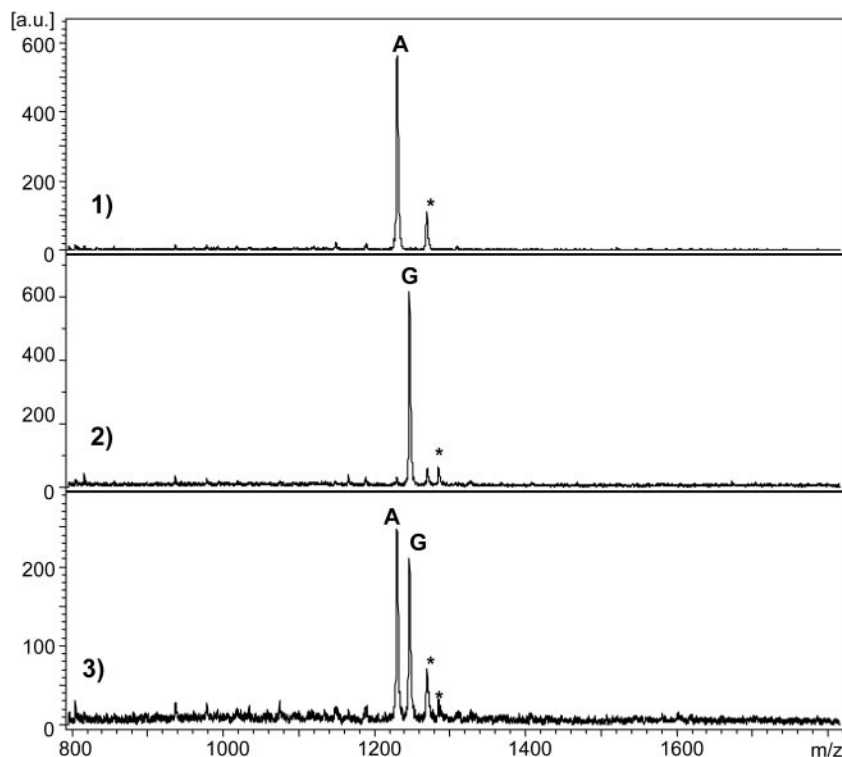
Figure 2. Spectra of the SNP KIAA 0604_18550 (A/G): (a) shows cleavage with NaOH. Na + adduct peaks (asterisk) are observed at +22 Da from the real allele-peaks; (b) shows cleavage with KOH. K + adduct peaks (asterisk) are observed at +38 Da from the real allele-peaks. In addition +22 Da Na + adducts are detected due to ubiquitous Na + . (1) Mass spectrum of a homozygous DNA sample for the first allele, (2) mass spectrum of a homozygous DNA sample for the second allele, and (3) mass spectrum of a heterozygous sample.
