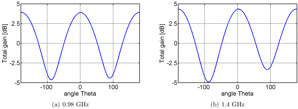
Figure 2.25: Cuts of radiation pattern at \phi = 0^\circ of the asymmetrical Archimedean spiral of Fig. 2.23(a).
