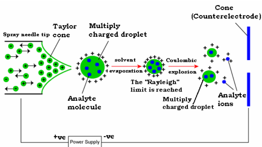
Figure 3: A scheme showing the formation of ions by electro-spray method. The above figure has been taken from the mass spectrometry resource of department of chemistry of University of Bristol. 6
