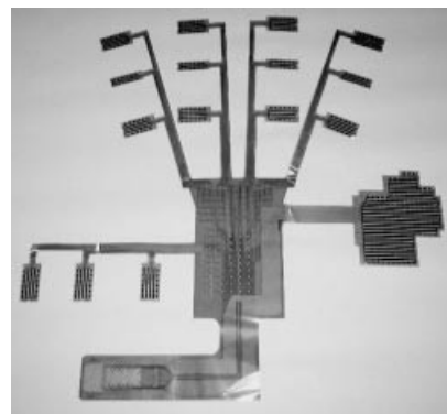
(b) The sensor has grid pattern electrodes and uses conductive ink whose electric resistance changes in proportion to pressure.
