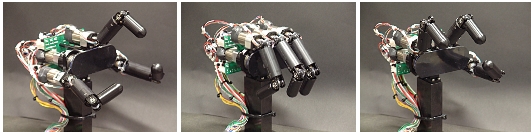
(a) A few of many different kinematic configurations. Each finger has two flexion/extension degrees of freedom. The middle finger is fixed on the palm; the other ones can rotate around it.
