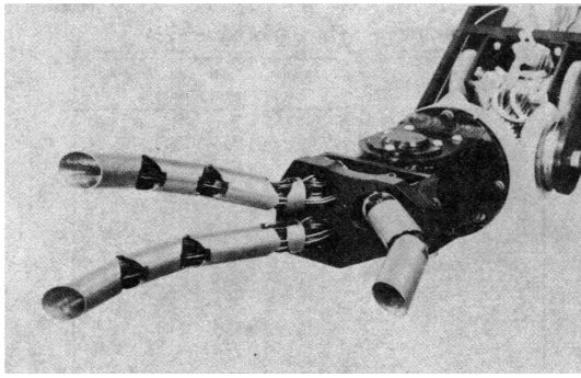
(a) Close-up photograph of the hand. The finger ends may be stuffed with small rubber balls.
