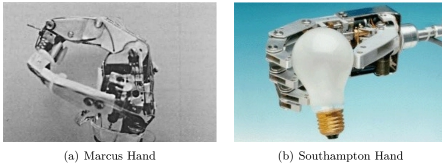
Figure 3.35 – Two artificial hands implementing the Southampton Adaptive Manipulation Scheme for hierarchical control of grasping
