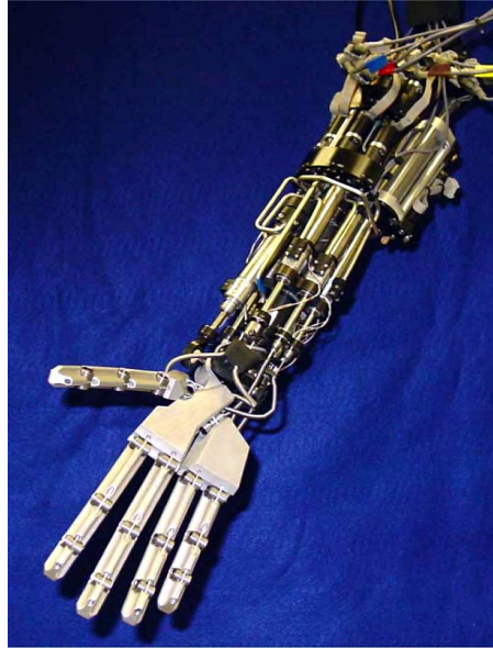
Figure 3.25 – The prosthetic Vanderbilt Arm. The pneumatic actuators are located in the forearm, similarly to our muscles (see section 2.1.2 on muscle anatomy, in chapter 2).
