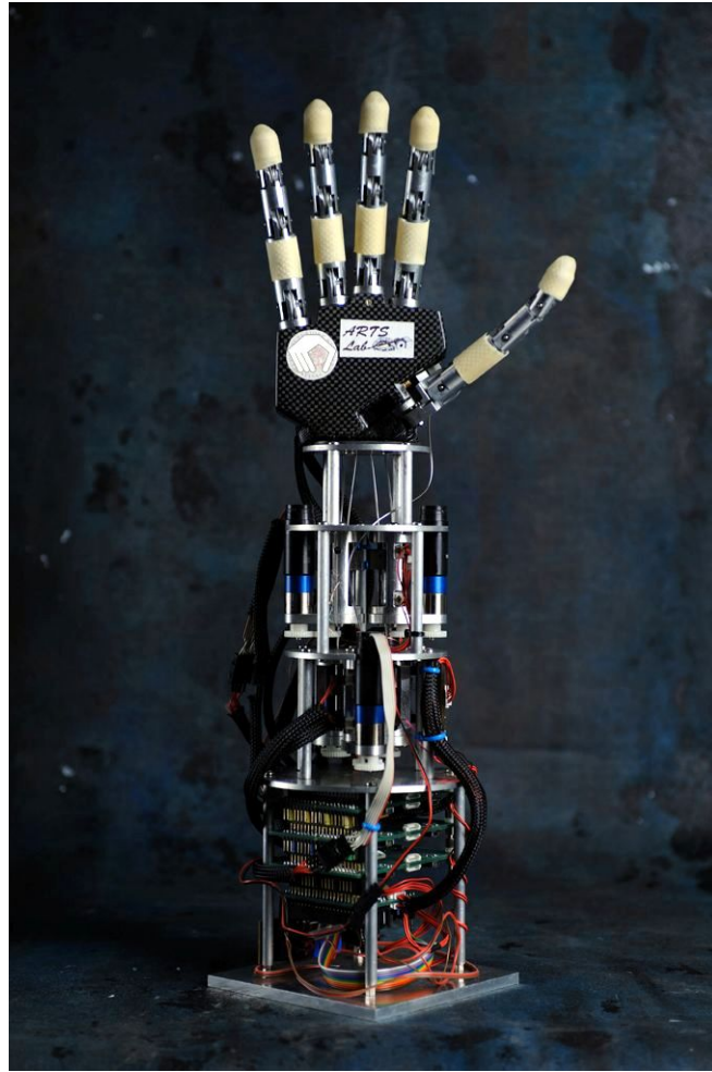
Figure 3.39 – Complete view of the CyberHand prototype prosthesis. The extrinsic electric actuators are visible below the hand, as well as the control printed circuit boards, below the motors.
