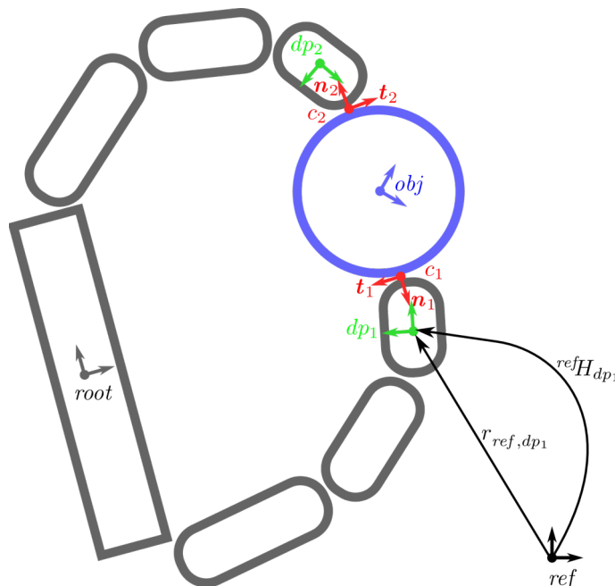
Figure 5.2 – Reference frames, body frames, contact frames, and rigid transformations between these frames
