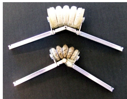
(b) The bellows that are inside the actuators (two sizes of actuators) (Gaiser, Pylatiuk, Schulz, Kargov, Oberle, and Werner 2009).
