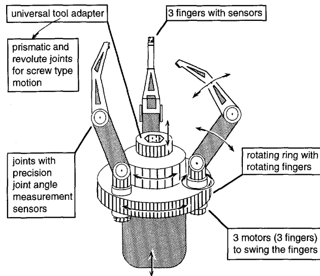
Figure 3.99 – A drawing of the Teleman Dextrous Gripper (1993) and its degrees of freedom. From Ham (1997, page 14).
