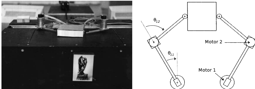
Figure 3.77 – Styx Hand (1988). Photograph from Murray, Z. Li, and Sastry (1994, page 12), drawing from Murray and Sastry (1989).
