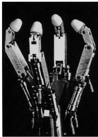
Figure 3.98 – The TUM Hand (1993)
