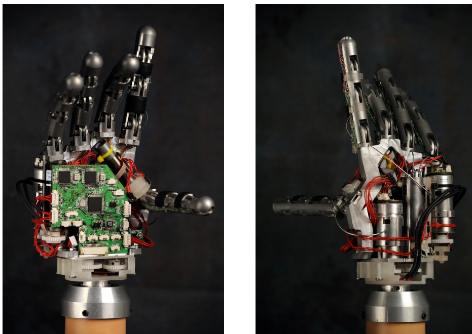
Figure 3.40 – SmartHand self-contained design: the electric actuation units and the control printed circuit board are in the palm of the hand. The dimensions are comparable to that of the human hand.
