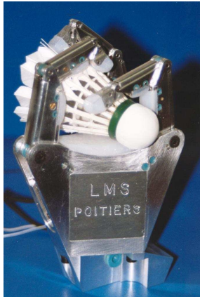
(a) An adaptive three-fingered hand with three phalanges per finger and one actuator for the whole device, developed at the University of Poitiers (1991). From Zegloul, Arsicault, and Gazeau (2007).
