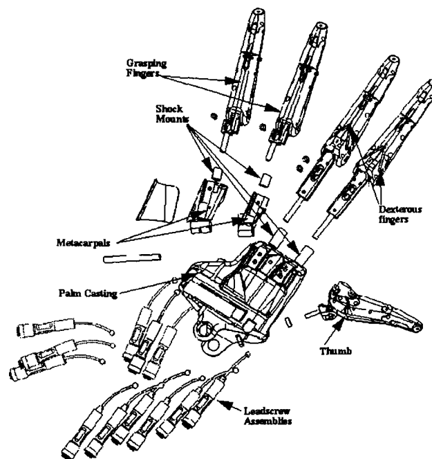
Figure 3.114 – Robonaut 1 Hand (Lovchik and Diftler 1999)
