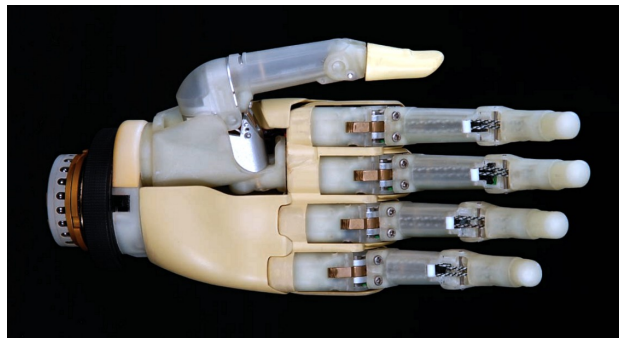
Figure 3.13 – An example of (advanced) myoelectric hand prosthesis: i-Limb Hand, by British company Touch Bionics (2009) of Edinburgh, Scotland. It is pictured here without its artificial skin covering.
