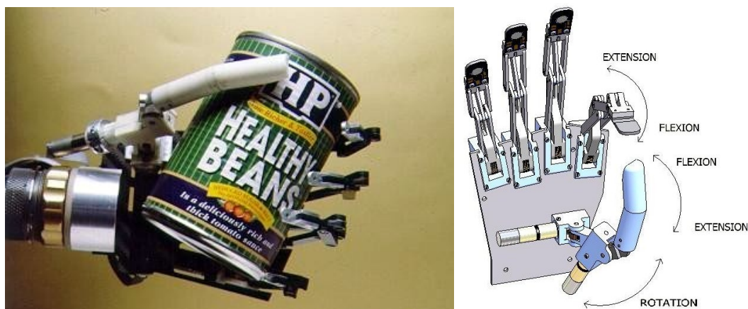
Figure 3.36 – The Southampton Remedi Hand and its six actuated degrees of freedom
