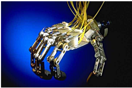
(a) The bare exoskeleton design makes the hand quite unfit to whole-hand grasping. It is more adapted to fingertip manipulation.
