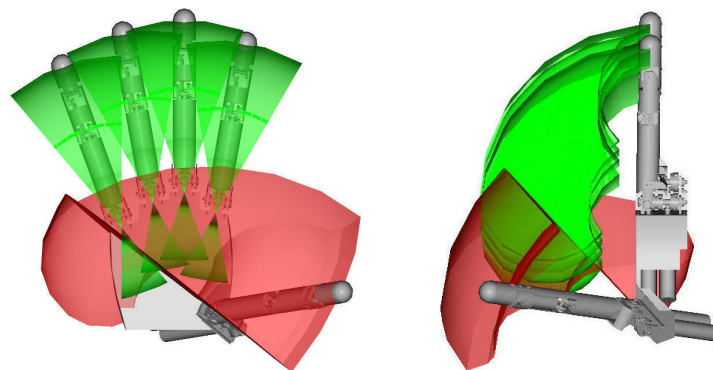
Figure 3.133 – Workspace of the fingertips of the Gifu Hand III
