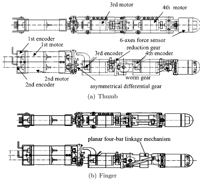
Figure 3.130 – Mechanical design of the digits of the Gifu Hand II. They are built as exoskeletons, and the thumb is slightly longer. All the servomotors use DC motors and reduction gears, and include magnetic position encoders. The transmission to the joints is gear-based and does not include tendons.
