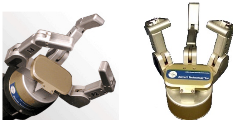
Figure 3.79 – The Barrett Hand (1999). Also known as BH8, 8 for the number of axes.
