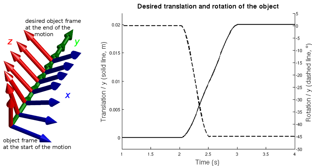
Figure 5.16 – Desired motion for the object’s body frame
