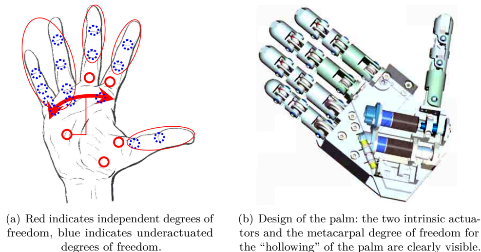
Figure 3.146 – Degrees of freedom and degrees of actuation in iCub’s hands
