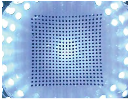
Figure 2.46 – The compliant sensor by Y. Ito, Y. W. Kim, and Obinata (2009). View from inside the fingertip.
