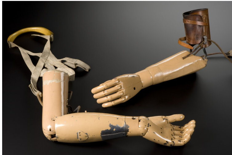
Figure 3.20 – Carnes arms for above-elbow and below-elbow amputations (1915). Each finger has two degrees of freedom in flexion-extension. The thumb has only one degree of freedom which makes it approximated to the index finger in a precision grip. The wrist has flexion-extension and pronosupination.
