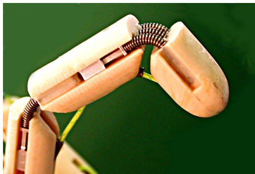
(a) Load cell used in the final version of the hand (at the basis of the spring). It has one strain gauge on each side.
