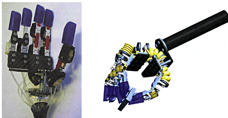
Figure 3.88 – FRH-4 Hand (2008). The picture on the right illustrates the three-jaw gripper behavior. We are left to think that FRH stands for “fluidic-driven robotic hand”.
