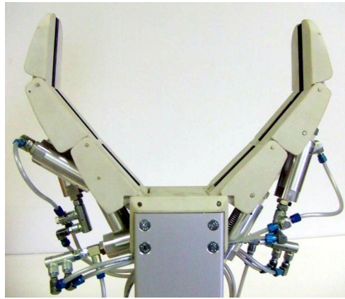
(b) The Twix Hand, made at the University of Montpellier (2007). Each phalanx is actuated by its own air cylinder, but all cylinders are connected to the same source of pressured air, hence the underactuation. The gripper is probably named after the Twix candy bars, shaped like fingers and sold in pairs. From Bégoc, Krut, Dombre, Durand, and Pierrot (2007a).
