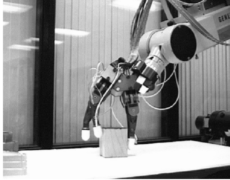
(b) It can be mounted as the end-effector of a manipulator arm.
