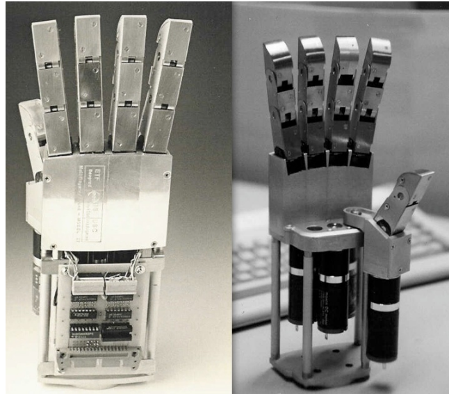
Figure 3.71 – The Belgrade/USC Hand (1990), without its external contact/force sensors
