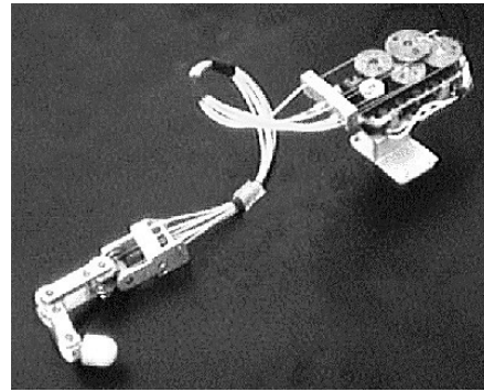
(b) A finger with its six tendons and five actuators (sheathed polyester cables, DC electric motors with reduction gears)
