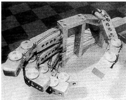
(a) In half-open position. The tendon cables and pulleys are visible on the side of the fingers.
