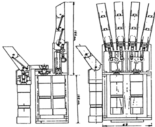
Figure 3.72 – The rocker arm mechanisms coupling the fingers are visible on the right, in the palm area. The linkages coupling the phalanges are visible on the left.
