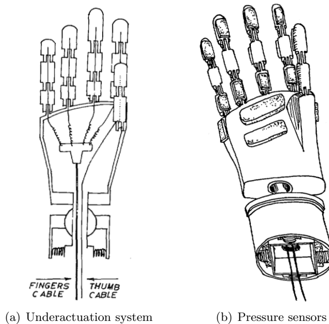
Figure 3.30 – The adaptive hand described by Tomović and Boni (1962). The pressure sensors are visible on the palm, proximal phalanges and distal phalanges.
