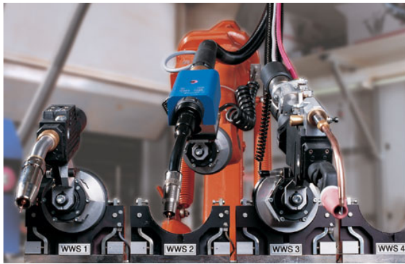
(a) A rack-based tool changing system sold by the German firm Abicor-Binzel. The tools are different welding torches.
