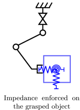
Figure 5.6 – Principle of compliance control and impedance control, for a single manipulator, with only the virtual spring elements depicted (adapted from T. Yoshikawa 2010)
