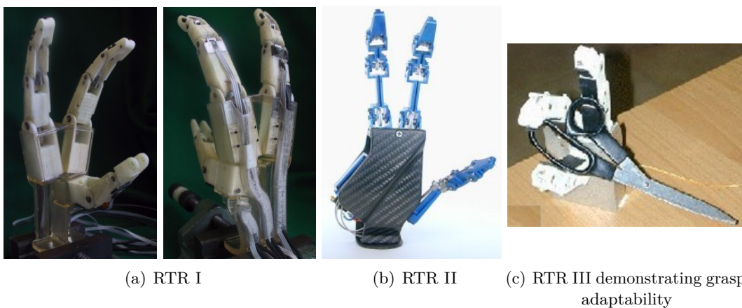
Figure 3.38 – The RTR Hand series
