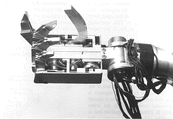
Figure 3.86 – Crowder’s hand for a glove box manipulator (1987)
