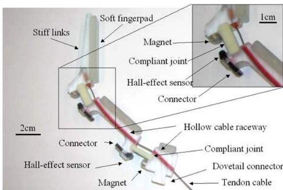
Figure 3.84 – The SDM Hand (2006). From Dollar and Howe (2006b).
