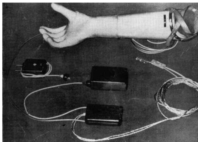
Figure 3.29 – The Russian Hand (mid-1950s). From Childress (1985): “The external battery pack is shown in the center of the photograph. The electronic package is beneath the battery. The battery charger is at left. Note the long electrode wires and the prosthesis suspension straps.”
