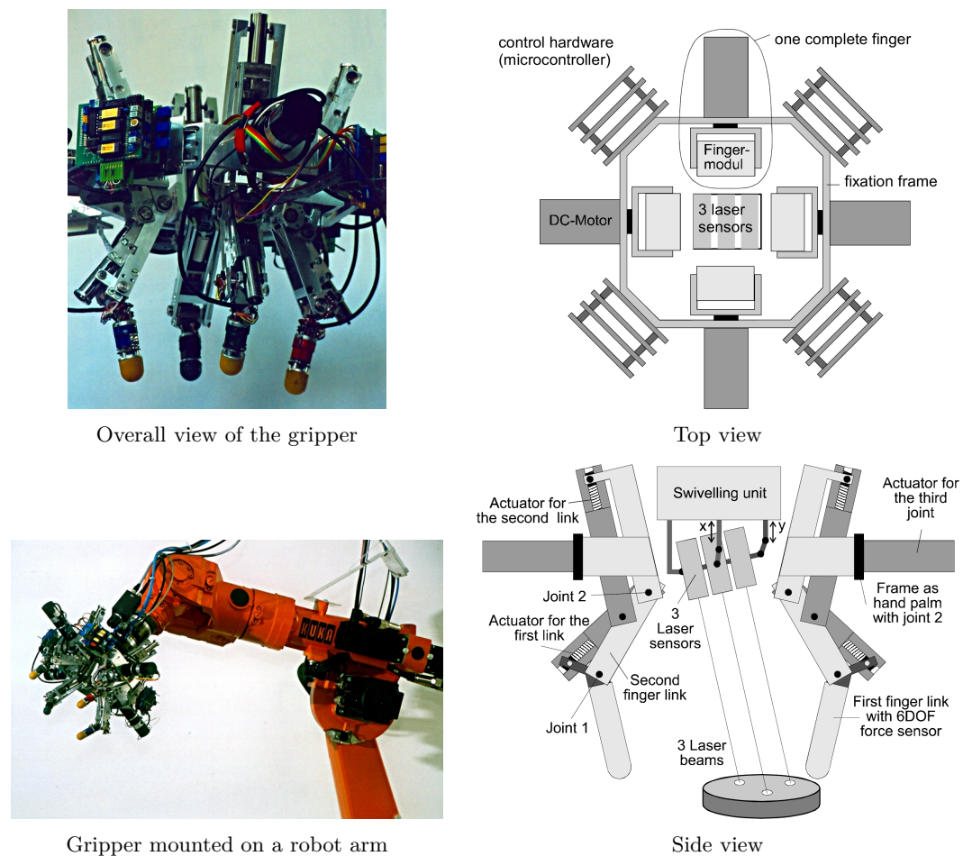
Figure 3.94 – The Karlsruhe Dextrous Hand II (1997). From Osswald and Wörn (2001).
