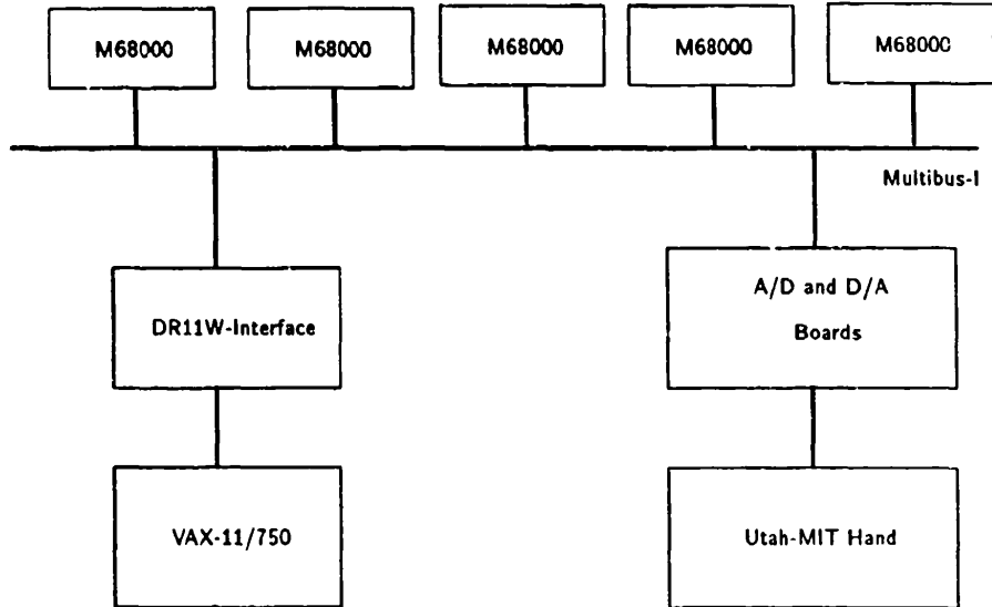
(a) Version I of the hardware
