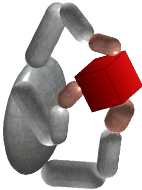
Figure 5.13 – A bad case of kinematic redundancy and articular limit violation during a three-fingered manipulation. If anthropomorphism of joint configuration is not specified as a control objective, there is no reason for the control to achieve it.
