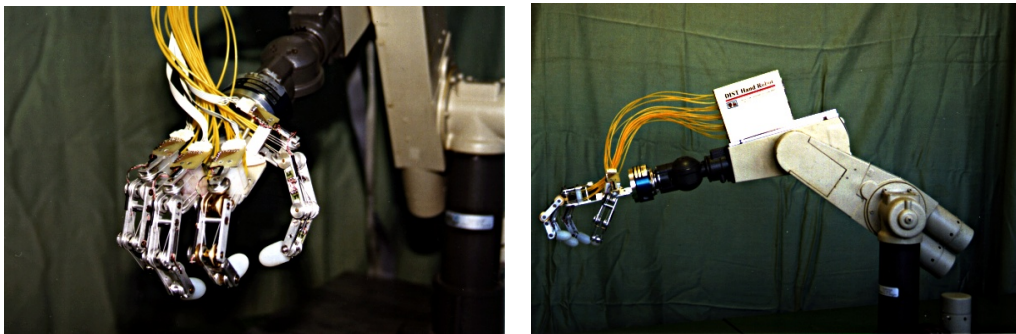
Figure 3.125 – The DIST Hand and its actuator pack mounted on the forearm of a small PUMA manipulator (Panin 2002)
