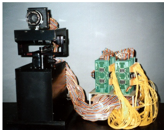
Figure 3.100 – First high speed vision system from the University of Tokyo, Ishikawa/Oku Laboratory. The image sensor, located on top of its pan/tilt unit, is connected to the processing electronics via parallel lines.
