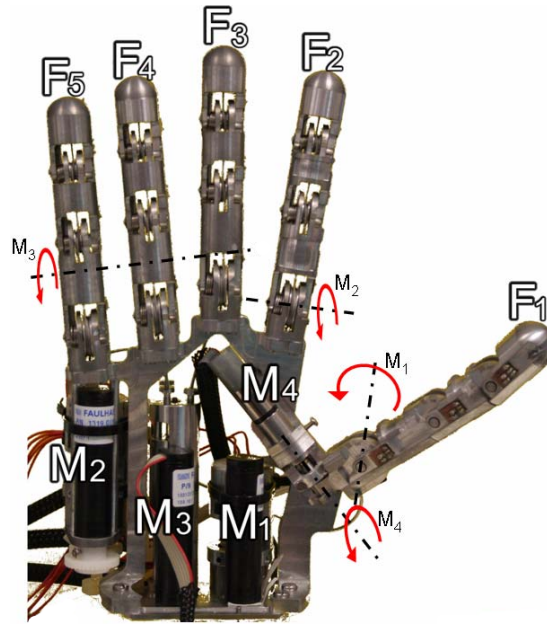
Figure 3.41 – SmartHand motors and degrees of actuation: M1 flexes the thumb, M2 the index finger, M3 the middle, ring and little fingers through a differential mechanism, and M4 rotates the thumb.
