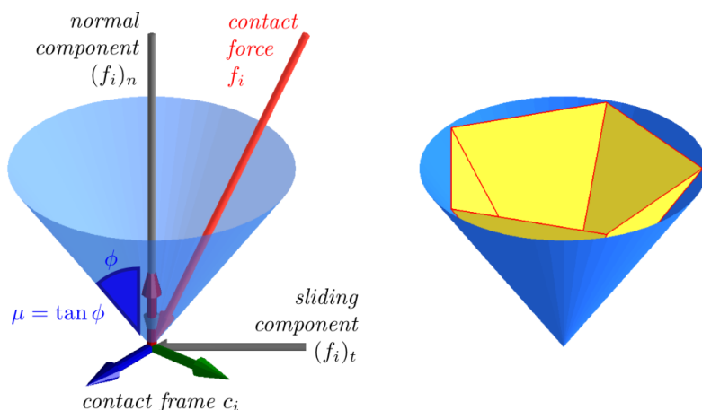
Figure 6.12 – A non-sliding contact, its exact contact cone, and a linearized contact cone
