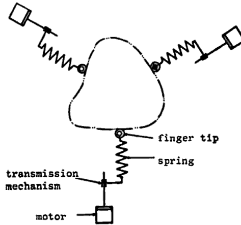
Figure 3.59 – A schematic drawing of Hanafusa and Asada’s “robot hand with elastic fingers” (1977). It is a planar construction designed to grasp two-dimensional objects stably and to execute incremental motions of the object within the grasp.
