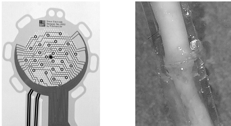
(b) Sieve electrode are implanted by transecting the nerve stump and letting its fibers regenerate through the array of holes, encased in a guidance tube (Navarro, Krueger, Lago, Micera, Stieglitz, and Dario 2005). Some of the holes are platinum-deposited contact electrodes, in black on the picture on the left. The picture on the right shows a regenerated nerve through a polyimide sieve electrode.
