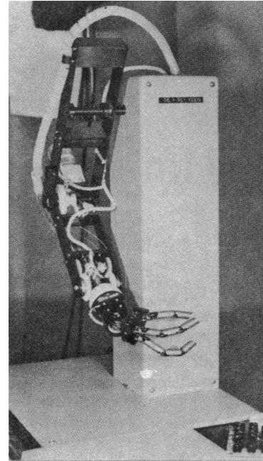
(c) The complete system. All the motors of the hand are inside the big box, and the tendons come out of it through the large hose, each in its own sheath, to go all the way down the hand.
