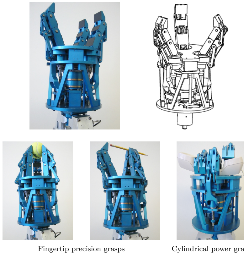
Figure 3.82 – The Sarah Hand (1999). The name stands for “self adaptive robotic auxiliary hand”. The linkage-based underactuation mechanisms are visible on the back of each finger. From Laval University Robotics Laboratory (2010).
