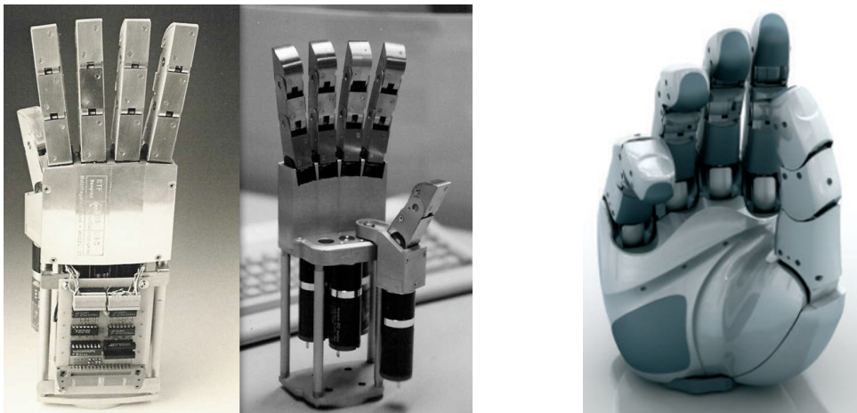
(a) The Belgrade/USC Hand, developed in the 1980s at the University of Belgrade in Yugoslavia (now Serbia) and the University of Southern California in Los Angeles, California. A milestone in the history of robot hands.
