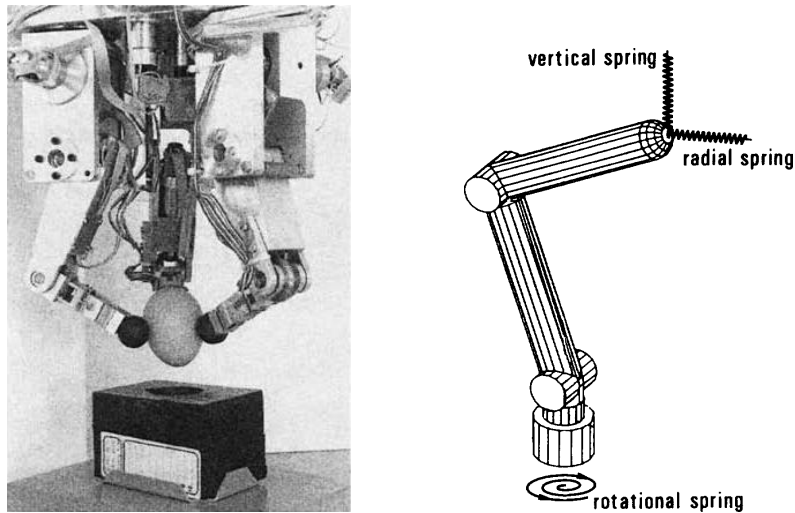
Figure 3.96 – The Leuven Hand (1989) and a schematic representation of the low-level control of a finger
