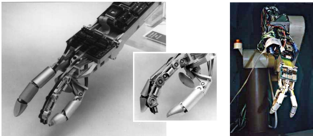
Figure 3.119 – Various views of the UB Hand 2 (1992). The covers of one of the upper fingers are removed to show the inside.
