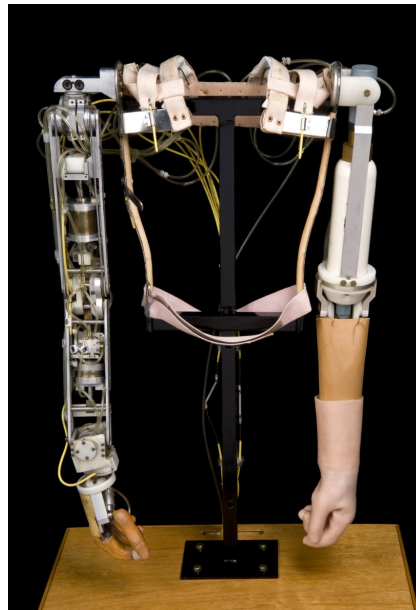
Figure 3.24 – A gas-powered prosthetic system for thalidomide children with upper bilateral amelia, made in the 1960s at the orthopedic hospital in Edinburgh, United Kingdom (Science Museum London 1979). The active arm may be hidden by clothes or a cosmesis. The compressed carbon dioxide is stored in canisters in the passive arm.
