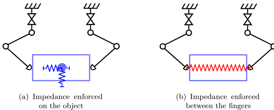
Figure 5.11 – Principle of compliance control and impedance control, for fingers, with only the virtual spring elements depicted (adapted from T. Yoshikawa 2010)
