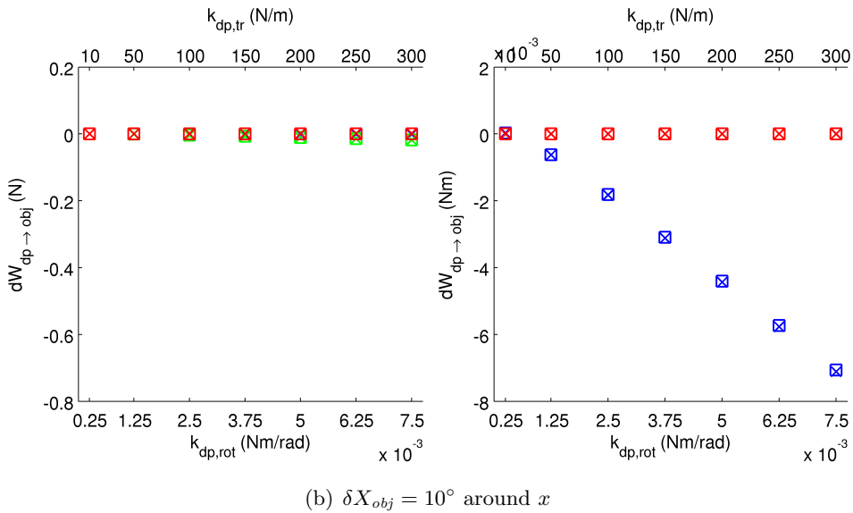
Figure 7.10 – dW_{dp \rightarrow obj} as predicted by (7.27) (boxes) and returned by the simulation (ticks), for various values of k_{dp,tr} (top horizontal axis) and k_{dp,rot} (bottom horizontal axis). We tried six different cases of \delta X_{obj} ; this figure presents the motions relative to the axis x of the object frame. In each case, the left subplot shows the three coordinates of the force part of dW_{dp \rightarrow obj} and the right subplot shows the three coordinates of its moment part. Blue, green, and red correspond respectively to the x , y , and z coordinates of the forces and moments, in the object frame (blue boxes and ticks are sometimes hidden by the green or red ones at the zero horizontal line).
