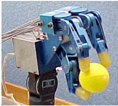
(a) The hand's kinematic structure is optimized for fingertip manipulation of one-inch wide spheres.
