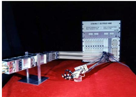
Figure 3.69 – The whole Utah/MIT Dextrous Hand system: actuators, remotizer, hand, and low-level control system in the background (it is a box of control circuits, only the front side is visible).
