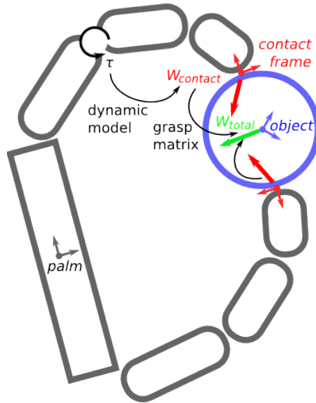
Figure 5.12 – A very shortened description of multifingered hand control.
