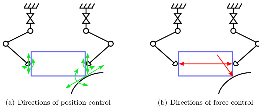
Figure 5.10 – Principle of hybrid force/position control, for fingers (adapted from T. Yoshikawa 2010)
