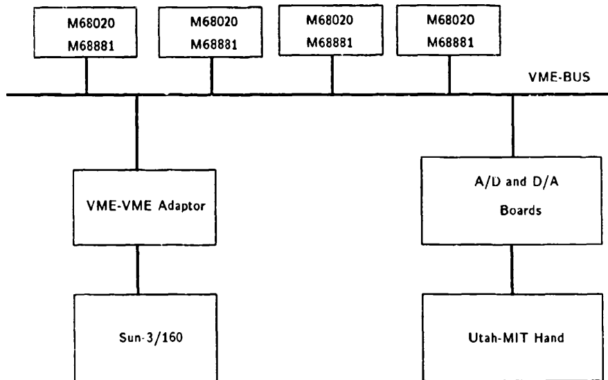
(b) Version II of the hardware
