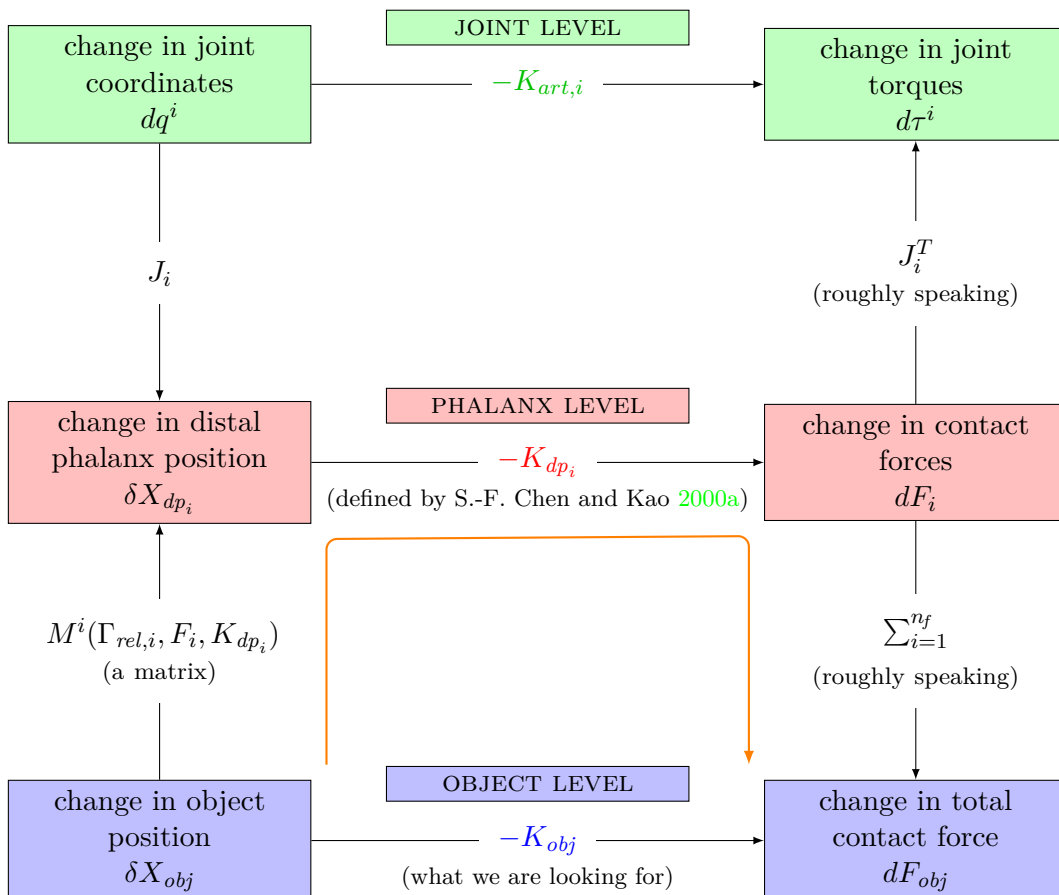
Figure 7.5 – Stiffness mappings at joint, phalanx, and object level. Our method for finding K_{obj} is represented by the orange arrow.
