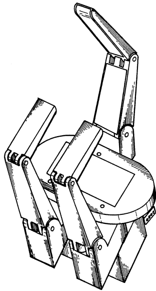
Figure 3.78 – A drawing of the UPenn Hand (1988), from Ulrich (1990)
