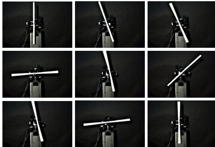
Figure 3.105 – High Speed Multifingered Hand spinning a stick between its fingers. The photographs are taken at intervals of 50 ms (i.e. from t = 0 s to t = 0.4 s).
