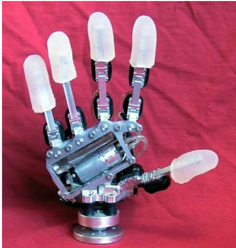
(a) FluidHand I (Schulz, Pylatiuk, Kargov, Oberle, and Bretthauer 2004a)
