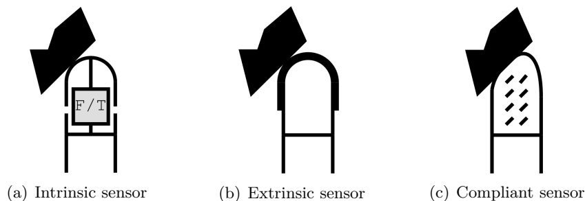
Figure 2.45 – Types of tactile sensors (from Tegin and Wikander 2004)
