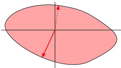
Figure 6.7 – How to describe the maximal robustness of a grasp without calculating the whole boundary of the admissible disturbance wrench space: a second approximation method
