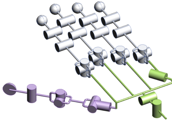
Figure 3.137 – Kinematic structure of the Shadow Dextrous Hand C6
