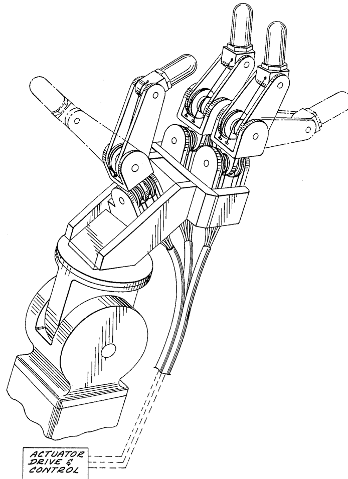
Figure 3.62 – A drawing of the Stanford/JPL Hand (1981). The three bundles of wires are the tendons, in their respective sheaths. From Ruoff and Salisbury (1990).
