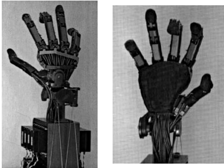
Figure 3.109 – The Anthrobot-3, back and front sides (Kyriakopoulos, Van Riper, Zink, and Stephanou 1997). The sheaths of the tendons are visible in the wrist and in the dorsum of the hand. The black boxes on each side of the base are servomotors.
