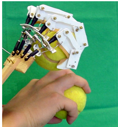
Figure 3.87 – The TUAT/Karlsruhe Hand (2000). The intermetacarpal joints are clearly visible, and the actuator tendon is also visible on the left.
