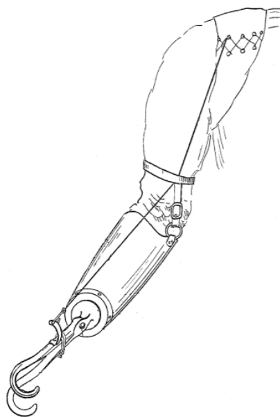
(a) The original split hook, as patented by Dorrance (1912)
