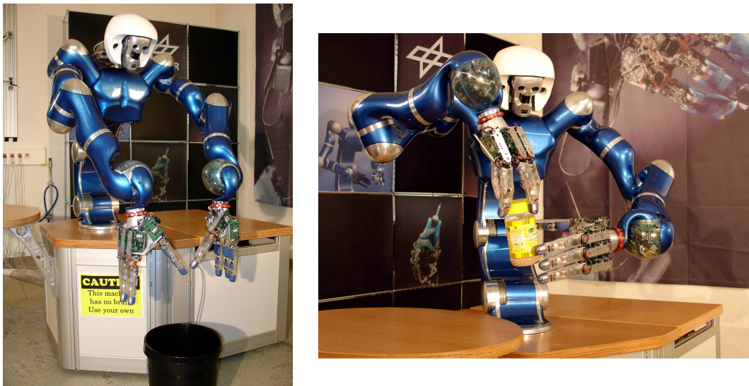
Figure 3.129 – DLR’s Justin, so called because it was finished “just in time” for the 2006 Automatica fair in Munich. The half-humanoid combines two of DLR’s most well-known realizations: the Lightweight Robot Arm III and the Hand II.
