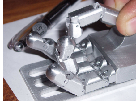
(b) Small four-fingered hand for the 70 cm humanoid robot UiNiKi of the University of Poitiers, France (Zeghloul, Arsicault, and Gazeau 2007). The hand has one actuator.
