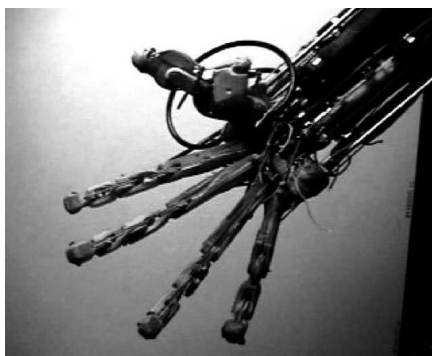
(a) Hand A. The skeletal frame has individualized metacarpals, and it is made of wood (maple).
