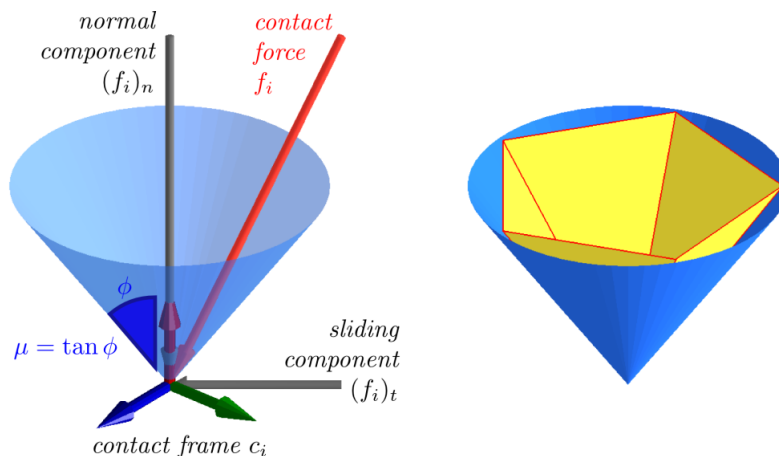
Figure 5.3 – A non-sliding contact, its exact contact cone and its five-faceted linearized contact cone
