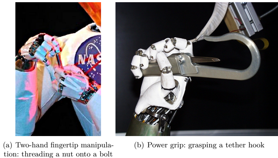
Figure 3.113 – Close-up views of Robonaut 1 Hands (1999)
