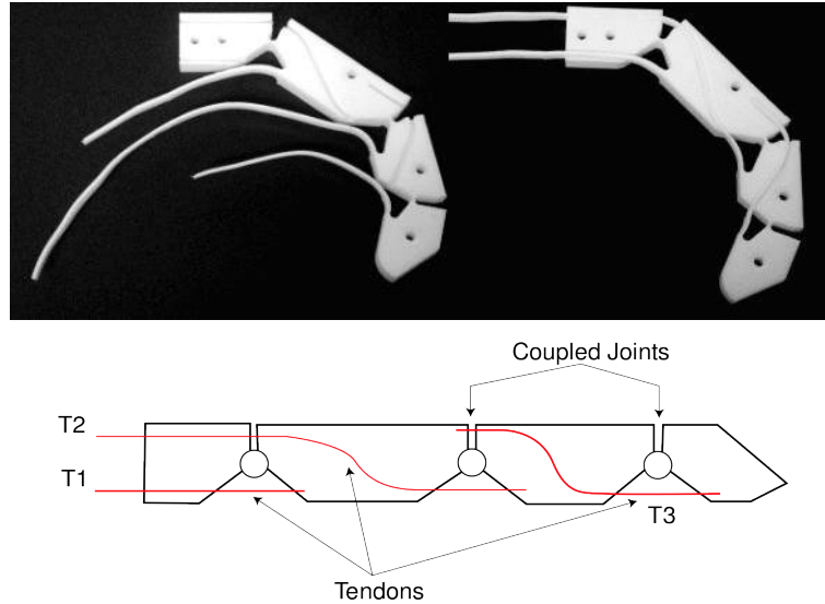
Figure 3.121 – A UB Hand 3 finger prototype (2002) as it comes out of the milling machine (left) and with the tendons put in place (right). Several routing paths have been tried out; here there are two motor tendons and one internal tendon coupling the two distal joints.
