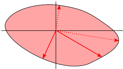
Figure 6.6 – How to describe the maximal robustness of a grasp without calculating the whole boundary of the admissible disturbance wrench space: a first approximation method
