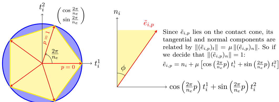
Figure 5.4 – Expression of the edges of a discretized contact cone. See also figure 5.3. Left: circular section seen from above; right: vertical section with respect to the p -th edge.
