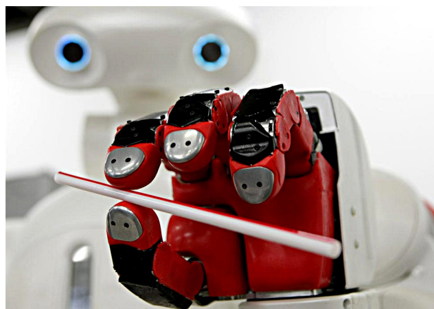
Figure 3.142 – Twendy-One's manipulation abilities have been demonstrated with a straw: the robot is able to switch between several opposition patterns without dropping it (thumb against index finger, against middle finger, against index and ring fingers, and so on). A video of this demonstration is available on the robot's website (Waseda University Twendy Team 2011).
