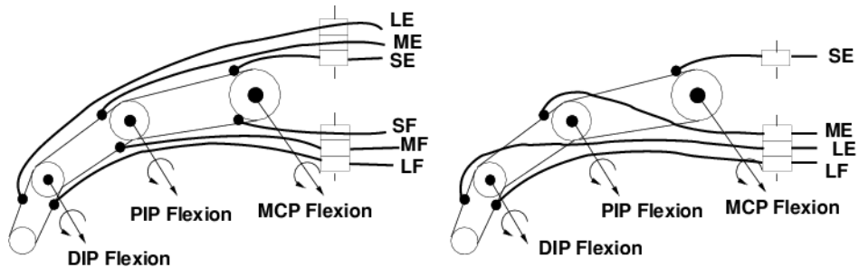
Figure 3.64 – Tendon actuation patterns: a “ 2n design” and a “ n + 1 design”. MCP, PIP, DIP: metacarpophalangeal, proximal interphalangeal, distal interphalangeal. E, F: extensor, flexor. L, M, S: long, medium, short.
