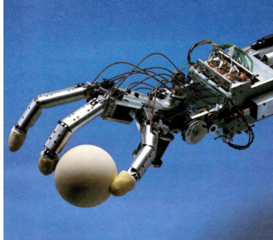
Figure 3.75 – The Hitachi Hand (1984), actuated by shape memory alloys
