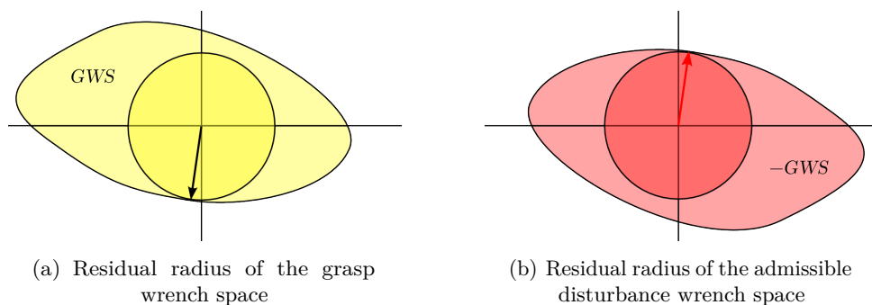
Figure 6.9 – A grasp quality measure, the criteria of the largest ball. It is the magnitude of the largest-minimum resisted external wrench.
