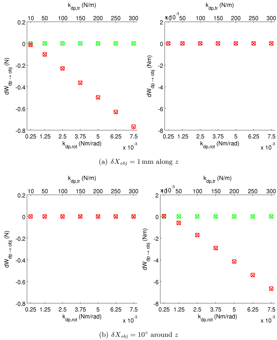
Figure 7.12 – Same as figures 7.10 and 7.11, but for the motions \delta X_{obj} relative to the axis z of the object frame.
