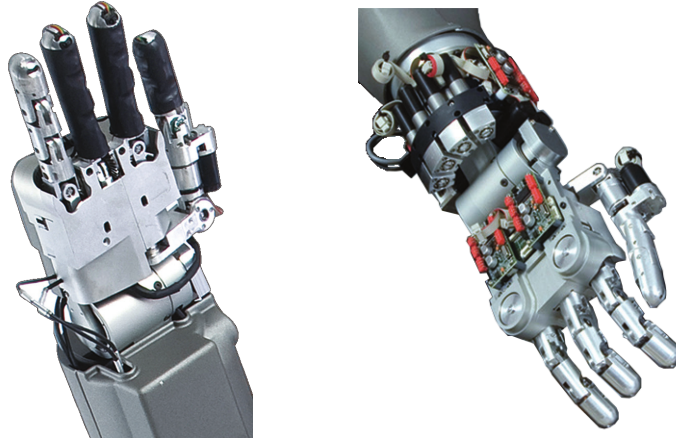
Figure 3.144 – The multifingered hand of Reem-B, palmar and dorsal views (from PAL Robotics 2011b)
