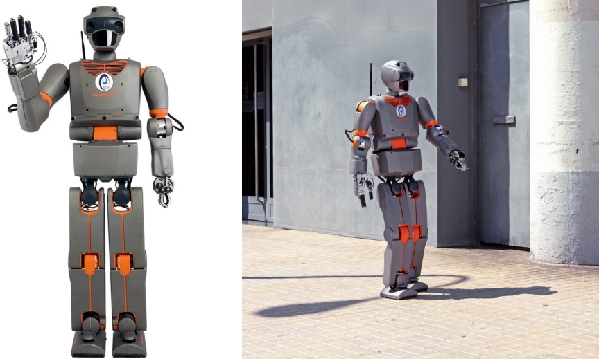
Figure 3.143 – Reem-B (2008). The humanoid is 147 cm tall and weights 60 kg. Its left hand is a two-degree-of-freedom gripper that can grasp heavy objects like bottles or books, whereas its right hand can grasp smaller objects in fingertip precision grips. The previous prototype Reem-A had only grippers, and the following Reem-H and Reem have three-fingered gripper hands.
