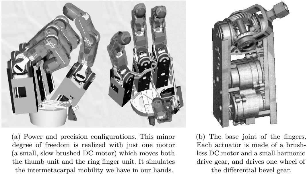
Figure 3.128 – Mechanical details of the DLR Hand II
