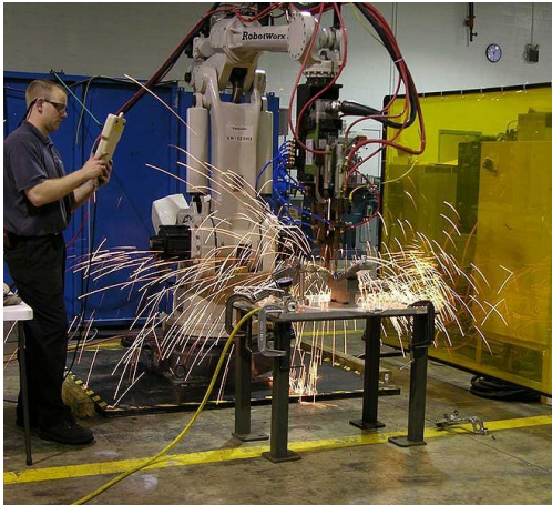
(a) A spot welding end effector, common in assembly lines. This one is human-operated.
