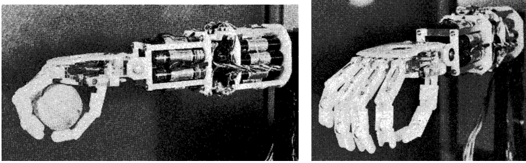
Figure 3.106 – Anthropomorphic hand for teleoperation, by Maeda, Tachi, and Fujikawa (1989). The actuators are arranged around an empty space and the wires which transmit power to the joints pass through this space. The forearm weights 2970 g, of which 2180 g are motors, including reduction gears and encoders. The hand weights only 370 g.
