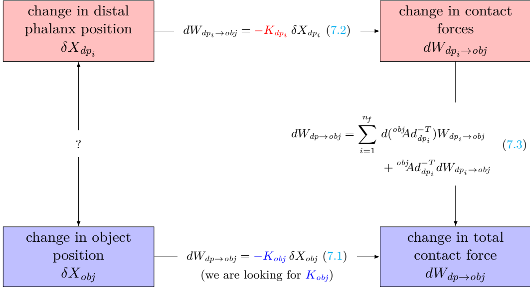
Figure 7.7 – Stiffness mappings in the cartesian space, at phalanx and object levels. Detailed relationships.
