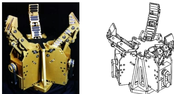
Figure 3.81 – The Mars Hand (1996). The name stands for “main articulé robuste sous-actionnée”, French for “robust underactuated articulated hand”. From Laval University Robotics Laboratory (2010).
