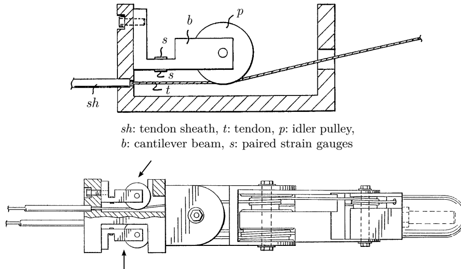
Figure 3.65 – Tendon tension sensors of the Stanford/JPL Hand, and their position at the base of the finger. From Ruoff and Salisbury (1990).
