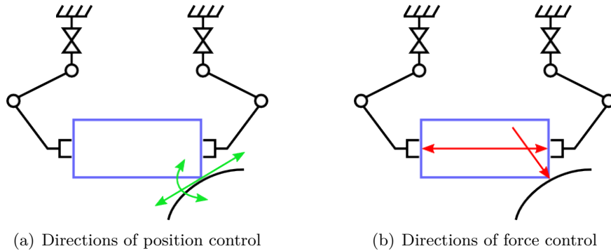
Figure 5.8 – Principle of hybrid force/position control, for manipulators (adapted from T. Yoshikawa 2010)
