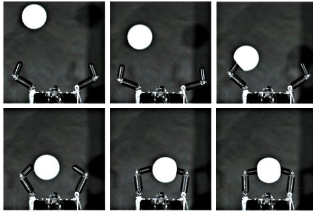
Figure 3.104 – High Speed Multifingered Hand catching a rubber ball in freefall directly into a two-finger fingertip precision grip. The photographs are taken at intervals of 15 ms (i.e. from t = 0 s to t = 0.075 s).
