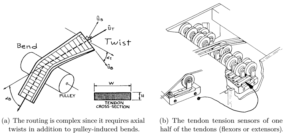
Figure 3.68 – The flat tendons of the Utah/MIT Hand (Jacobsen, Iversen, Knutti, T. Johnson, and Biggers 1986)
