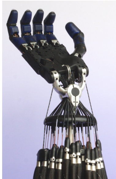
Figure 2.44 – The epitome of tendon-driven robot hands: the Shadow Dextrous Hand, manufactured by the Shadow Robot Company, London, United Kingdom. The joints are driven by tendons actuated by forty pneumatic artificial muscles placed in the forearm.
