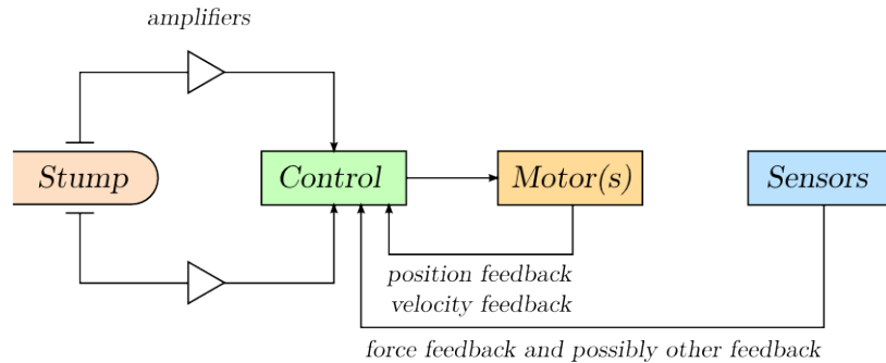
Figure 3.28 – Simplified block diagram of a myoelectric prosthetic hand
