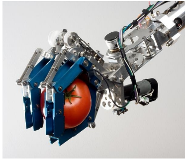
Delft Hand 1 (Meijneke and Wilbers 2009)
