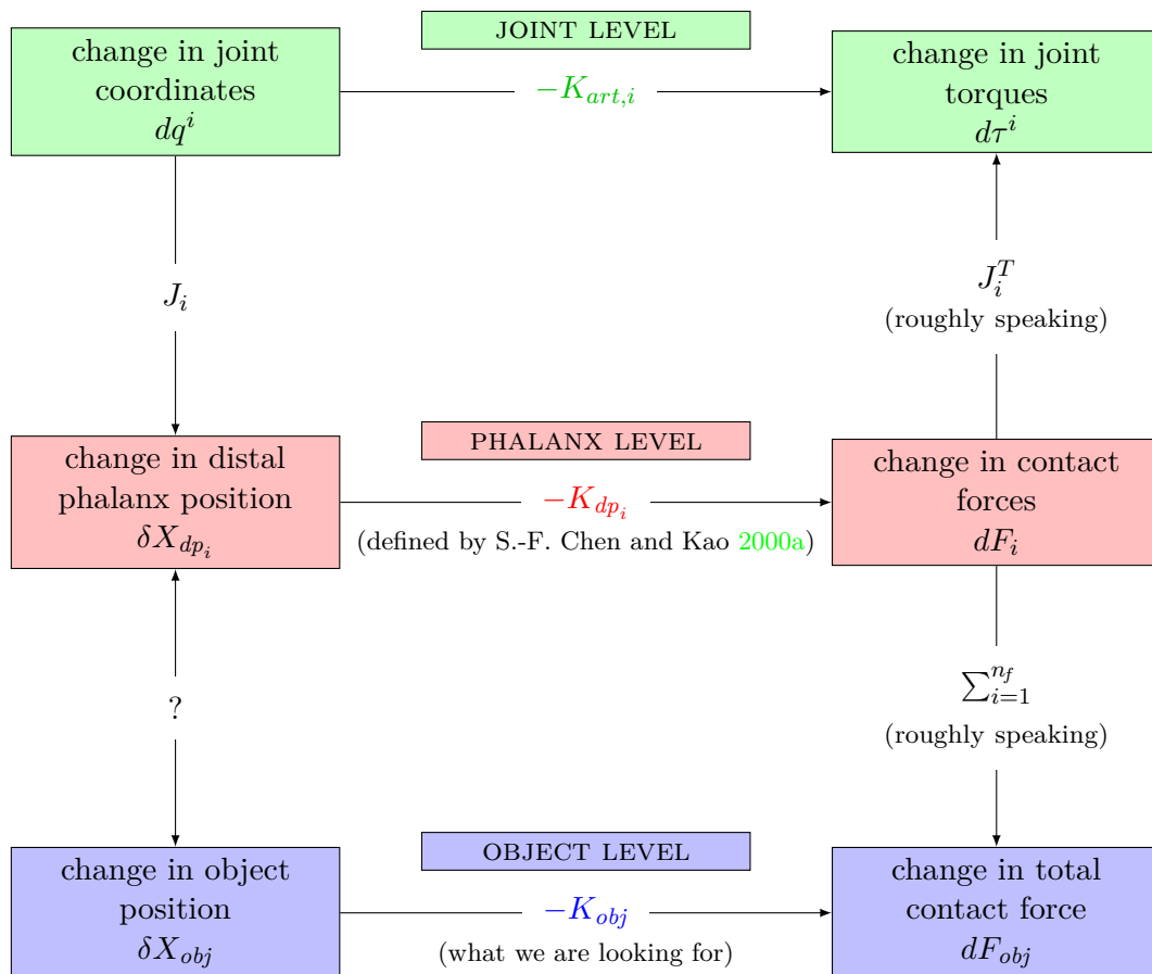
Figure 7.4 – Stiffness mappings at joint, phalanx, and object level. The relationship indicated with a question mark is not trivial to find, contrary to the other relationships in this diagram. We are looking for K_{obj} as a function of K_{dp_i} (and of anything else that will be necessary).
