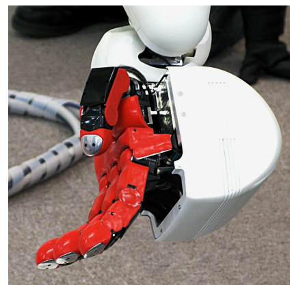
(b) Left hand, side view. Most of the red material is a compliant artificial skin.
