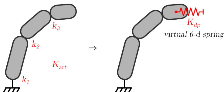
Figure 7.1 – Joint stiffness and cartesian stiffness of a finger
