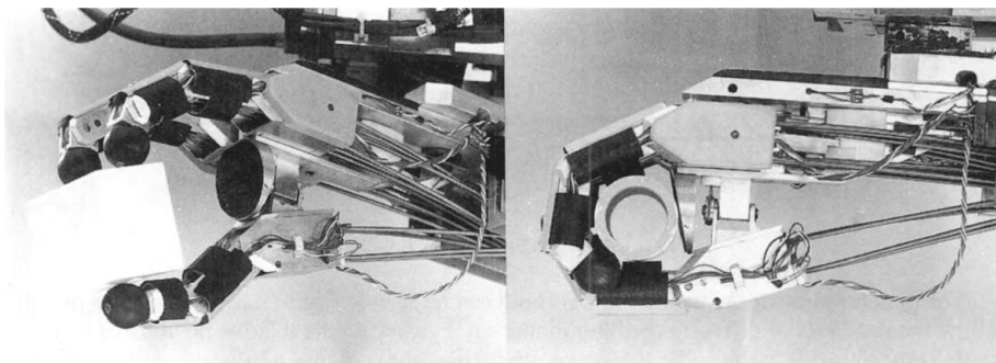
Figure 3.118 – A fingertip precision grip and a whole-hand power grip performed by the UB Hand 1 (1988)
