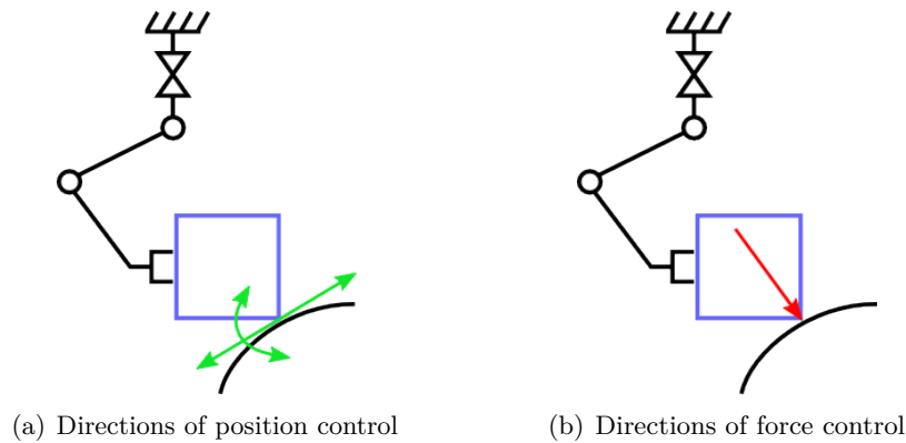
Figure 5.5 – Principle of hybrid force/position control, for a single manipulator (adapted from T. Yoshikawa 2010)
