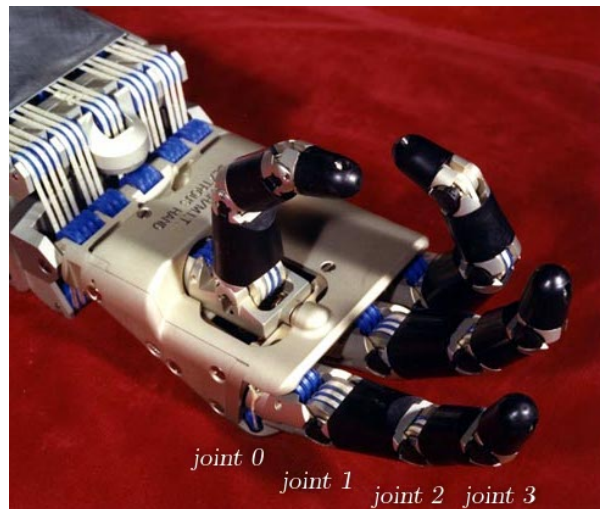
Figure 3.66 – The Utah/MIT Dextrous Hand (1986). The white bands are tendons, the blue rollers are pulleys, the black parts are removable covers.
