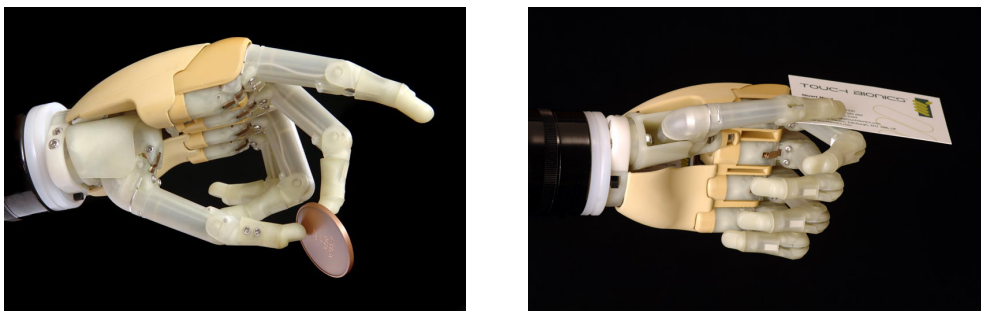
Figure 3.31 – Touch Bionics' i-Limb hand without its cosmetic skin
