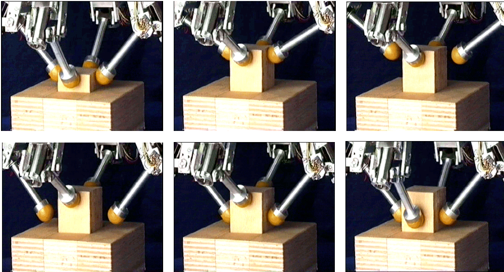
Figure 3.95 – Translation with regrasping: the Karlsruhe Dextrous Hand II pulling a peg out of a hole (Osswald and Wörn 2001)
