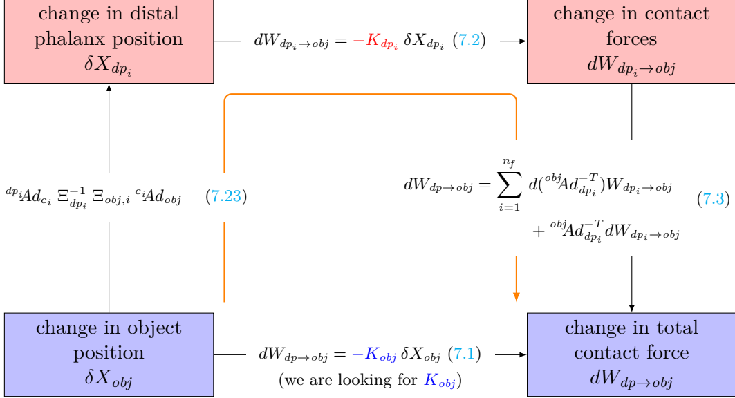
Figure 7.8 – Stiffness mappings in the cartesian space, at phalanx and object levels. Detailed relationships, complete diagram.
