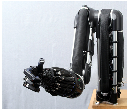
Hand and forearm mounted on a biomorphic arm. The arm uses air muscles too.
