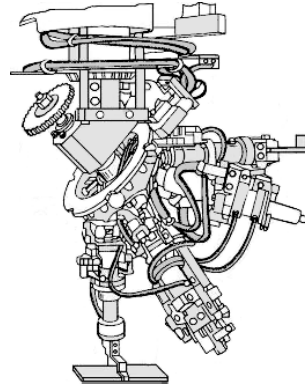
(b) A turret with six separate end effectors, four of which are visible (Monkman, Hesse, Steinmann, and H. Schunk 2004/2007)
