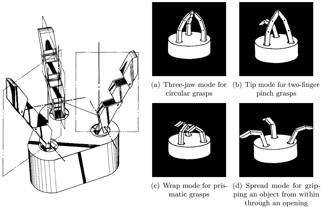
Figure 3.57 – A drawing of Skinner’s three-fingered “multiple prehension manipulator system” and its four prehension modes (1975)
