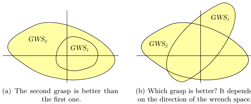
Figure 6.2 – Comparison of grasps by their grasp wrench spaces
