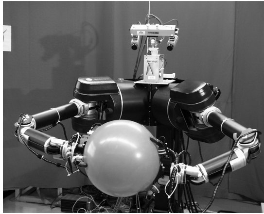
Figure 3.80 – The robot Dexter, at the University of Massachusetts, is a platform for studying bi-manual dexterity. Its limbs are Barrett Arms with Barrett Hands at the end.
