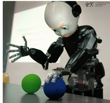
(b) iCub grasps (and learns) various spheres.
