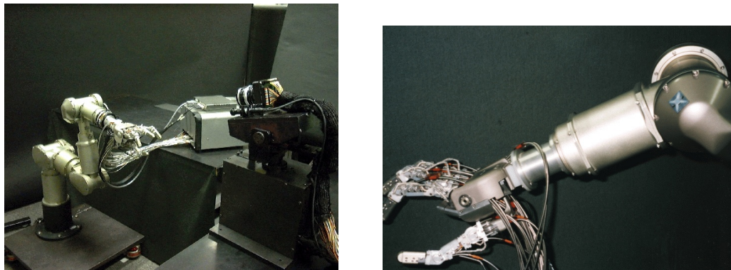
Figure 3.101 – High speed sensory-motor fusion system, University of Tokyo, Ishikawa/Oku Laboratory. On the left: robot arm, multifingered hand, actuator package for the hand, high-speed vision system. On the right: close-up of the hand.
