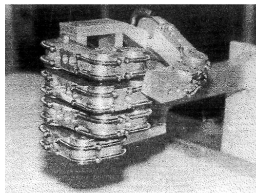
(b) With all the fingers closed. The return springs are visible on the back of the fingers.
