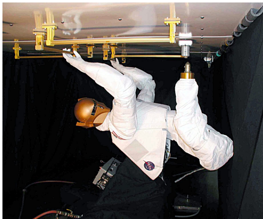
(a) Like astronauts, a spacewalking Robonaut would move around the International Space Station using the external handrails and latch onto the station using the same sockets used by astronauts for foot restraint. It is shown here mounted on an air-bearing sled simulating zero-gravity, in 2004.
