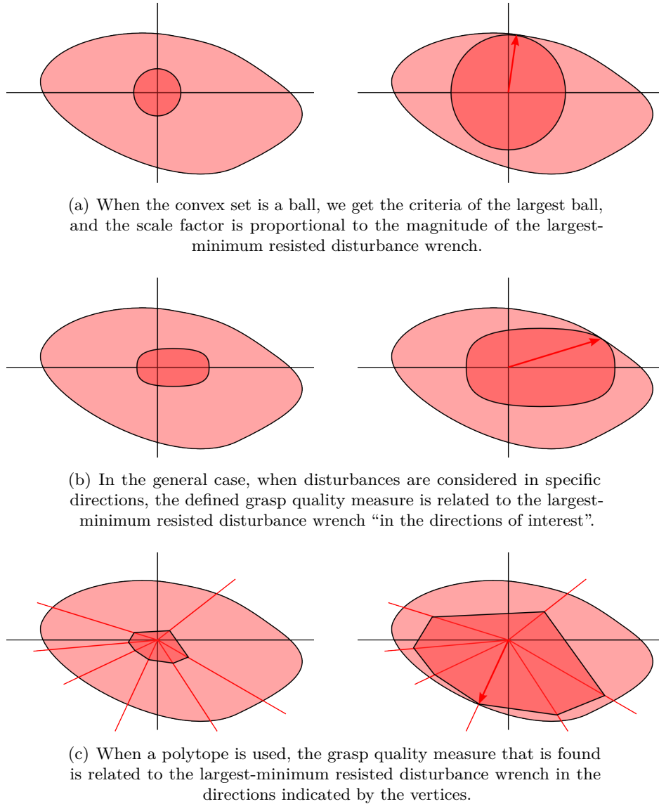
Figure 6.10 – A variation of the criteria of the largest ball. The quality measure is the scale factor between the chosen convex set, on the left, and the maximal homothetic one, on the right.
