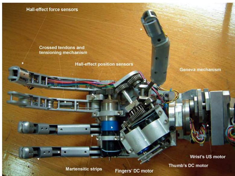
Figure 3.37 – The Manus Hand (Pons, Rocon, Ceres, Reynaerts, Saro, Levin, and Moorleghem 2004)
