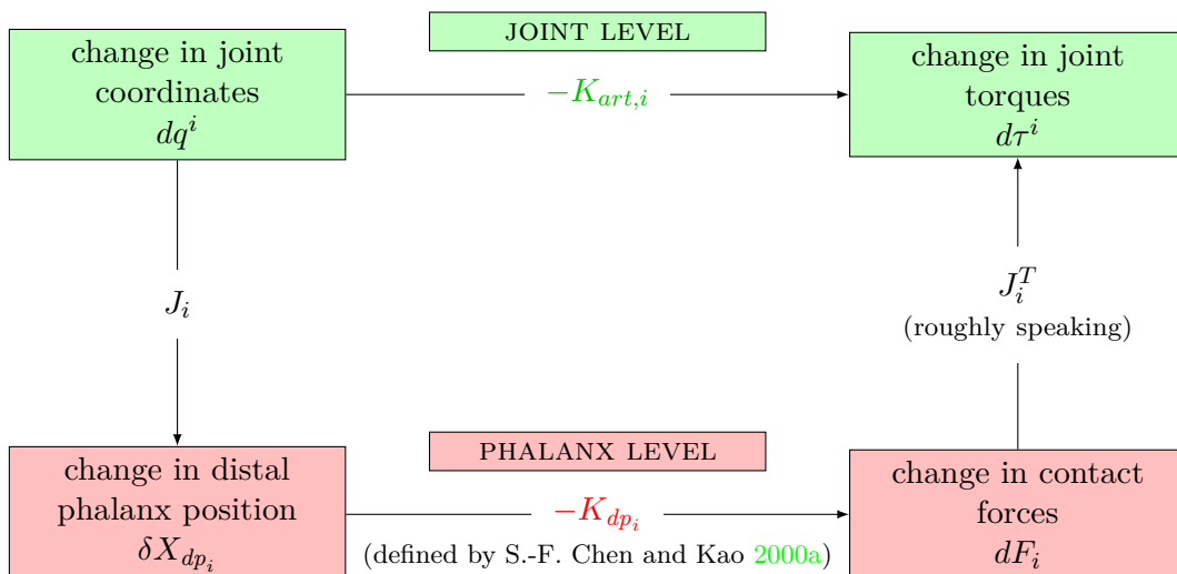
Figure 7.2 – Stiffness mappings at joint and phalanx level, for the i -th finger. An arrow from a to b with the matrix M on it means b = Ma . “Roughly speaking” means that there is more to it than just a matrix (in the present case, \tau^i = J_i^T F_i \Rightarrow d\tau^i = J_i^T dF_i + d(J_i^T)F_i ).
