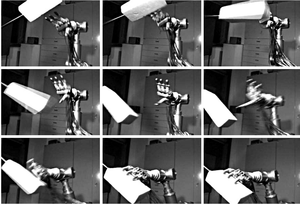
Figure 3.102 – Grasping an object with the high-speed sensory-motor fusion system (M. Ishikawa, Komuro, Namiki, and Ishii 1999). The photographs are taken at intervals of 0.1 s (i.e. from t = 0 s to t = 0.9 s).
