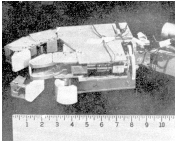
Figure 3.56 – Crossley and Umholtz’s three-fingered hand for teleoperated grasping in space (1975)
