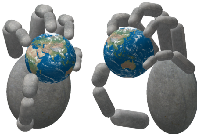
Figure 5.1 – A computer-simulated model of a five-fingered robot hand (front and side views). The phalanges are pill-shaped and the palm is simply a flat ellipsoid: from a control perspective, their geometry doesn't count as much as their dynamics, as long as the contacts between the hand and the object are limited to a few point contacts.
