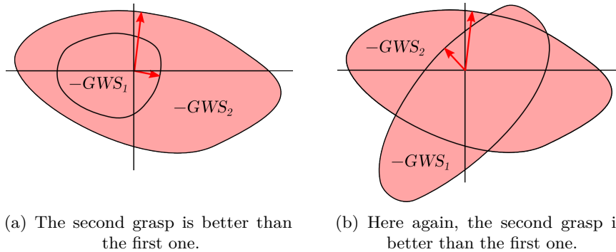
Figure 6.5 – Comparison of grasps by their largest-minimum resisted disturbance wrenches
