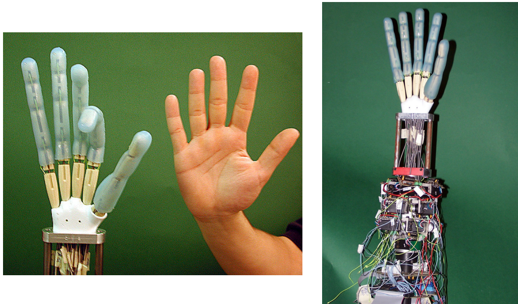
Figure 3.120 – The UB Hand 3 (2005). To keep the hand simple, the four fingers are identical, hence the oversized little finger.
