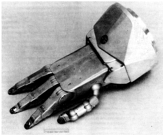
(b) Jau/JPL Hand
