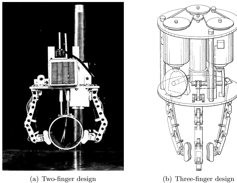
Figure 3.58 – Rovetta’s “multipurpose mechanical hand” (1977, 1980)
