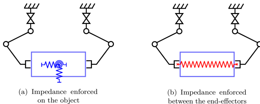
Figure 5.9 – Principle of compliance control and impedance control, for manipulators, with only the virtual spring elements depicted (adapted from T. Yoshikawa 2010)
