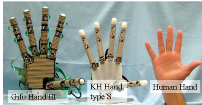
Figure 3.134 – Size comparison between Gifu Hand III, KH Hand type S, and human hand. All the wires in the robotic hands run along the back, so as not to hinder finger motion.
