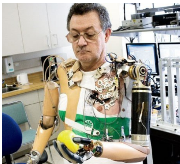
Figure 3.52 – Bilateral shoulder amputee Jesse Sullivan, the first tester of targeted muscle reinnervation surgery, operates an early version of the DARPA prosthetic arm system made by Johns Hopkins University Applied Physics Laboratory (his right arm is a more classic powered split hook). The electrode array on his chest indicates a pattern-recognition-based control.
