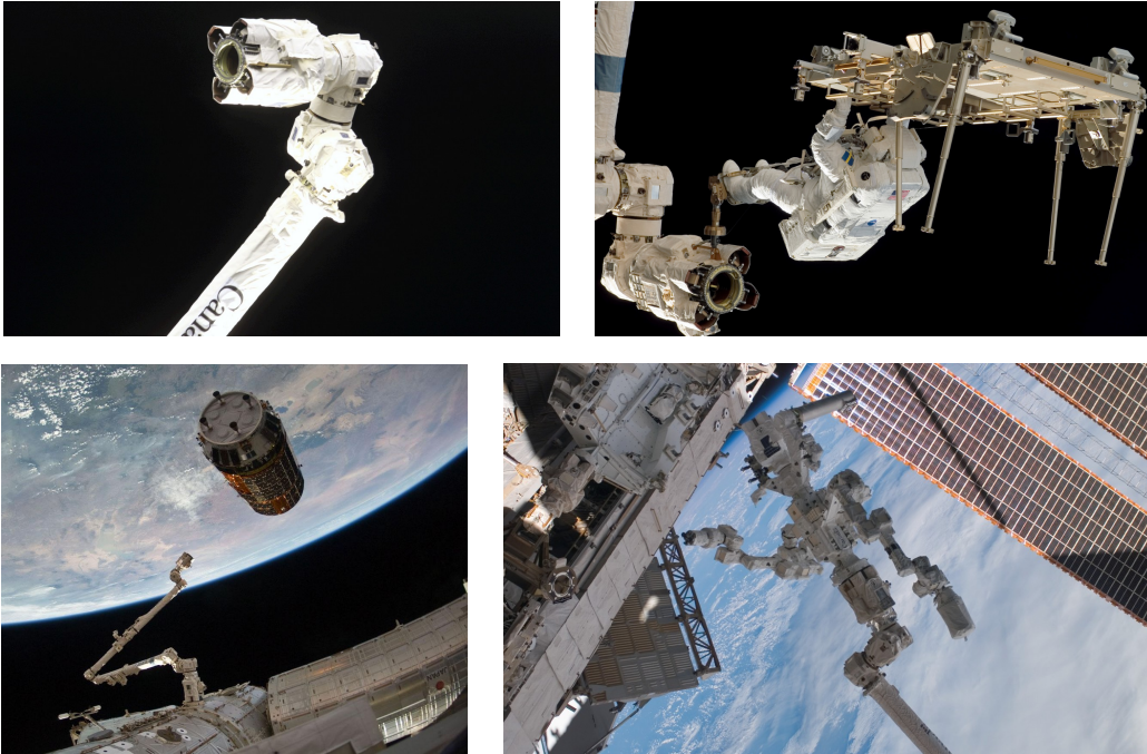
(a) The previous version of this arm, the smaller and lighter Canadarm, is used on space shuttles since 1981, chiefly for deployment of payloads from the cargo bay and inspection of the shuttle's surface. The new version was launched in 2001 and used to build the station. Its missions now include station maintenance, replacement of plug-in equipment, assistance in docking and unloading the shuttle, moving of payloads and astronauts (top right), and many more. Its end effector is able to capture free-flying unmanned spacecrafts (bottom left). A set of two smaller robotic arms, called Dextre, complements the arm when the task needs other end effectors (bottom right).
