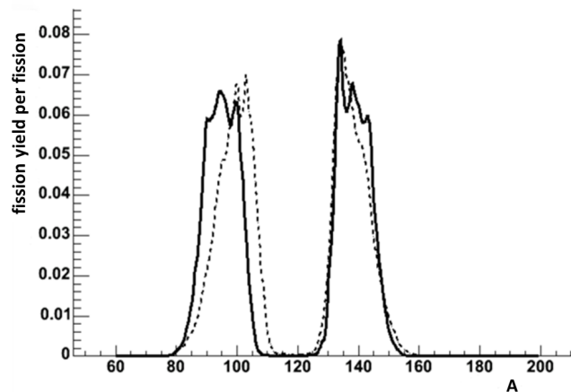
FIGURE 1 – Discrepancies in the fission products distributions for 235 U and 239 Pu ( database : ENDF/B 6.8).
