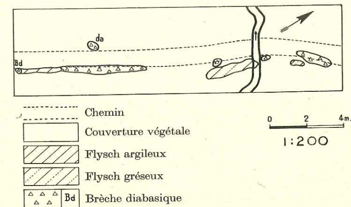
Fig. 19. Mont Caly. da: diabase amygdalaire.
