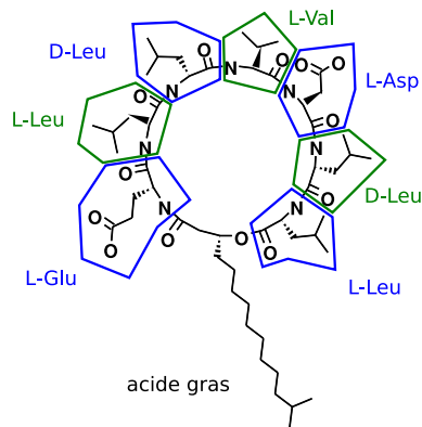
FIG. 1.9 – Structure de la surfactine
