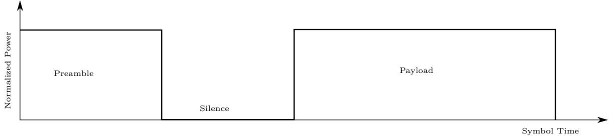
Figure 2.4: Frame Structure.
