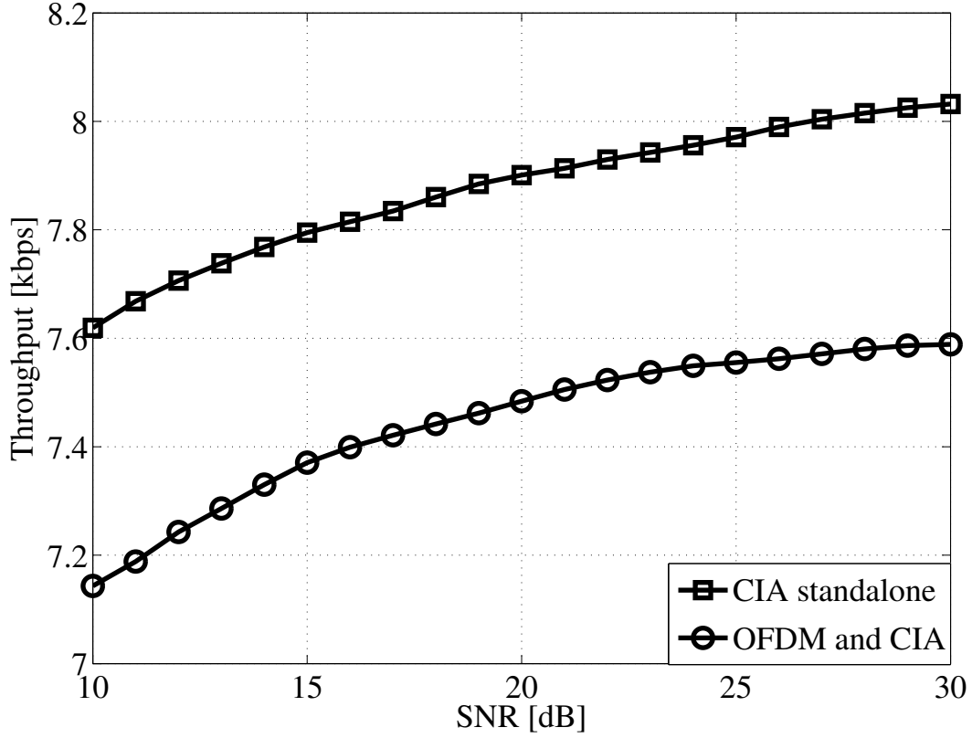
Figure 8.12: Throughput of the secondary transmission at CT for both standalone CIA and hybrid (OFDM and CIA) transmissions.
