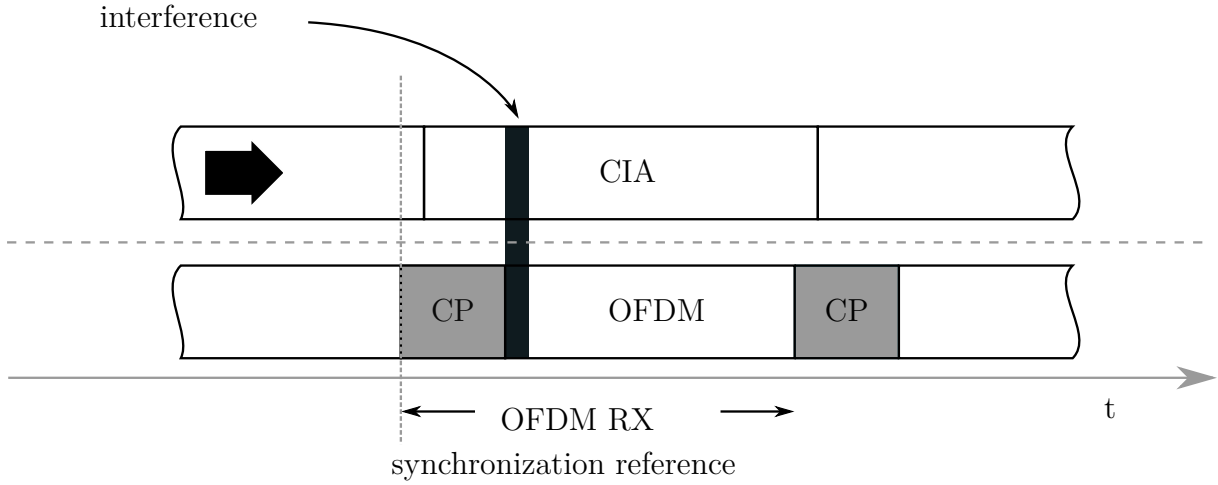
Figure 5.8: Wrong synchronization: CIA signal arriving at the OFDM receiver after the OFDM signal.
