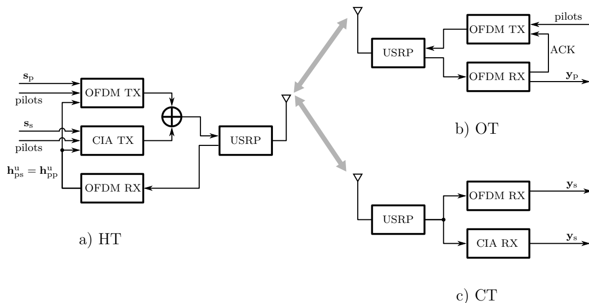
FIGURE 5 – Structure des Transceivers.
