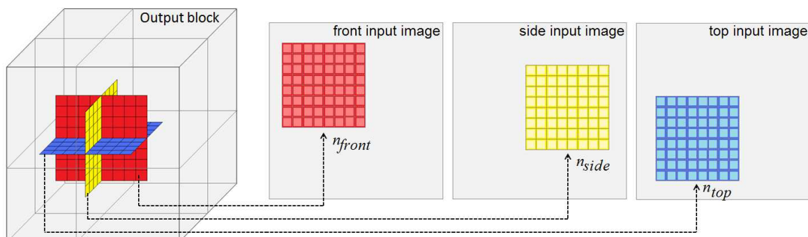
Figure 3.5 – Principle of non-parametric synthesis: extract three neighbourhoods in the output block (front view, side view and top view), search the best three neighbourhoods in the input image, and combine their corresponding input pixel values to modify the output voxel.
