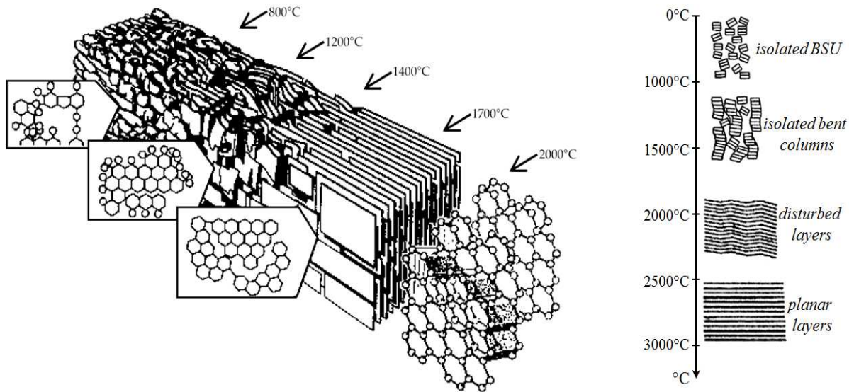
Figure 6.5 – Illustrating the carbon structure evolution with the temperature (on the left) and the crystallites alignment during graphitization stages (on the right) [Obe89].
