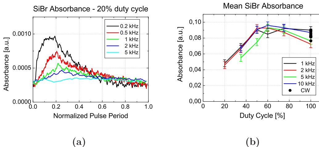
Figure 4.3.: (a) Time-resolved SiBr absorption measurements for different frequencies at a duty cycle of 20% and (b) time-averaged absorption for different duty cycles at various frequencies above 1 kHz (HBr/O 2 , 200 sccm/5 sccm, 20 mTorr, 750 W source power, 200 W bias power).
