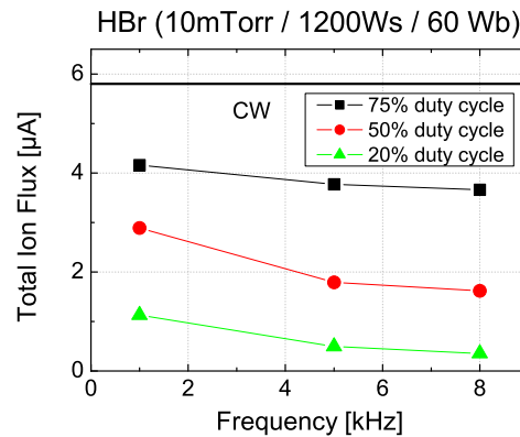
Figure 4.10.: Total ion flux for pulsed HBr plasma conditions (200 sccm, 10 mTorr, 1200 W source power, 60 W bias power) from RFA measurements.
