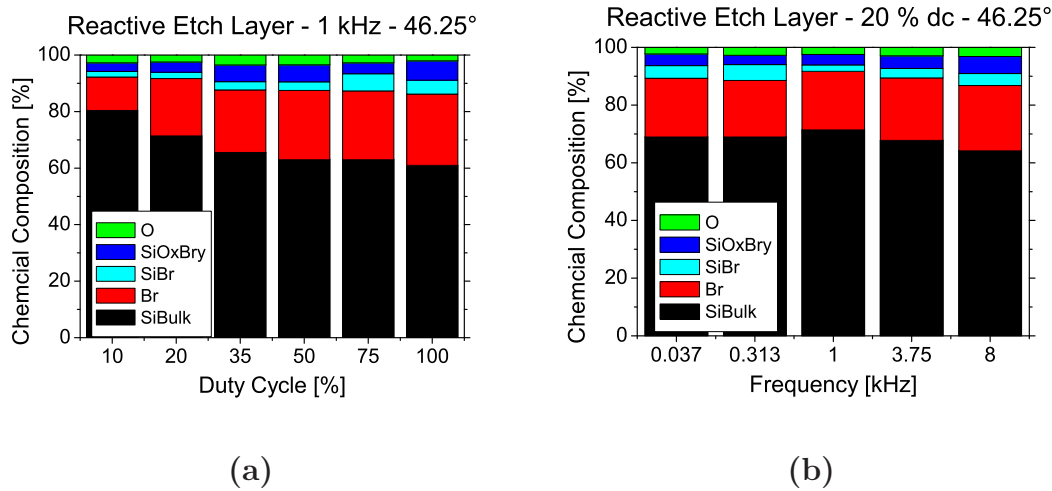
Figure 4.11.: (a) Chemical composition of the XPS signal (at 46.25°) from the reactive etch layer for different duty cycles (at 1 kHz) and (b) frequencies (at 20% duty cycle). Standard plasma etch conditions (200 sccm HBr/5 sccm O 2 , 20 mTorr, 750 W source power, 200 W bias power).
