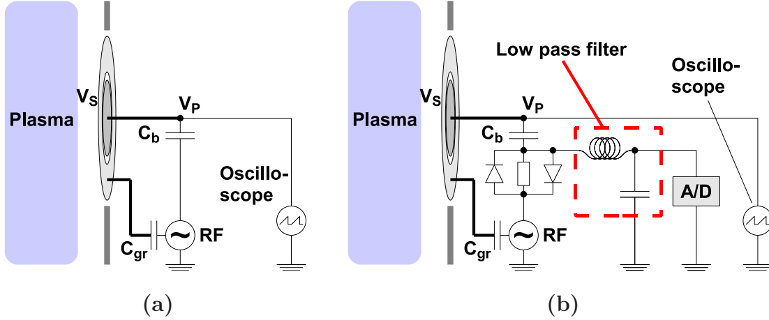
Figure 2.11.: Sketch of the ion flux probe with (a) traditional and (b) newly developed direct current measurement system.
