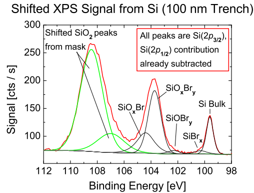
Figure 2.18.: XPS signal from Si: the signal from the oxide mask is shifted to the left towards higher binding energies due to the secondary electrons produced from an electron beam with an energy of 300 eV.
