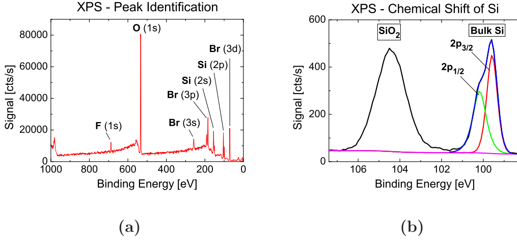
Figure 2.16.: (a) Overview spectrum to show identification of elements. (b) Spectrum of a thin layer of SiO 2 on the silicon bulk to show the chemical shift and the spin orbital splitting.
