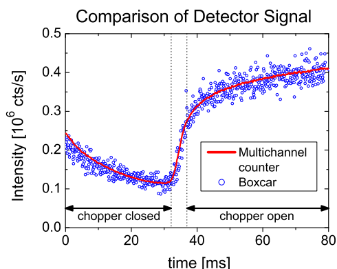
Figure 2.5.: Comparison between detector signals: boxcar vs. multi-channel pulse counter.
