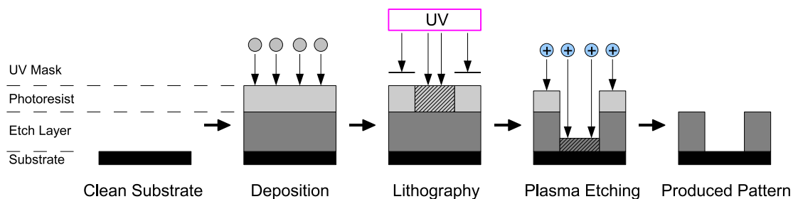
Figure 1.1.: Sketch of the main microelectronics fabrication steps: deposition, lithography and plasma etching. A repeated sequence of these processes can be used to fabricate complicated patterns on the silicon substrate, e. g. for transistors or interconnecting lines.
