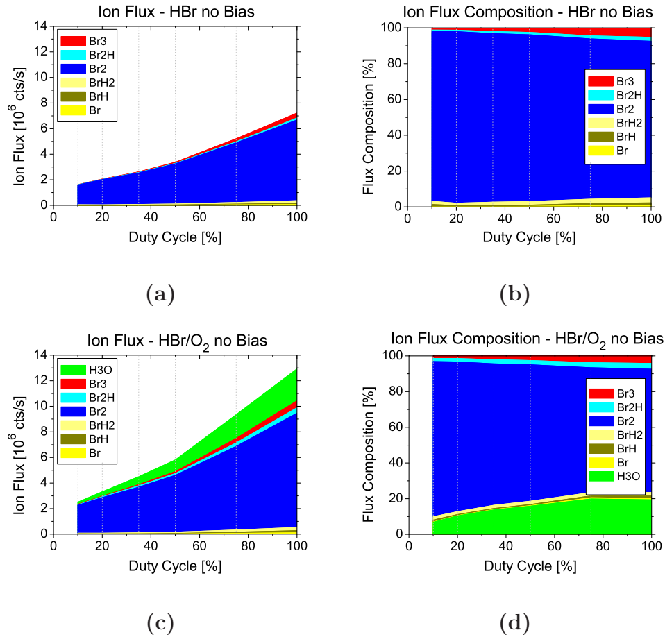
Figure 3.10.: Total ion flux ((a),(c)) and ion flux composition ((b),(d)) for HBr and HBr/ \text{O}_2 , respectively (200 sccm/5 sccm, 10 mTorr, 750 W source power).
