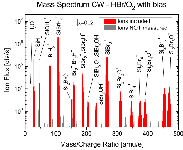
Figure 4.4.: Ion mass spectra in CW mode for an HBr/O 2 plasma (200 sccm/5 sccm, 10 mTorr, 750 W source power, 200 W bias power).
