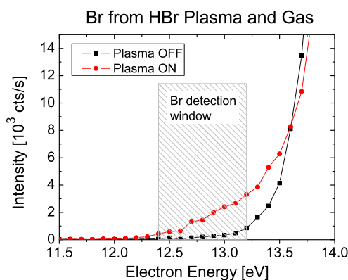
Figure 2.6.: Dissociative ionization ( Plasma OFF ) and combined dissociative/direct ionization ( Plasma ON ) of Br from an HBr plasma/gas.
