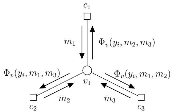
Figure 1.3: Update of the messages at a variable node with d_v = 3 .
