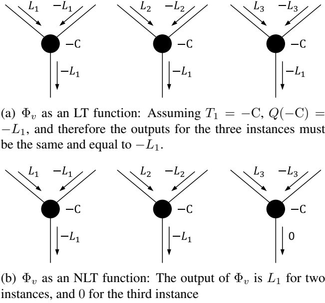
Figure 2.3: Comparison of possible outputs of \Phi_v between LT and NLT functions for three different instances of message-passing.
