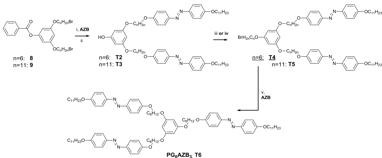
Scheme 13 Synthesis of phloroglucinol based dendrons: HO-PG 6 AZB 2 ( T2 ) and HO-PG 11 AZB 2 ( T3 ) and homolithic trimer ( T6 ) Reagents and conditions: (i) K 2 CO 3 , DMF or THF, reflux, (ii) KOH, THF/H 2 O, reflux, (iii) n=11: BrC 11 H 22 Br, K 2 CO 3 , THF, reflux, (iv) BrC 6 H 12 Br, K 2 CO 3 , 18-crown-6, THF, reflux, (v) K 2 CO 3 , DMF, 70°C
