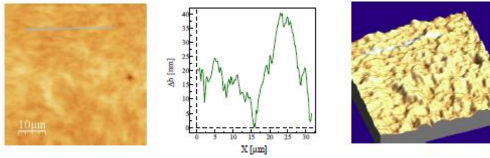
Figure 69 Views 2D (left) and 3D (right) of AFM scans (50x50 \mu\text{m} ), and the surface profile (middle) of the film surface of the PG 6 OCB 2 AZB before diffraction grating recording process.
