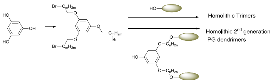
Scheme 3 General synthetic scheme of homolitic trimers and dendrimers using tribromide derivatives
