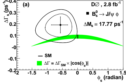
FIGURE 6.18: D\bar{0} confidence level contours in the \Delta\Gamma_s - \phi_s plane. The curves correspond to expected 68% C.L. (dashed) and 90% (solid). The green band corresponds to the Equation \Delta\Gamma_s = \Delta\Gamma_s^{SM} \cdot |\cos(\phi_s)| .
