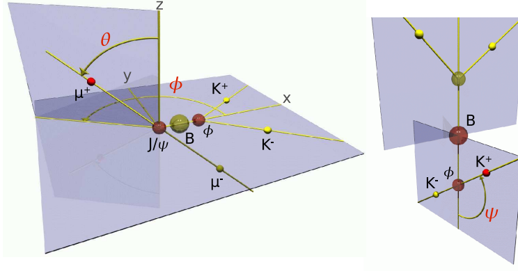
FIGURE 5.1: Transversity basis and angles definition for the B_s^0 \rightarrow J/\psi(\rightarrow \mu^+\mu^-)\phi(\rightarrow K^+K^-) decay mode.
