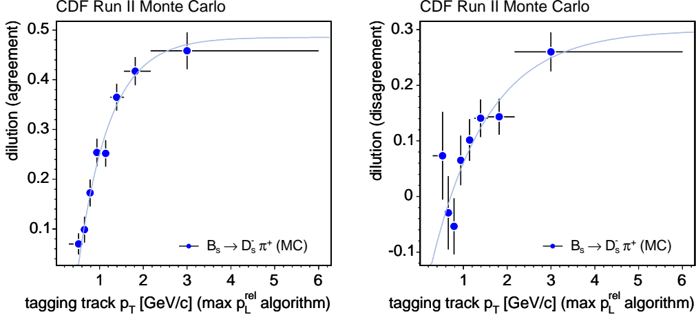
FIGURE 4.16: Dilution parametrization as a function of transverse momentum p_T of the flavor tagging candidate, for the max p_L^{rel} algorithm. The plot on the left contains all the cases when only one tagging candidate or more than one tagging candidate with the same charge are available. The right plot contains all the cases when more than one tagging candidate is available but they disagree in charge.
