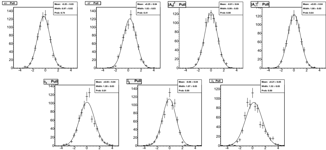
FIGURE 5.13: Signal pulls distributions for the B_s^0 \rightarrow J/\psi\phi angular analysis with 10,000 events, input \beta_s = 0.05 .
