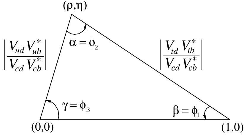
FIGURE 1.1: A sketch of the Unitarity Triangle.
