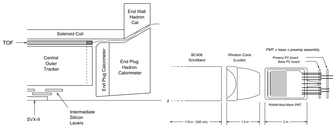
FIGURE 2.11: The Time Of Flight detector. On the left, the location of TOF is shown in a side view of CDF II. On the right, the arrangement of the scintillator, Winston cone and photomultiplier assembly. The Winston cone optimizes the optical coupling between the scintillator and the photomultiplier.
