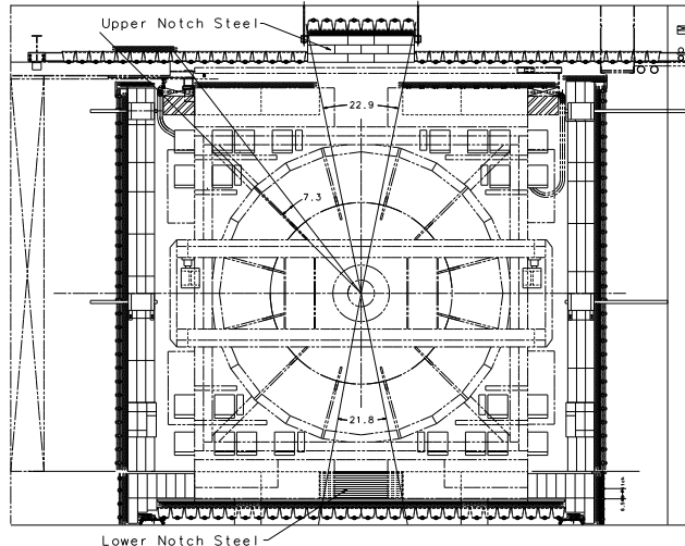
FIGURE 2.15: Central Muon uPgrade CMP. In this x - y section of the CDF detector, the CMP forms a rectangular box (dark shaded area) which surrounds the other parts of the CDF detector.
