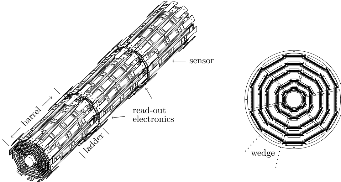
FIGURE 2.6: The Silicon Vertex detector SVXII. An illustration of the three instrumented barrels of SVXII (left) and a cross-sectional view of a barrel in the r - \varphi plane.
