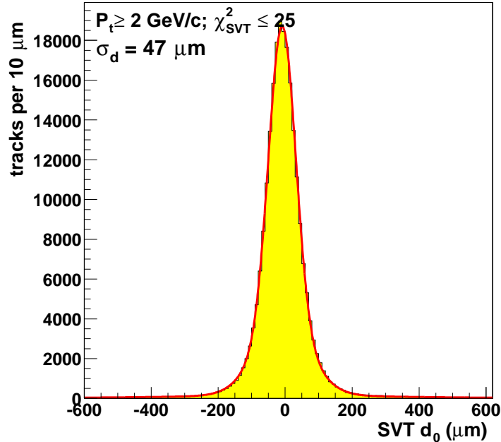
FIGURE 2.20: Impact parameter resolution as measured by SVT. The distribution includes the effect of the beam size. The SVT measures impact parameters with a r.m.s. width of 35 \mu\text{m} .
