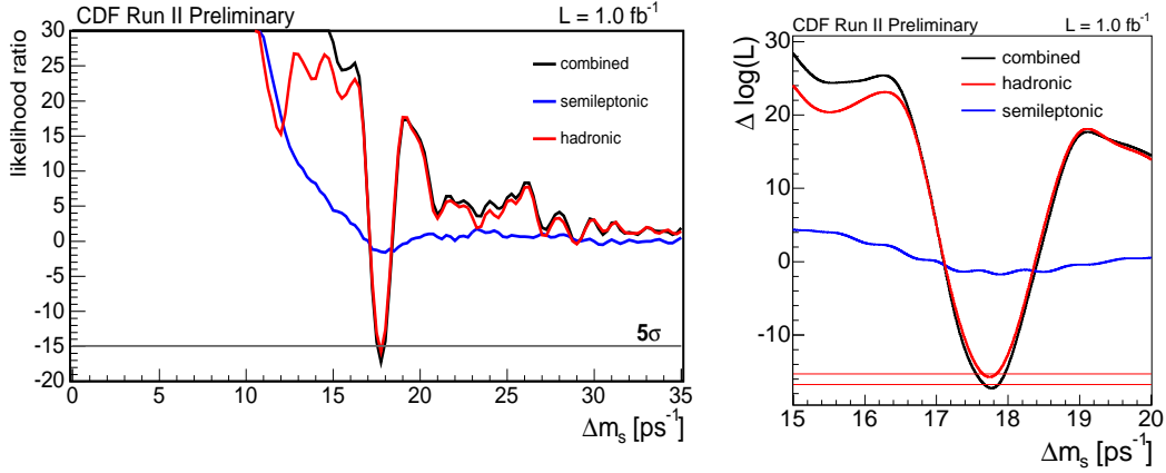
FIGURE 6.5: Likelihood profile: likelihood ratio as a function of \Delta m_s (left) with a zoom-in of the [15, 20] \text{ps}^{-1} region. The contribution of hadronic (red), semileptonic (blue) and their combination (black) are shown separately.
