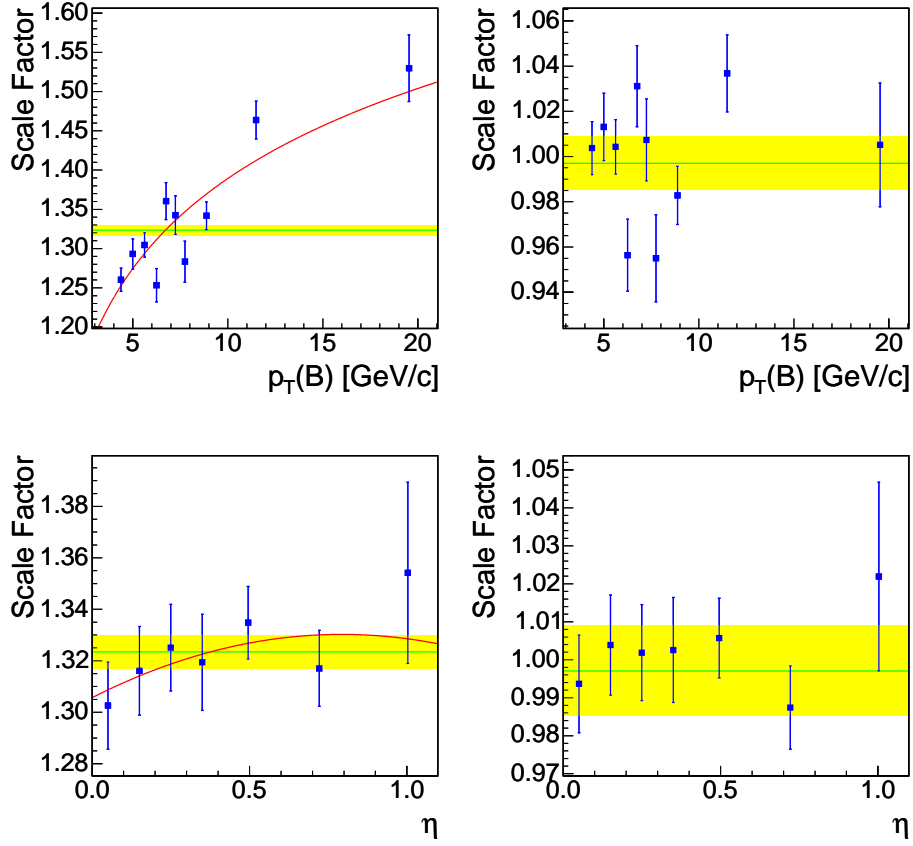
FIGURE 4.26: Proper decay time scale factor dependence on different decay variables, before (left) and after (right) tuning. In order, from top to bottom: p_T(B_s^0) , \eta(B_s^0) .
