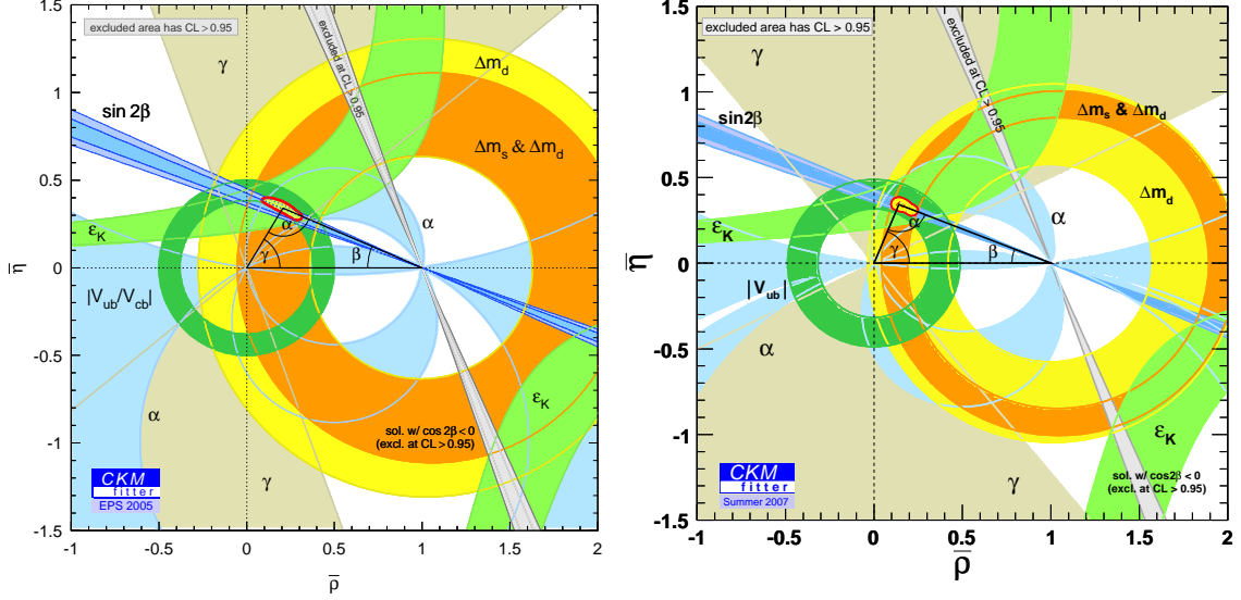
FIGURE 6.9: CKM fit of the Unitarity Triangle at EPS2005 (left) compared with the most recent one, which includes the CDF observation (right).
