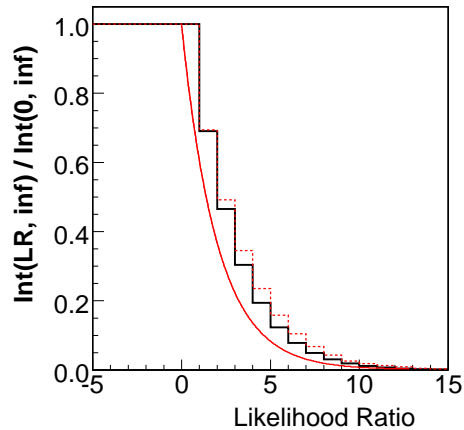
FIGURE 6.20: Likelihood ratio distributions used as reference to correct the likelihood ratio obtained on data assuming the parabolic behaviour of the likelihood. The continuous red line represents the 2-degrees-of-freedom \chi^2 distribution compared to the nominal Feldman-Cousins (black line) and the Feldman-Cousins with the correction due to the nuisance parameters variation (dashed red line).
