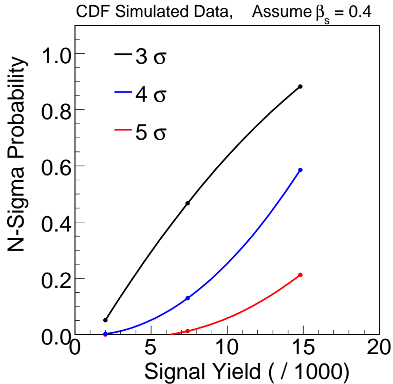
FIGURE 7.18: Probabilities to observe a 3, 4, 5 \sigma (s) effect, if \beta_s = 0.4 rad, as a function of the luminosity (top) and as a function of the yield of data (bottom). The N-sigma probability curves assumes the same data taking efficiency a no improvements in the analysis.
