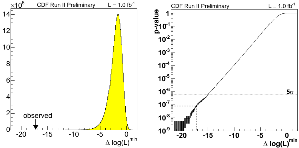
FIGURE 6.6: Distribution of the \Lambda_{min} obtained from the randomized data(left) and p -value as a function of the \Lambda_{min} , which is the cumulative of the distribution of \Lambda_{min} shown on the left.
