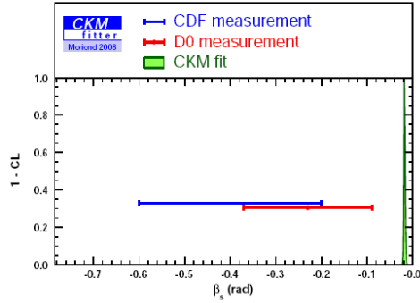
FIGURE 6.19: Comparison of the CDF and D\bar{0} results as presented at the conference Moriond EWK 08 by the CKM fitter collaboration. The blue line corresponds to the CDF Feldman-Cousins one-dimensional confidence region when all the constraints on \Gamma_{12} , \delta_{\parallel} , \delta_{\perp} and B^0 width. The red line corresponds to the D\bar{0} result \phi_s = -0.26 \pm 0.14 obtained when \Delta\Gamma_s is constrained by the expected relation \Delta\Gamma_s^{SM} \cdot \cos(\phi_s) . The green distribution corresponds to the SM expectation for the CKM fit \beta_s = -0.0183_{-0.0008}^{+0.0009} rad. In the CKM collaboration the nomenclature adopted is \beta_s^{CKM} = -\beta_s^{CDF} = \phi_s^{D\bar{0}}/2 .
