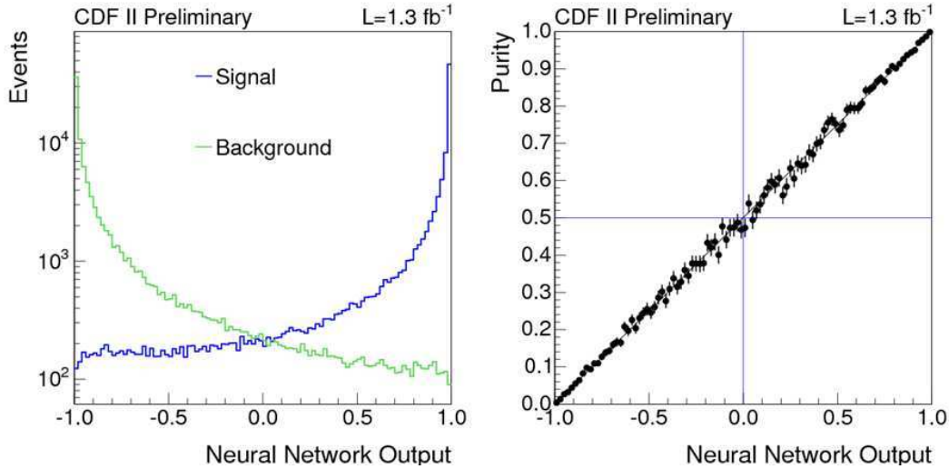
FIGURE 7.3: Left: Neural Network output distributions for simulated B 0 meson reconstructed with the correct mass assignment for the kaon and pion produced in the K *0 decay and treated as signal (blue line) and for the same simulated events but reconstructed with the wrong mass assignment as background (green line). Right: purity of the training sample as a function of the swap suppression Neural Network output.
