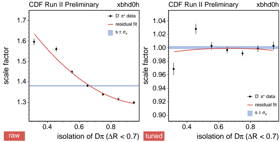
FIGURE 4.6: Scale factor dependence before (left) and after (right) parametrization for the isolation variable for the D\pi topology.
