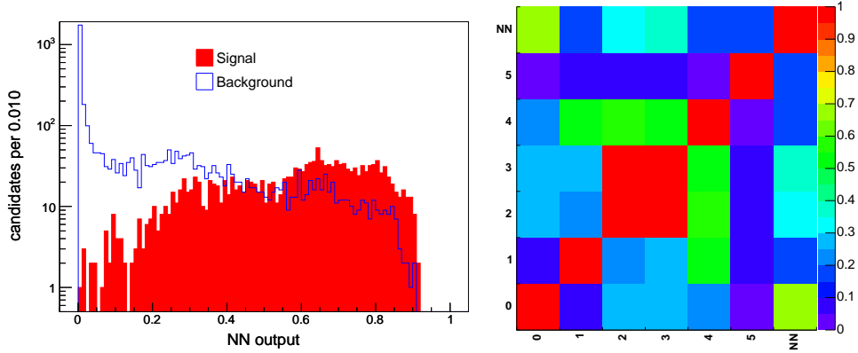
FIGURE 4.19: Neural Network distributions. Left: distribution of the ANN output for signal and background. Right: distribution of the correlations among the input variables; the number from 0 to 6 identify CLL, p_T , p_T^{rel} , p_L^{rel} , \Delta R and the Boolean variable. The training is performed on PYTHIA-MC sample of B_s^0 \rightarrow D_s^- \pi^+ , D_s^- \rightarrow \phi \pi^- decay mode candidates.
